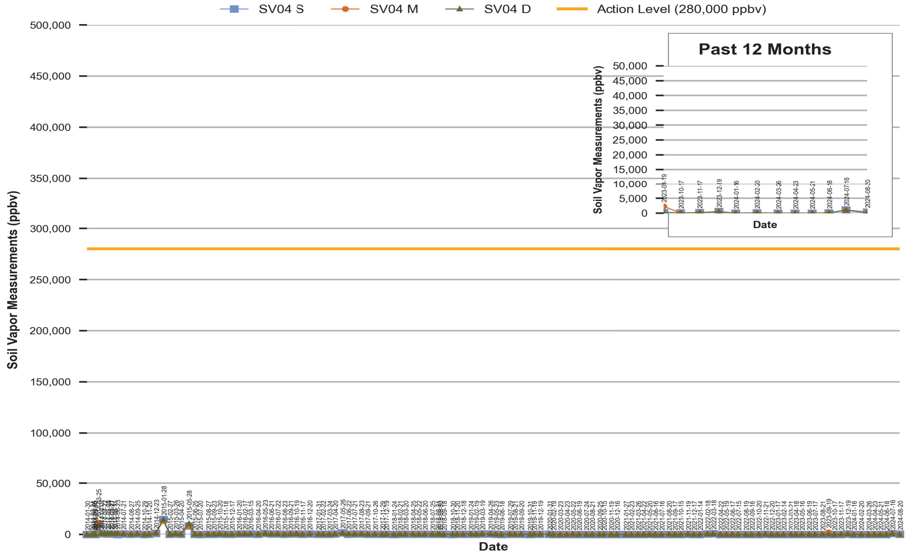
Figure 3 Red Hill - Tank 04 (F-24) Soil Vapor Measurements (Jan 2014 Through Aug 2024)
