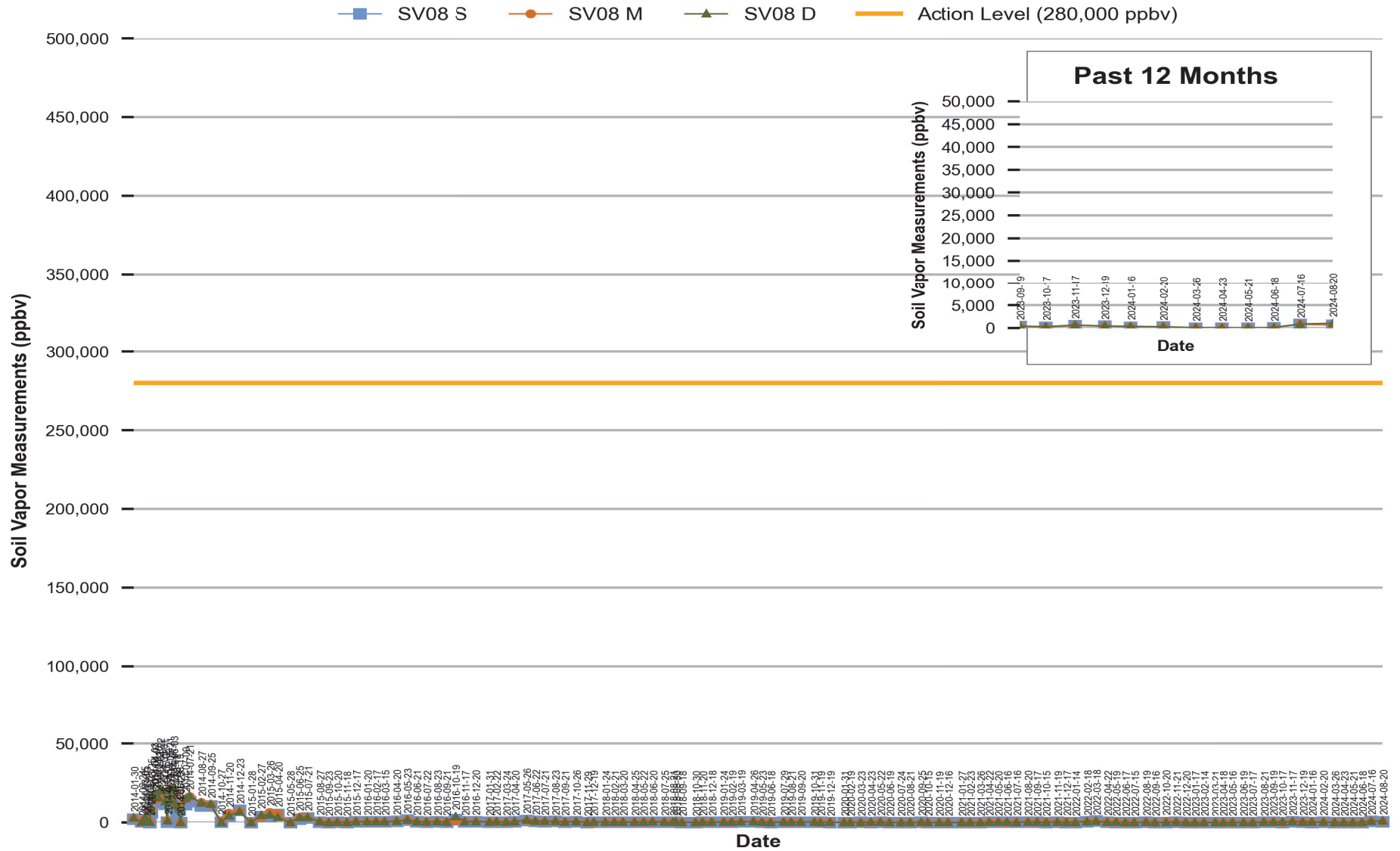
Figure 7 Red Hill - Tank 08 (JP-5) Soil Vapor Measurements (Jan 2014 Through Aug 2024)
