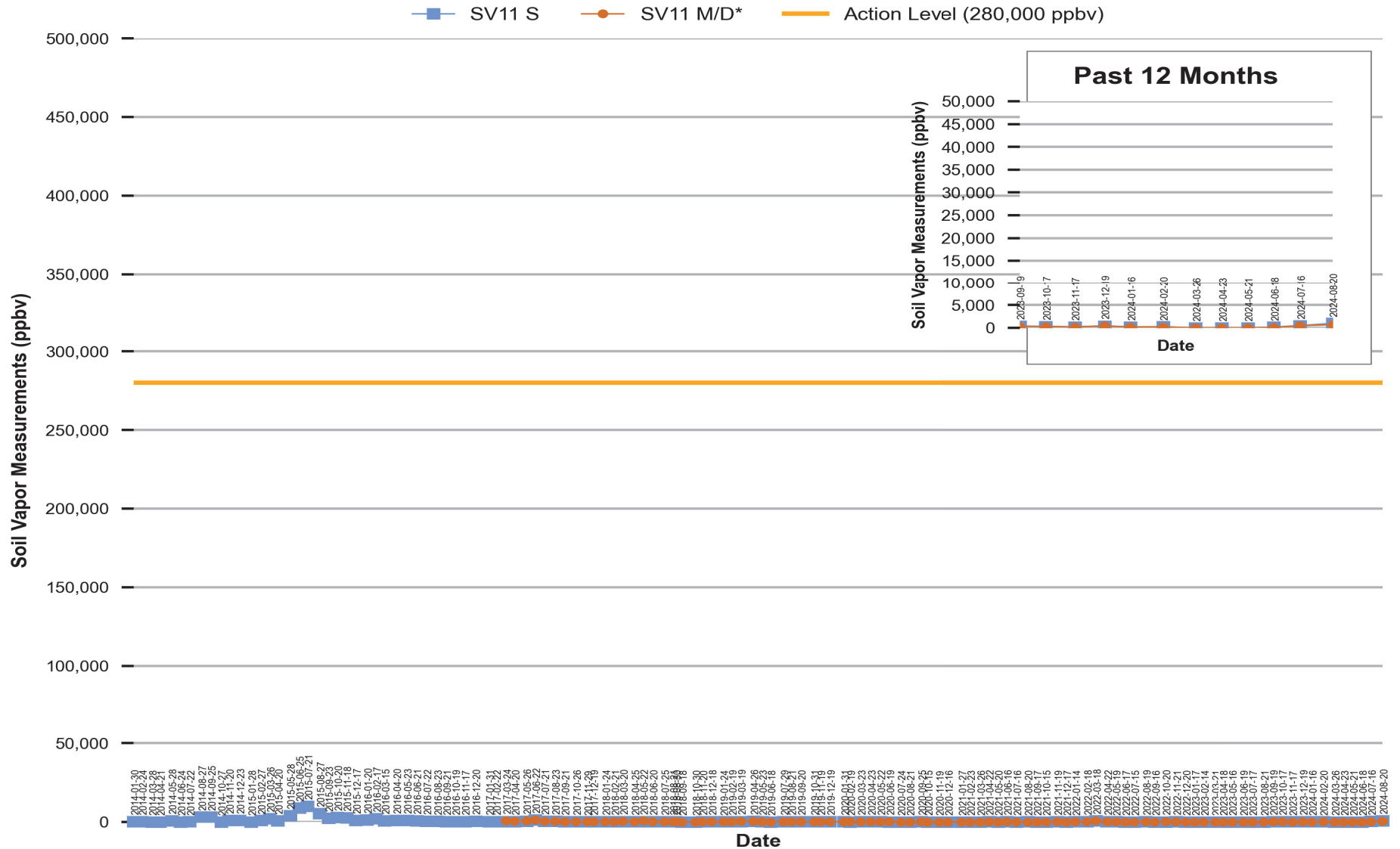
Figure 10 Red Hill - Tank 11 (JP-5) Soil Vapor Measurements (Jan 2014 Through Aug 2024)
