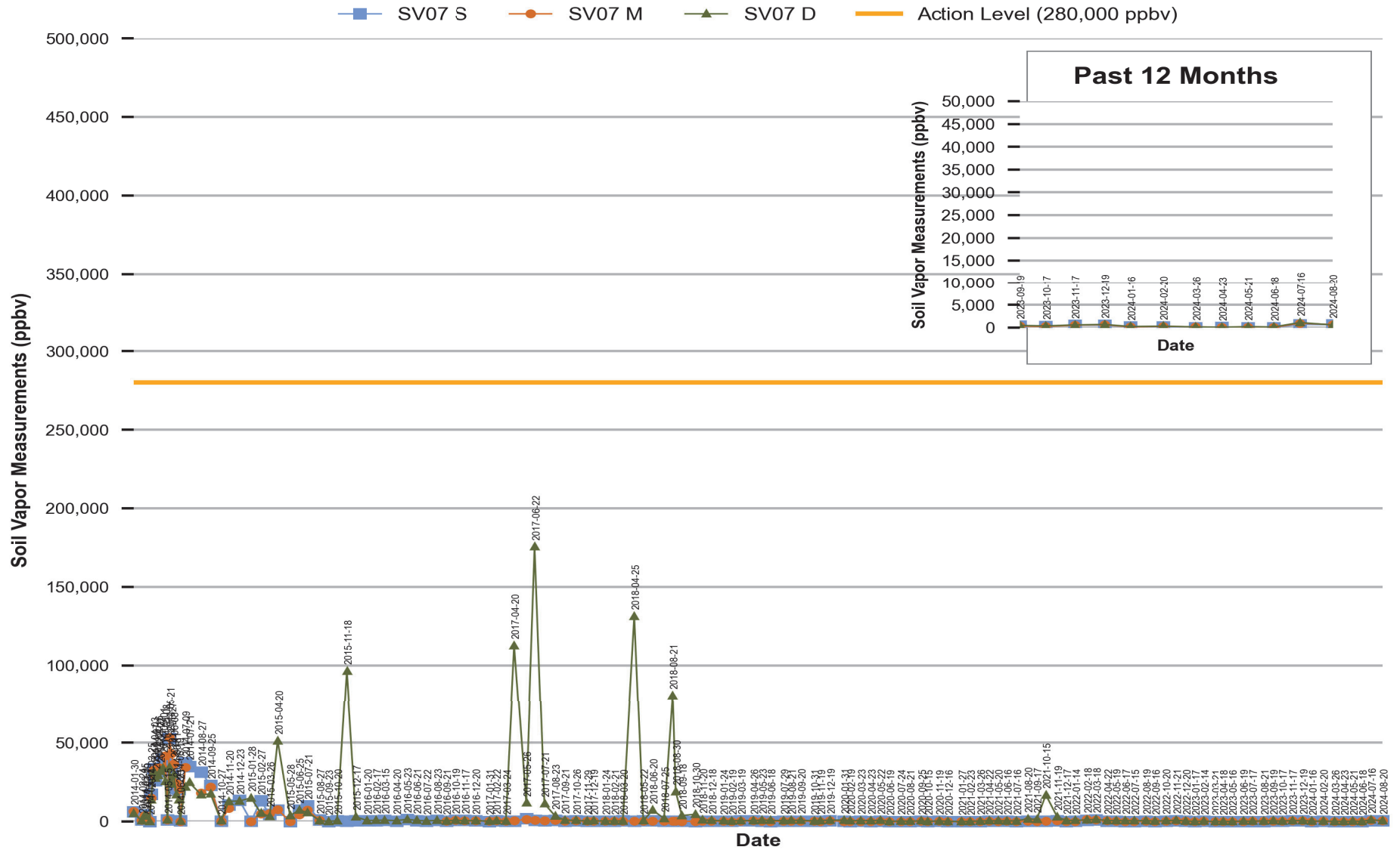
Figure 6 Red Hill - Tank 07 (JP-5) Soil Vapor Measurements (Jan 2014 Through Aug 2024)
