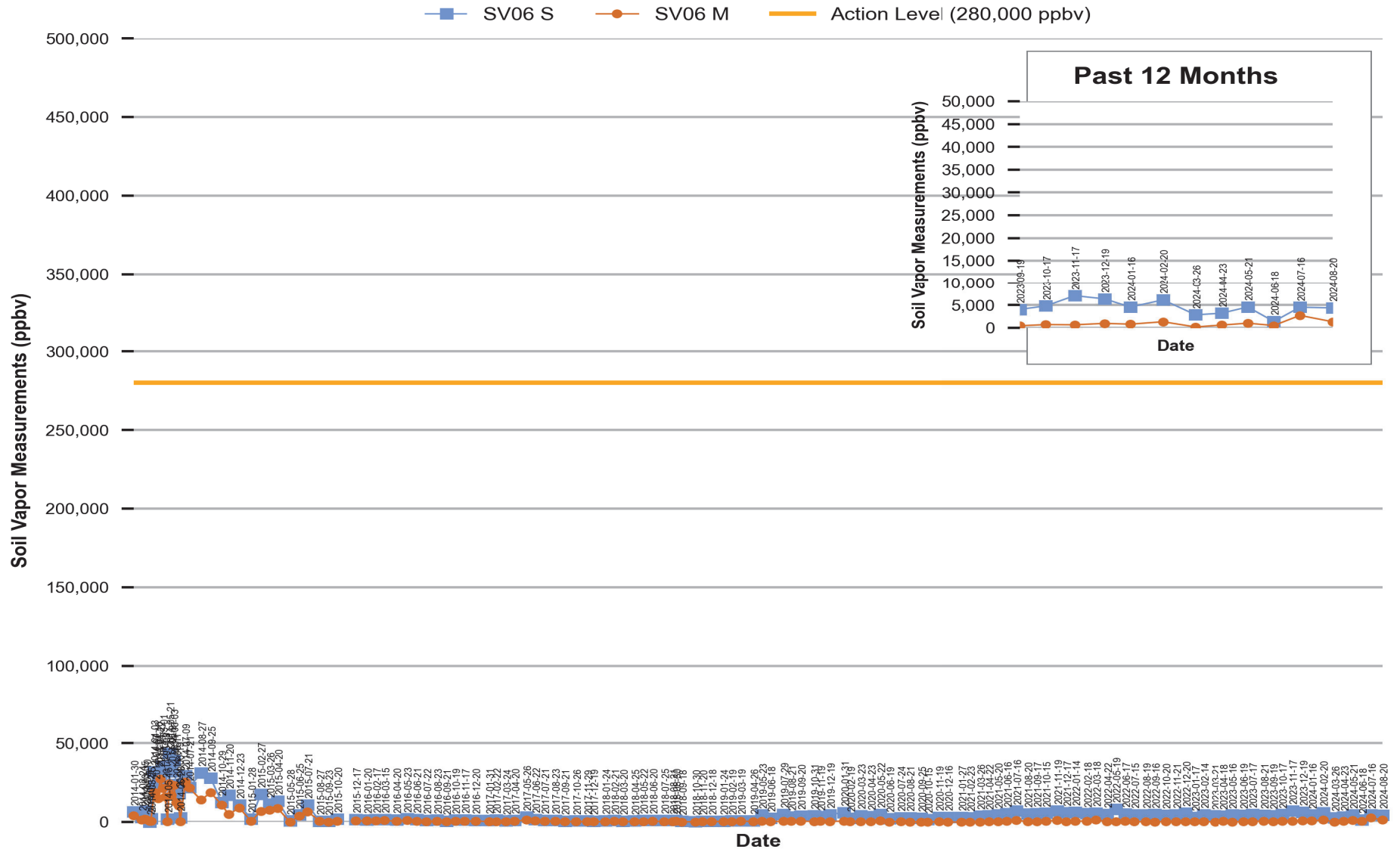
Figure 5 Red Hill - Tank 06 (F-24) Soil Vapor Measurements (Jan 2014 Through Aug 2024)
