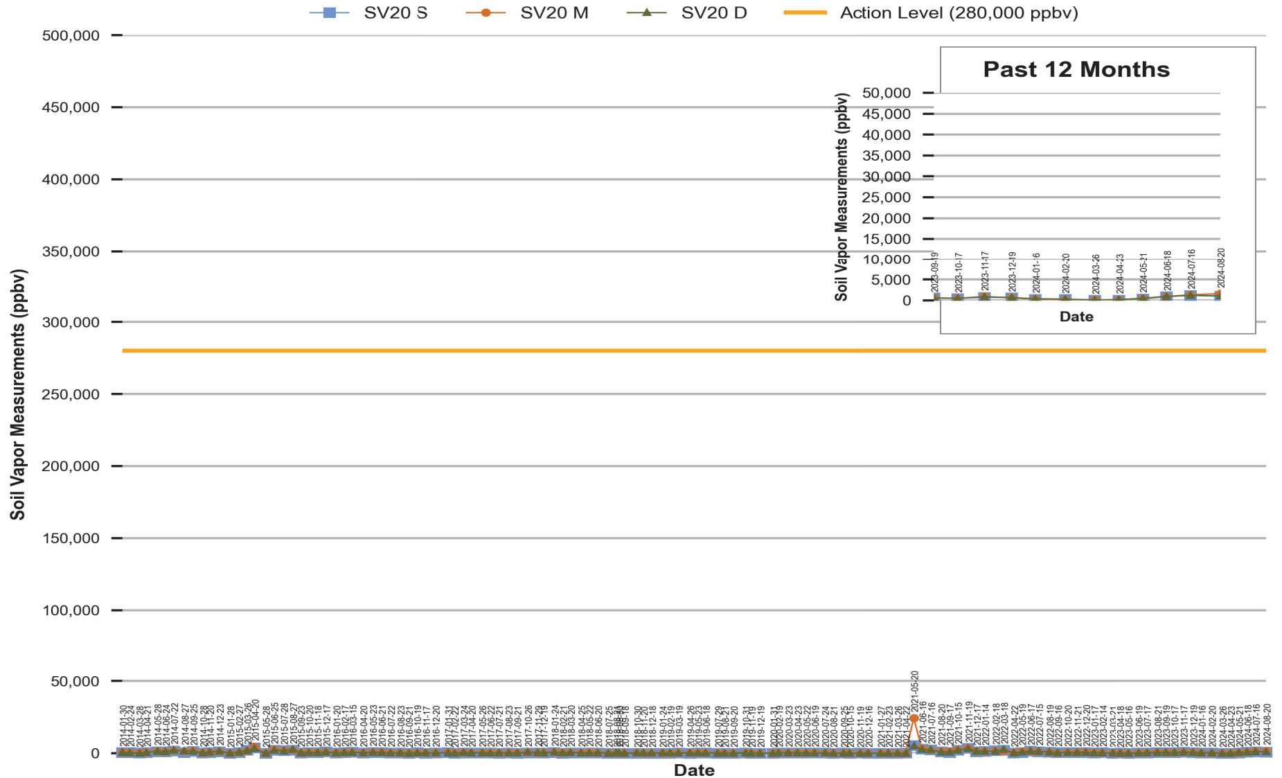
Figure 18 Red Hill - Tank 20 (JP-5) Soil Vapor Measurements (Jan 2014 Through Aug 2024)
