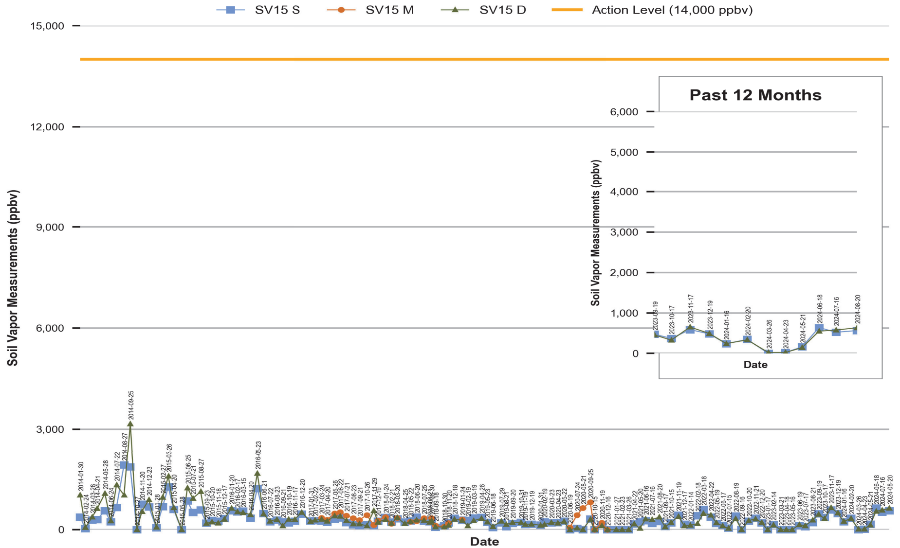
Figure 14 Red Hill - Tank 15 (F-76) Soil Vapor Measurements (Jan 2014 Through Aug 2024)
