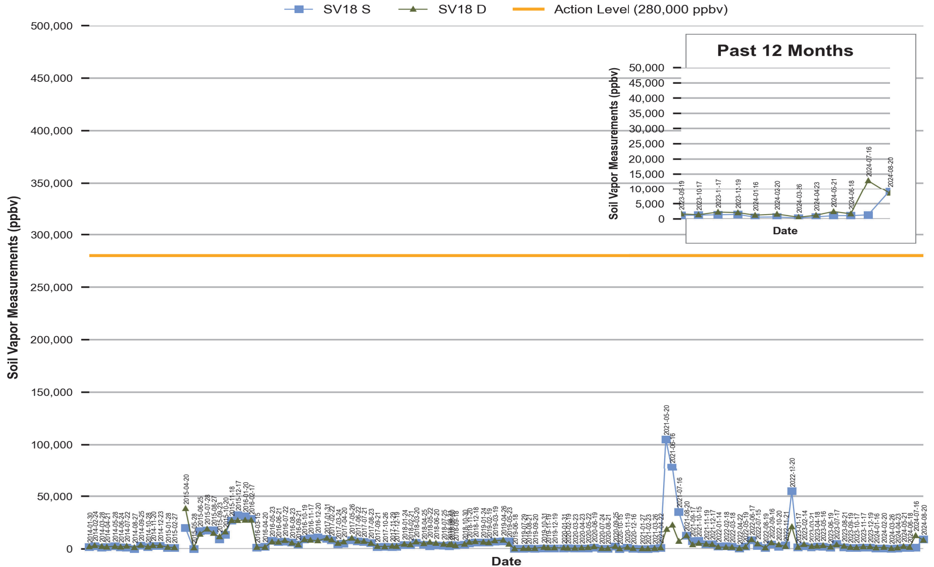
Figure 17 Red Hill - Tank 18 (JP-5) Soil Vapor Measurements (Jan 2014 Through Aug 2024)
