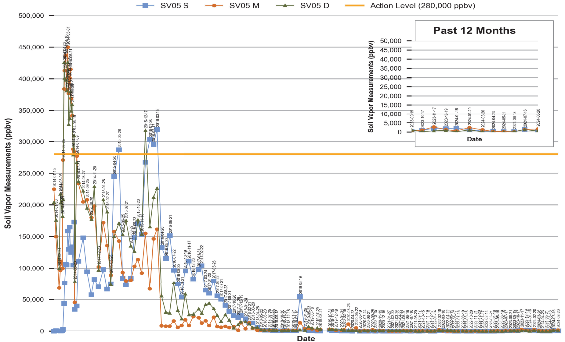
Figure 4 Red Hill - Tank 05 (F-24) Soil Vapor Measurements (Jan 2014 Through Aug 2024)
