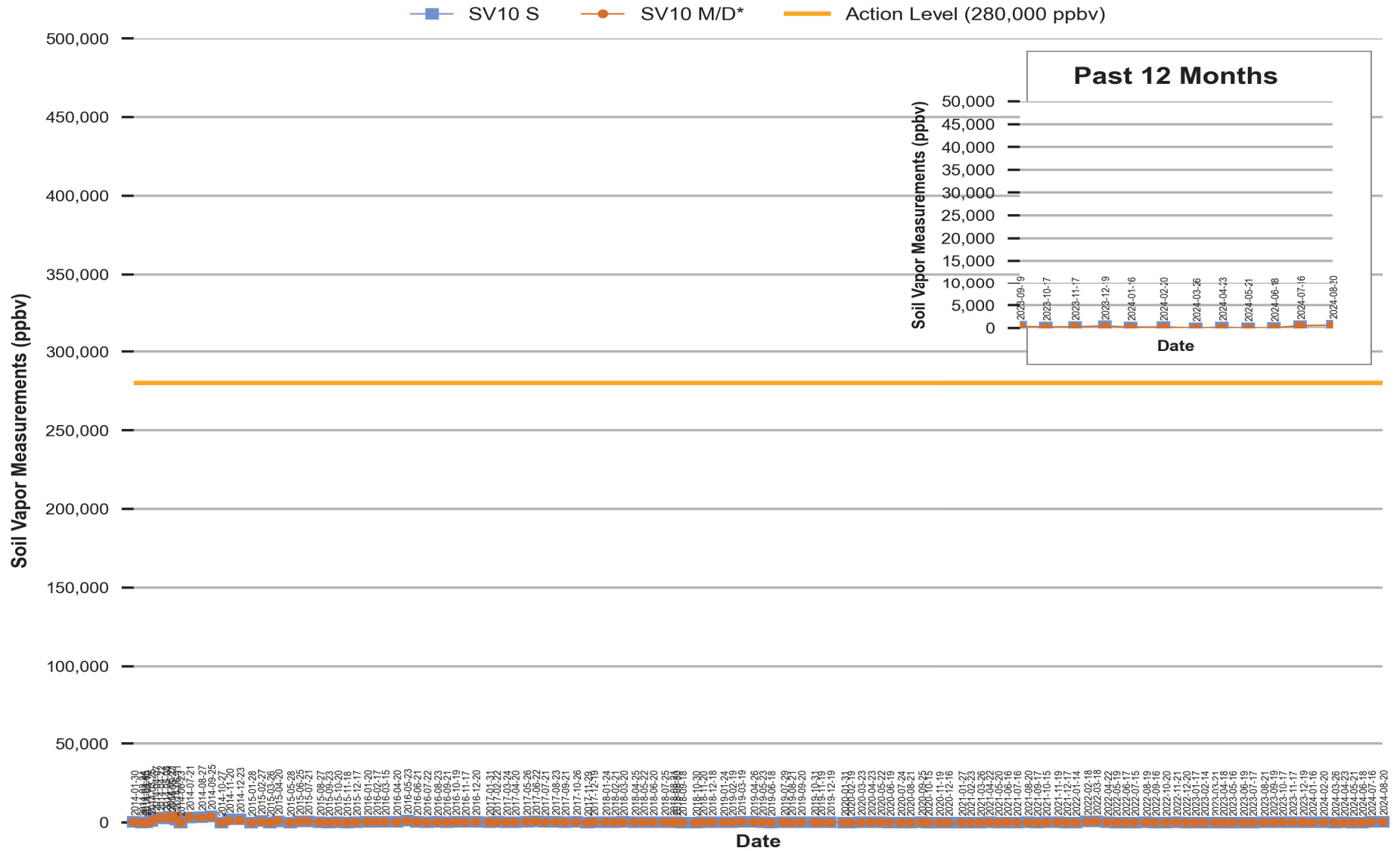
Figure 9 Red Hill - Tank 10 (JP-5) Soil Vapor Measurements (Jan 2014 Through Aug 2024)
