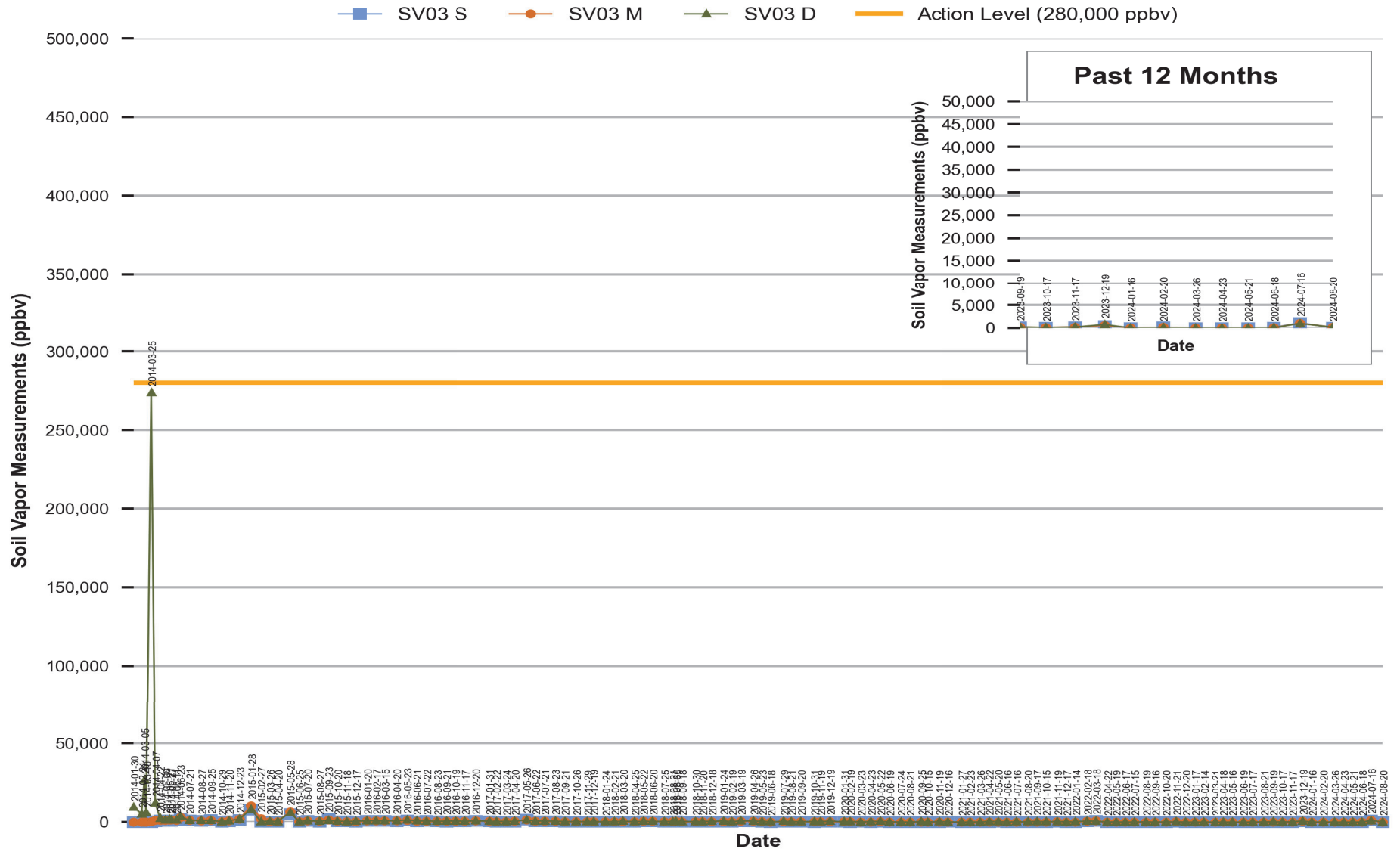
Figure 2 Red Hill - Tank 03 (F-24) Soil Vapor Measurements (Jan 2014 Through Aug 2024)
