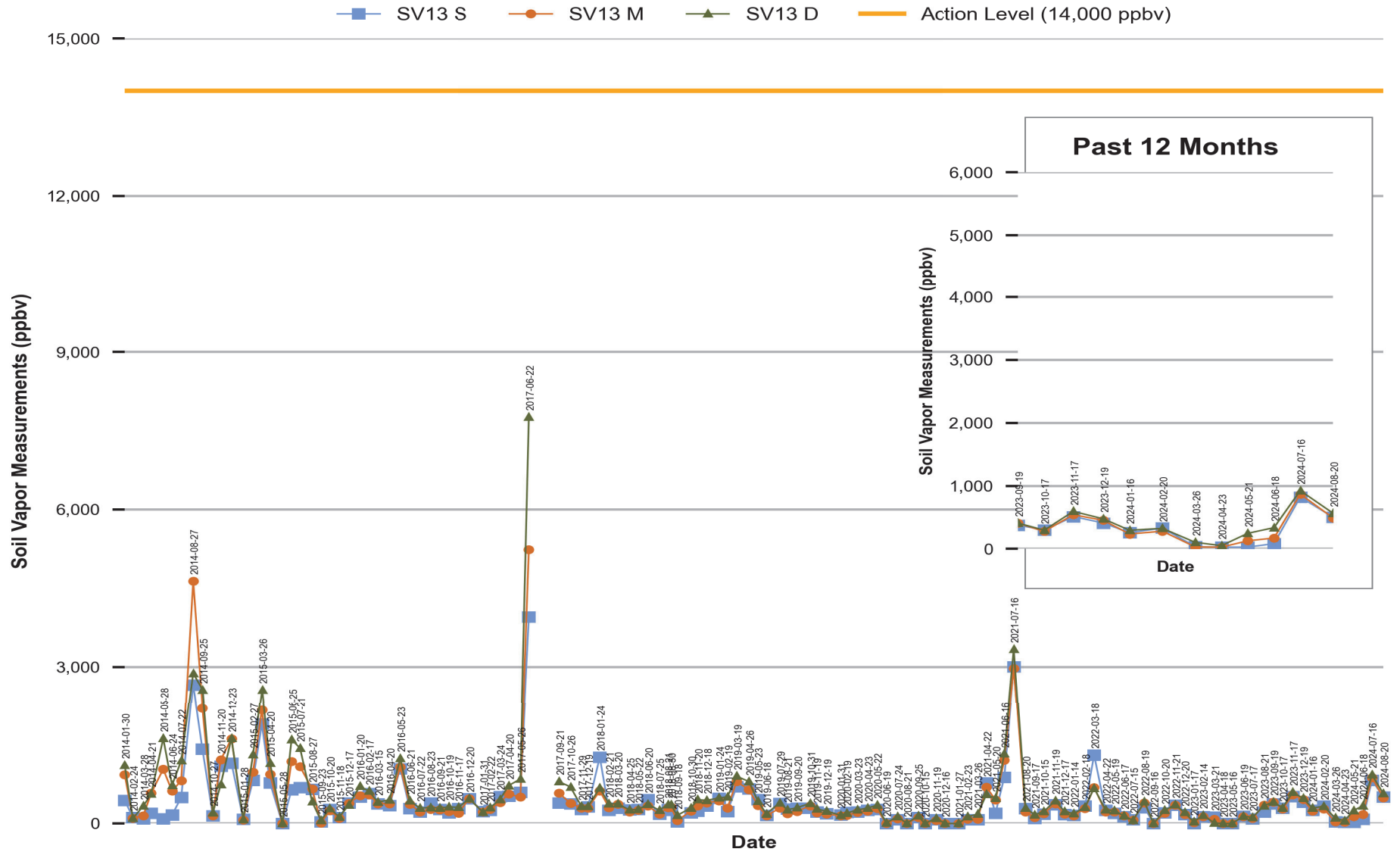
Figure 12 Red Hill - Tank 13 (F-76) Soil Vapor Measurements (Jan 2014 Through Aug 2024)
