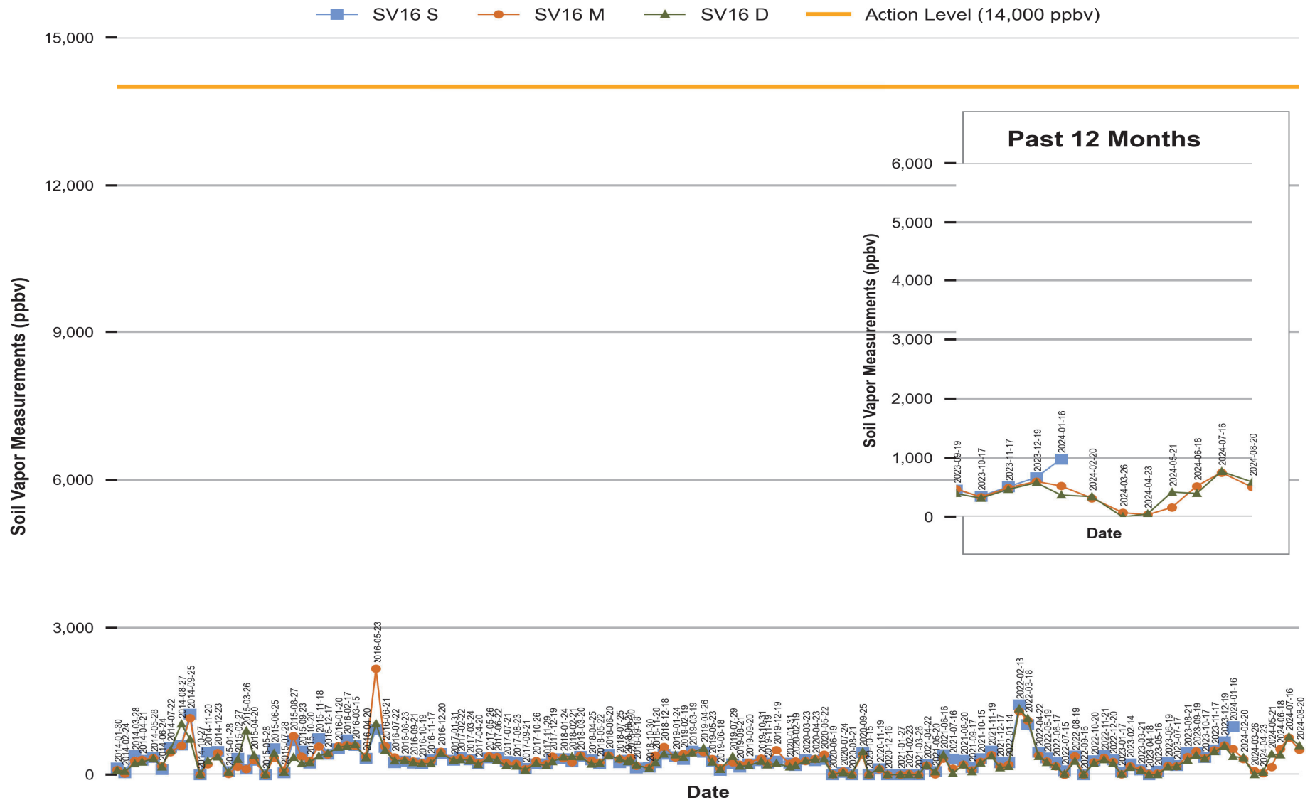
Figure 15 Red Hill - Tank 16 (F-76) Soil Vapor Measurements (Jan 2014 Through Aug 2024)
