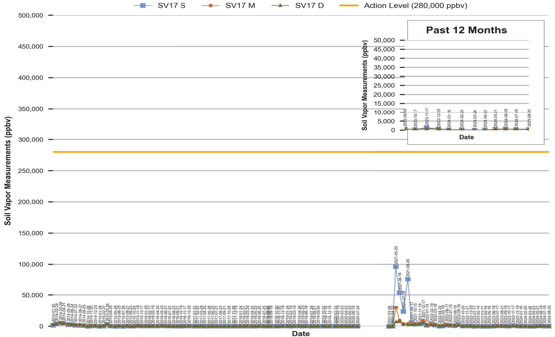
Figure 16 Red Hill - Tank 17 (JP-5) Soil Vapor Measurements (Jan 2014 Through Aug 2024)
