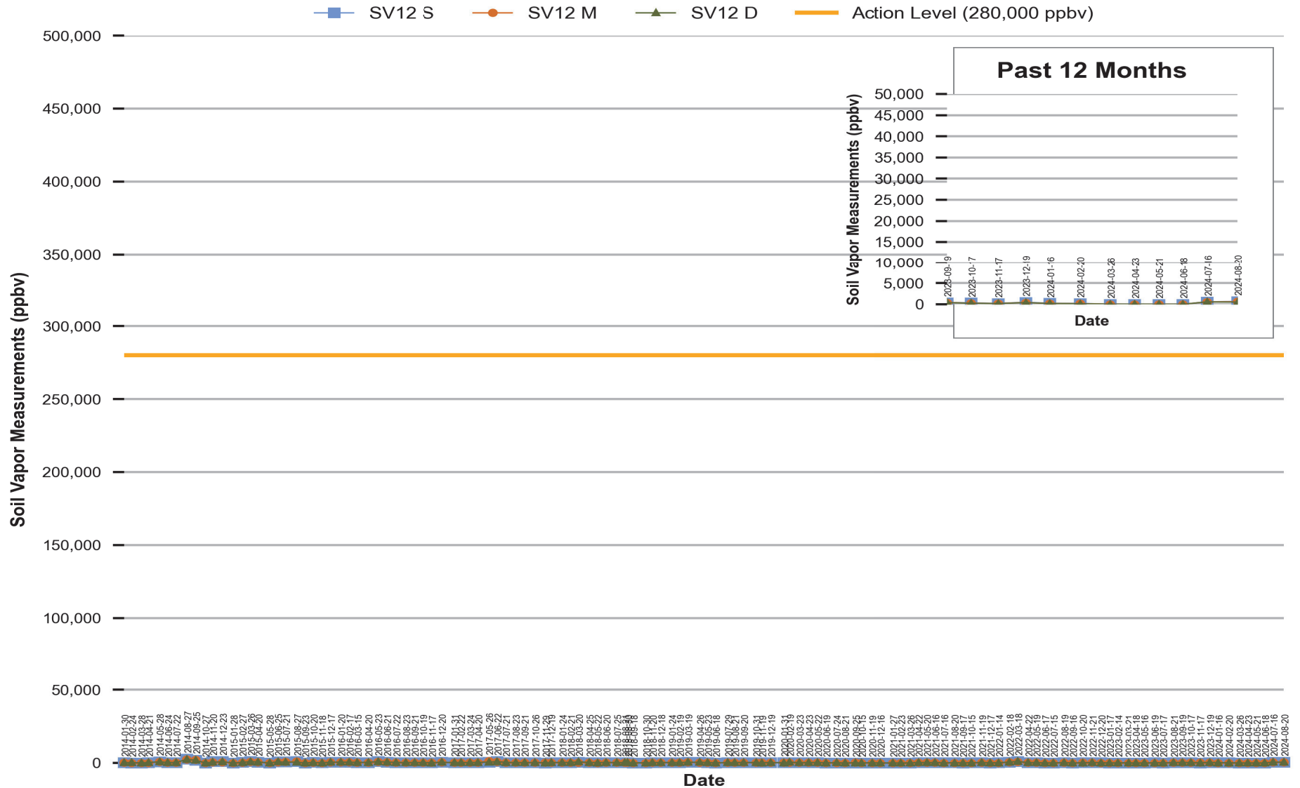
Figure 11 Red Hill - Tank 12 (JP-5) Soil Vapor Measurements (Jan 2014 Through Aug 2024)
