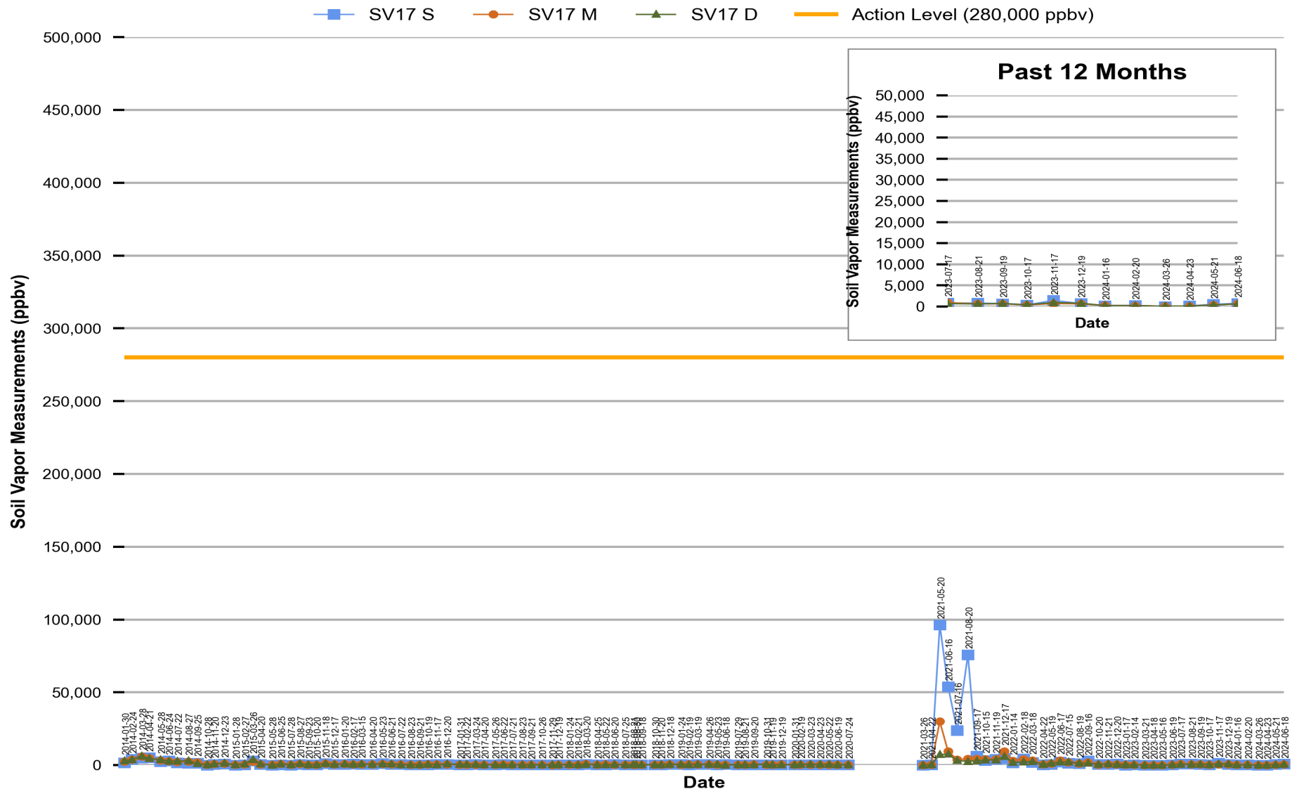
Figure 16 Red Hill - Tank 17 (JP-5) Soil Vapor Measurements (Jan 2014 Through Jun 2024)
