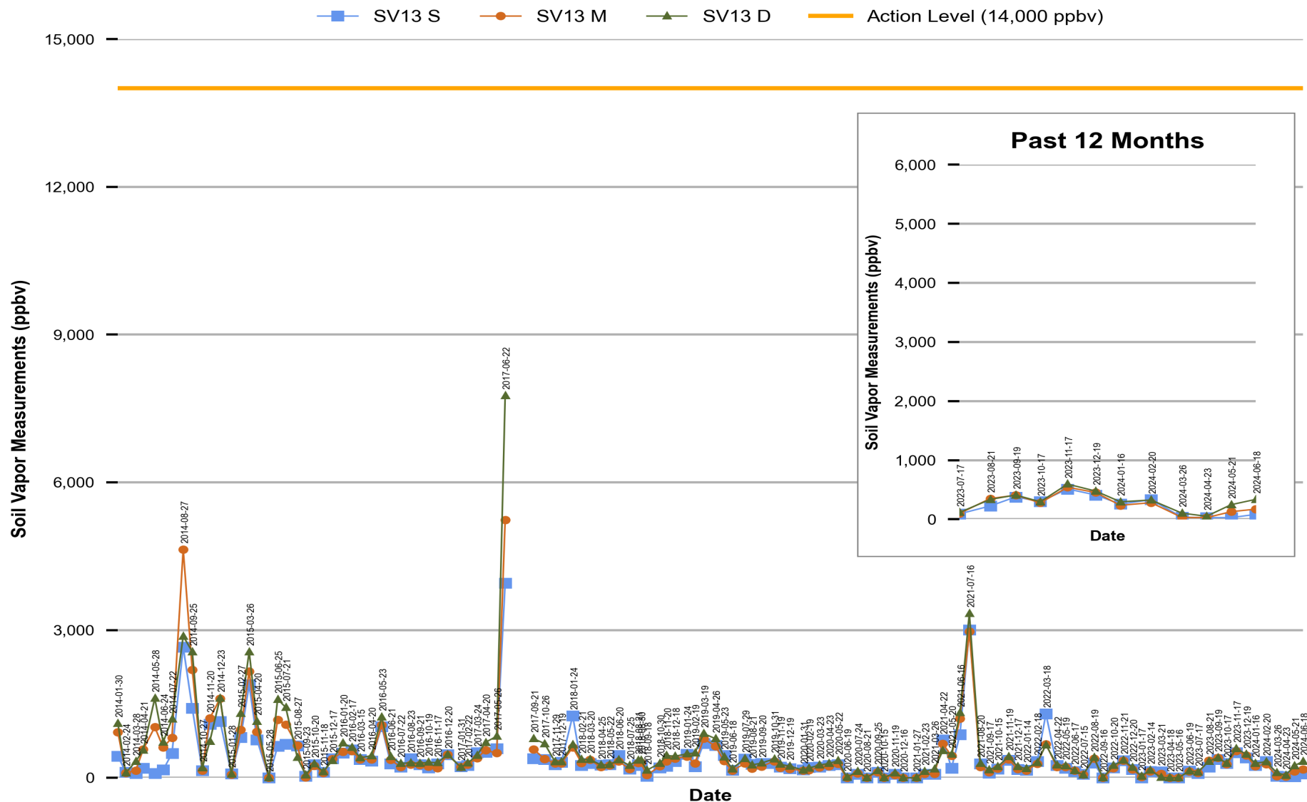
Figure 12 Red Hill - Tank 13 (F-76) Soil Vapor Measurements (Jan 2014 Through Jun 2024)
