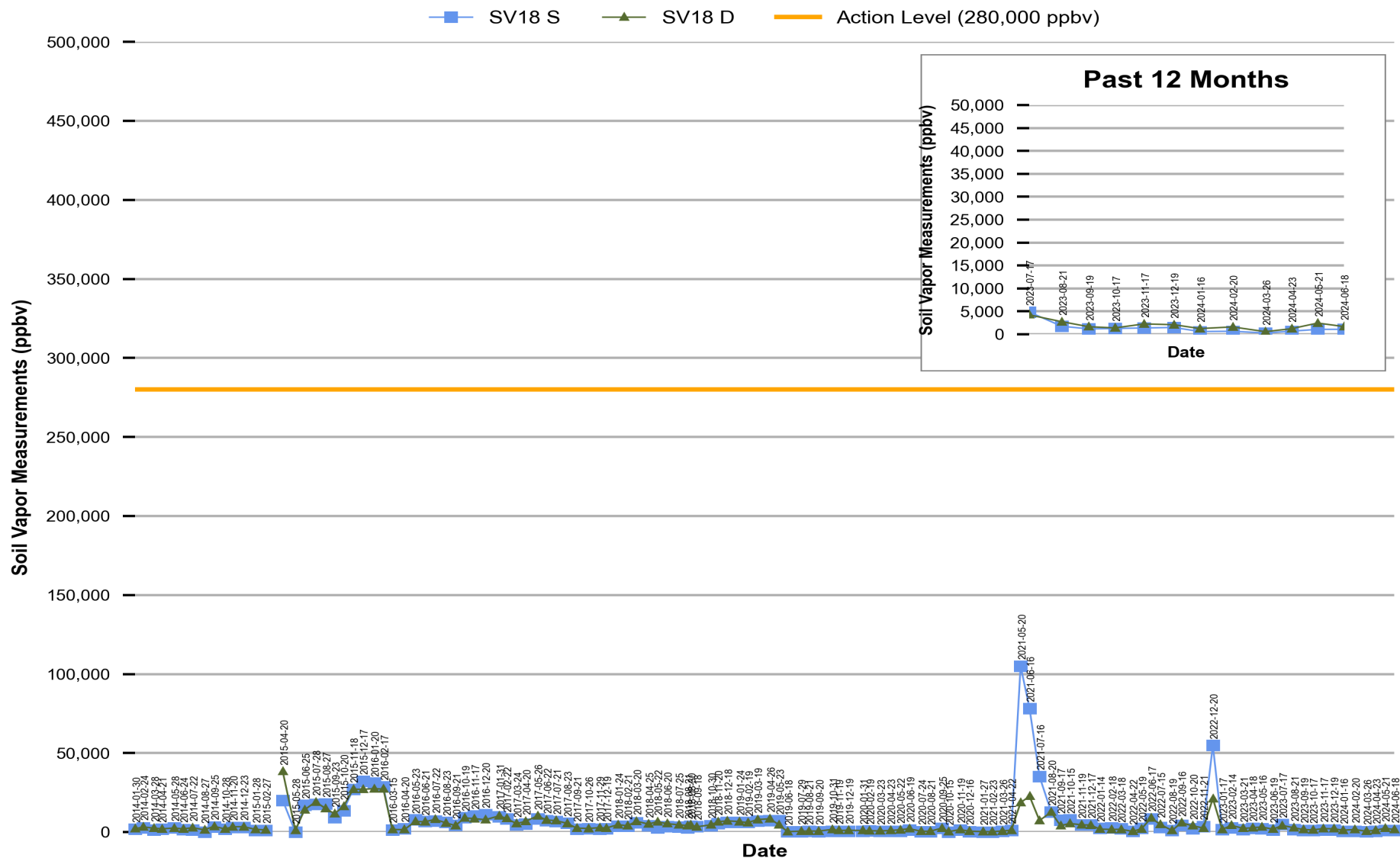
Figure 17 Red Hill - Tank 18 (JP-5) Soil Vapor Measurements (Jan 2014 Through Jun 2024)
