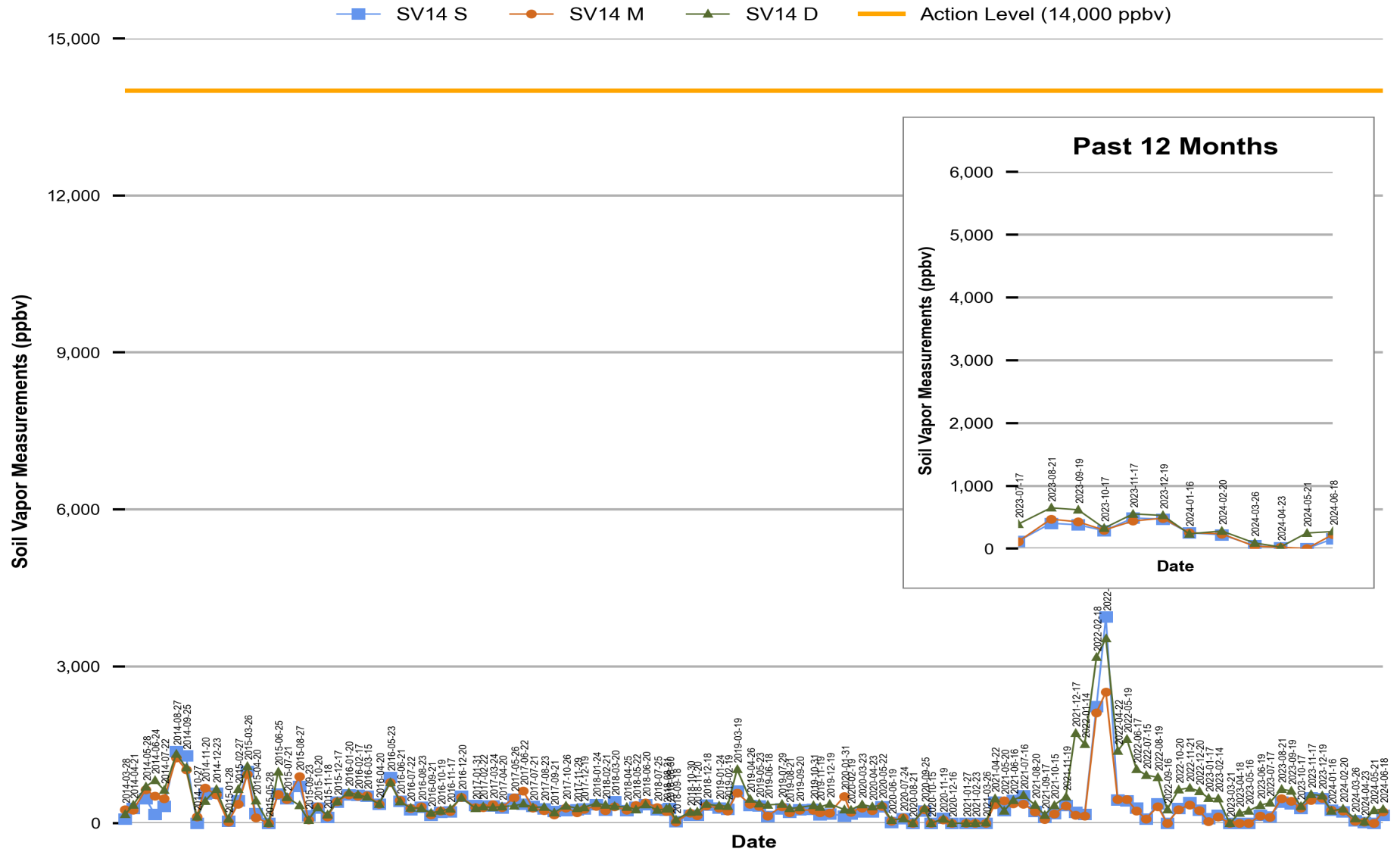
Figure 13 Red Hill - Tank 14 (F-76) Soil Vapor Measurements (Mar 2014 Through Jun 2024)
