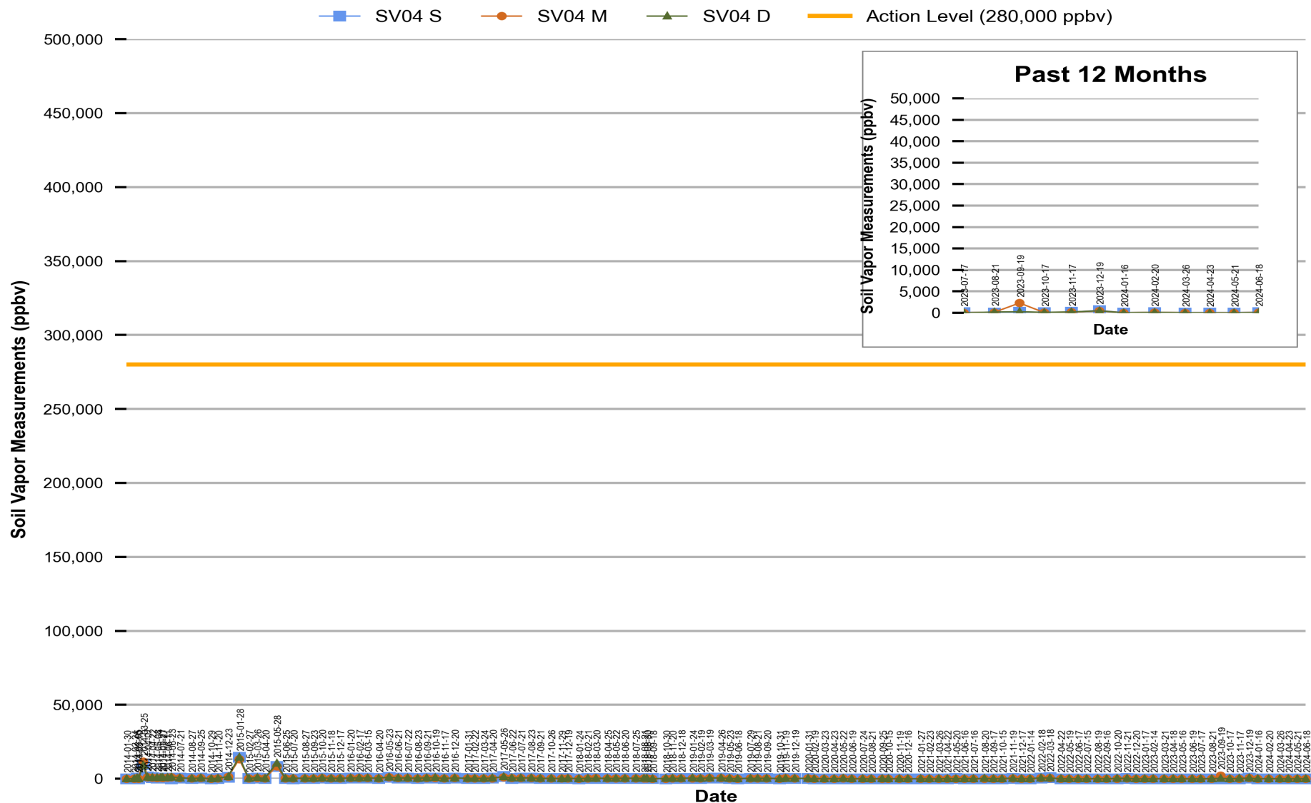
Figure 3 Red Hill - Tank 04 (F-24) Soil Vapor Measurements (Jan 2014 Through Jun 2024)
