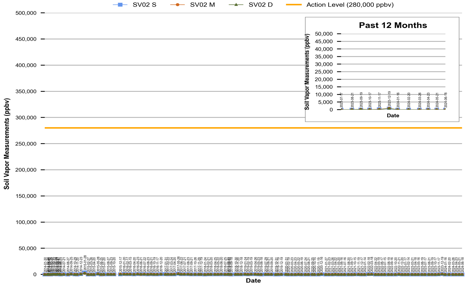
Figure 1 Red Hill - Tank 02 (F-24) Soil Vapor Measurements (Jan 2014 Through Jun 2024)
