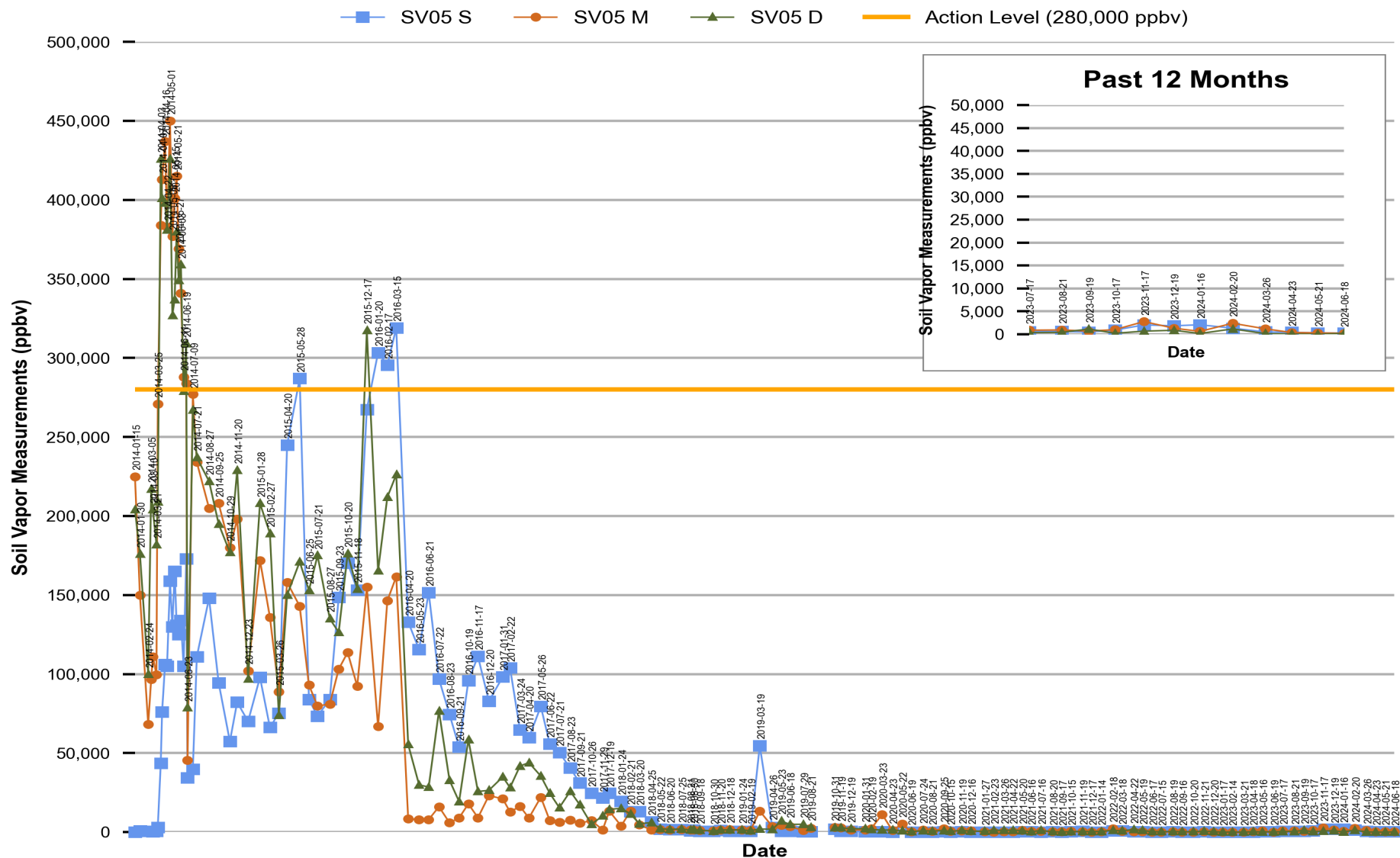
Figure 4 Red Hill - Tank 05 (F-24) Soil Vapor Measurements (Jan 2014 Through Jun 2024)
