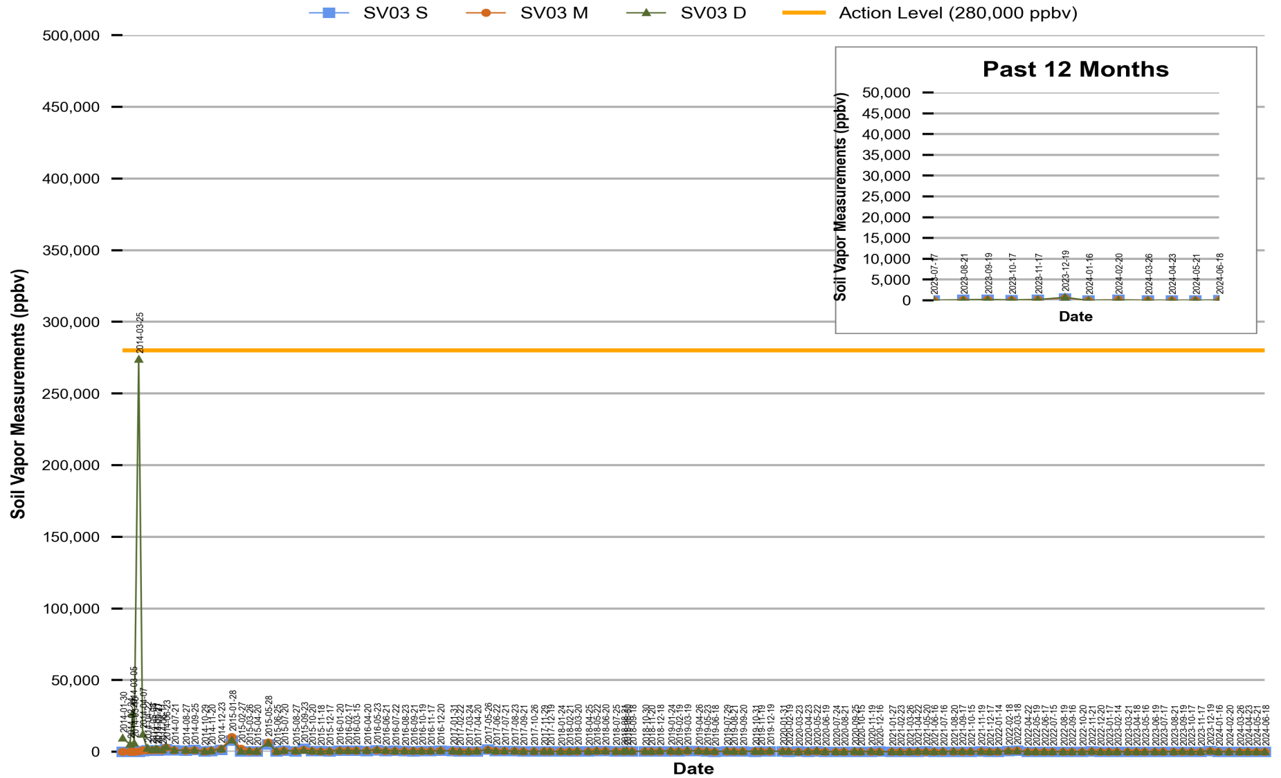
Figure 2 Red Hill - Tank 03 (F-24) Soil Vapor Measurements (Jan 2014 Through Jun 2024)
