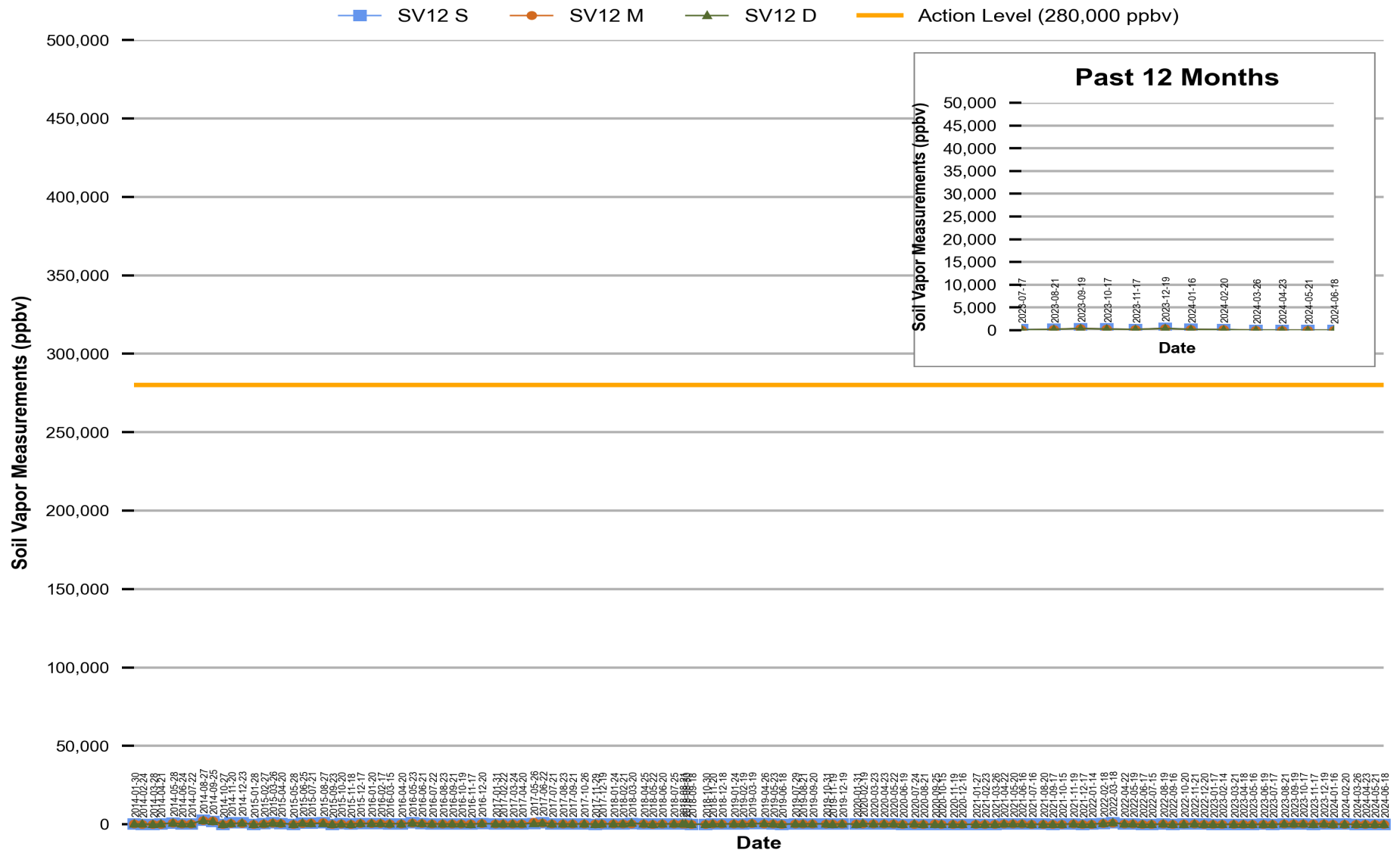
Figure 11 Red Hill - Tank 12 (JP-5) Soil Vapor Measurements (Jan 2014 Through Jun 2024)
