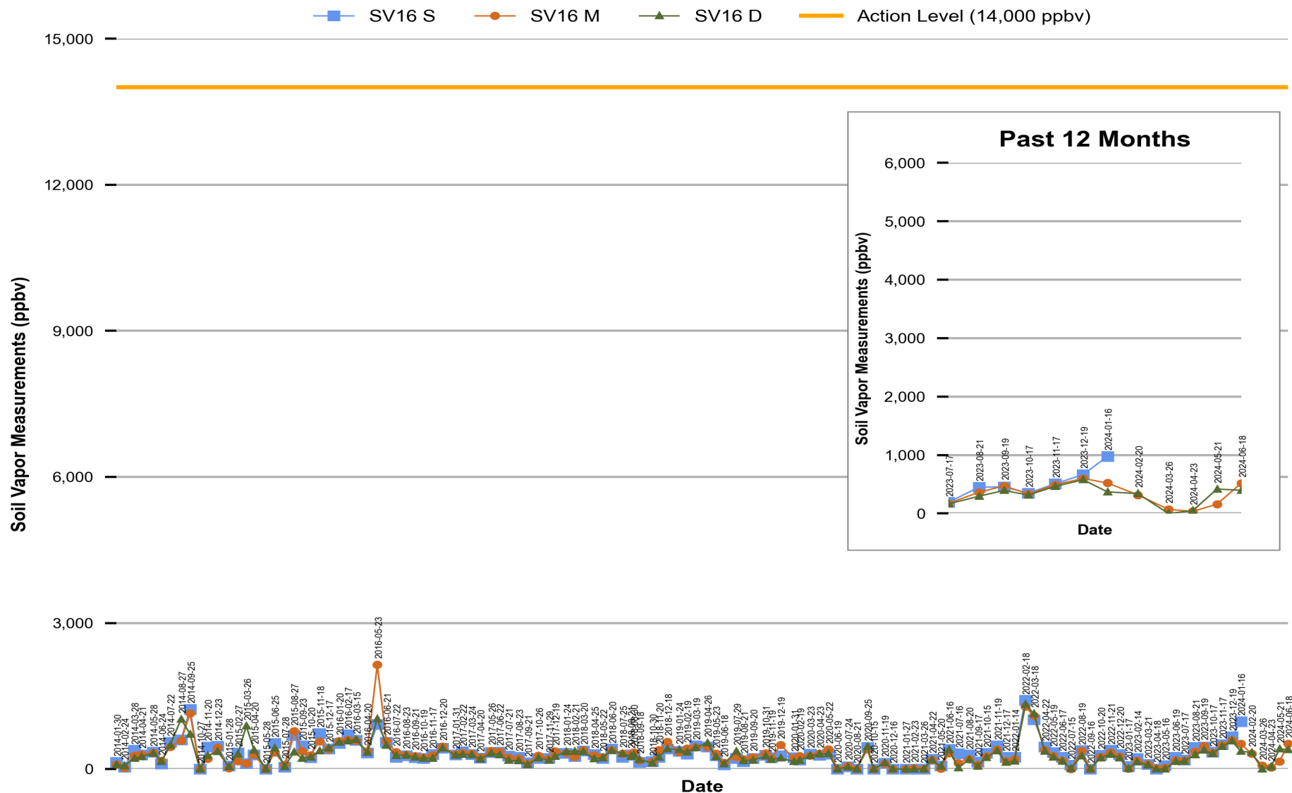
Figure 15 Red Hill - Tank 16 (F-76) Soil Vapor Measurements (Jan 2014 Through Jun 2024)
