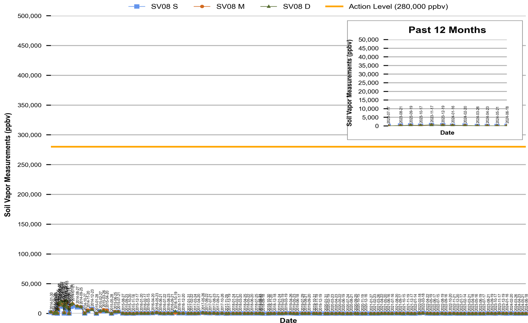
Figure 7 Red Hill - Tank 08 (JP-5) Soil Vapor Measurements (Jan 2014 Through Jun 2024)
