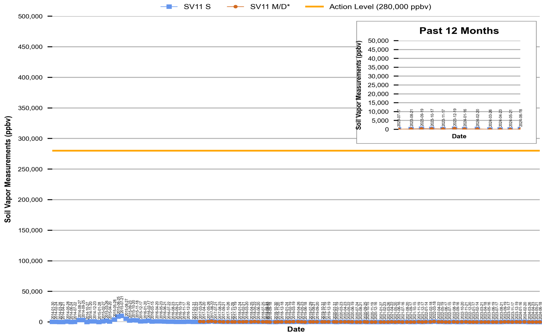
Figure 10 Red Hill - Tank 11 (JP-5) Soil Vapor Measurements (Jan 2014 Through Jun 2024)
