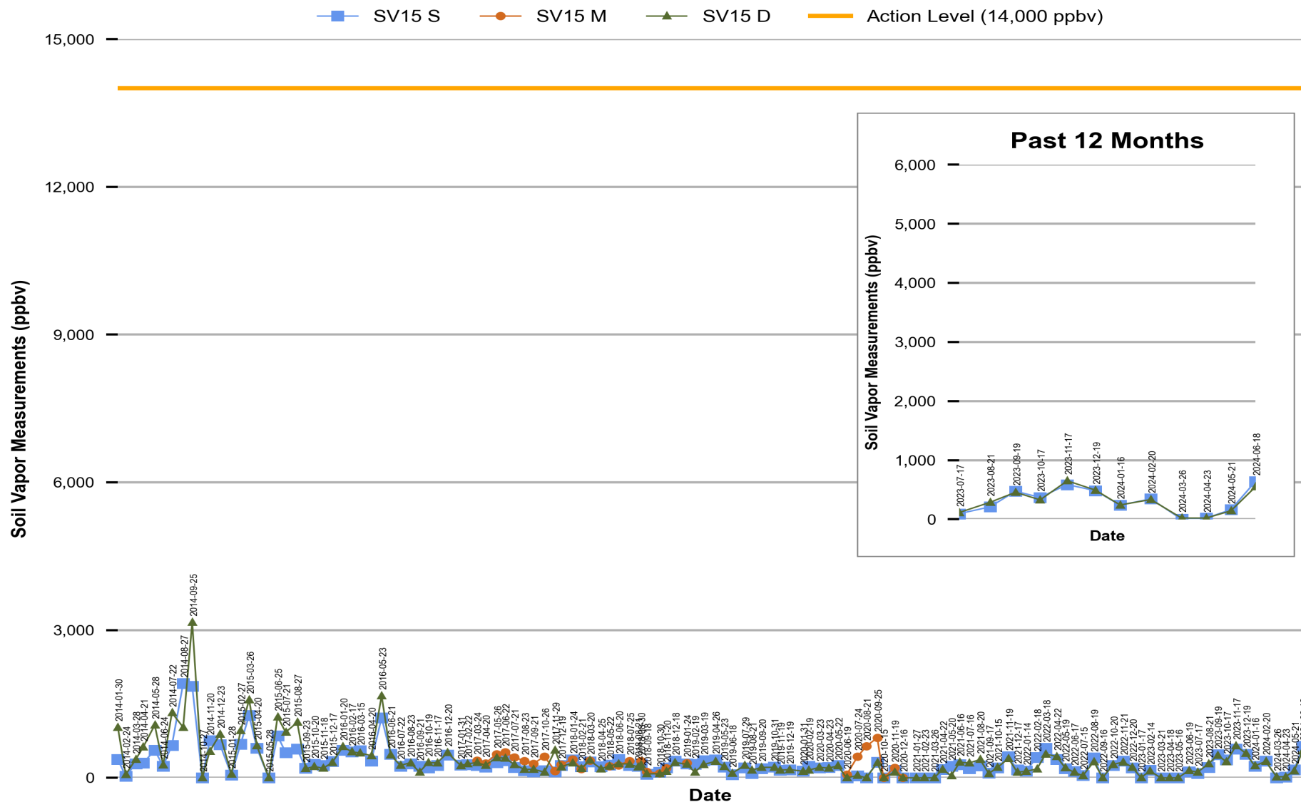
Figure 14 Red Hill - Tank 15 (F-76) Soil Vapor Measurements (Jan 2014 Through Jun 2024)
