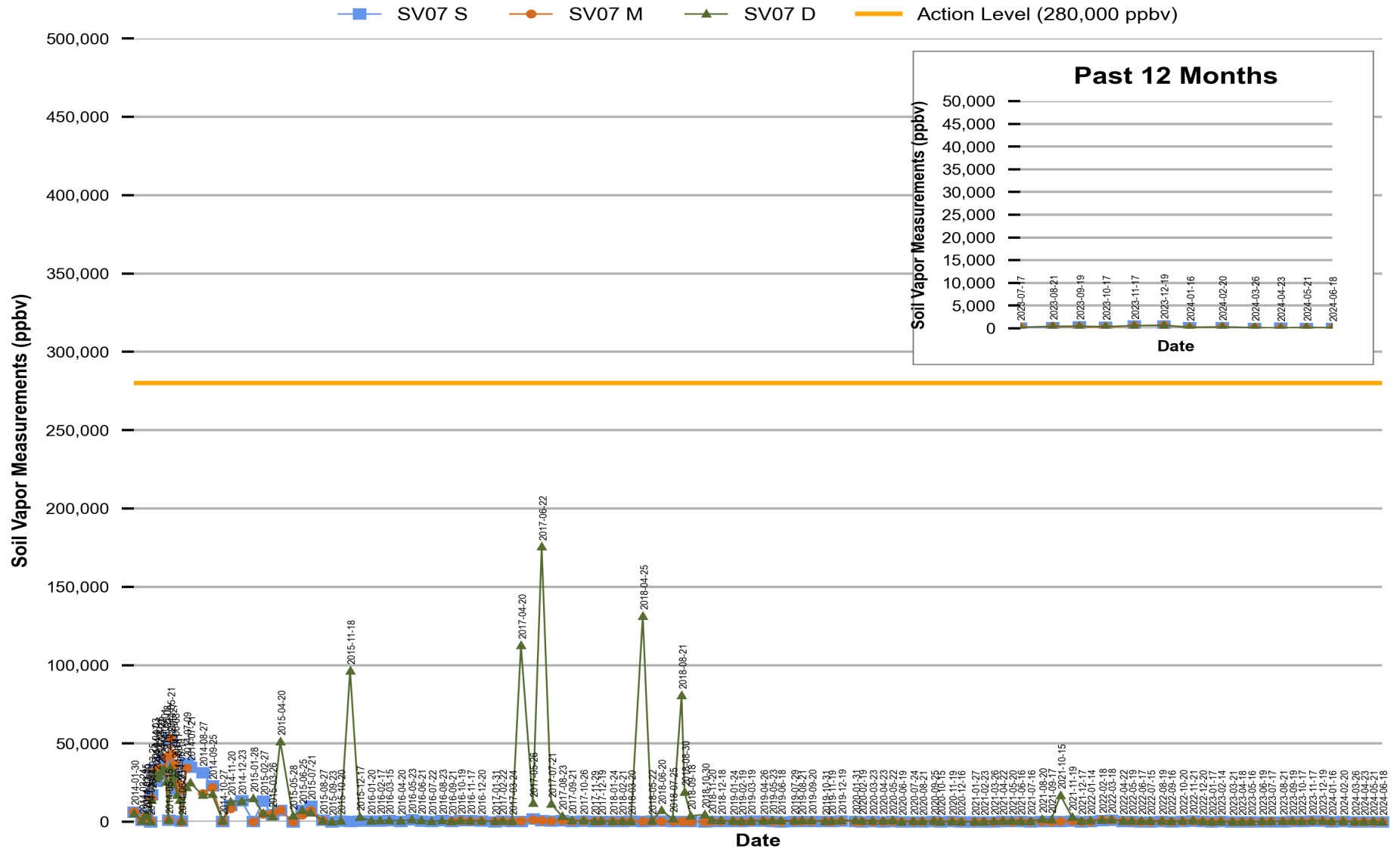
Figure 6 Red Hill - Tank 07 (JP-5) Soil Vapor Measurements (Jan 2014 Through Jun 2024)
