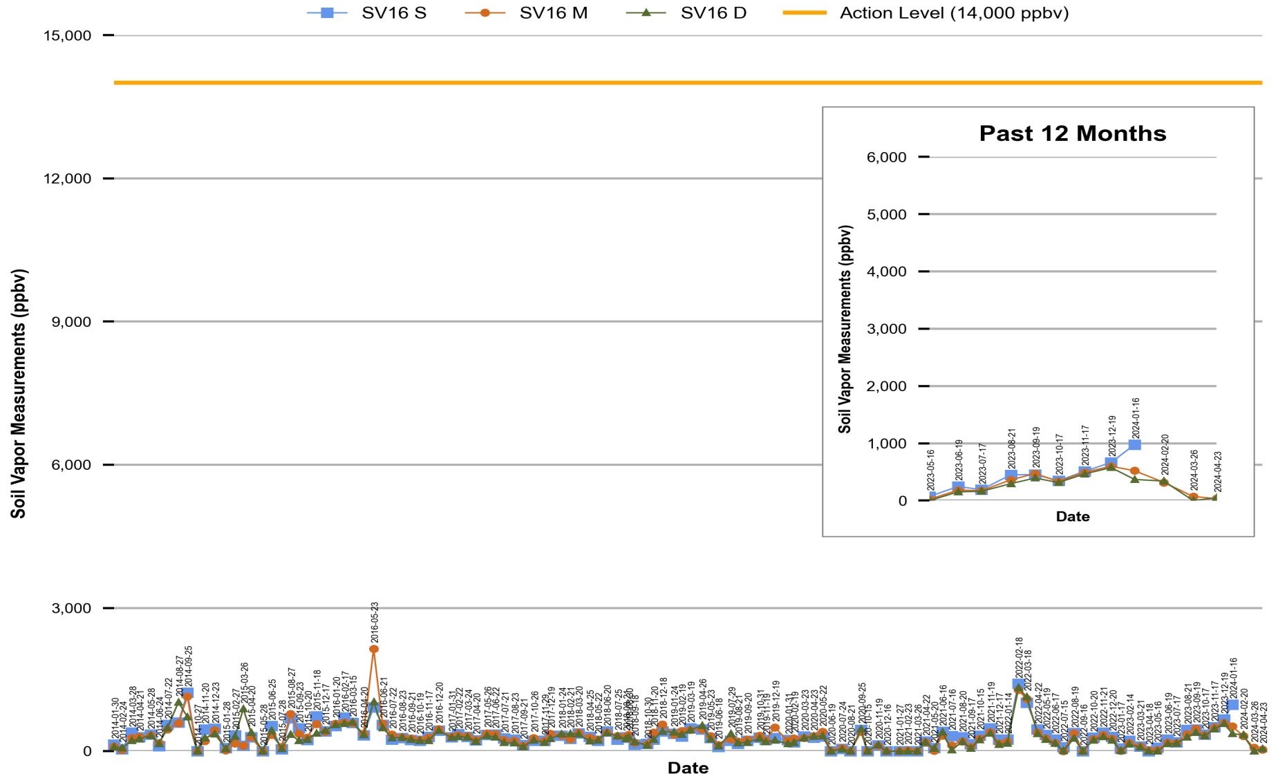
Figure 15 Red Hill - Tank 16 (F-76) Soil Vapor Measurements (Jan 2014 Through Apr 2024)
