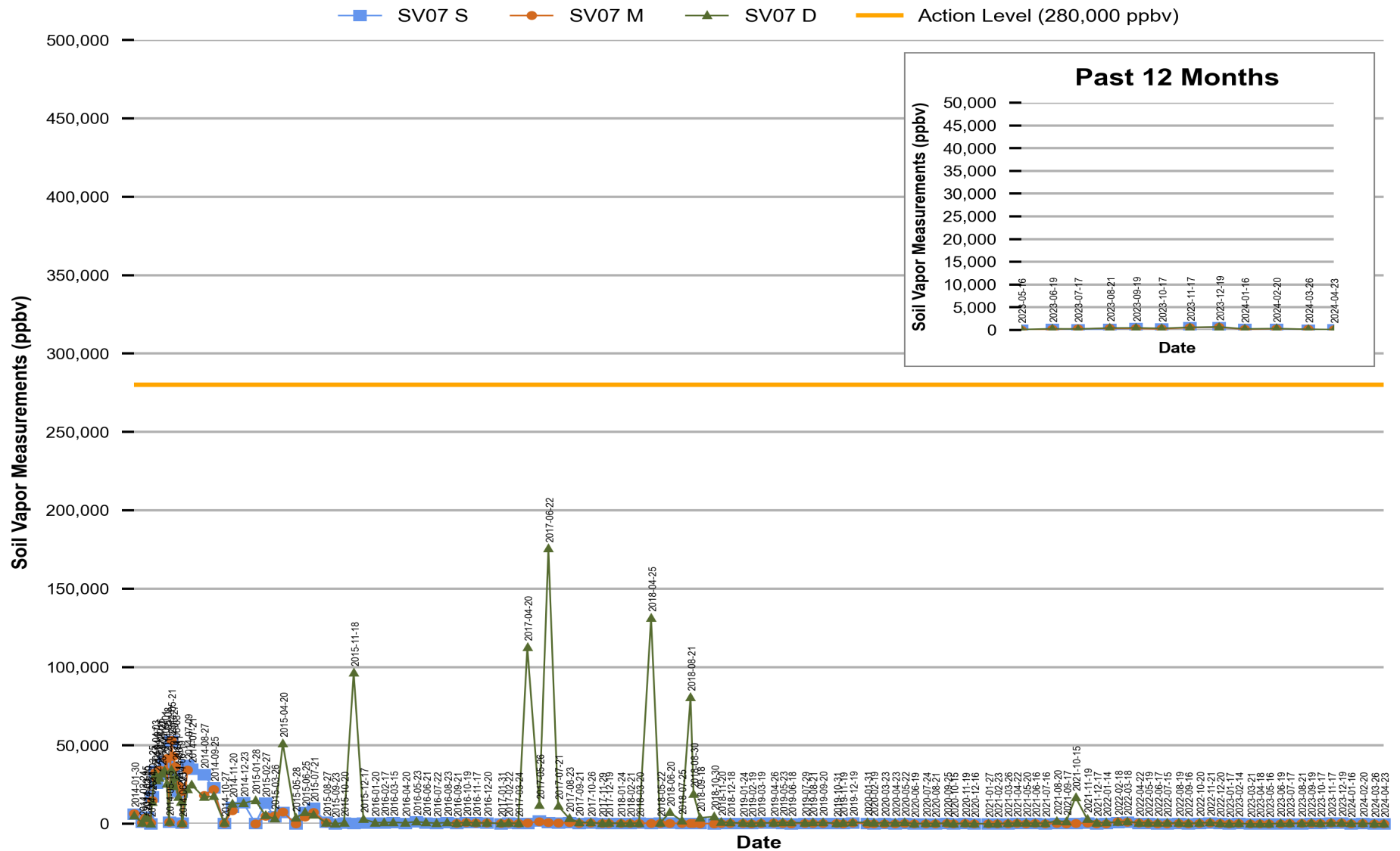
Figure 6 Red Hill - Tank 07 (JP-5) Soil Vapor Measurements (Jan 2014 Through Apr 2024)
