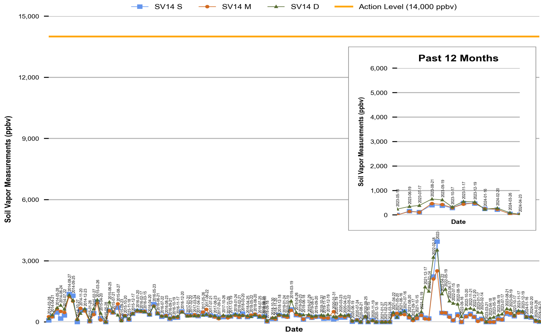
Figure 13 Red Hill - Tank 14 (F-76) Soil Vapor Measurements (Mar 2014 Through Apr 2024)
