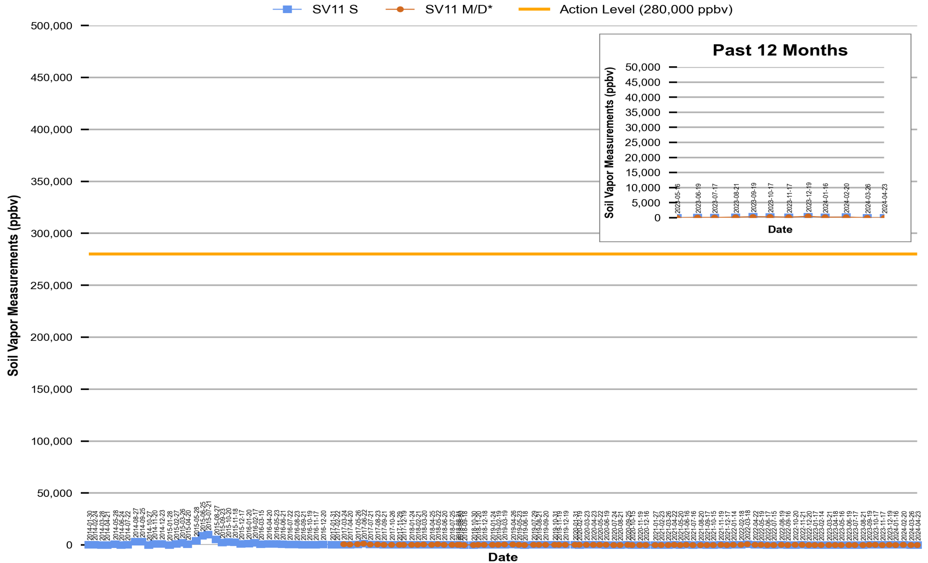
Figure 10 Red Hill - Tank 11 (JP-5) Soil Vapor Measurements (Jan 2014 Through Apr 2024)
