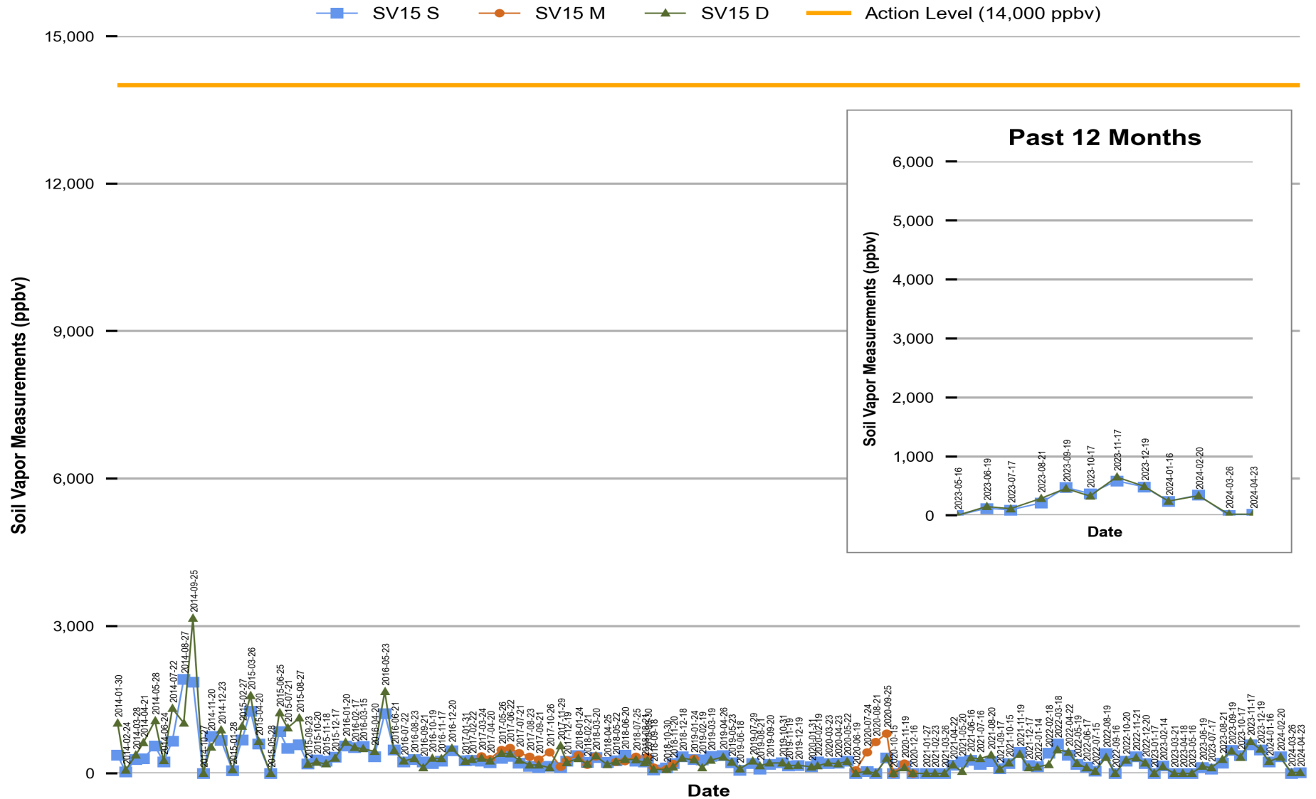
Figure 14 Red Hill - Tank 15 (F-76) Soil Vapor Measurements (Jan 2014 Through Apr 2024)
