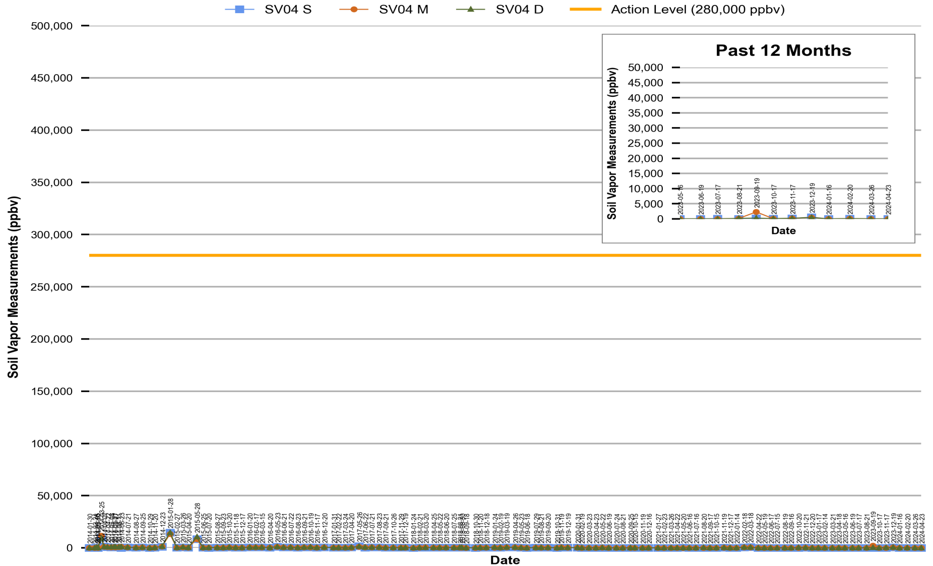
Figure 3 Red Hill - Tank 04 (F-24) Soil Vapor Measurements (Jan 2014 Through Apr 2024)
