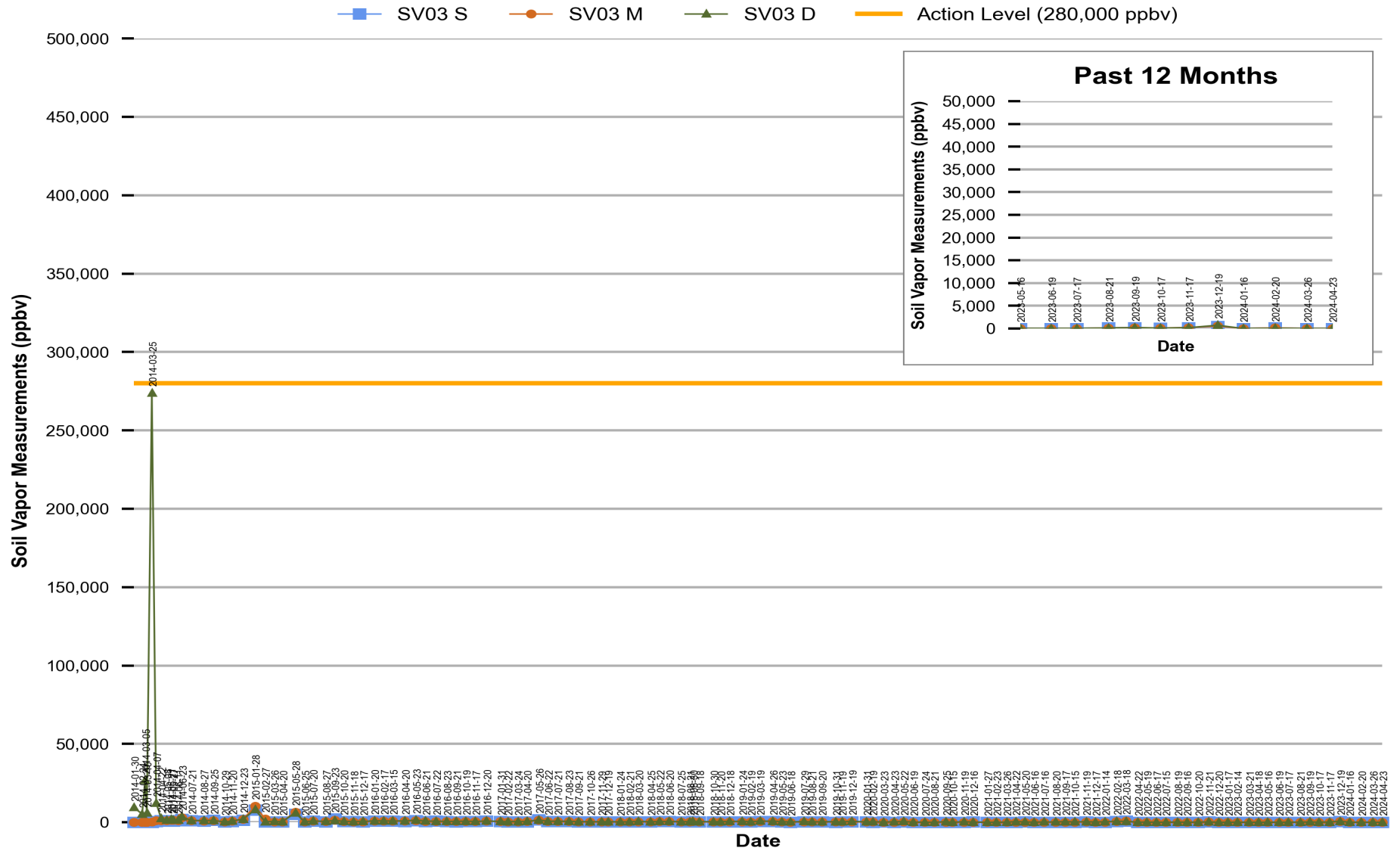
Figure 2 Red Hill - Tank 03 (F-24) Soil Vapor Measurements (Jan 2014 Through Apr 2024)
