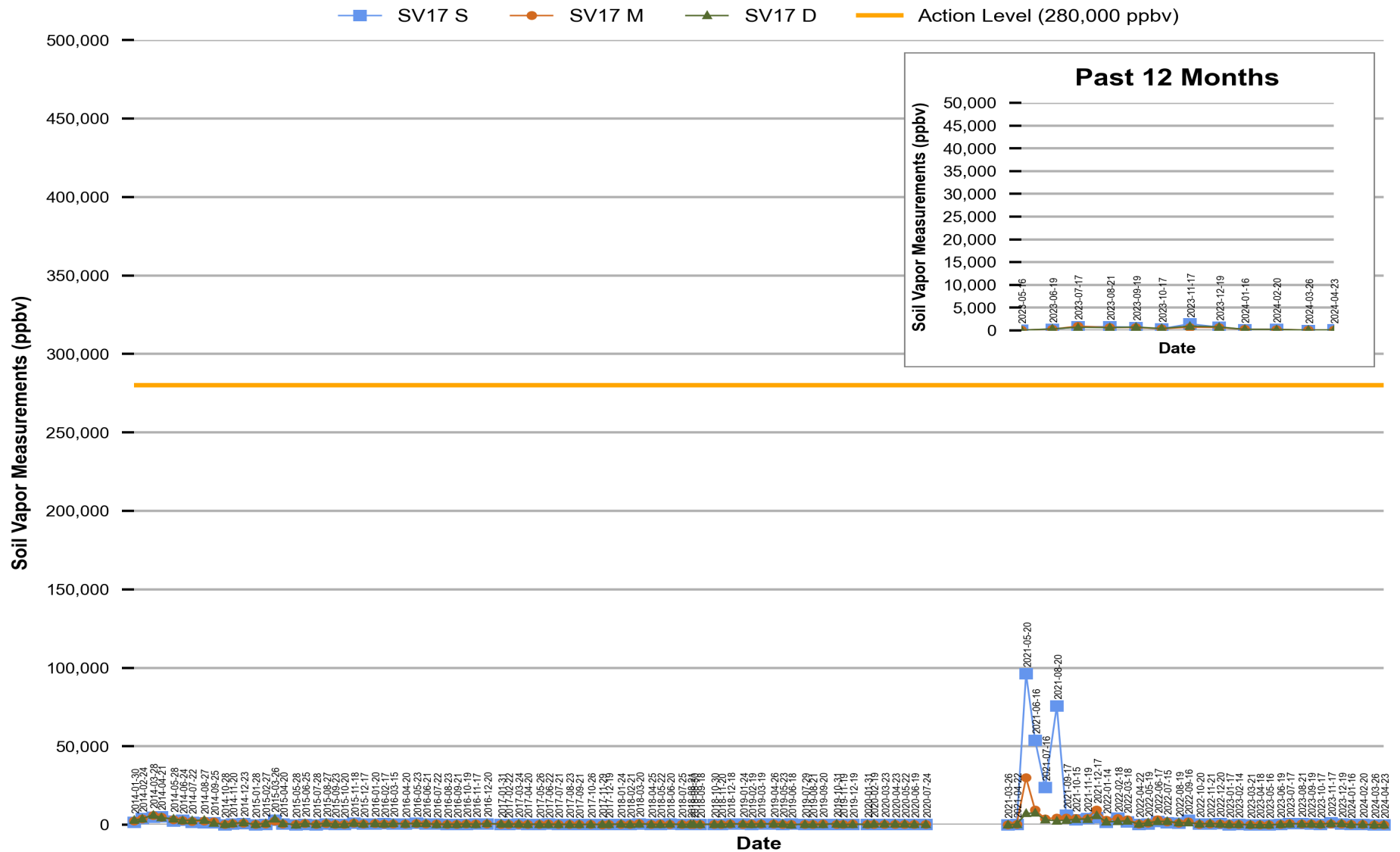
Figure 16 Red Hill - Tank 17 (JP-5) Soil Vapor Measurements (Jan 2014 Through Apr 2024)
