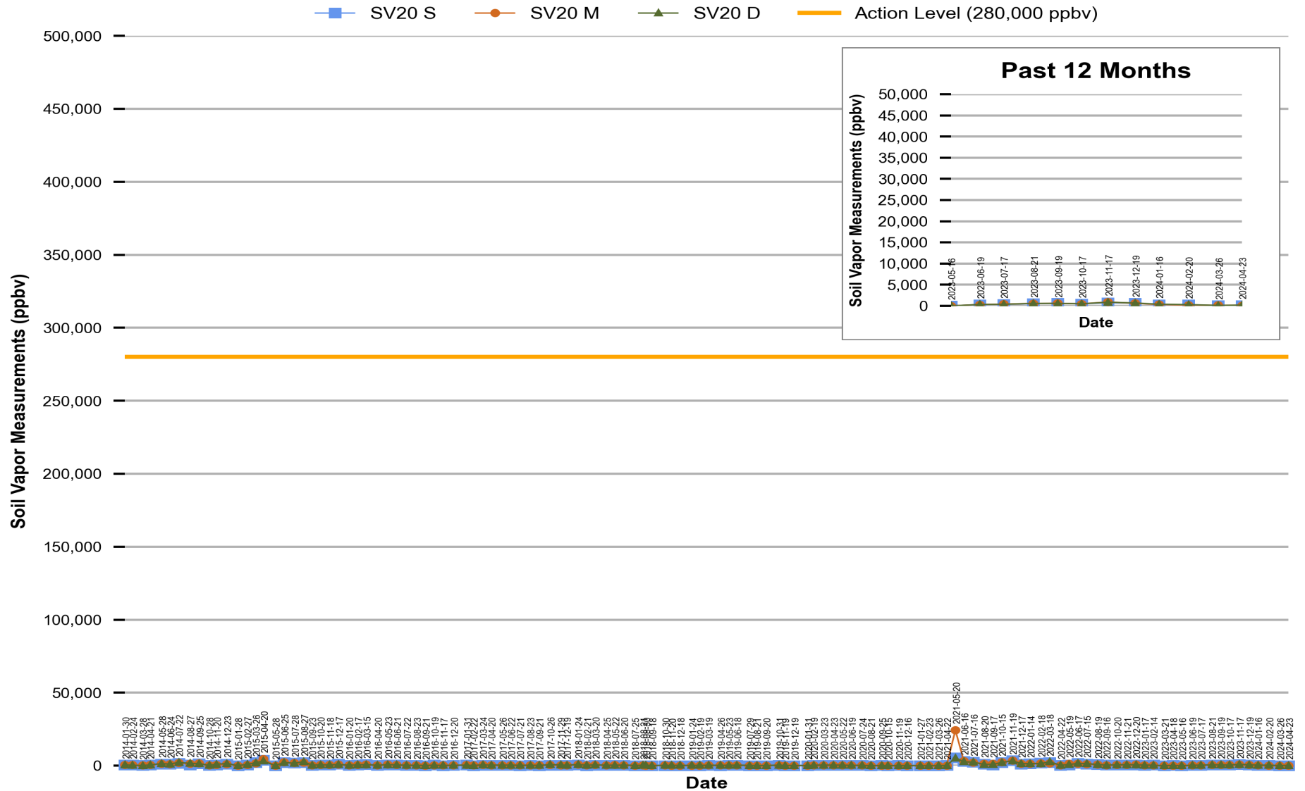
Figure 18 Red Hill - Tank 20 (JP-5) Soil Vapor Measurements (Jan 2014 Through Apr 2024)
