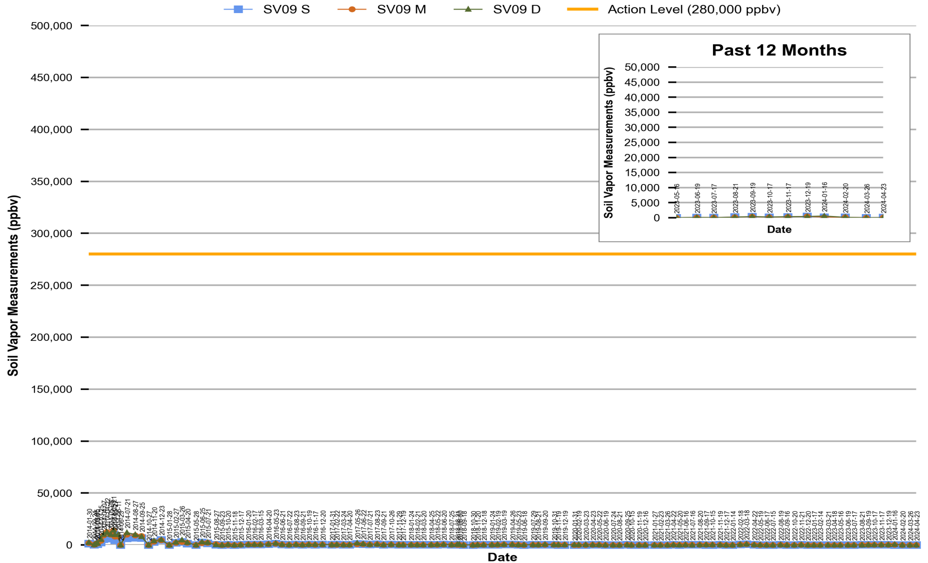
Figure 8 Red Hill - Tank 09 (JP-5) Soil Vapor Measurements (Jan 2014 Through Apr 2024)
