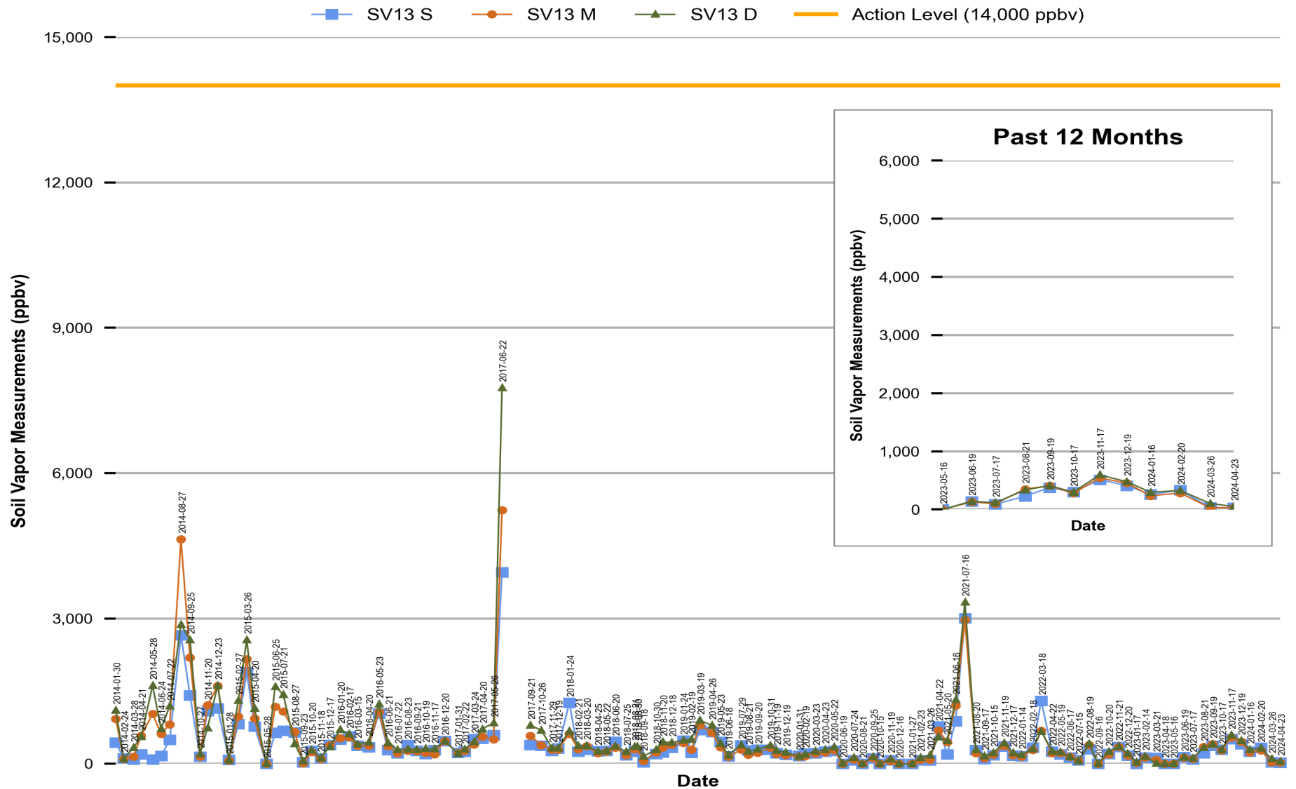
Figure 12 Red Hill - Tank 13 (F-76) Soil Vapor Measurements (Jan 2014 Through Apr 2024)
