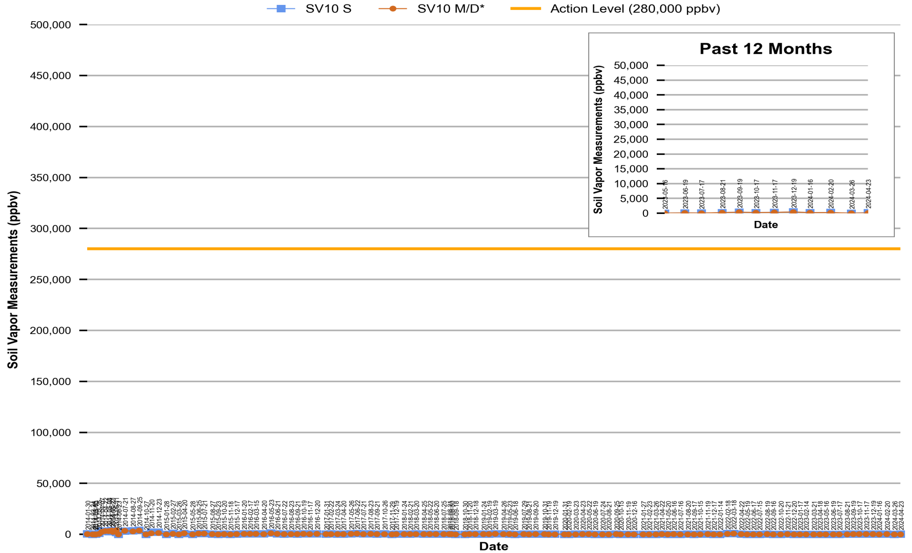
Figure 9 Red Hill - Tank 10 (JP-5) Soil Vapor Measurements (Jan 2014 Through Apr 2024)
