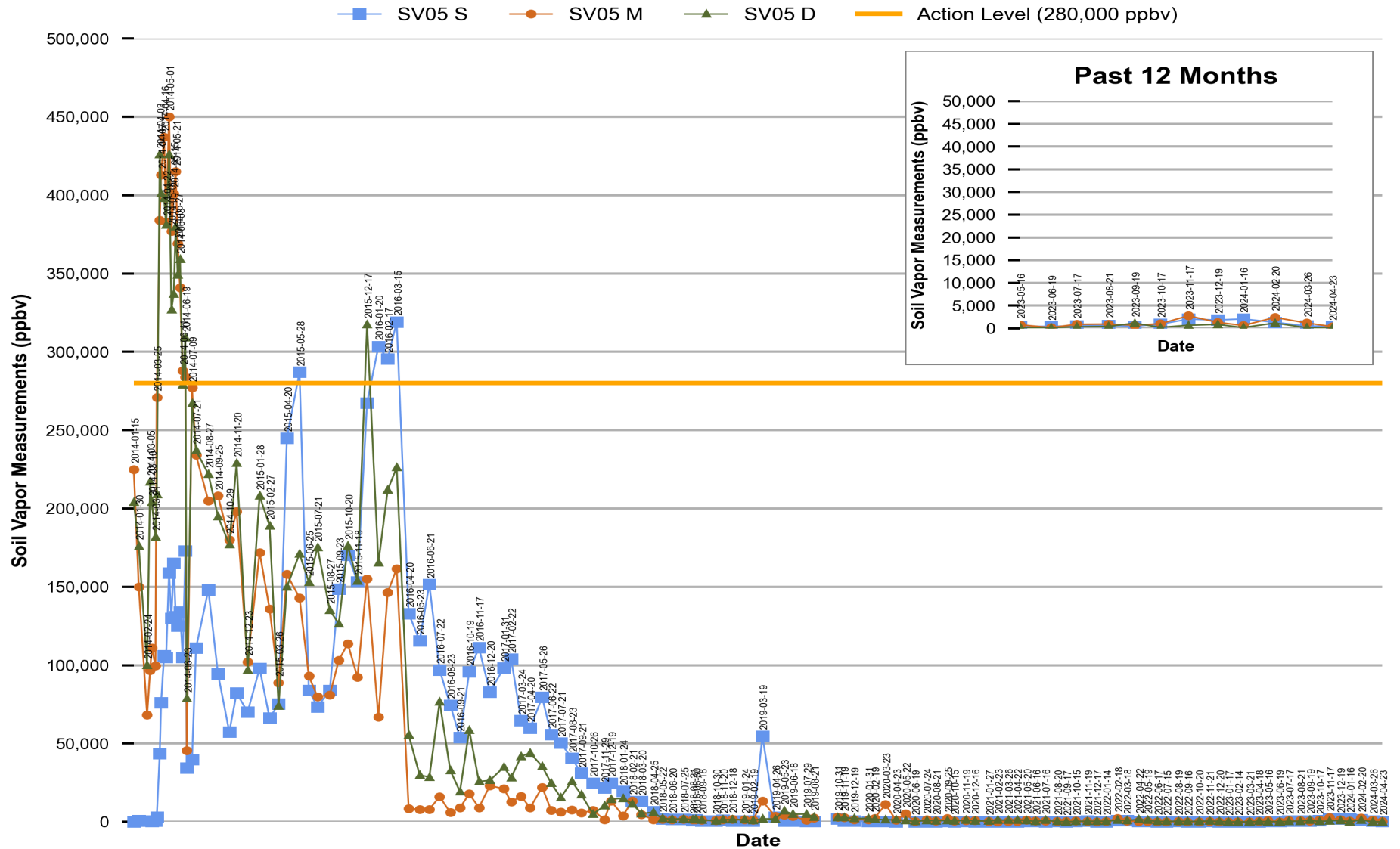
Figure 4 Red Hill - Tank 05 (F-24) Soil Vapor Measurements (Jan 2014 Through Apr 2024)
