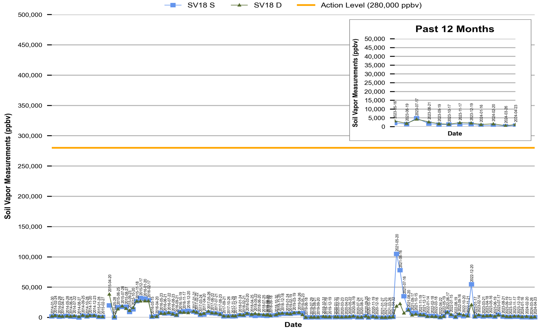
Figure 17 Red Hill - Tank 18 (JP-5) Soil Vapor Measurements (Jan 2014 Through Apr 2024)
