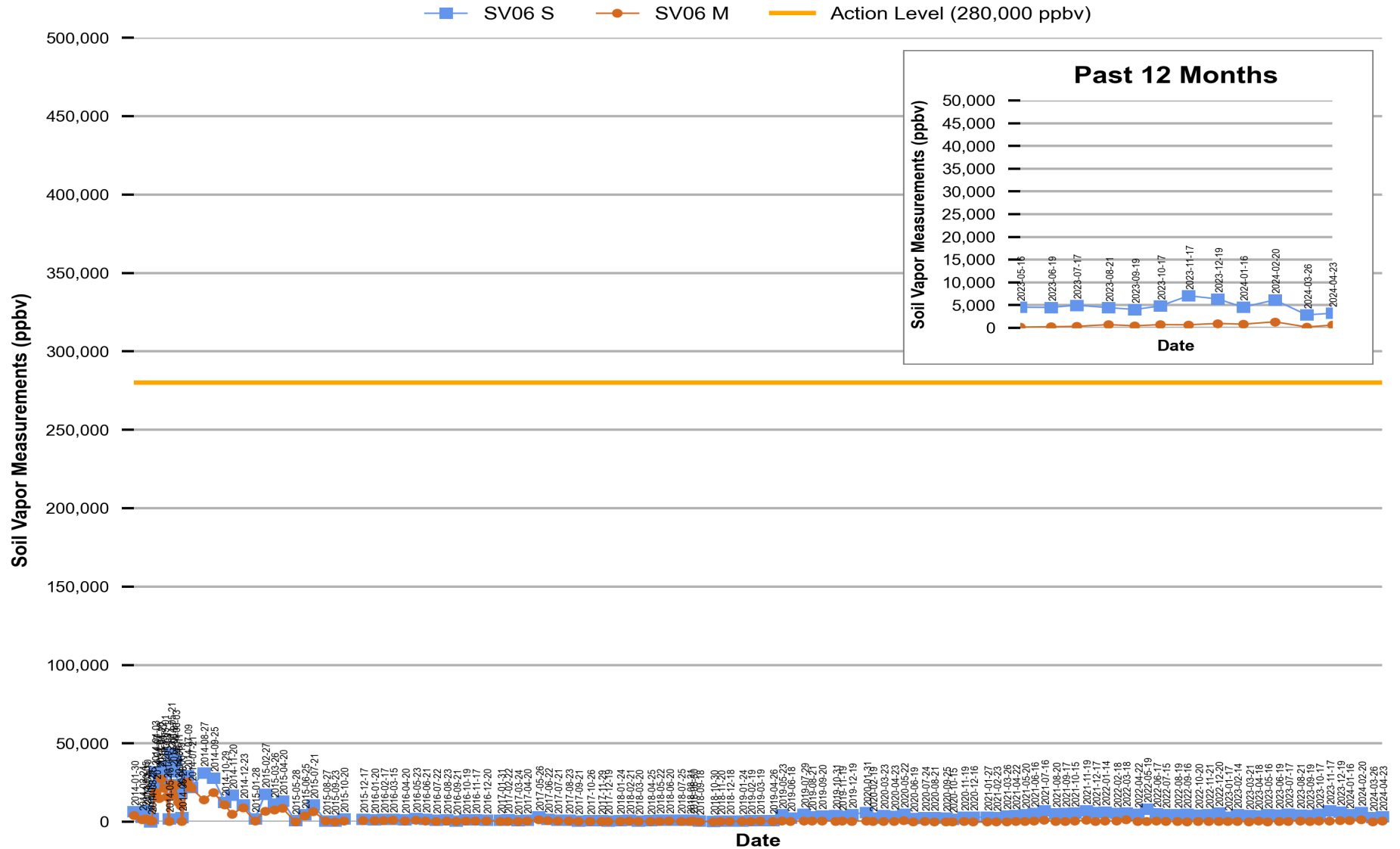
Figure 5 Red Hill - Tank 06 (F-24) Soil Vapor Measurements (Jan 2014 Through Apr 2024)
