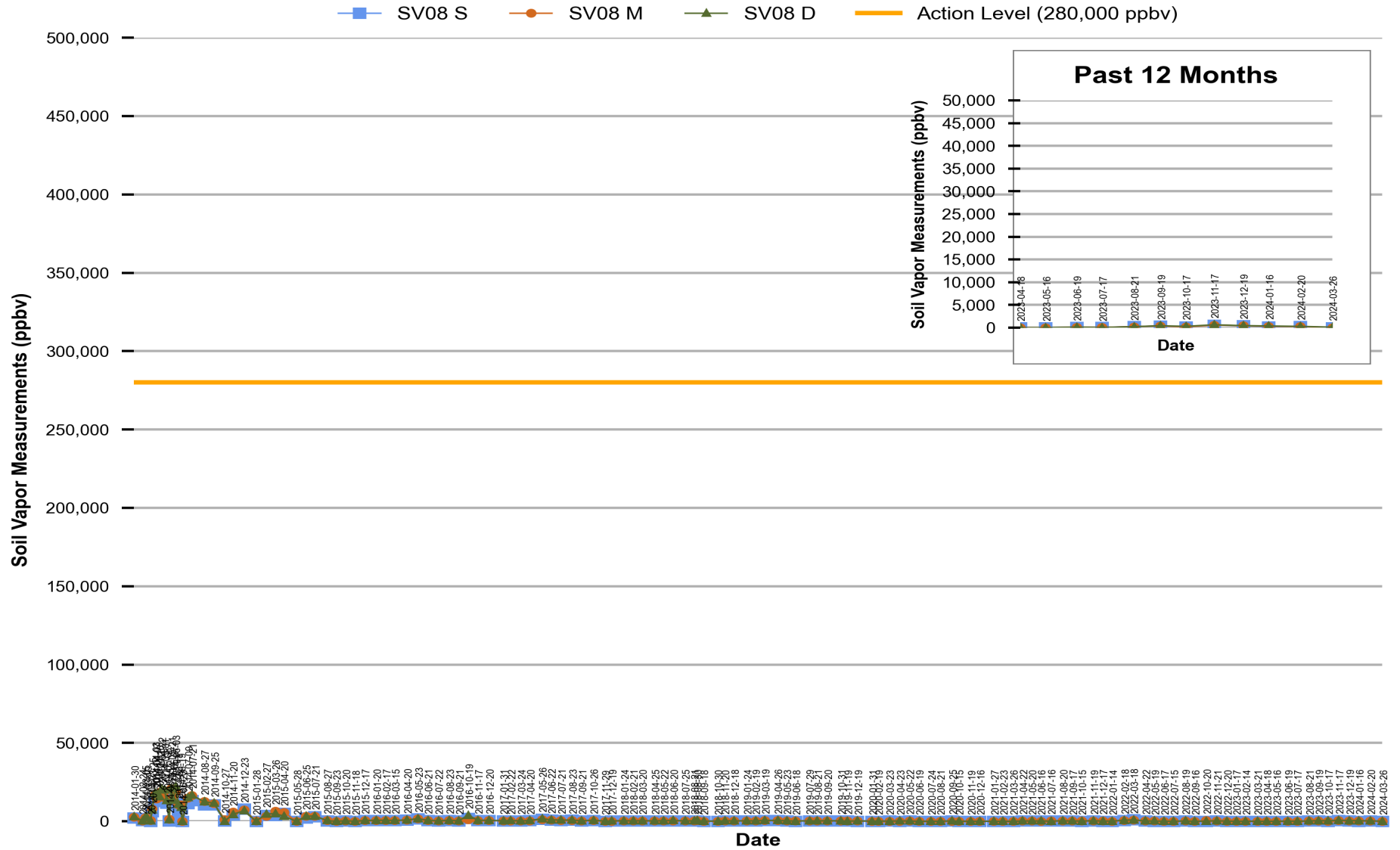
Figure 7 Red Hill - Tank 08 (JP-5) Soil Vapor Measurements (Jan 2014 Through Mar 2024)
