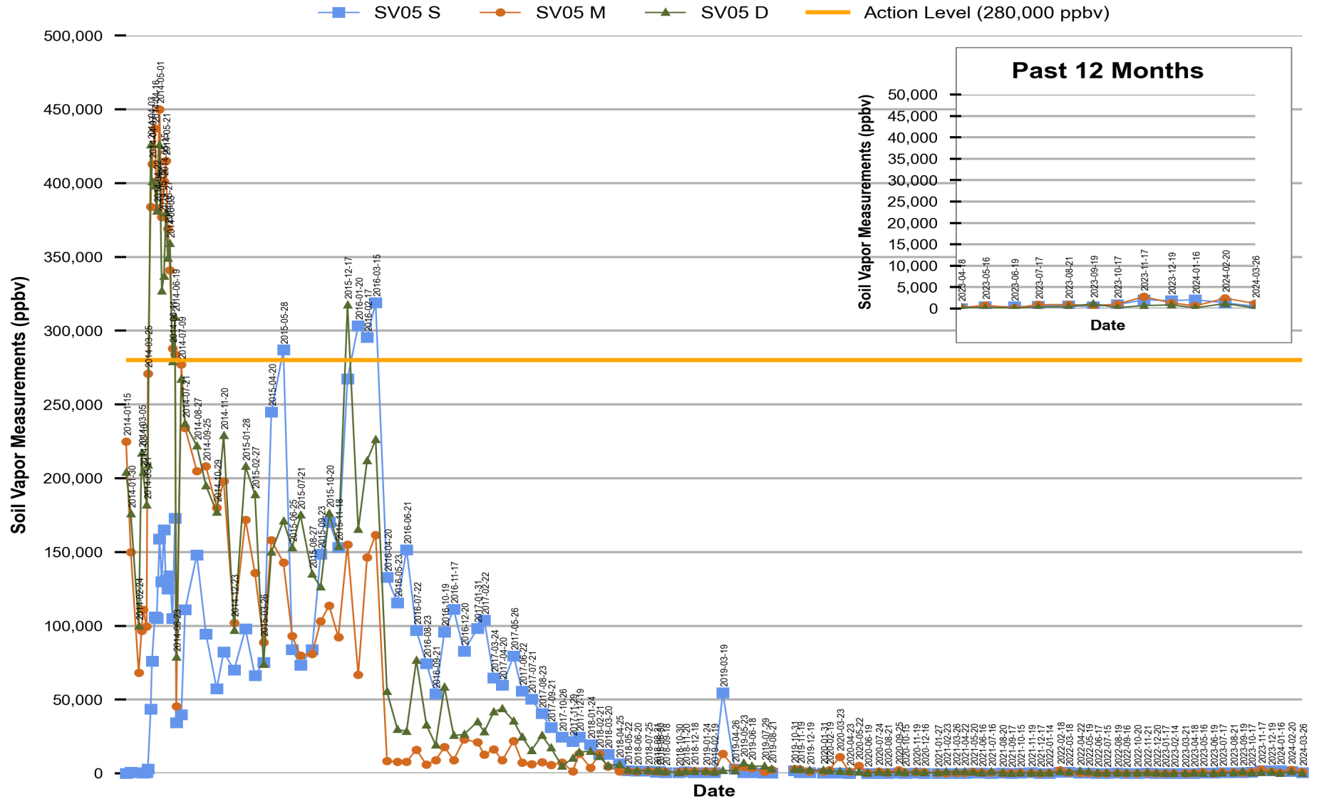
Figure 4 Red Hill - Tank 05 (F-24) Soil Vapor Measurements (Jan 2014 Through Mar 2024)
