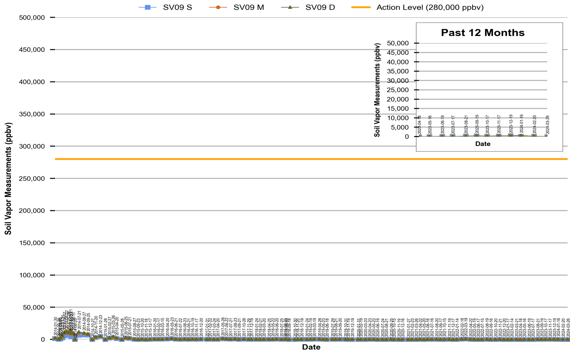
Figure 8 Red Hill - Tank 09 (JP-5) Soil Vapor Measurements (Jan 2014 Through Mar 2024)
