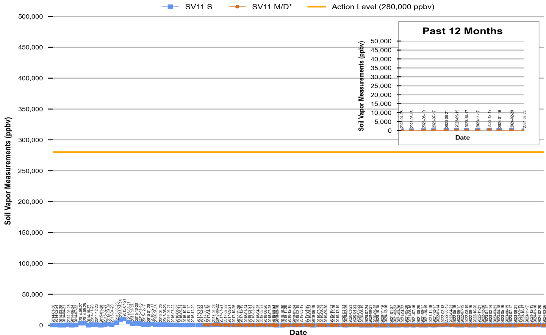
Figure 10 Red Hill - Tank 11 (JP-5) Soil Vapor Measurements (Jan 2014 Through Mar 2024)
