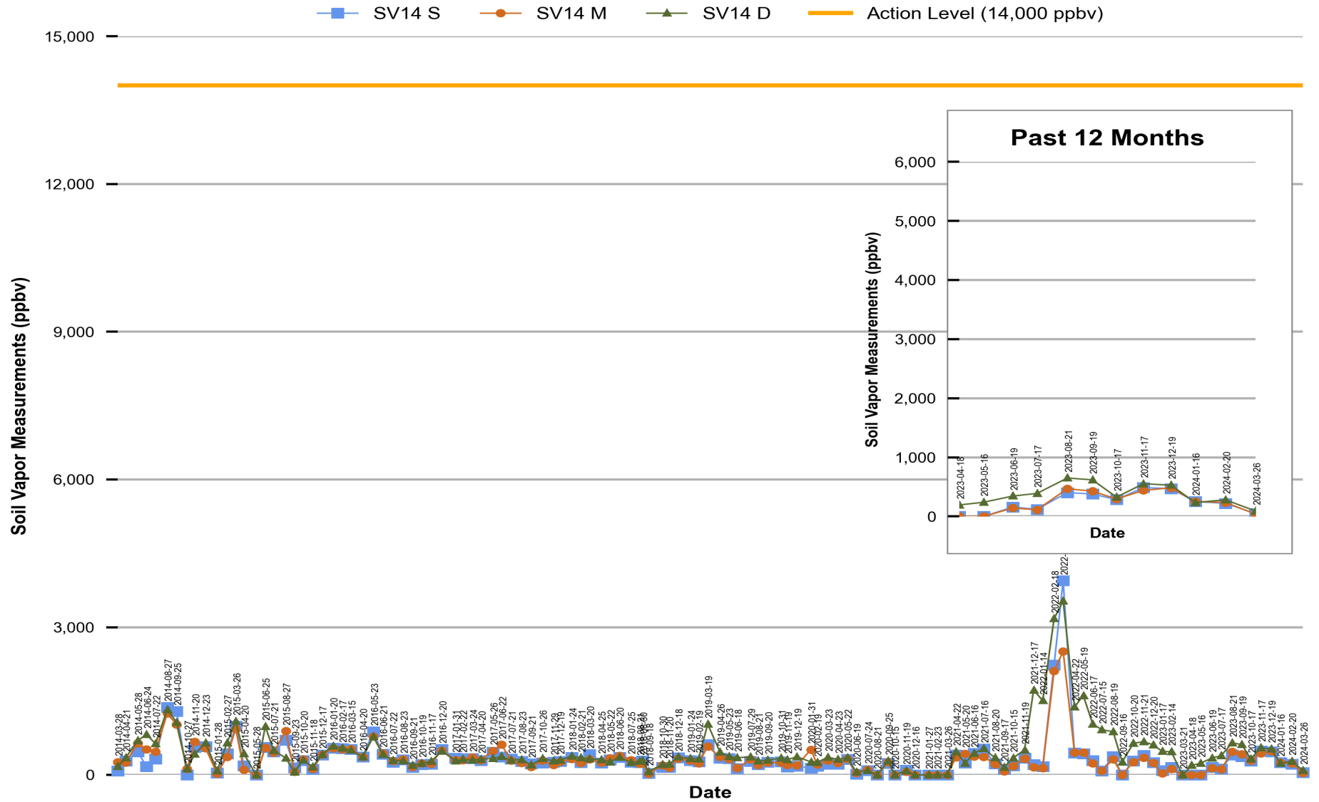
Figure 13 Red Hill - Tank 14 (F-76) Soil Vapor Measurements (Mar 2014 Through Mar 2024)
