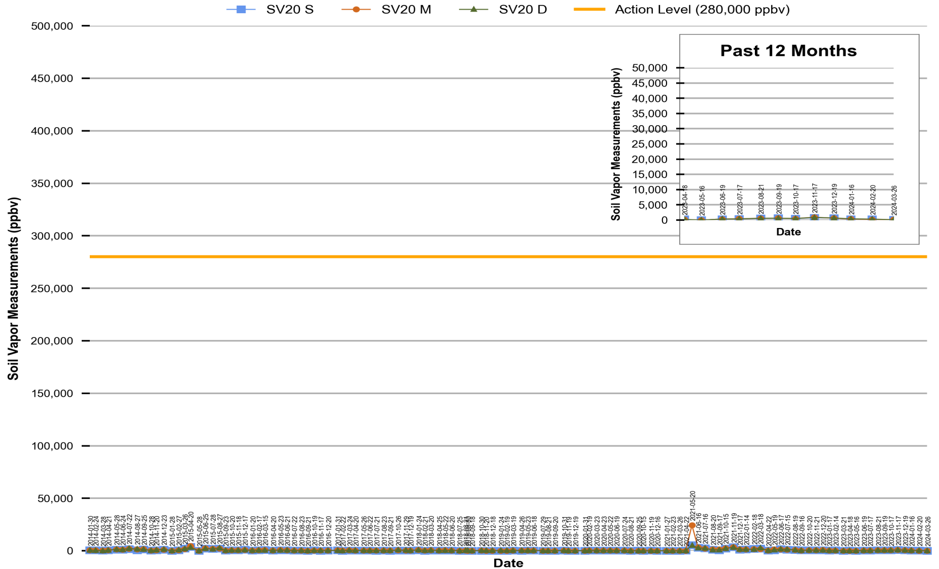
Figure 18 Red Hill - Tank 20 (JP-5) Soil Vapor Measurements (Jan 2014 Through Mar 2024)
