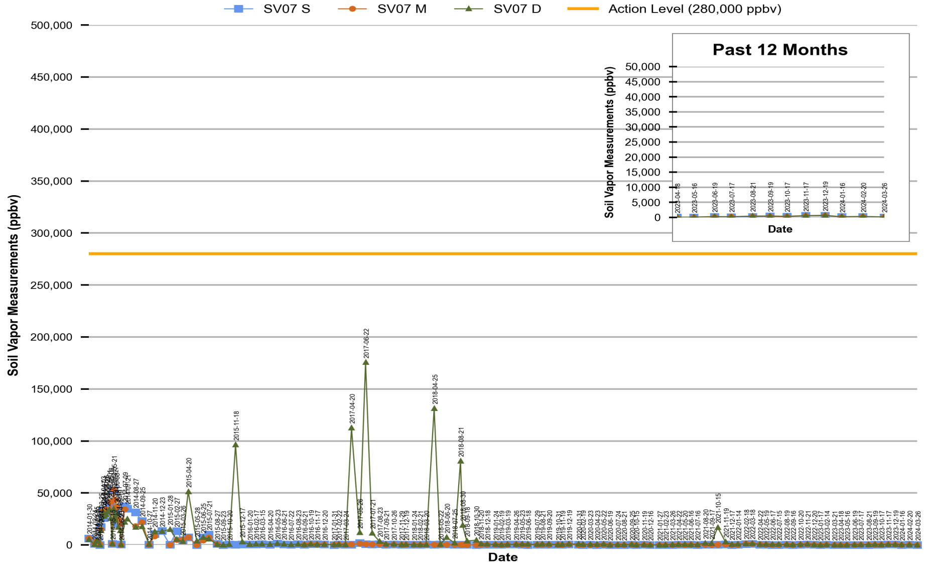
Figure 6 Red Hill - Tank 07 (JP-5) Soil Vapor Measurements (Jan 2014 Through Mar 2024)
