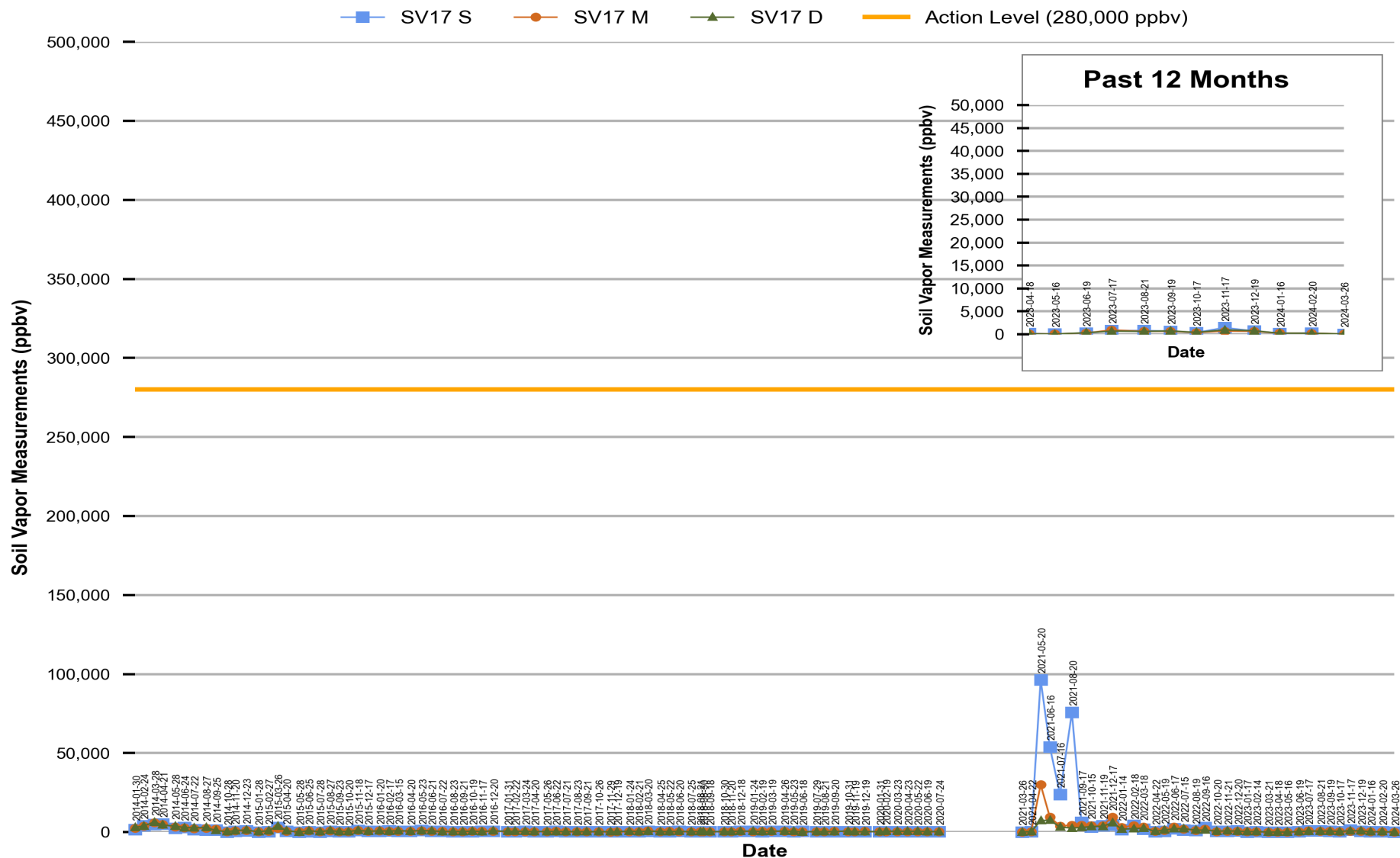
Figure 16 Red Hill - Tank 17 (JP-5) Soil Vapor Measurements (Jan 2014 Through Mar 2024)
