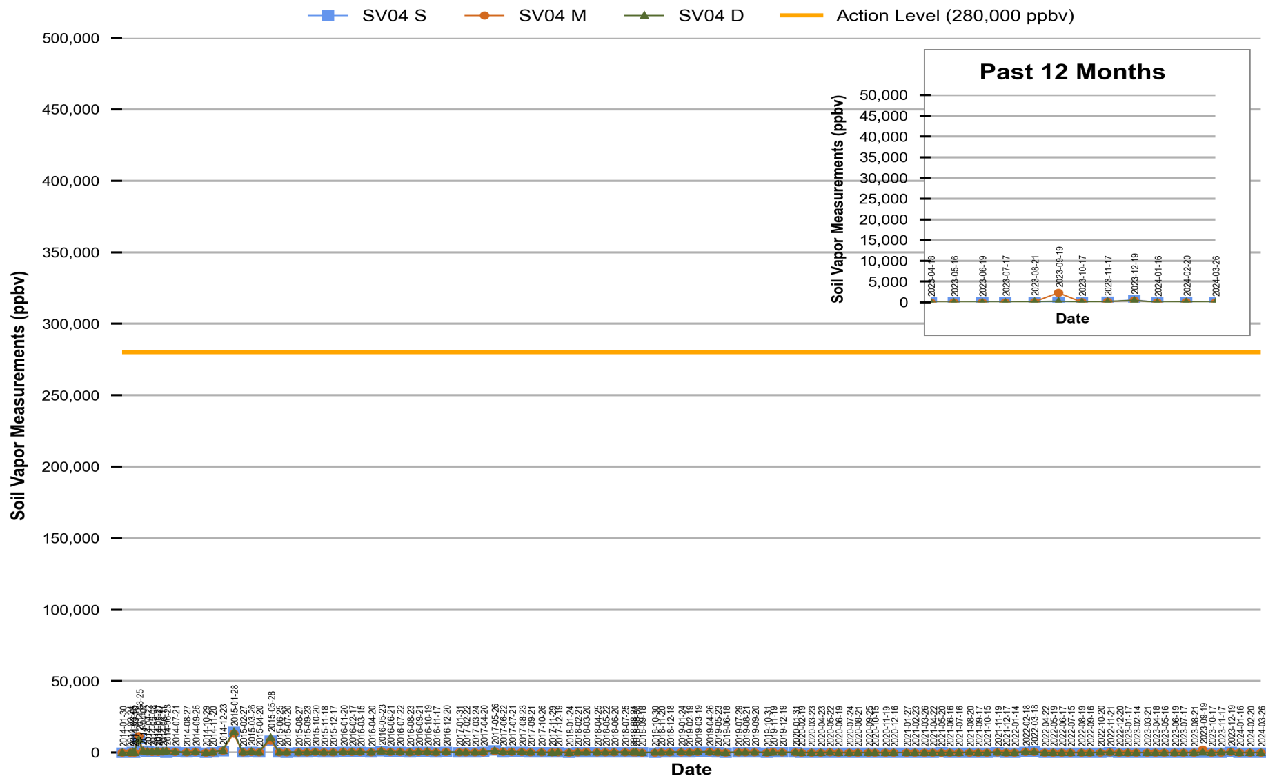
Figure 3 Red Hill - Tank 04 (F-24) Soil Vapor Measurements (Jan 2014 Through Mar 2024)
