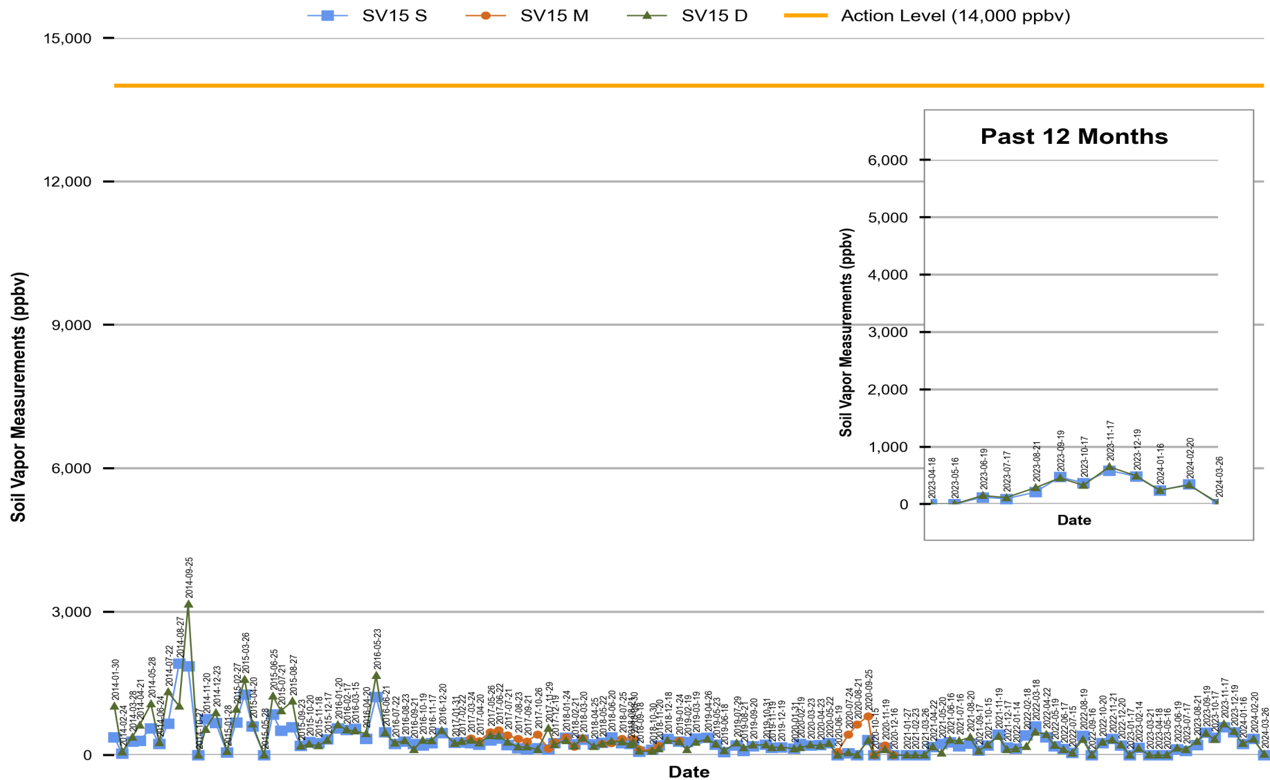
Figure 14 Red Hill - Tank 15 (F-76) Soil Vapor Measurements (Jan 2014 Through Mar 2024)
