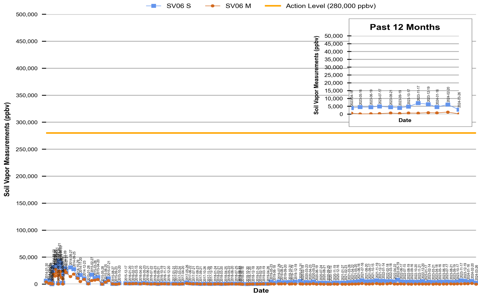
Figure 5 Red Hill - Tank 06 (F-24) Soil Vapor Measurements (Jan 2014 Through Mar 2024)
