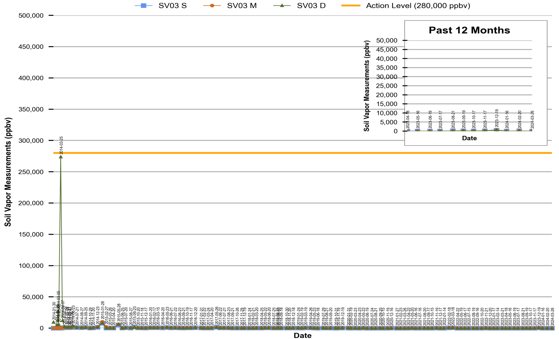
Figure 2 Red Hill - Tank 03 (F-24) Soil Vapor Measurements (Jan 2014 Through Mar 2024)
