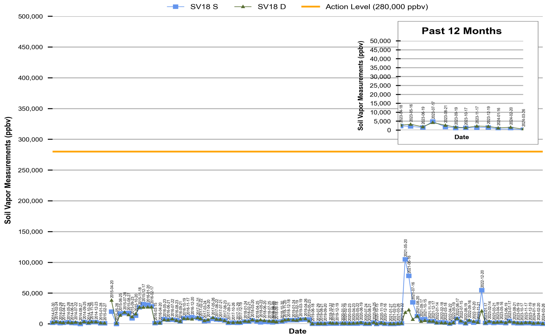
Figure 17 Red Hill - Tank 18 (JP-5) Soil Vapor Measurements (Jan 2014 Through Mar 2024)
