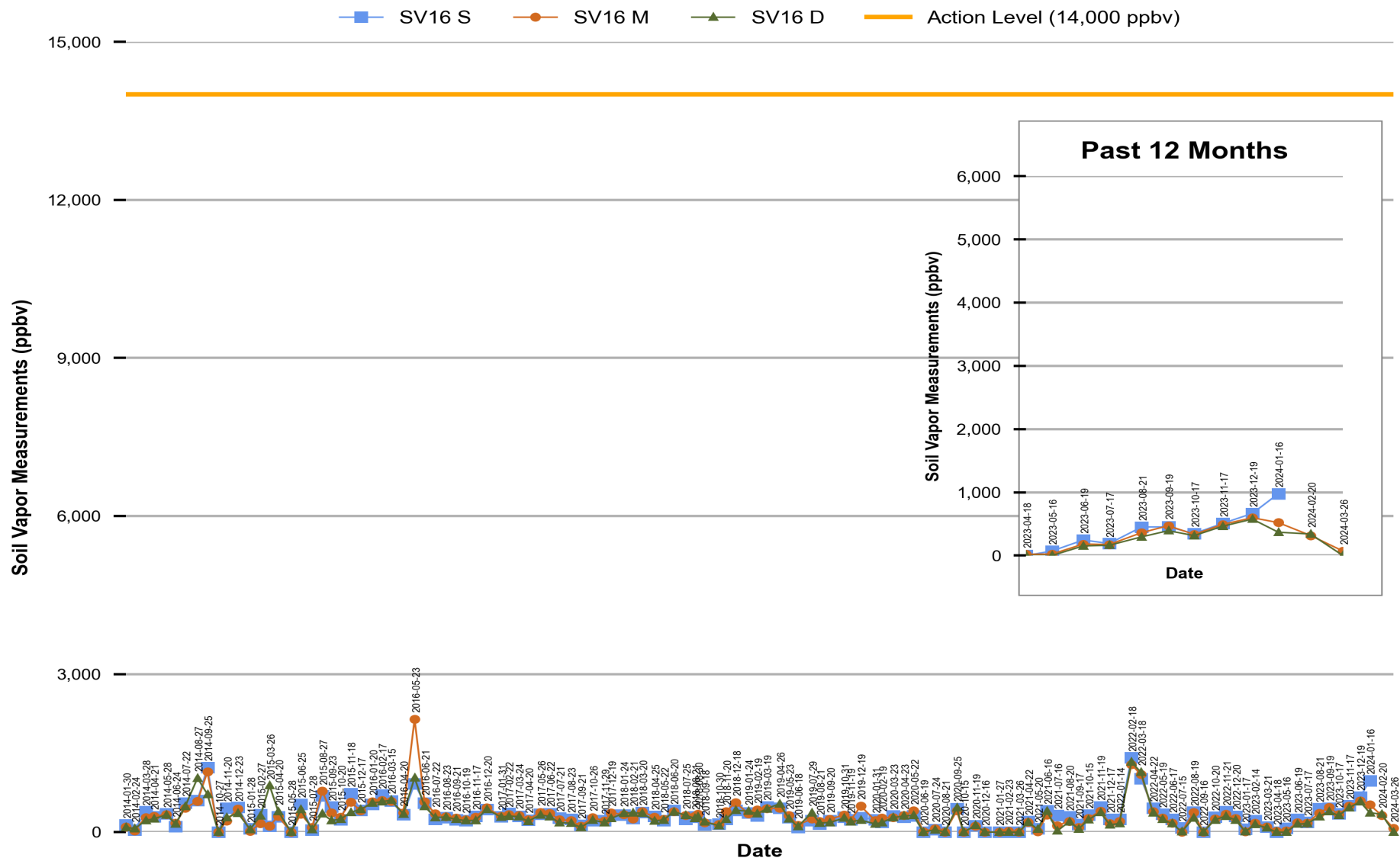
Figure 15 Red Hill - Tank 16 (F-76) Soil Vapor Measurements (Jan 2014 Through Mar 2024)
