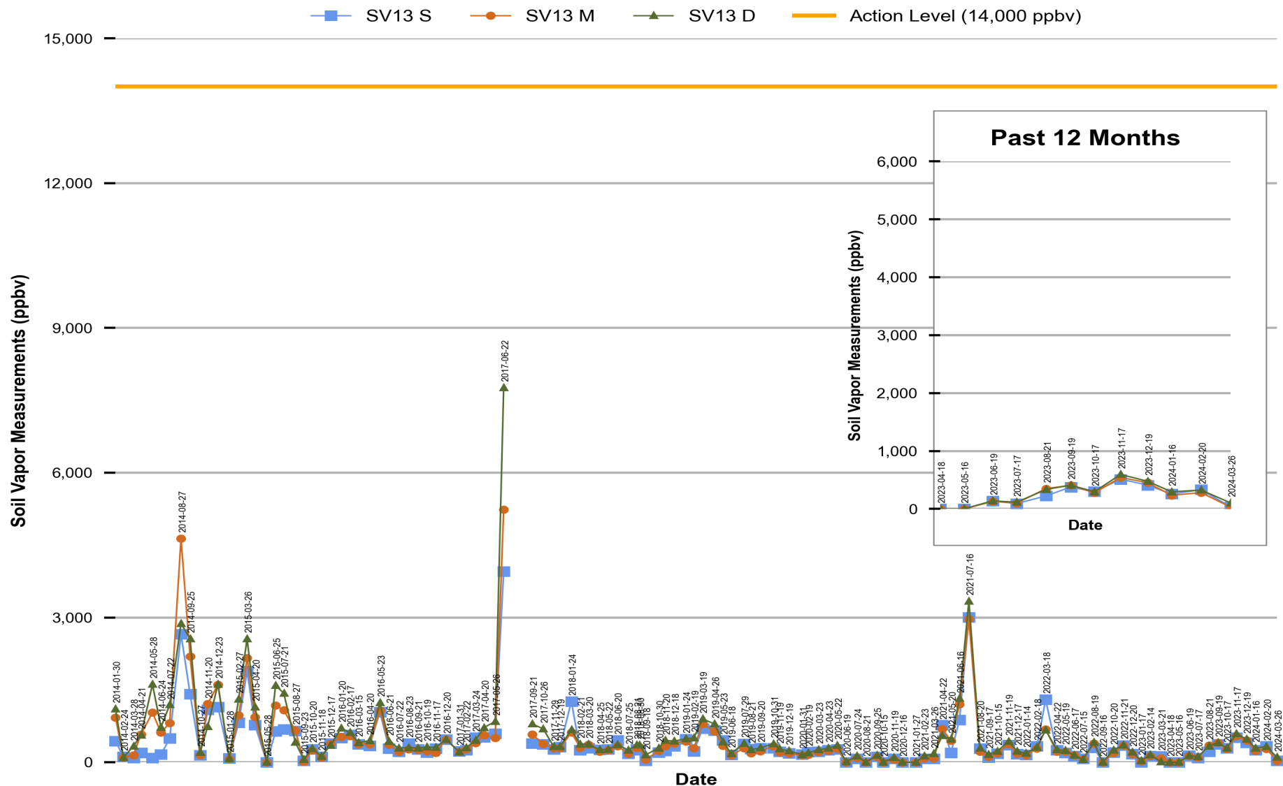
Figure 12 Red Hill - Tank 13 (F-76) Soil Vapor Measurements (Jan 2014 Through Mar 2024)
