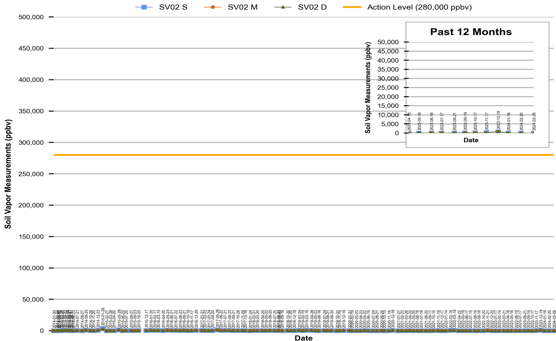
Figure 1 Red Hill - Tank 02 (F-24) Soil Vapor Measurements (Jan 2014 Through Mar 2024)
