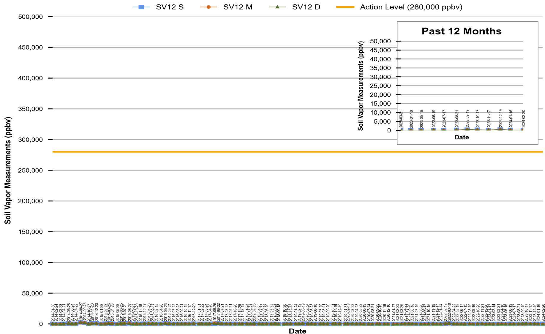
Figure 11 Red Hill - Tank 12 (JP-5) Soil Vapor Measurements (Jan 2014 Through Feb 2024)
