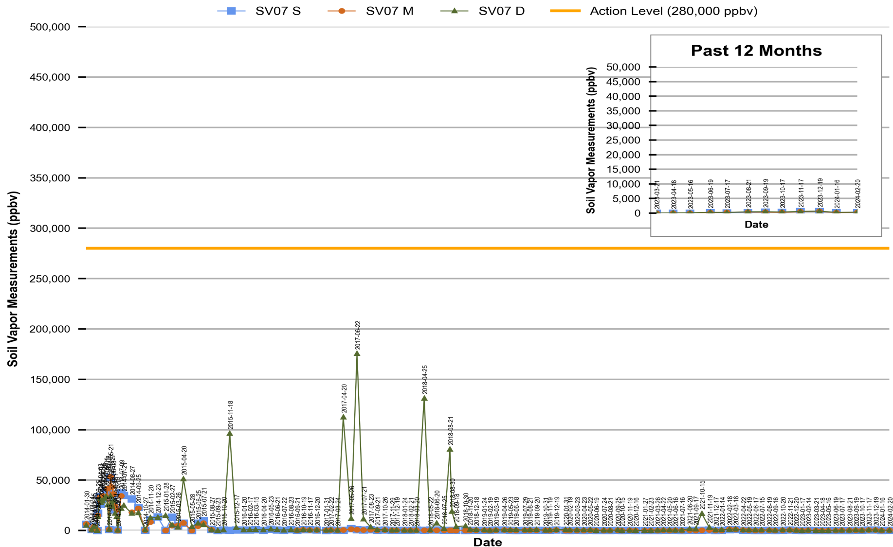
Figure 6 Red Hill - Tank 07 (JP-5) Soil Vapor Measurements (Jan 2014 Through Feb 2024)
