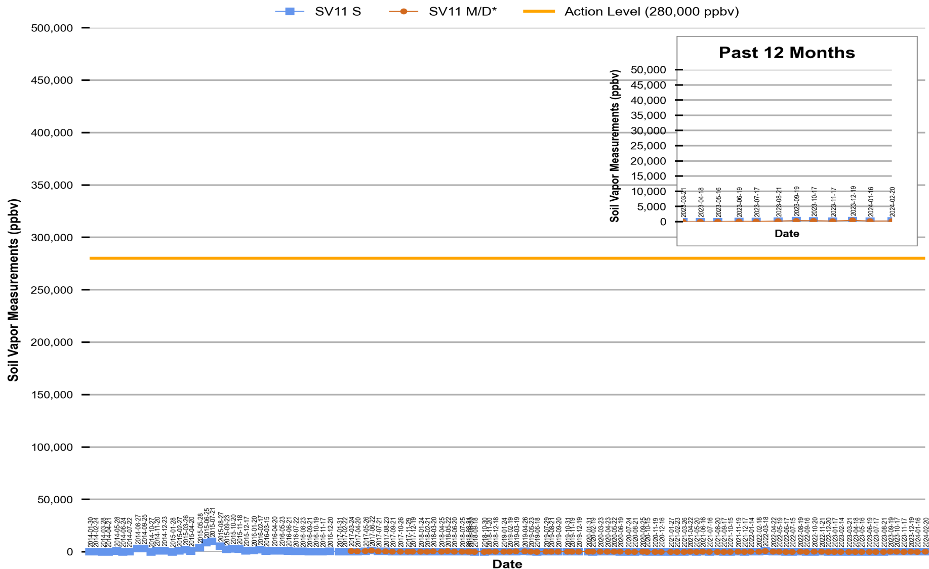
Figure 10 Red Hill - Tank 11 (JP-5) Soil Vapor Measurements (Jan 2014 Through Feb 2024)
