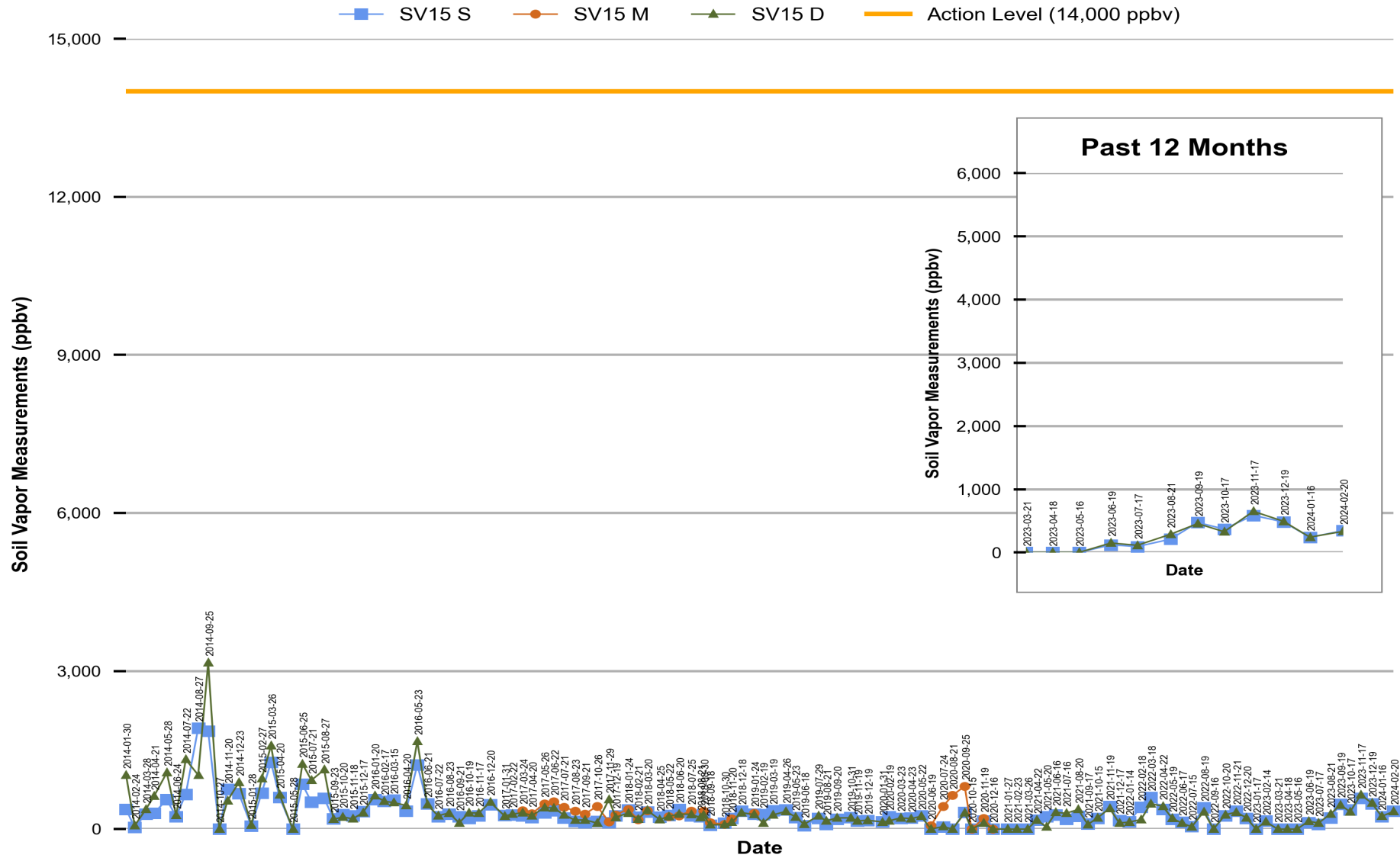
Figure 14 Red Hill - Tank 15 (F-76) Soil Vapor Measurements (Jan 2014 Through Feb 2024)
