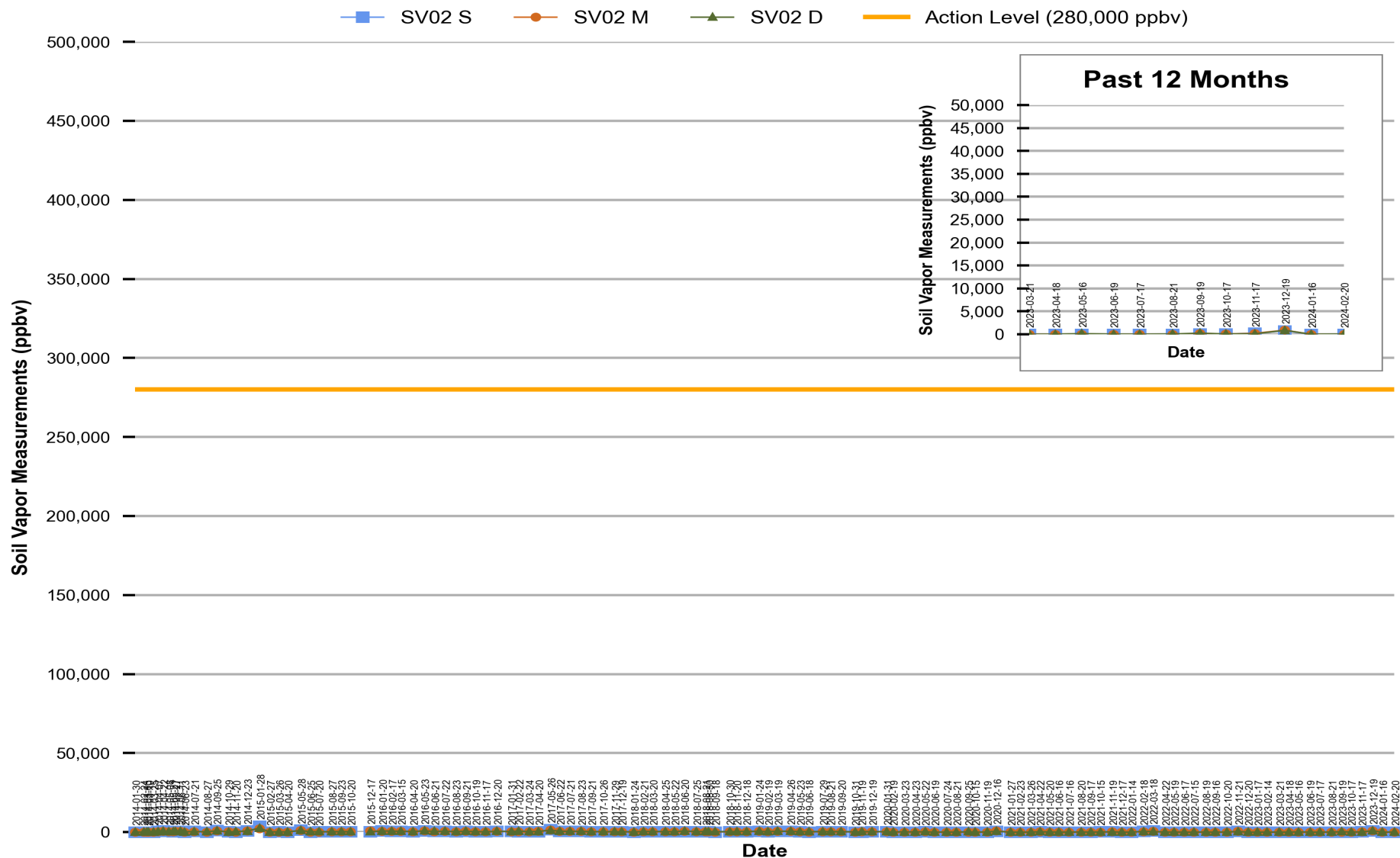
Figure 1 Red Hill - Tank 02 (F-24) Soil Vapor Measurements (Jan 2014 Through Feb 2024)
