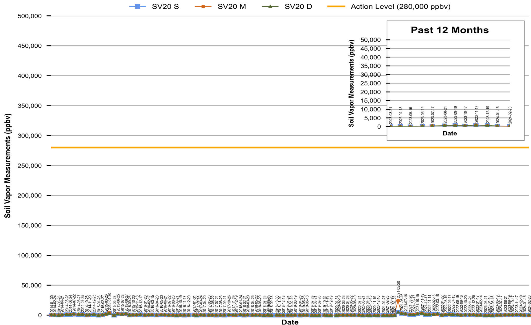
Figure 18 Red Hill - Tank 20 (JP-5) Soil Vapor Measurements (Jan 2014 Through Feb 2024)
