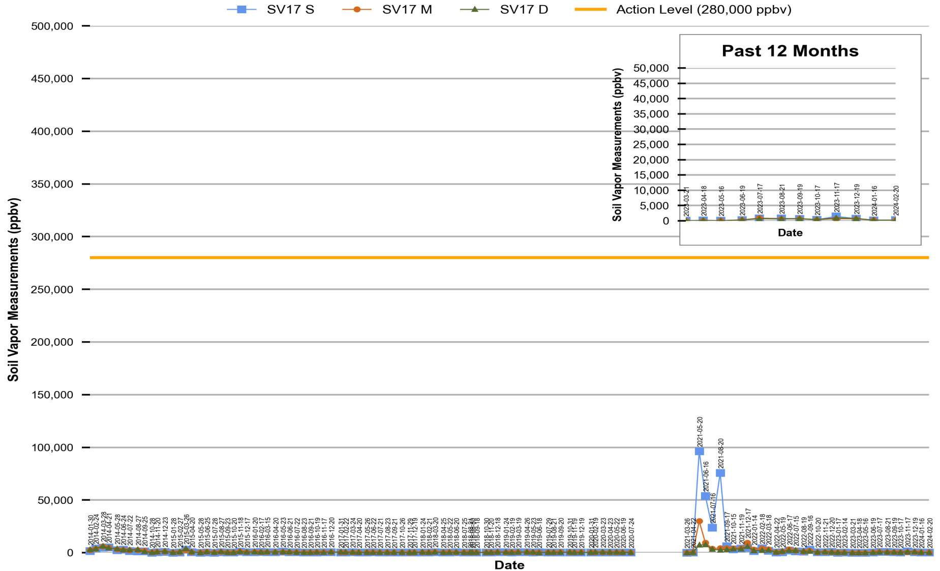
Figure 16 Red Hill - Tank 17 (JP-5) Soil Vapor Measurements (Jan 2014 Through Feb 2024)
