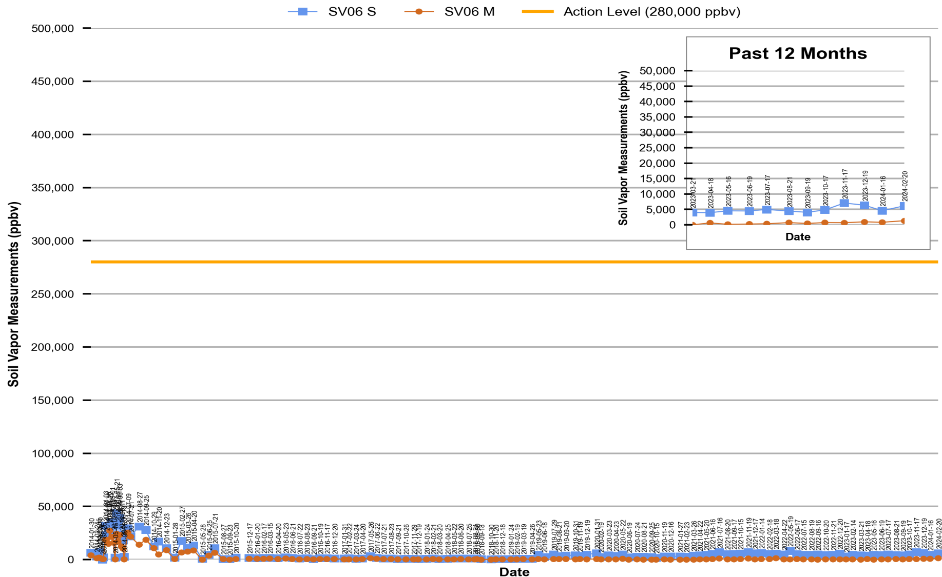
Figure 5 Red Hill - Tank 06 (F-24) Soil Vapor Measurements (Jan 2014 Through Feb 2024)
