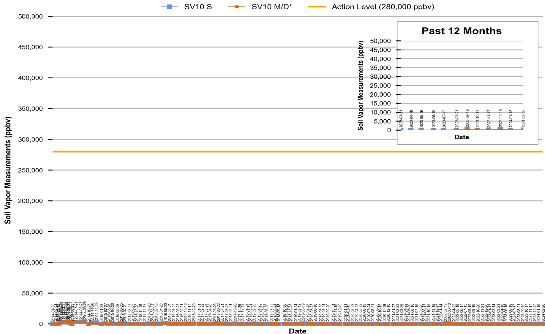
Figure 9 Red Hill - Tank 10 (JP-5) Soil Vapor Measurements (Jan 2014 Through Feb 2024)
