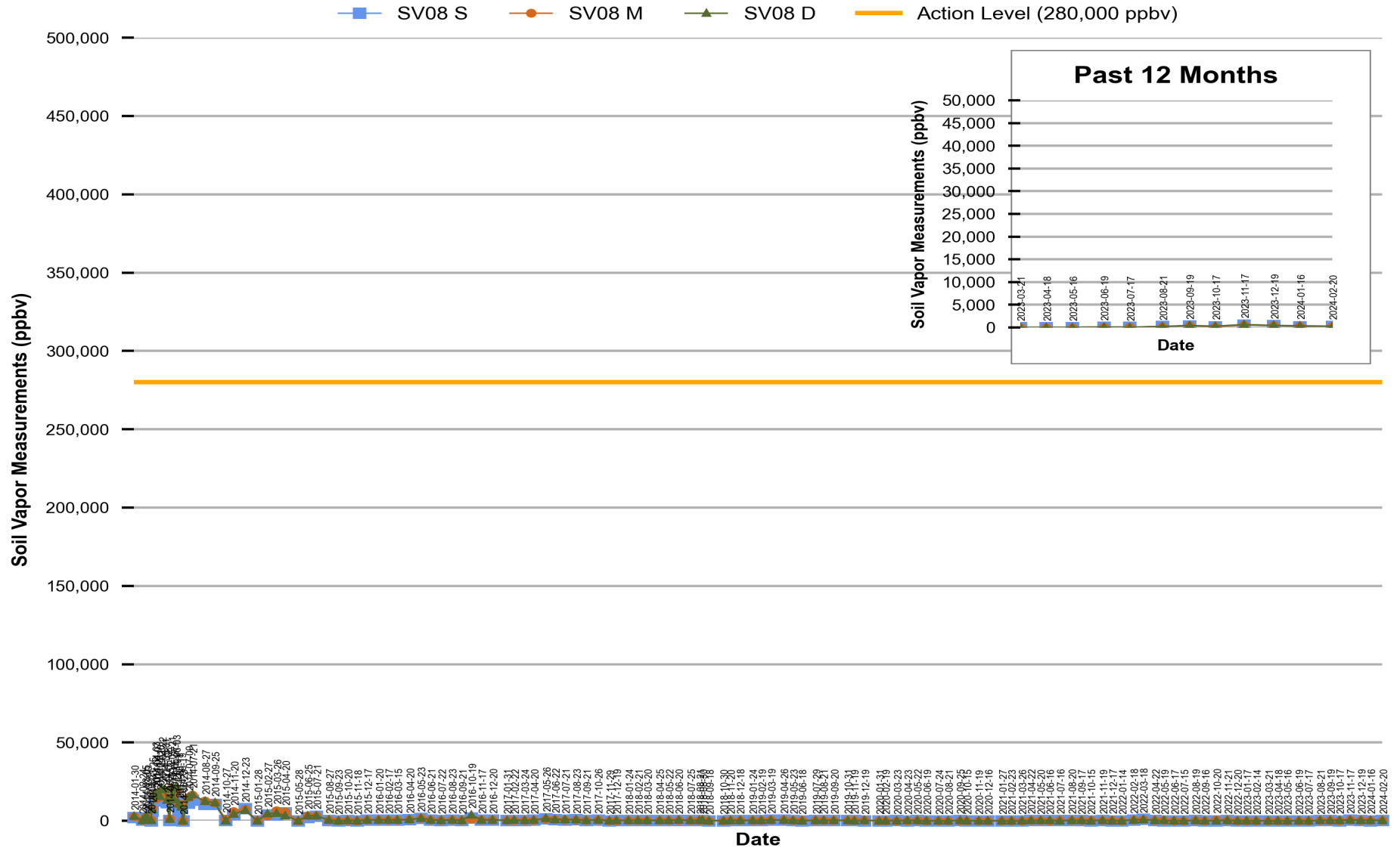
Figure 7 Red Hill - Tank 08 (JP-5) Soil Vapor Measurements (Jan 2014 Through Feb 2024)
