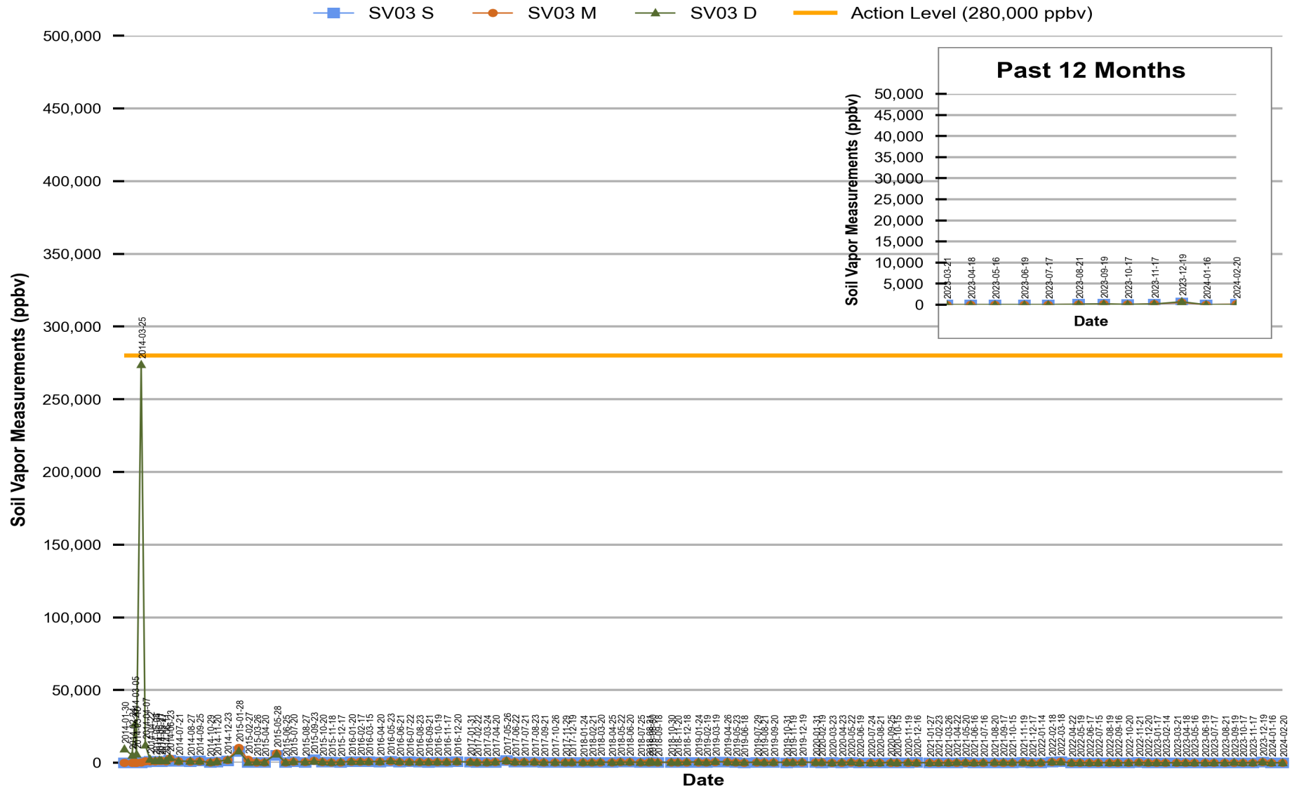
Figure 2 Red Hill - Tank 03 (F-24) Soil Vapor Measurements (Jan 2014 Through Feb 2024)
