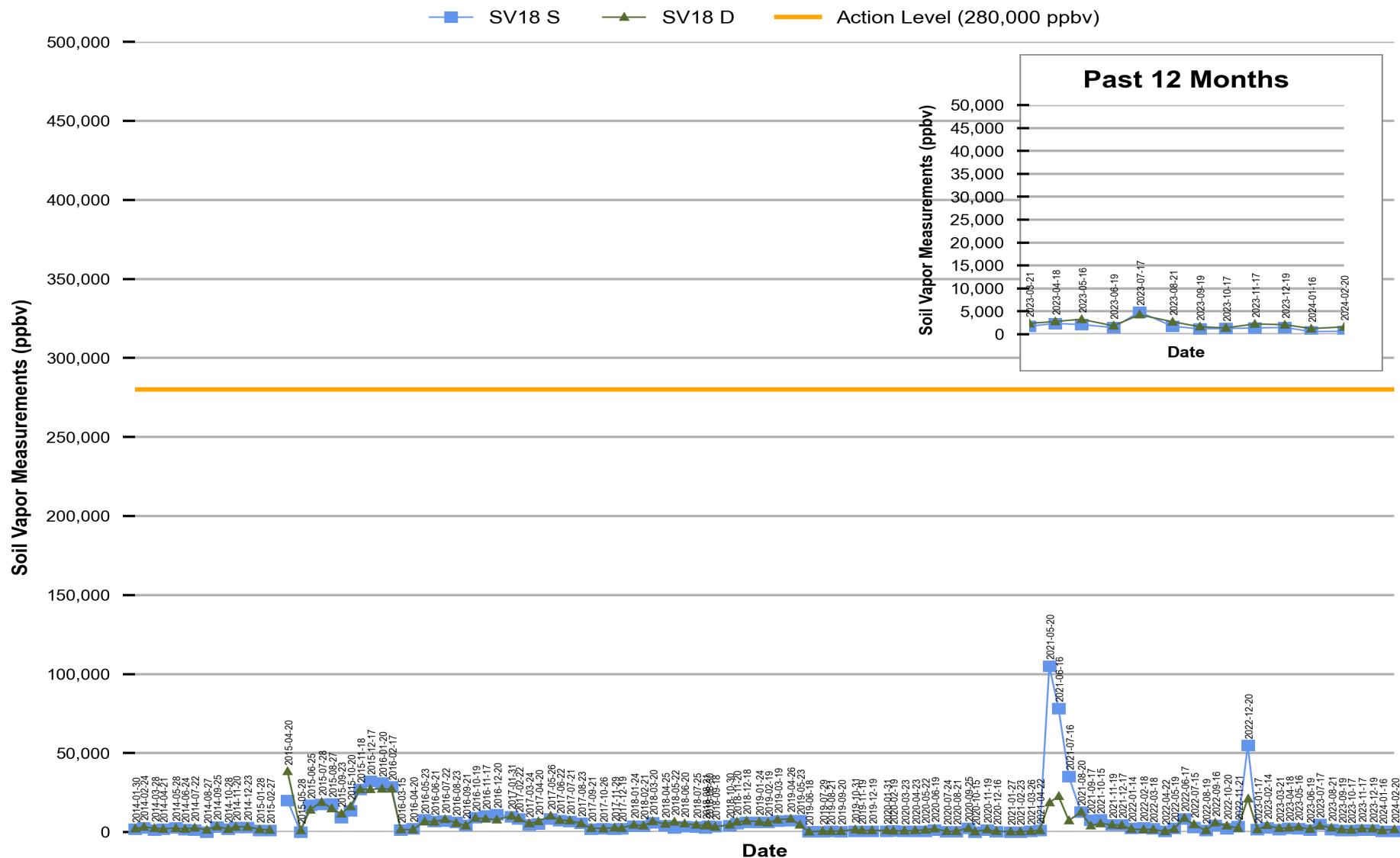
Figure 17 Red Hill - Tank 18 (JP-5) Soil Vapor Measurements (Jan 2014 Through Feb 2024)
