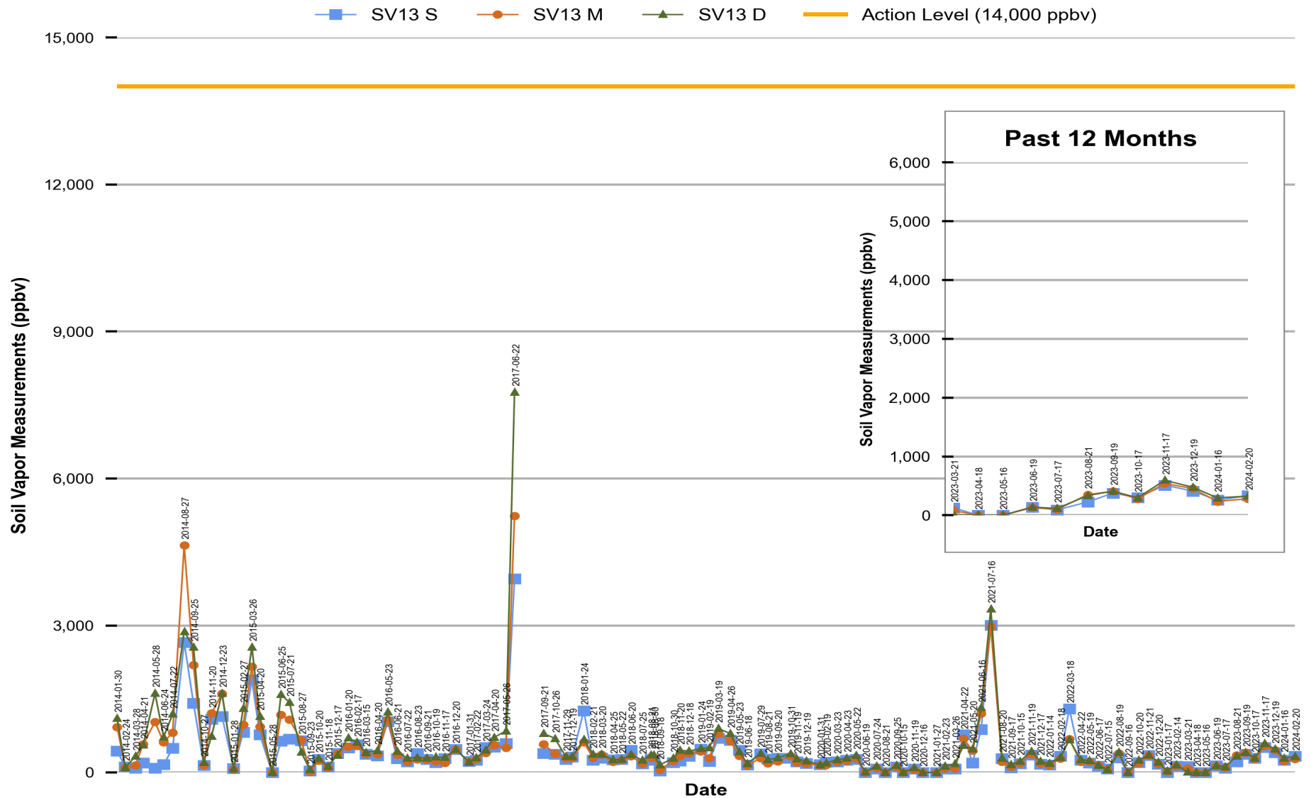
Figure 12 Red Hill - Tank 13 (F-76) Soil Vapor Measurements (Jan 2014 Through Feb 2024)
