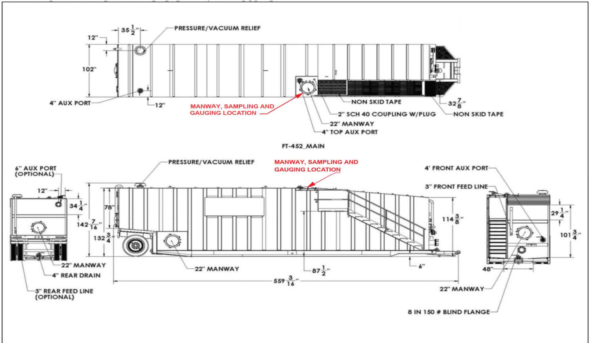
Figure 3: Tank Layout
