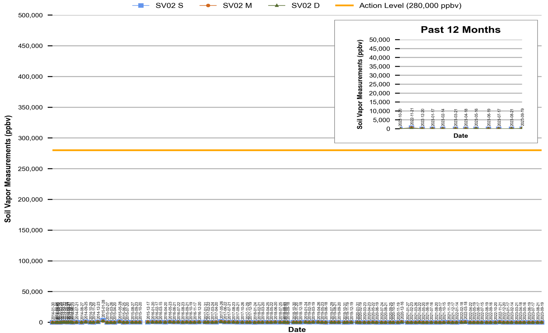
Figure 1 Red Hill - Tank 02 (F-24) Soil Vapor Measurements (Jan 2014 Through Sep 2023)
