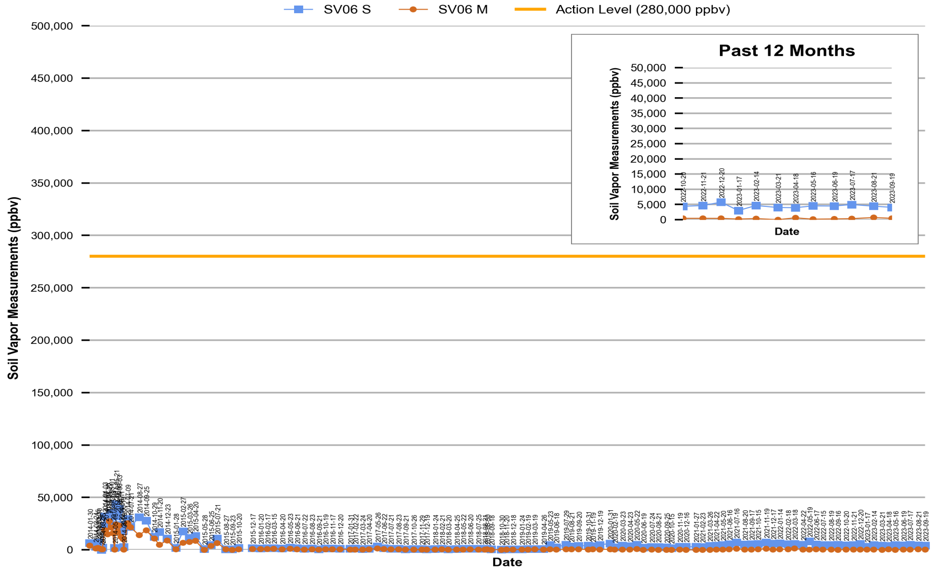
Figure 5 Red Hill - Tank 06 (F-24) Soil Vapor Measurements (Jan 2014 Through Sep 2023)
