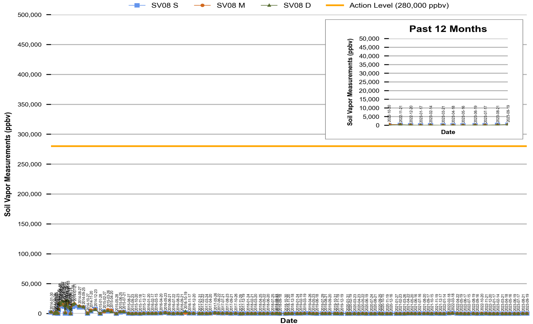
Figure 7 Red Hill - Tank 08 (JP-5) Soil Vapor Measurements (Jan 2014 Through Sep 2023)
