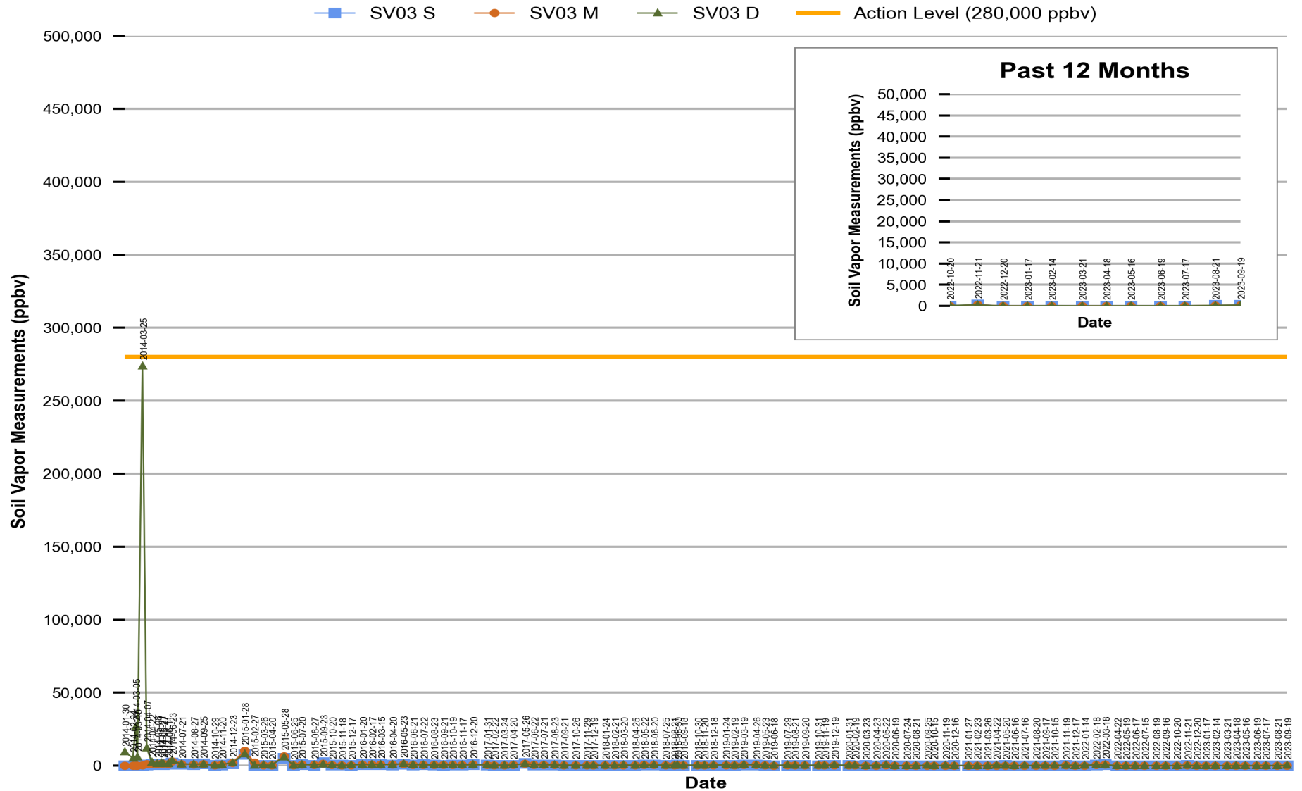
Figure 2 Red Hill - Tank 03 (F-24) Soil Vapor Measurements (Jan 2014 Through Sep 2023)
