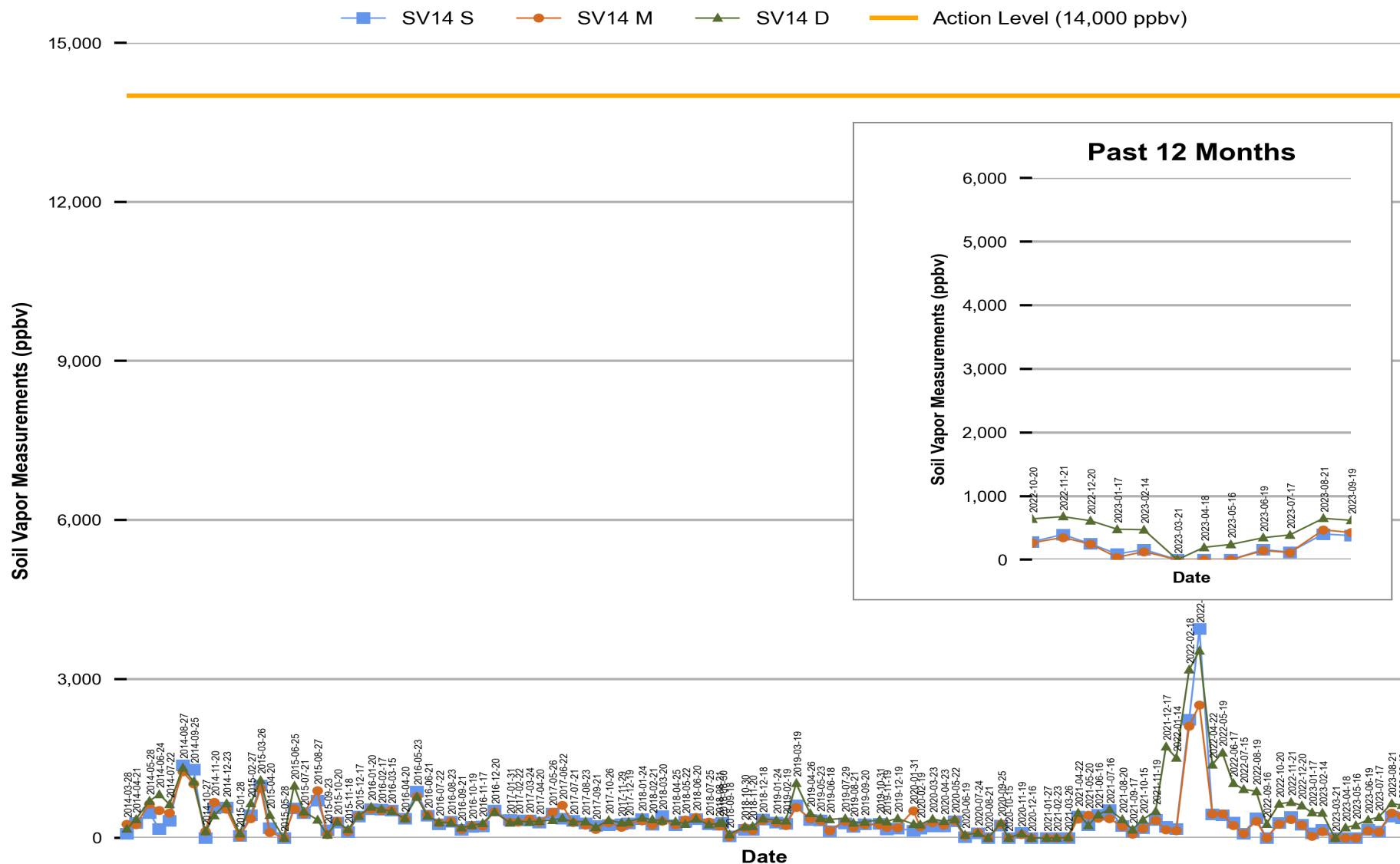
Figure 13 Red Hill - Tank 14 (F-76) EMPTY Soil Vapor Measurements (Mar 2014 Through Sep 2023)
