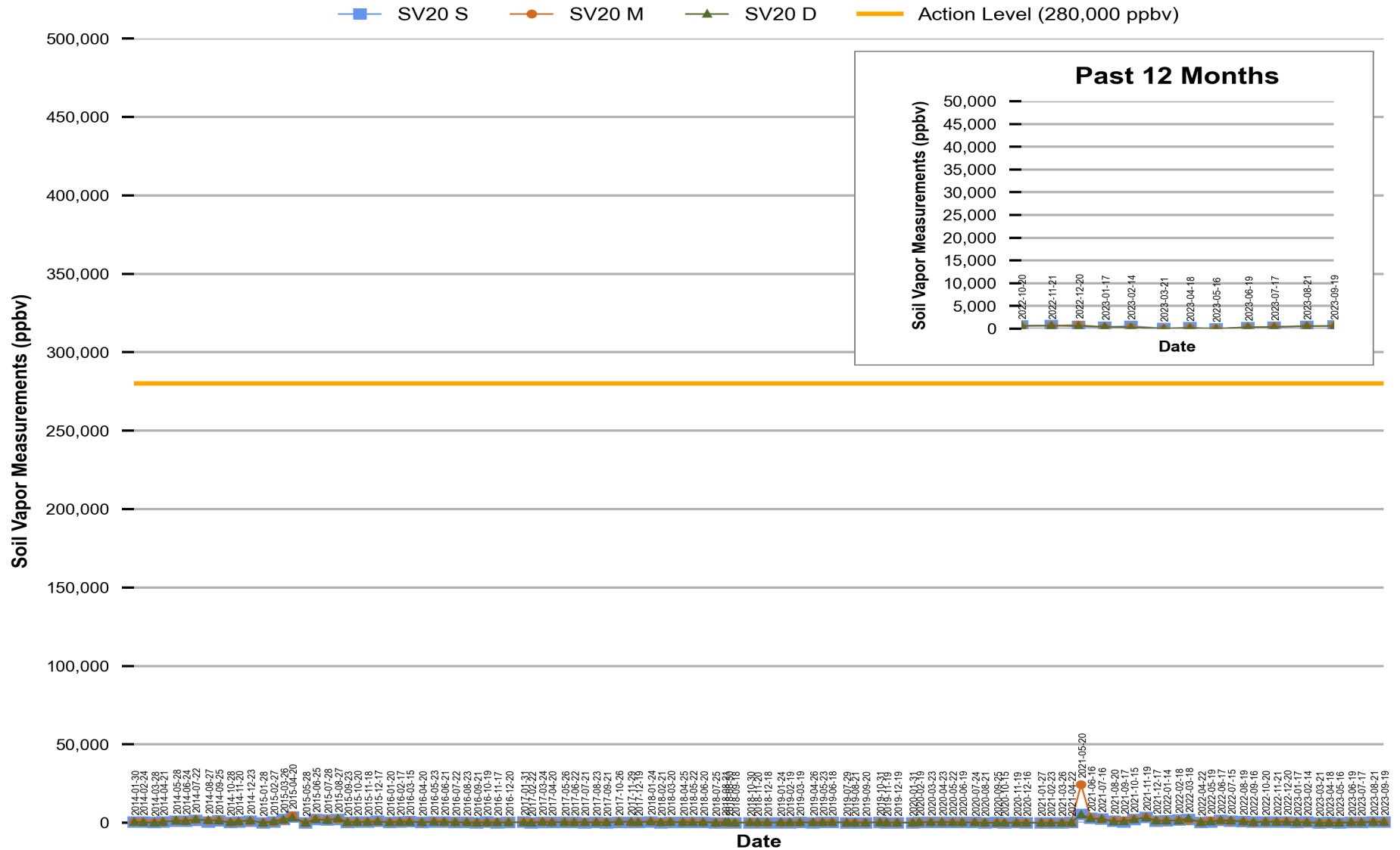
Figure 18 Red Hill - Tank 20 (JP-5) Soil Vapor Measurements (Jan 2014 Through Sep 2023)
