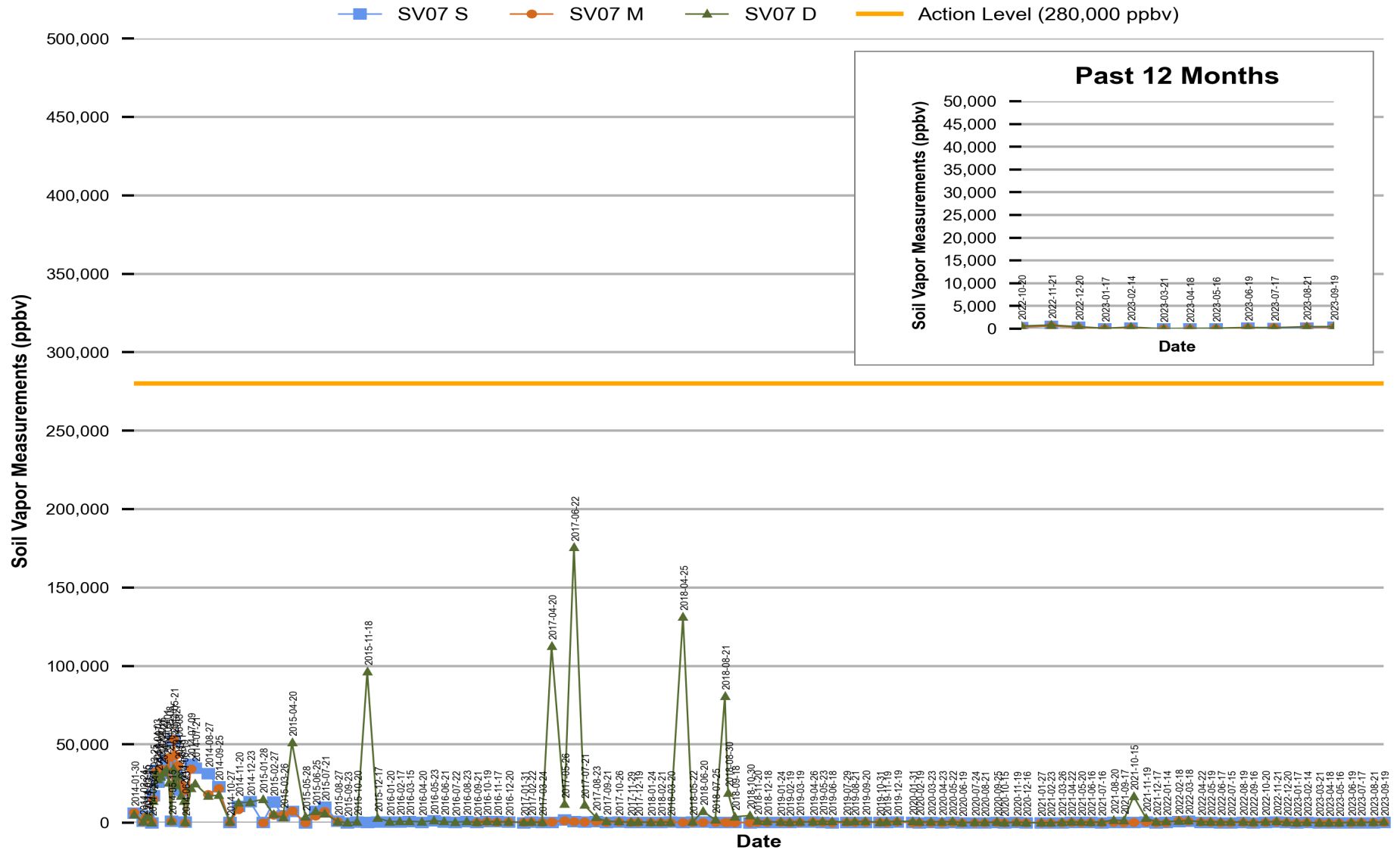
Figure 6 Red Hill - Tank 07 (JP-5) Soil Vapor Measurements (Jan 2014 Through Sep 2023)
