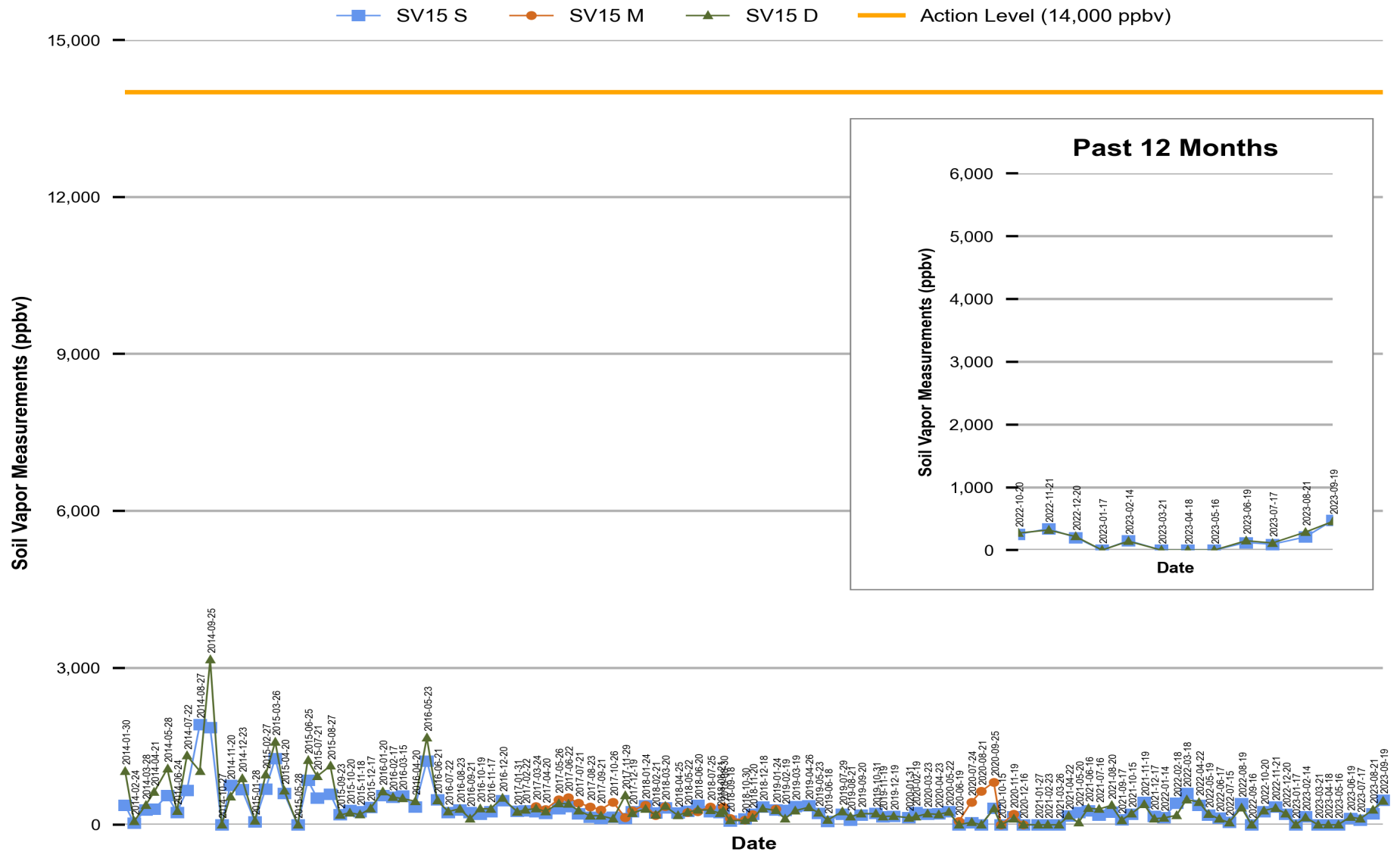
Figure 14 Red Hill - Tank 15 (F-76) EMPTY Soil Vapor Measurements (Jan 2014 Through Sep 2023)
