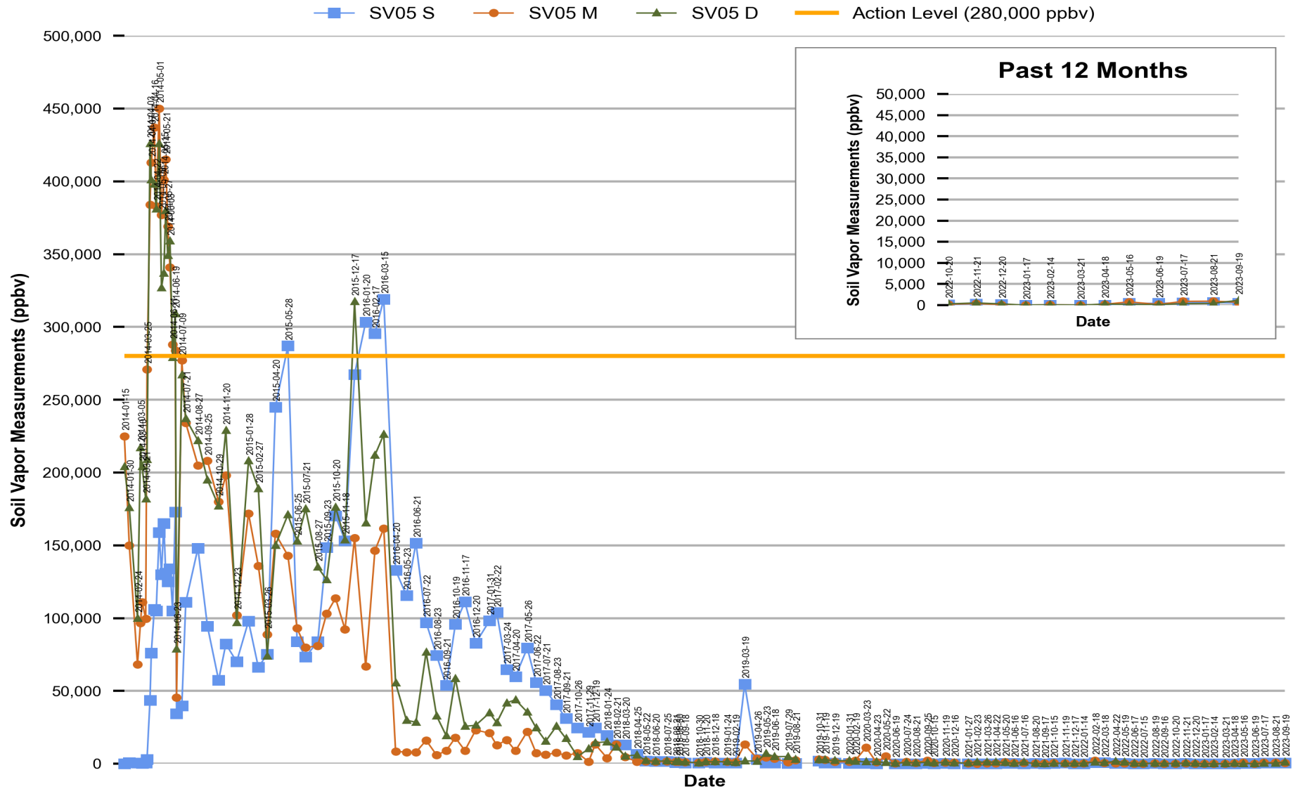
Figure 4 Red Hill - Tank 05 (F-24) Soil Vapor Measurements (Jan 2014 Through Sep 2023)
