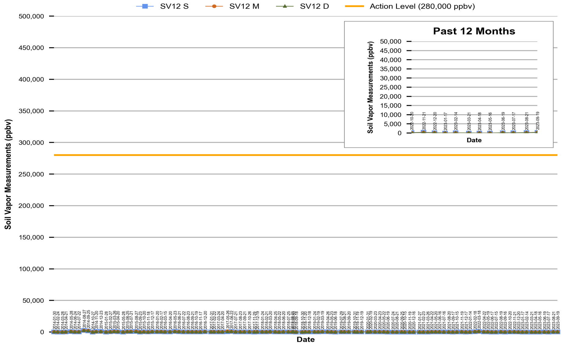
Figure 11 Red Hill - Tank 12 (JP-5) Soil Vapor Measurements (Jan 2014 Through Sep 2023)
