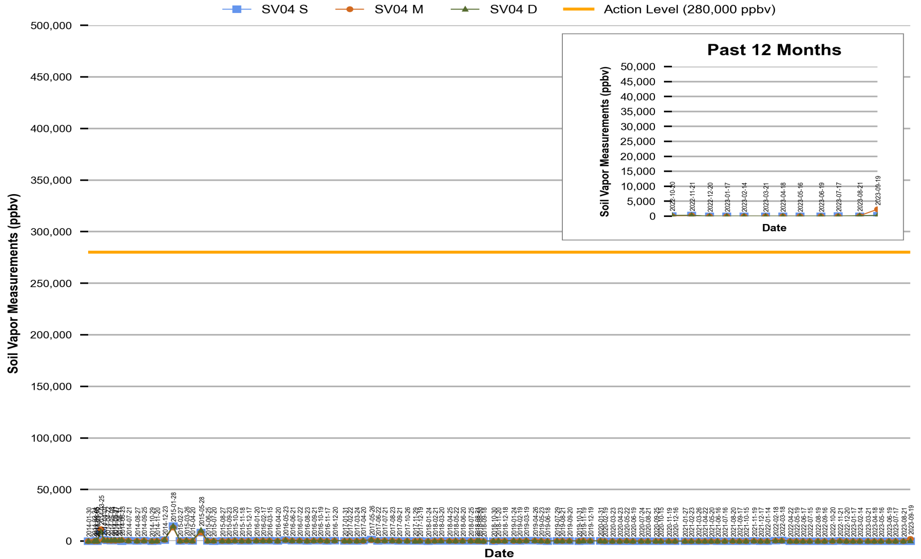
Figure 3 Red Hill - Tank 04 (F-24) Soil Vapor Measurements (Jan 2014 Through Sep 2023)
