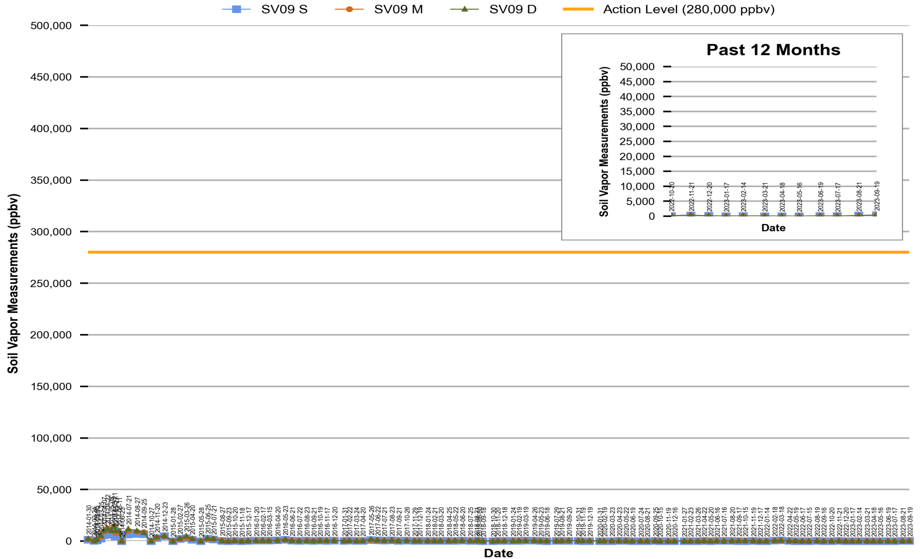
Figure 8 Red Hill - Tank 09 (JP-5) Soil Vapor Measurements (Jan 2014 Through Sep 2023)
