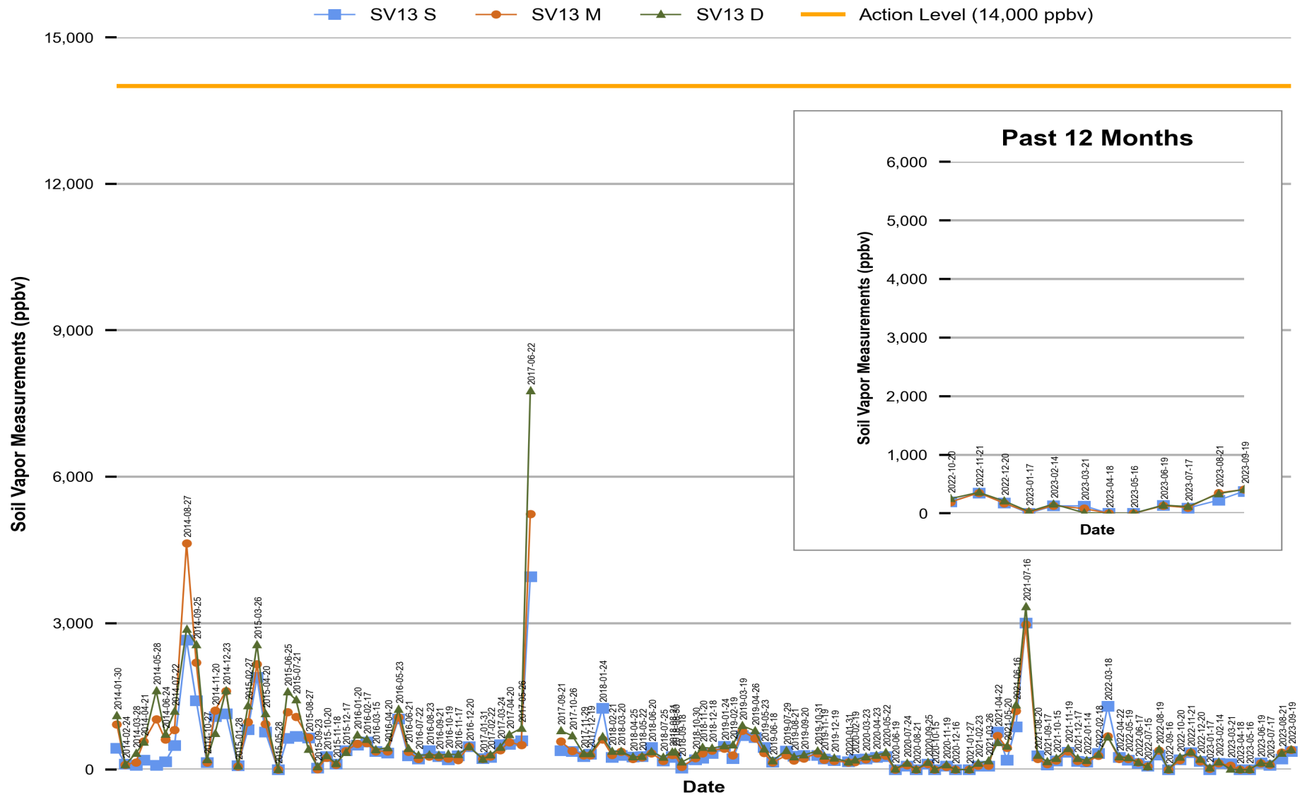
Figure 12 Red Hill - Tank 13 (F-76) Soil Vapor Measurements (Jan 2014 Through Sep 2023)
