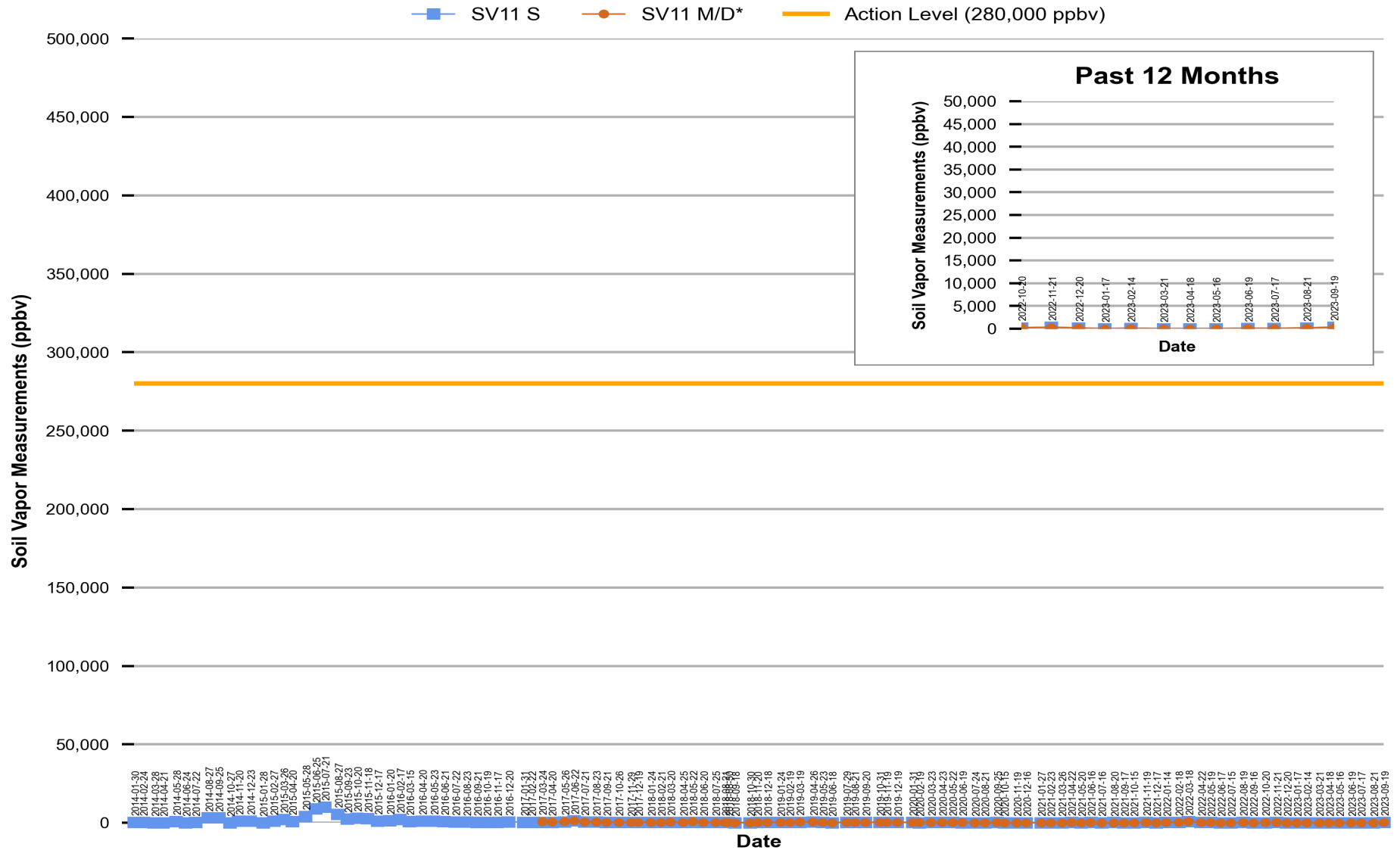
Figure 10 Red Hill - Tank 11 (JP-5) Soil Vapor Measurements (Jan 2014 Through Sep 2023)
