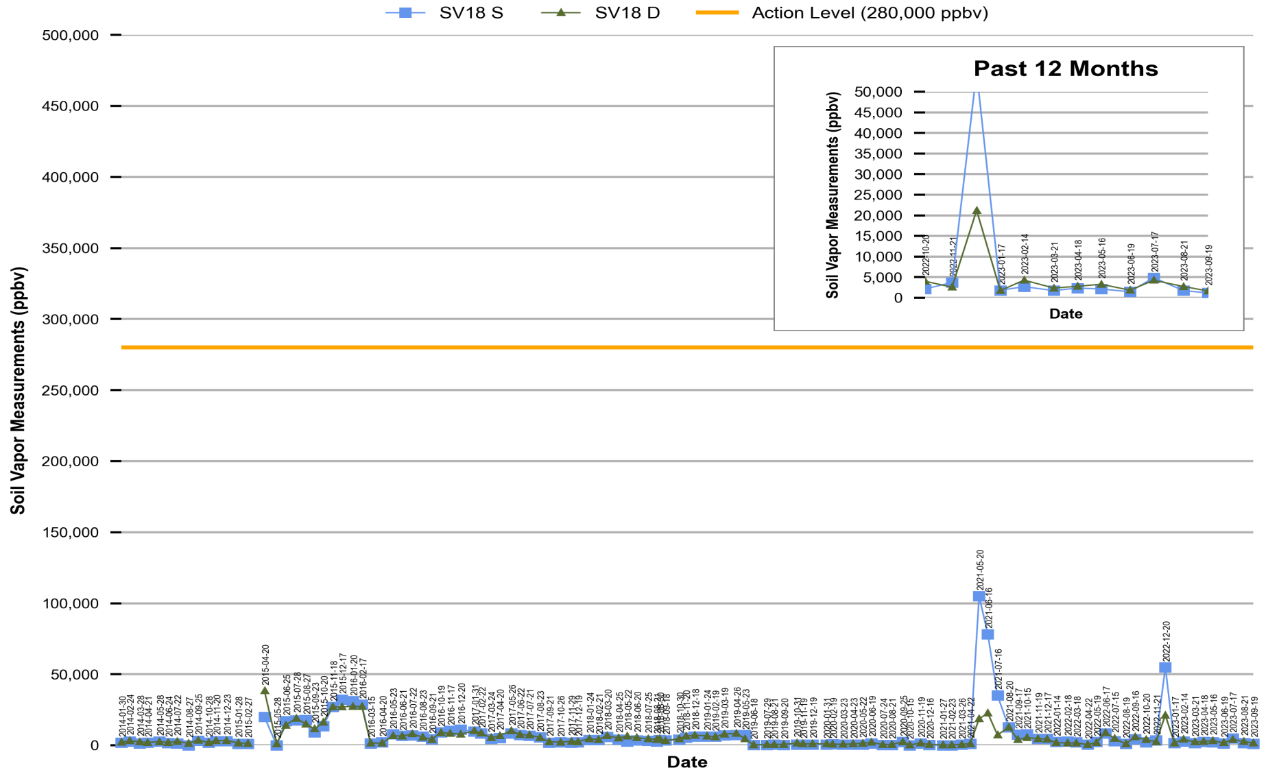
Figure 17 Red Hill - Tank 18 (JP-5) Soil Vapor Measurements (Jan 2014 Through Sep 2023)
