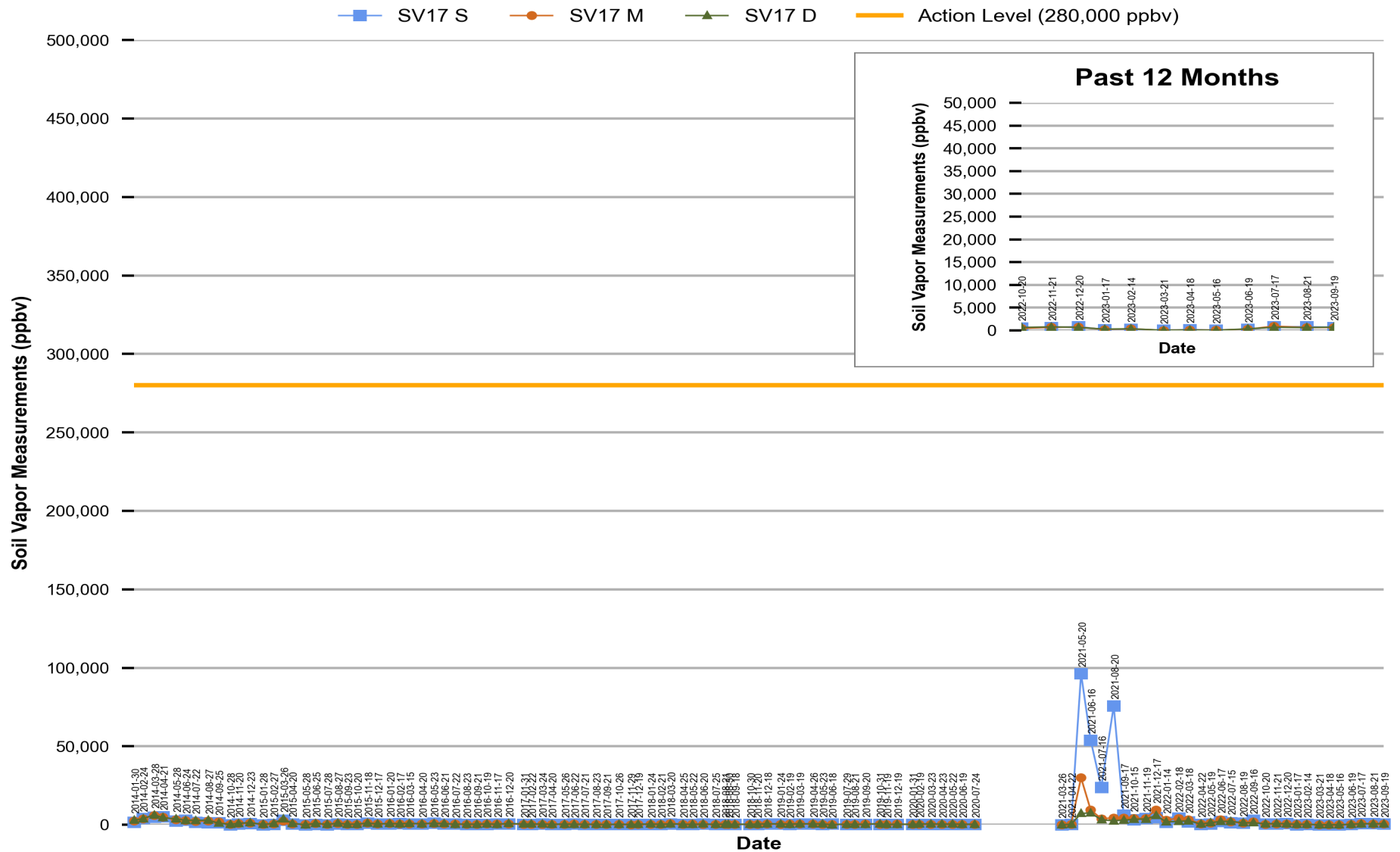
Figure 16 Red Hill - Tank 17 (JP-5) Soil Vapor Measurements (Jan 2014 Through Sep 2023)
