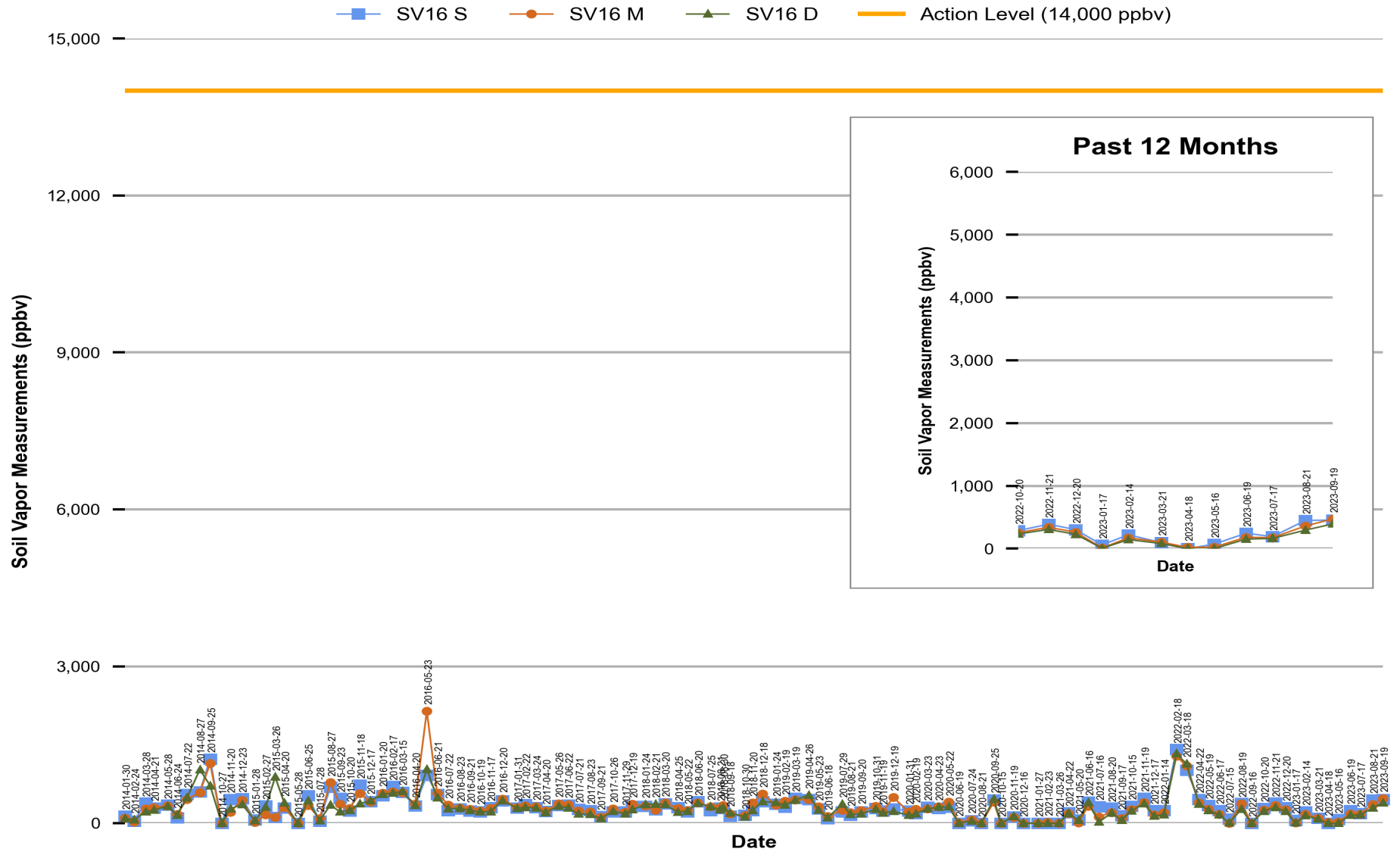
Figure 15 Red Hill - Tank 16 (F-76) Soil Vapor Measurements (Jan 2014 Through Sep 2023)
