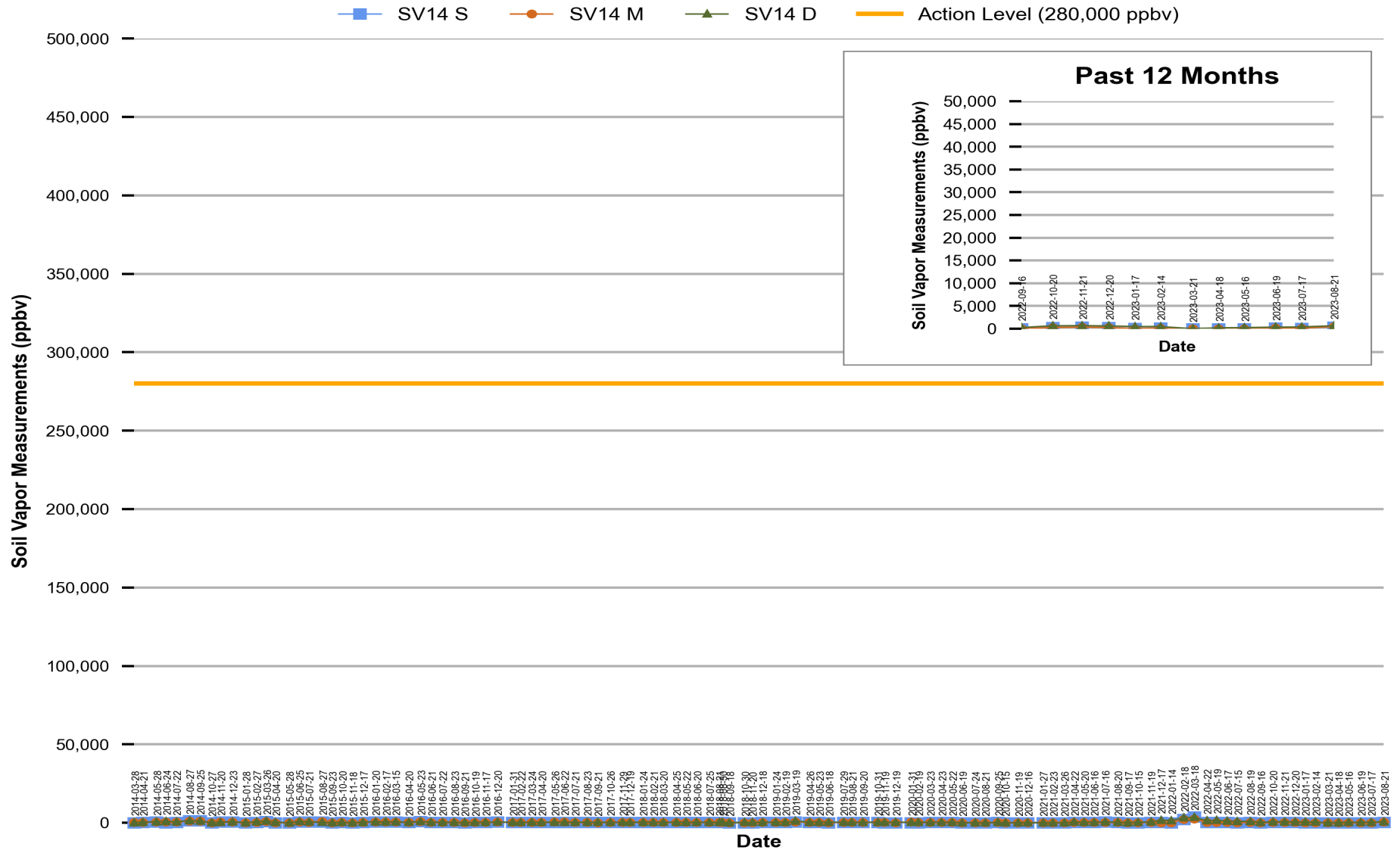
Figure 13 Red Hill - Tank 14 (JP-5) EMPTY Soil Vapor Measurements (Mar 2014 Through Aug 2023)
