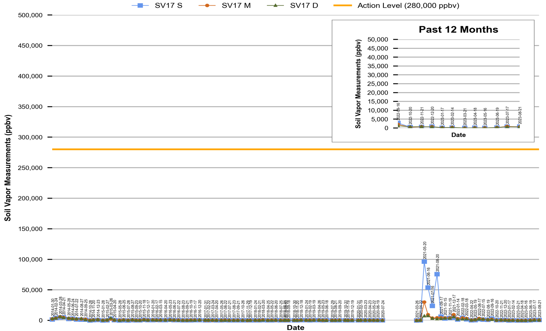
Figure 16 Red Hill - Tank 17 (JP-5) EMPTY Soil Vapor Measurements (Jan 2014 Through Aug 2023)
