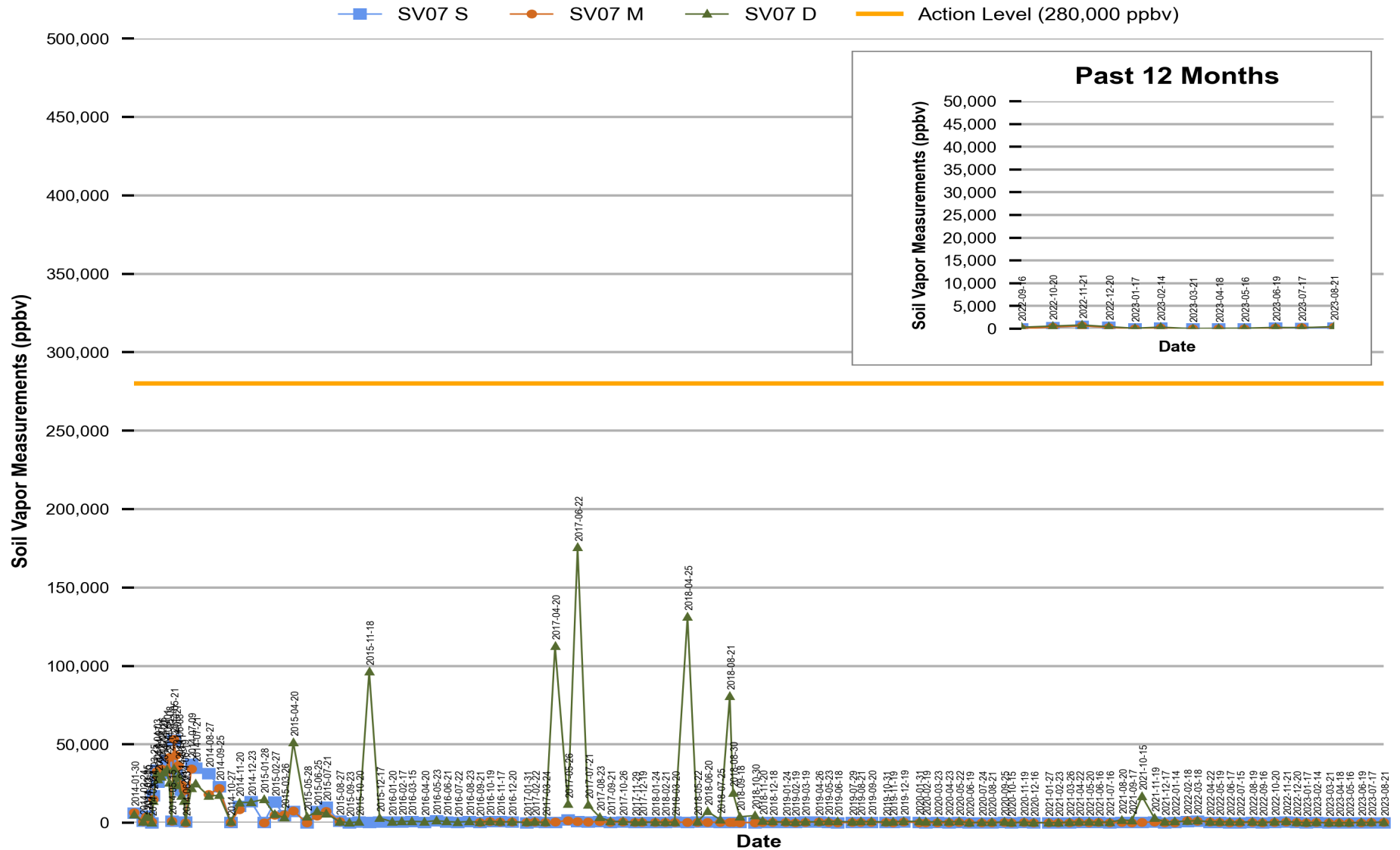
Figure 6 Red Hill - Tank 07 (JP-5) Soil Vapor Measurements (Jan 2014 Through Aug 2023)
