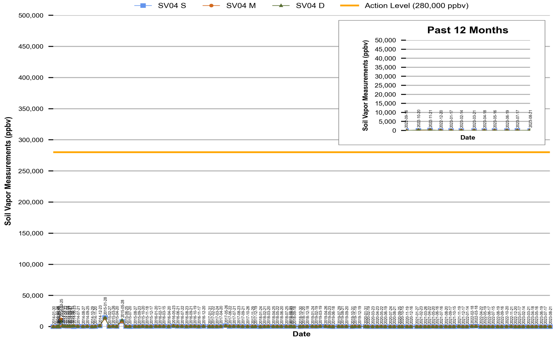
Figure 3 Red Hill - Tank 04 (F-24) Soil Vapor Measurements (Jan 2014 Through Aug 2023)
