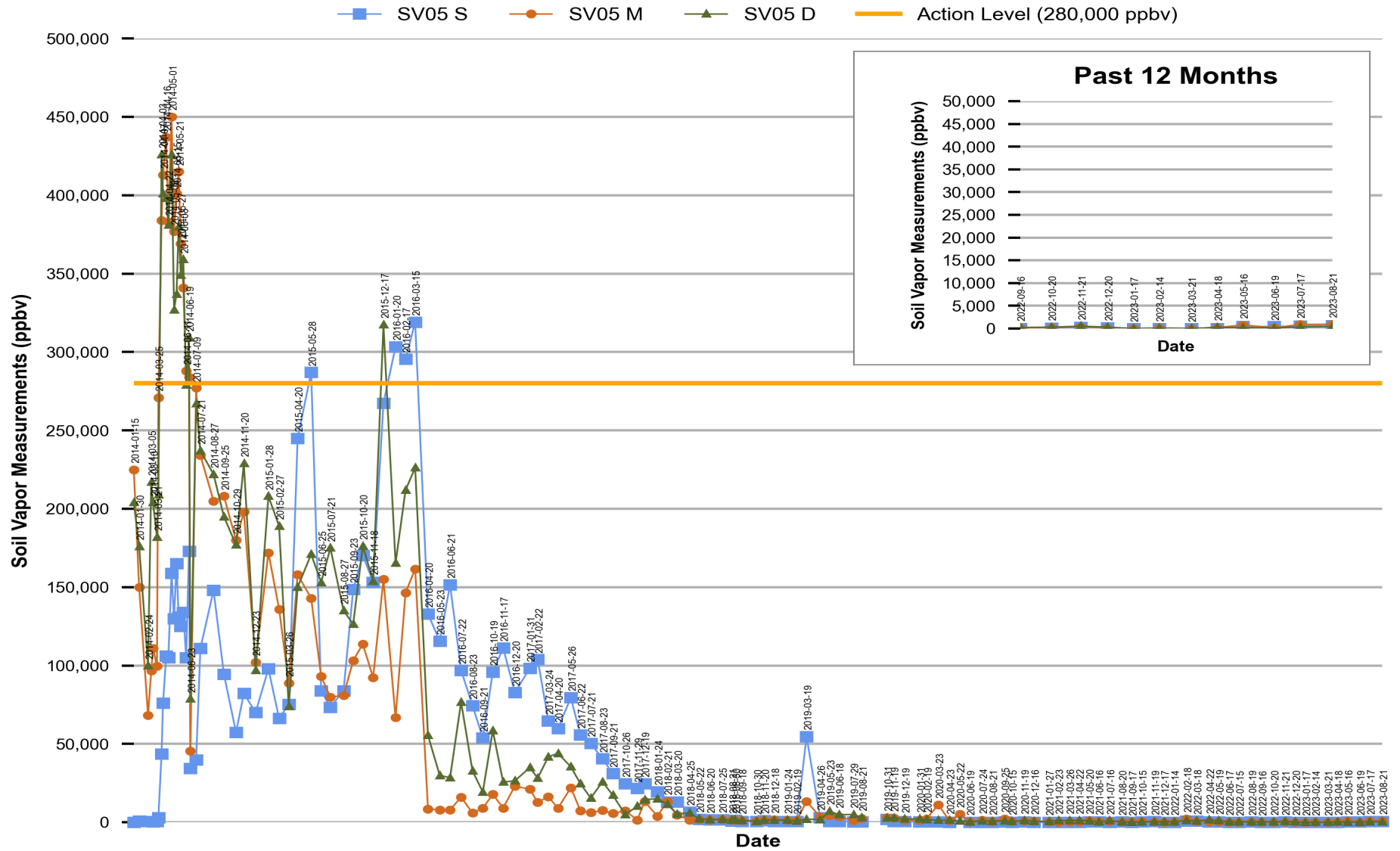
Figure 4 Red Hill - Tank 05 (F-24) Soil Vapor Measurements (Jan 2014 Through Aug 2023)
