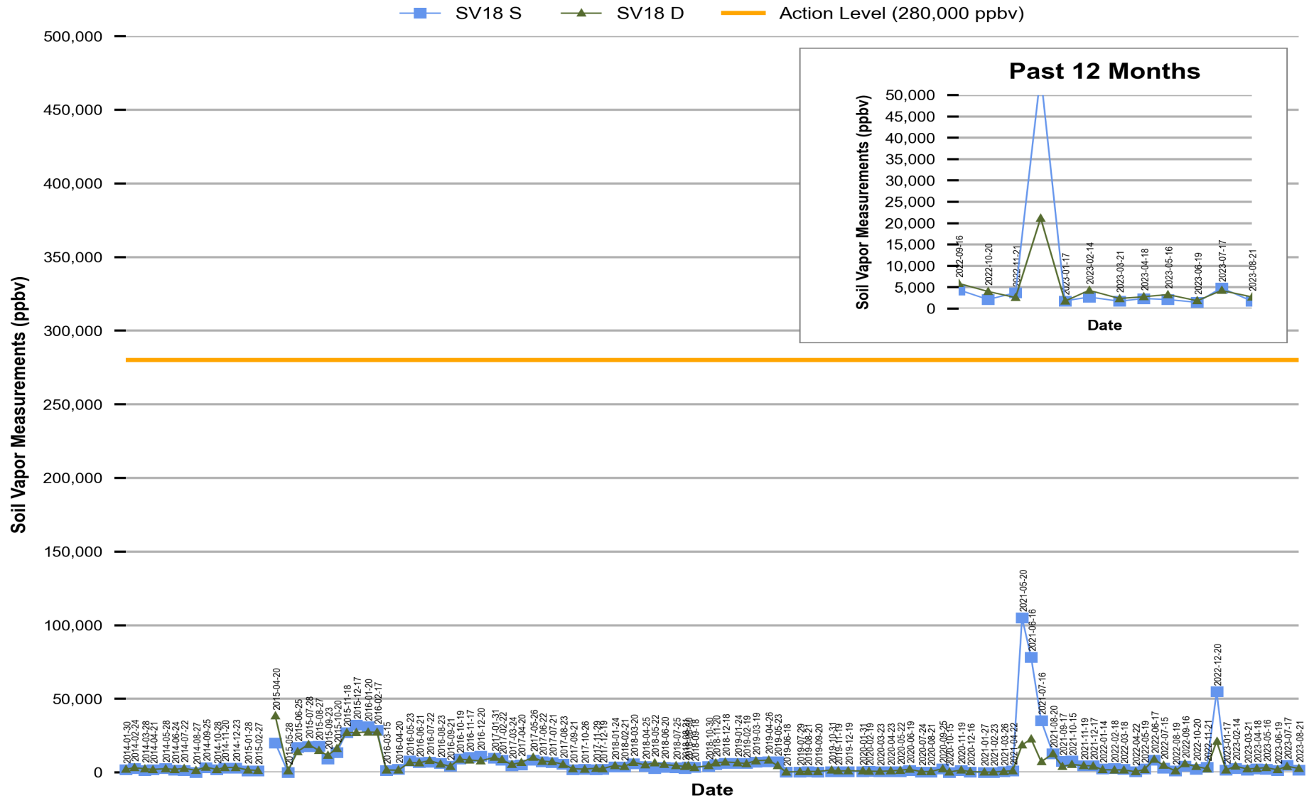
Figure 17 Red Hill - Tank 18 (JP-5) EMPTY Soil Vapor Measurements (Jan 2014 Through Aug 2023)
