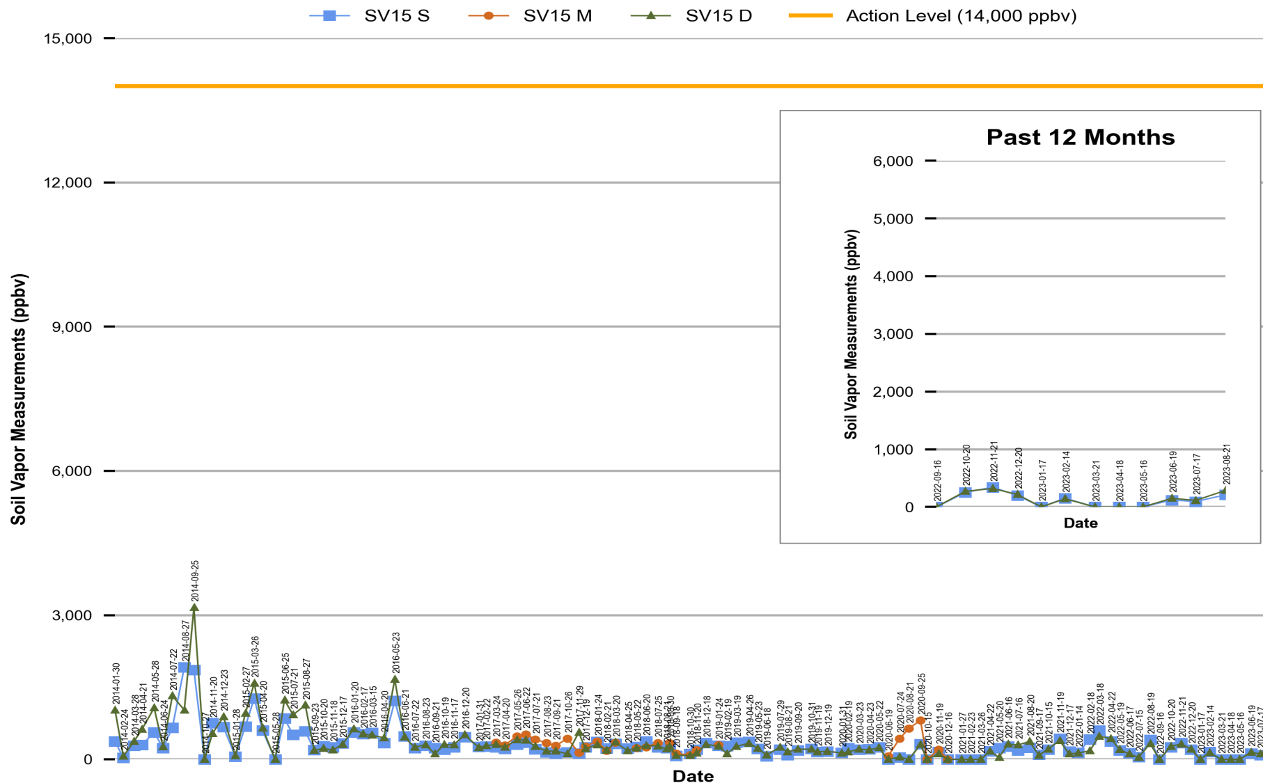
Figure 14 Red Hill - Tank 15 (F-76) Soil Vapor Measurements (Jan 2014 Through Aug 2023)
