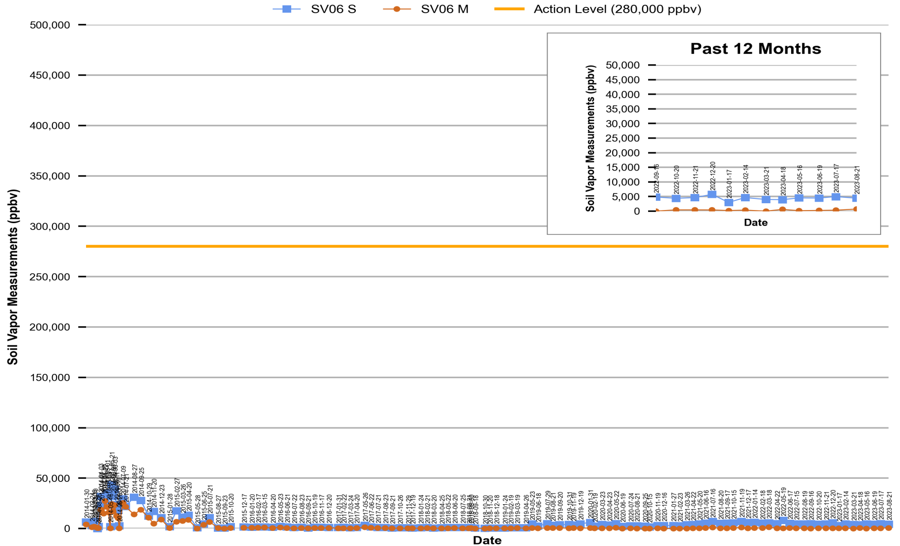
Figure 5 Red Hill - Tank 06 (F-24) Soil Vapor Measurements (Jan 2014 Through Aug 2023)
