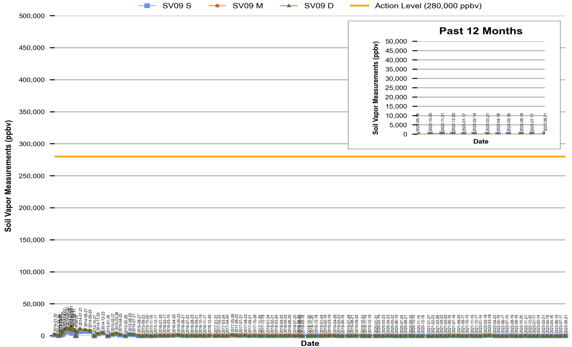
Figure 8 Red Hill - Tank 09 (JP-5) Soil Vapor Measurements (Jan 2014 Through Aug 2023)
