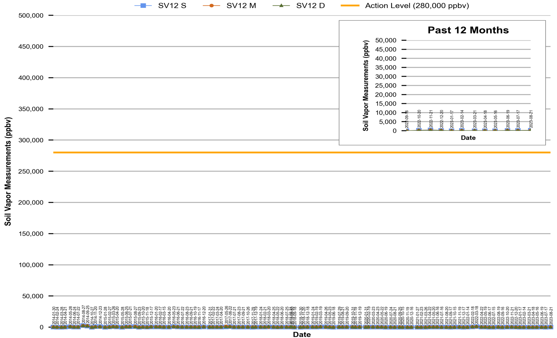
Figure 11 Red Hill - Tank 12 (JP-5) Soil Vapor Measurements (Jan 2014 Through Aug 2023)
