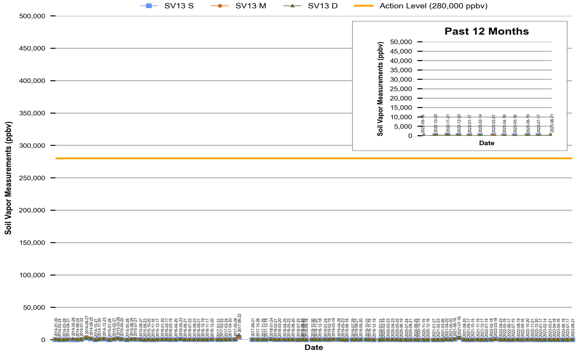
Figure 12 Red Hill - Tank 13 (JP-5) EMPTY Soil Vapor Measurements (Jan 2014 Through Aug 2023)
