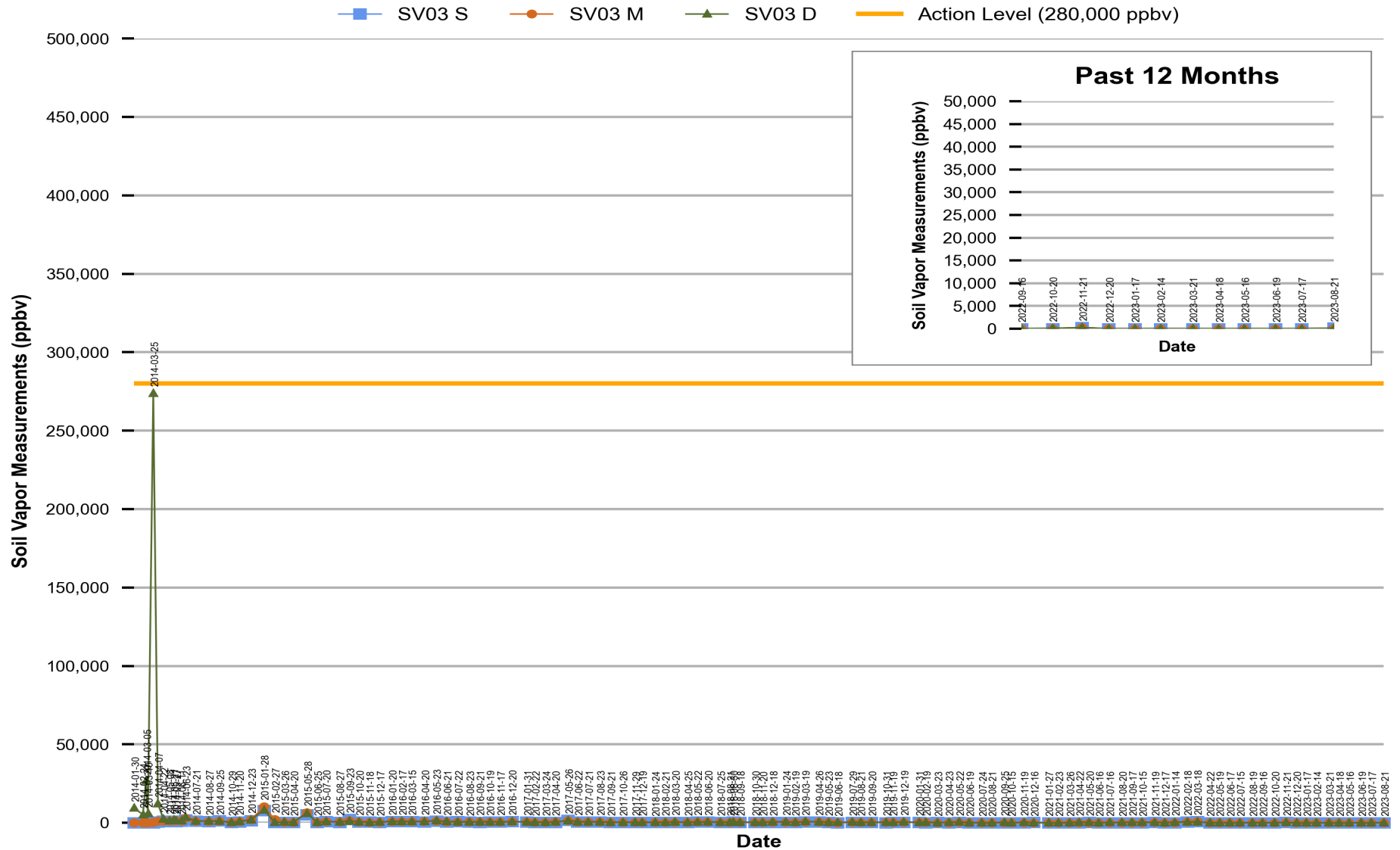
Figure 2 Red Hill - Tank 03 (F-24) Soil Vapor Measurements (Jan 2014 Through Aug 2023)
