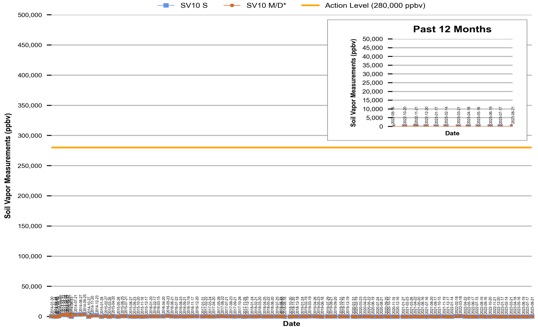
Figure 9 Red Hill - Tank 10 (JP-5) Soil Vapor Measurements (Jan 2014 Through Aug 2023)
