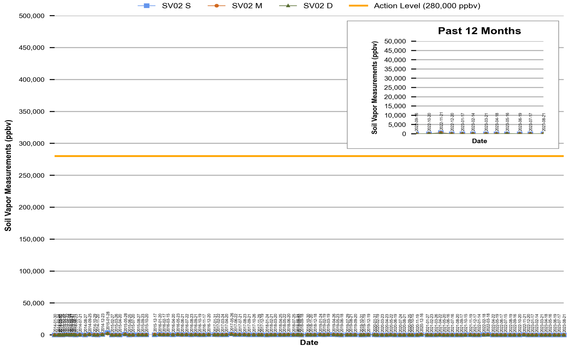
Figure 1 Red Hill - Tank 02 (F-24) Soil Vapor Measurements (Jan 2014 Through Aug 2023)
