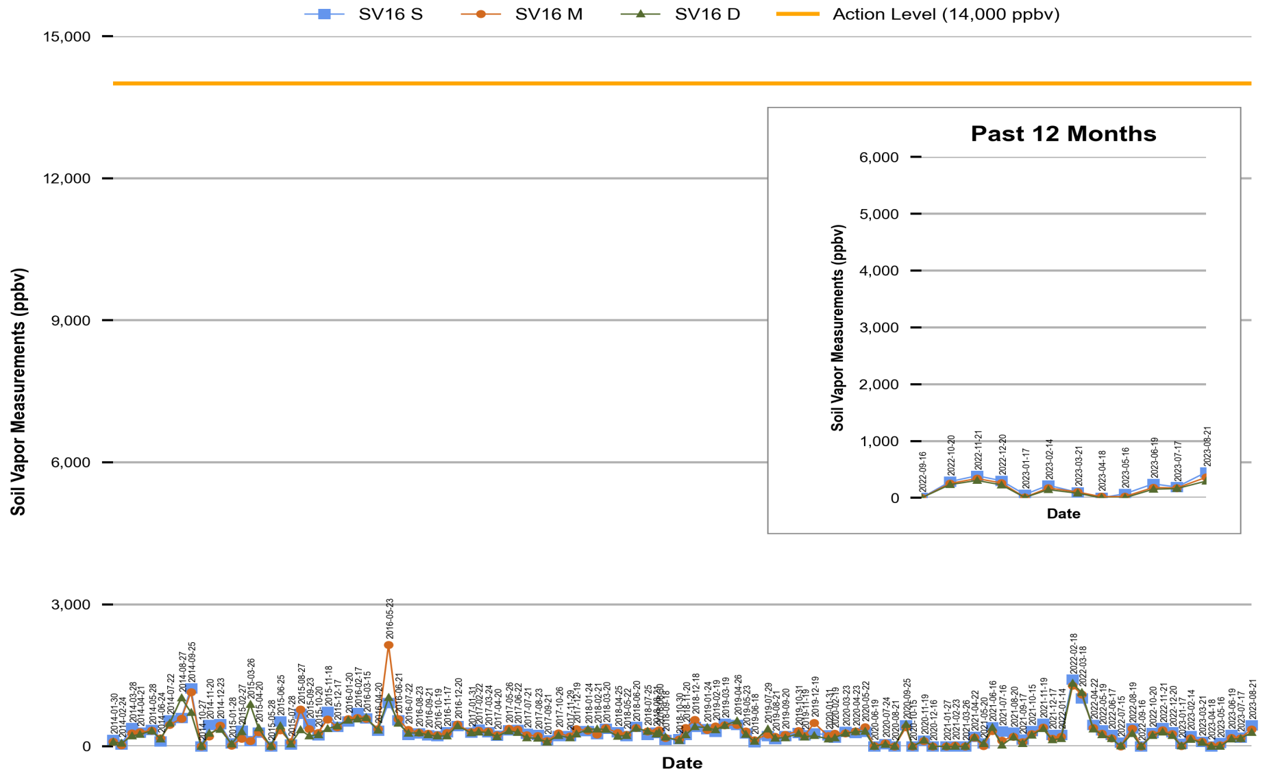
Figure 15 Red Hill - Tank 16 (F-76) Soil Vapor Measurements (Jan 2014 Through Aug 2023)
