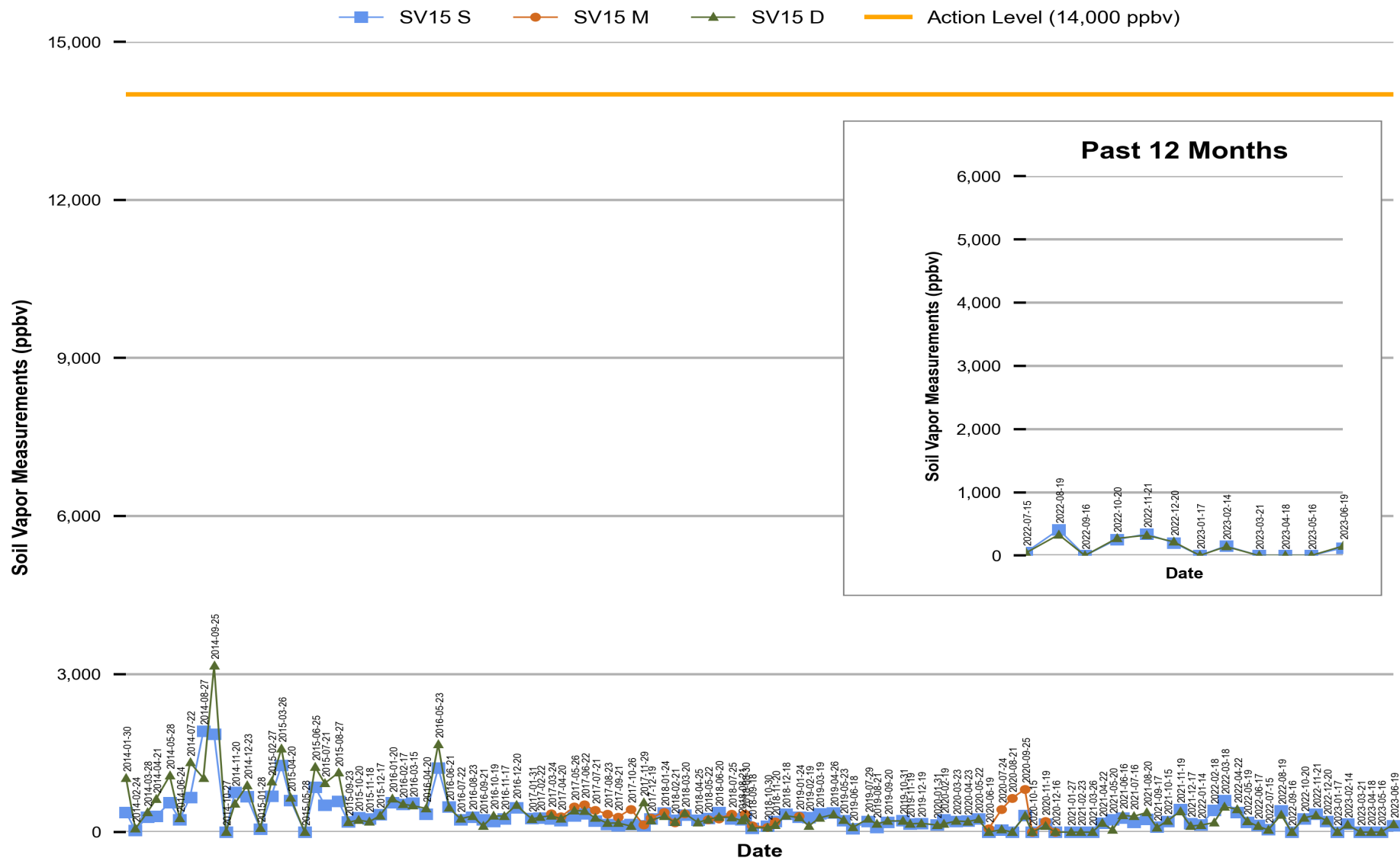
Figure 14 Red Hill - Tank 15 (F-76) Soil Vapor Measurements (Jan 2014 Through Jun 2023)
