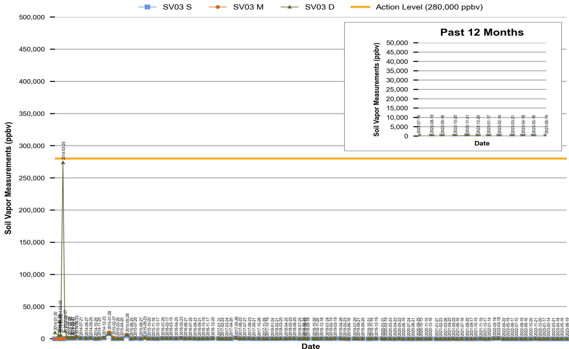
Figure 2 Red Hill - Tank 03 (F-24) Soil Vapor Measurements (Jan 2014 Through Jun 2023)
