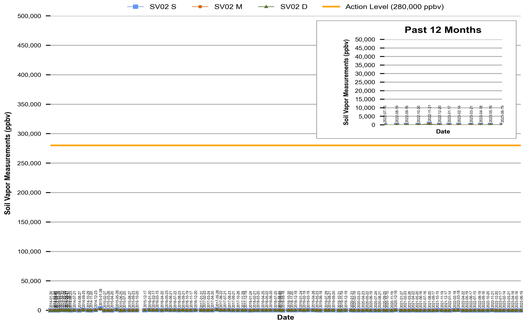
Figure 1 Red Hill - Tank 02 (F-24) Soil Vapor Measurements (Jan 2014 Through Jun 2023)
