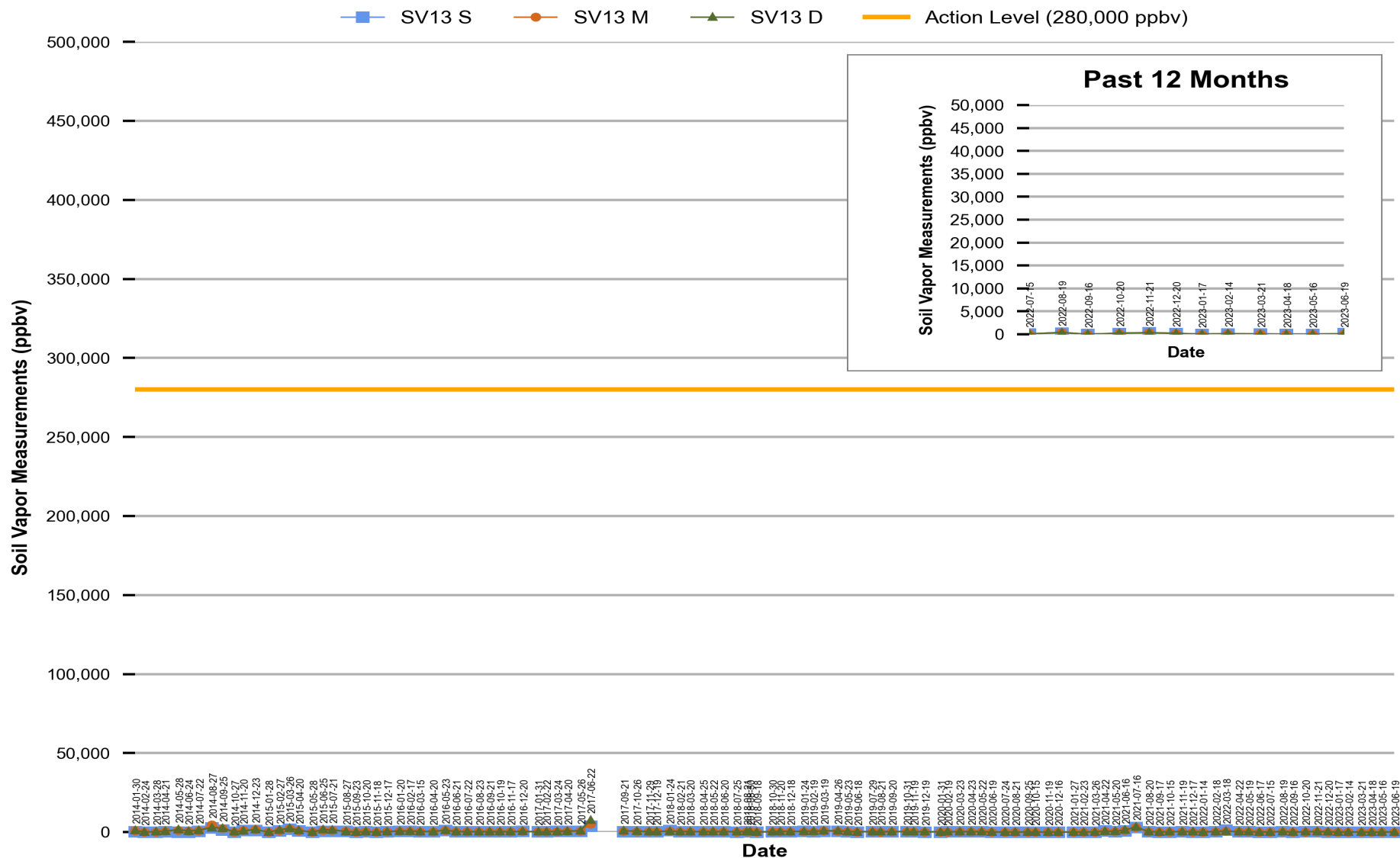
Figure 12 Red Hill - Tank 13 (JP-5) Soil Vapor Measurements (Jan 2014 Through Jun 2023)
