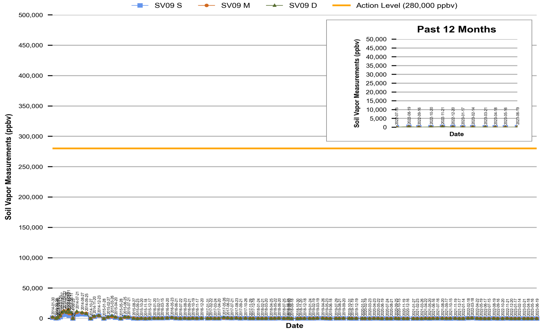
Figure 8 Red Hill - Tank 09 (JP-5) Soil Vapor Measurements (Jan 2014 Through Jun 2023)
