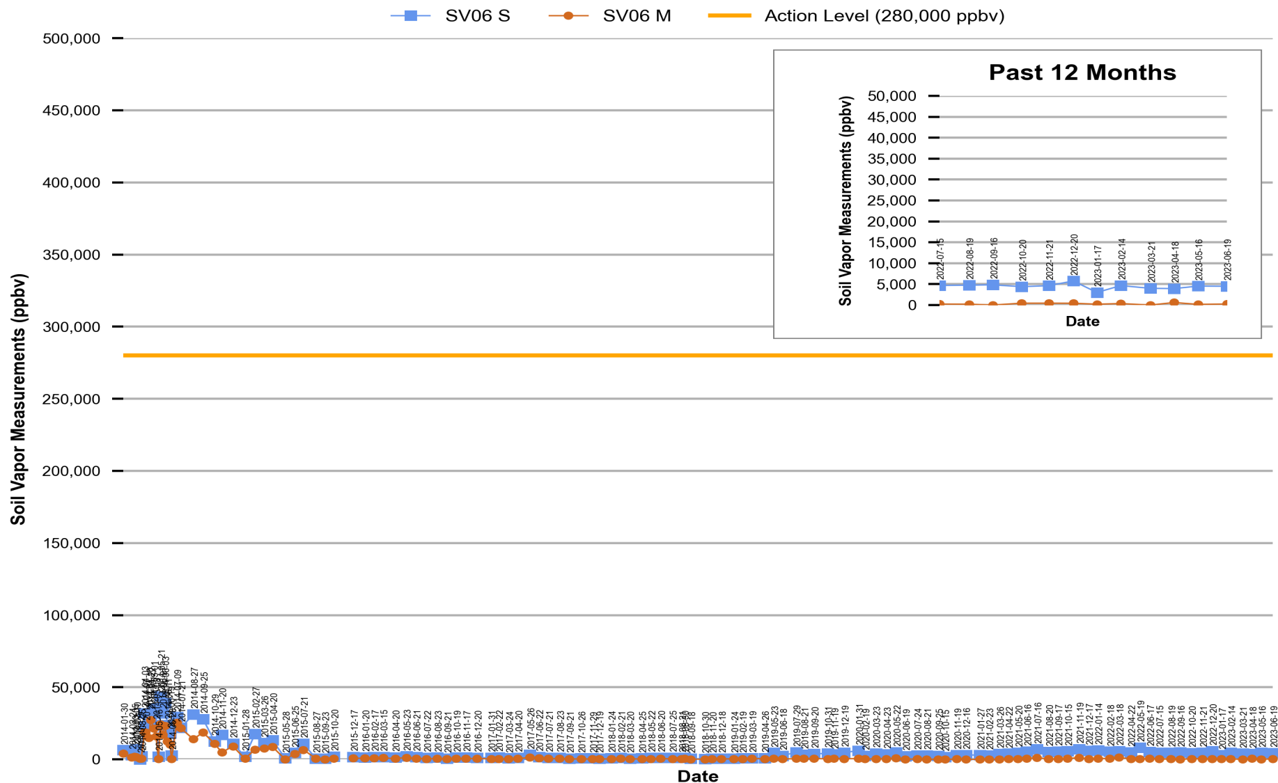
Figure 5 Red Hill - Tank 06 (F-24) Soil Vapor Measurements (Jan 2014 Through Jun 2023)
