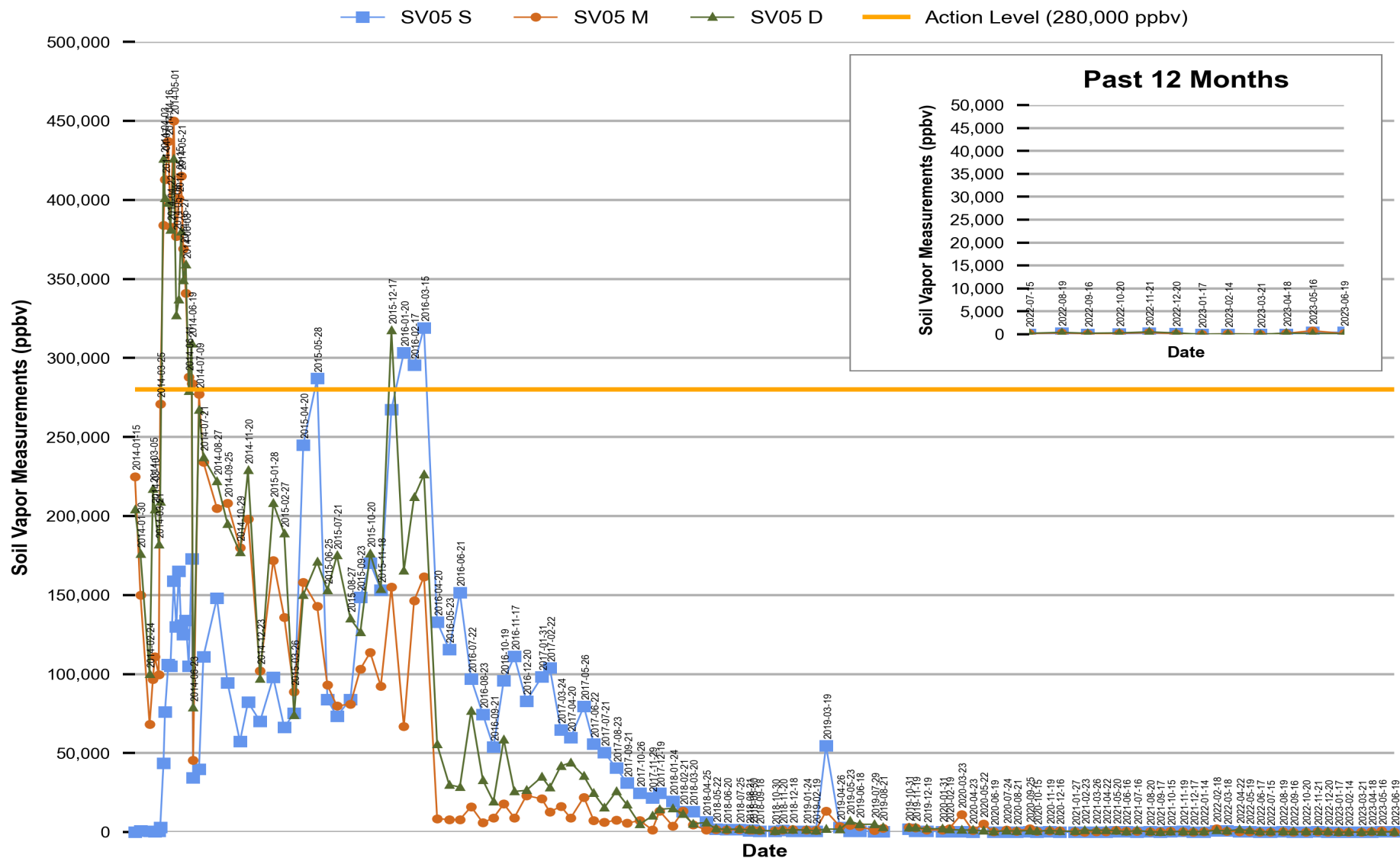
Figure 4 Red Hill - Tank 05 (F-24) Soil Vapor Measurements (Jan 2014 Through Jun 2023)
