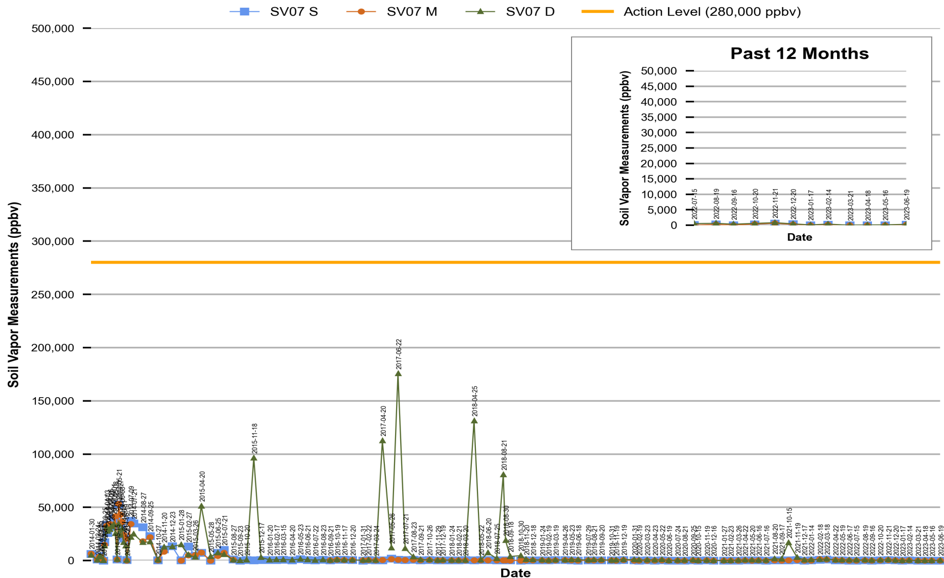
Figure 6 Red Hill - Tank 07 (JP-5) Soil Vapor Measurements (Jan 2014 Through Jun 2023)
