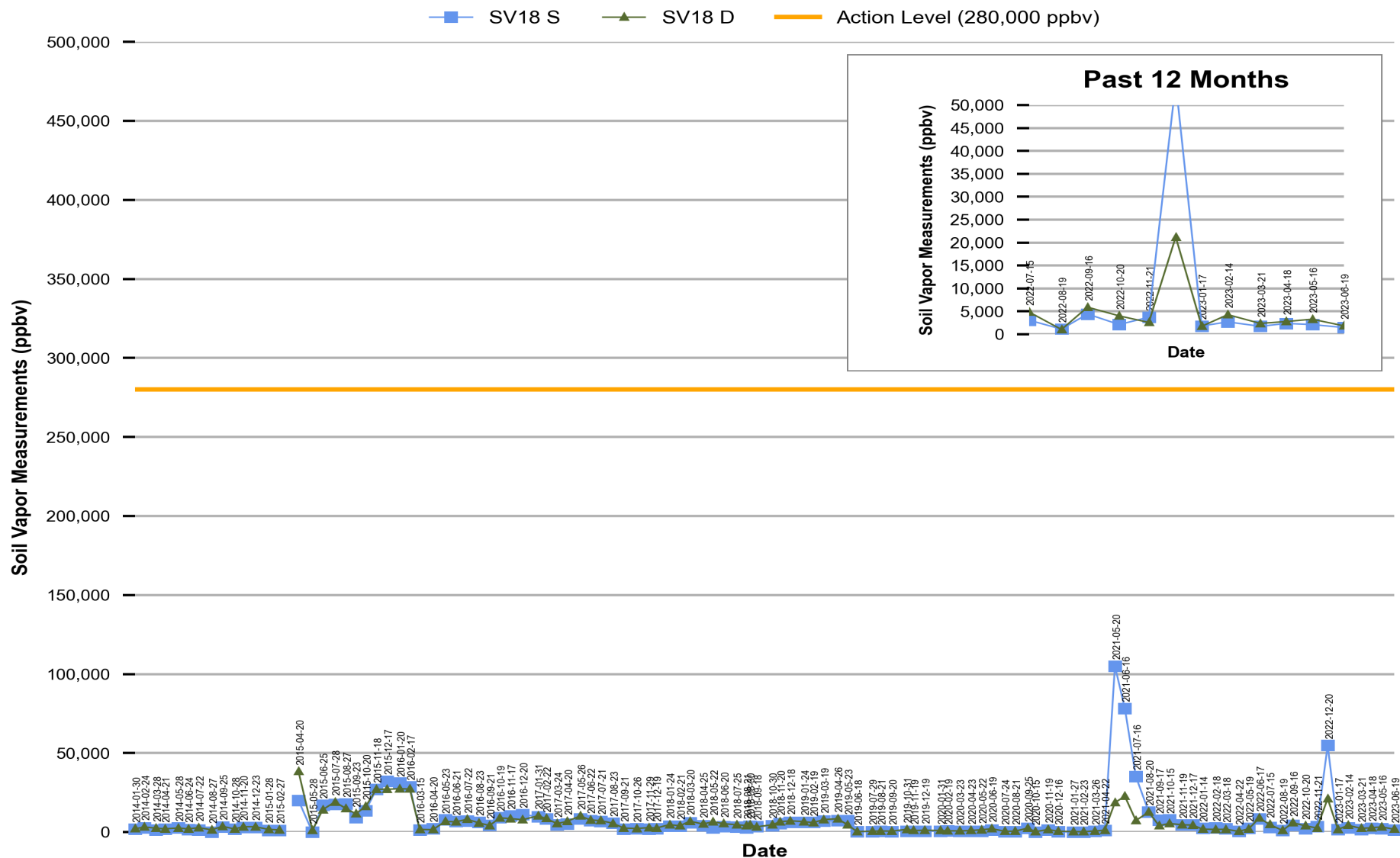
Figure 17 Red Hill - Tank 18 (JP-5) EMPTY Soil Vapor Measurements (Jan 2014 Through Jun 2023)
