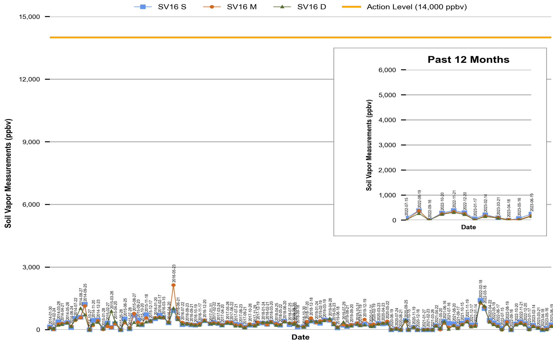
Figure 15 Red Hill - Tank 16 (F-76) Soil Vapor Measurements (Jan 2014 Through Jun 2023)
