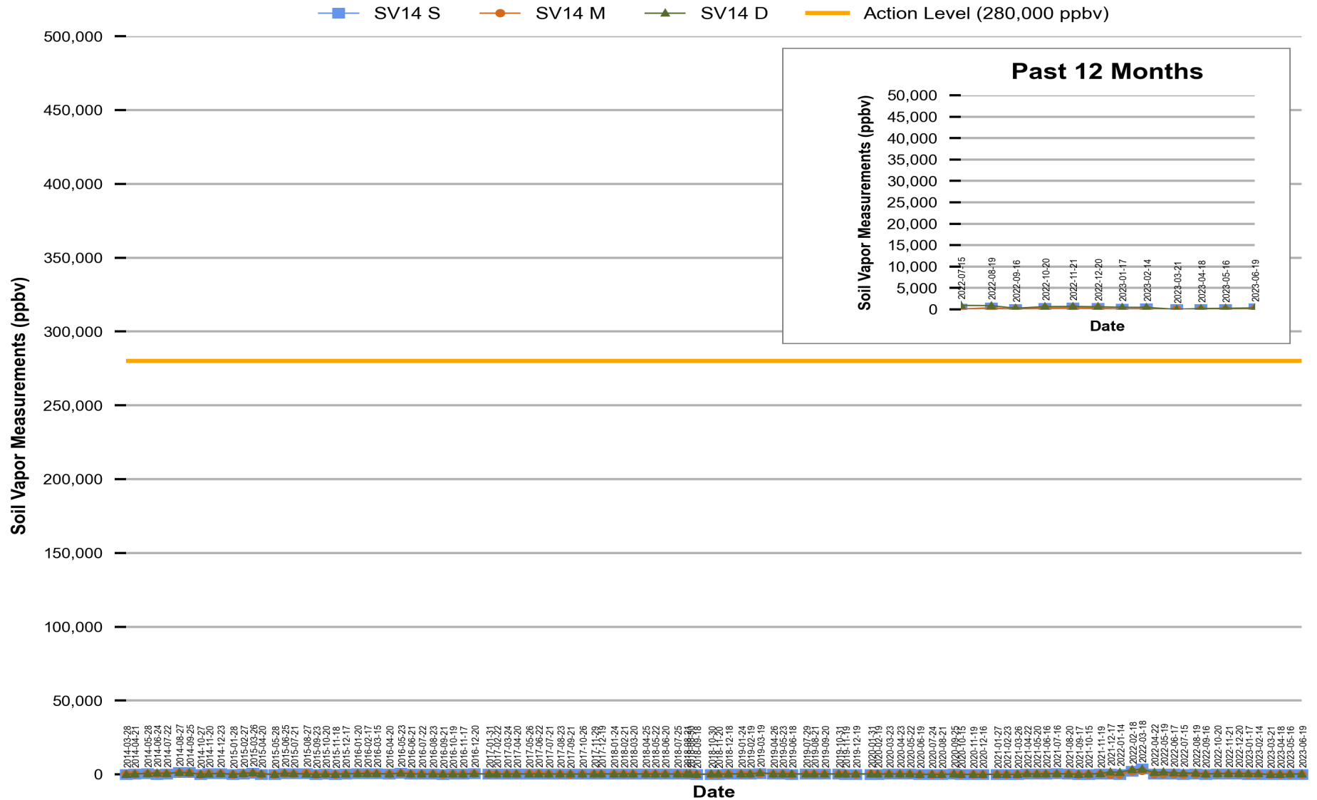
Figure 13 Red Hill - Tank 14 (JP-5) EMPTY Soil Vapor Measurements (Mar 2014 Through Jun 2023)
