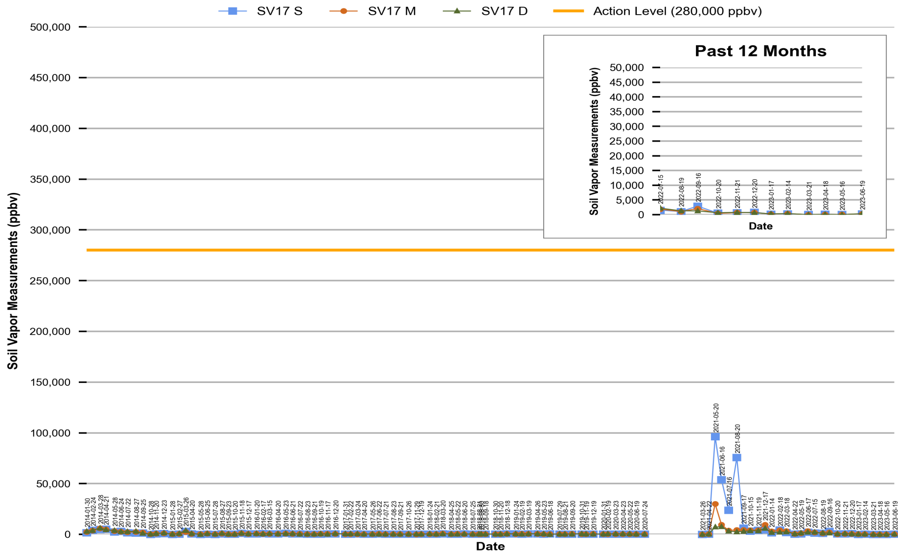
Figure 16 Red Hill - Tank 17 (JP-5) EMPTY Soil Vapor Measurements (Jan 2014 Through Jun 2023)
