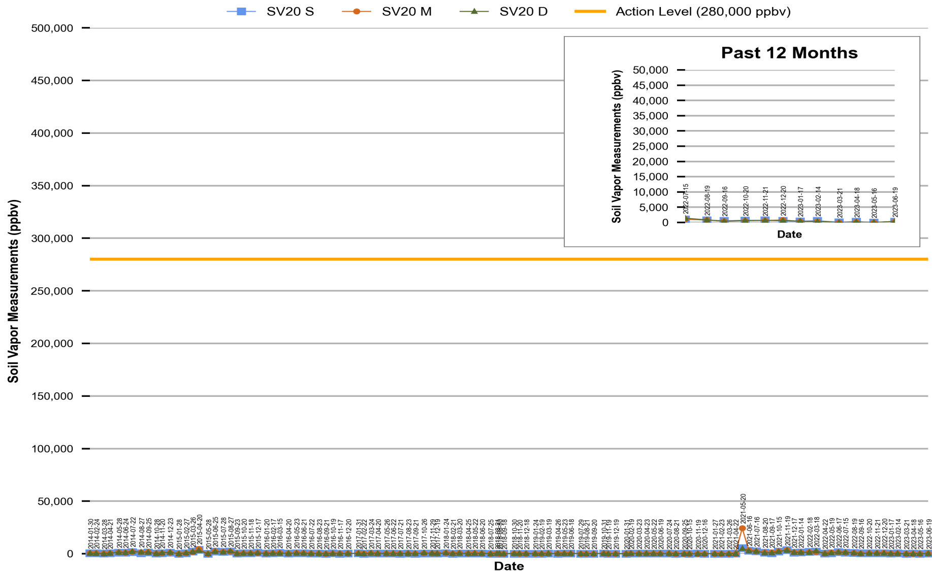
Figure 18 Red Hill - Tank 20 (JP-5) Soil Vapor Measurements (Jan 2014 Through Jun 2023)
