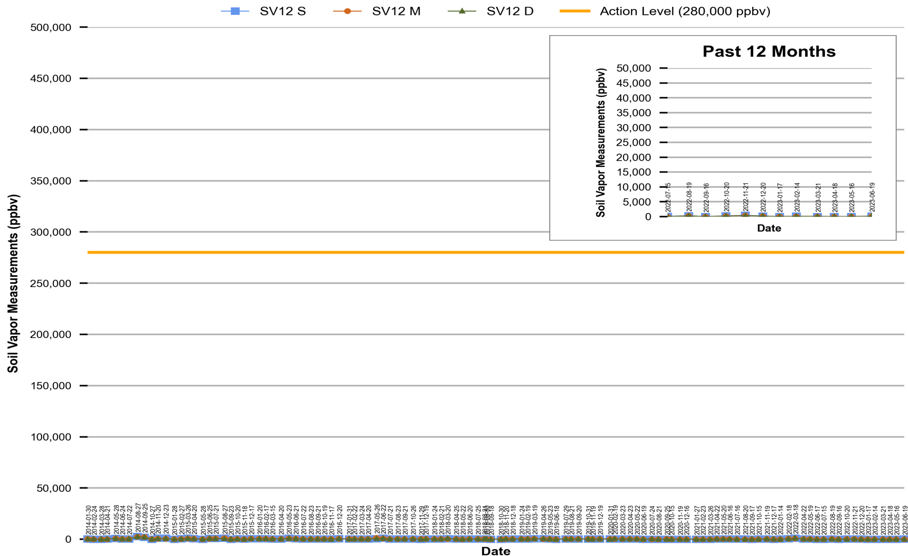
Figure 11 Red Hill - Tank 12 (JP-5) Soil Vapor Measurements (Jan 2014 Through Jun 2023)
