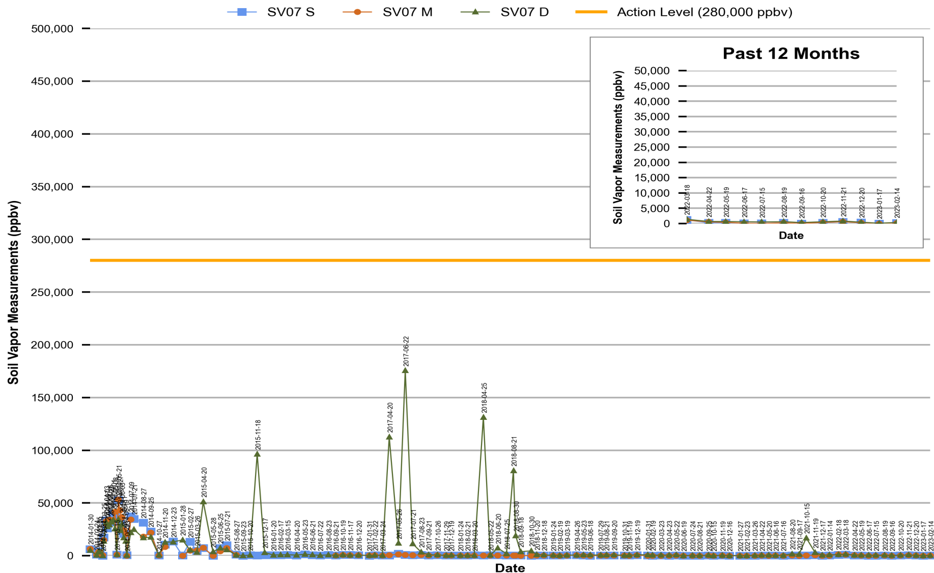
Figure 6 Red Hill - Tank 07 (JP-5) Soil Vapor Measurements (Jan 2014 Through Feb 2023)
