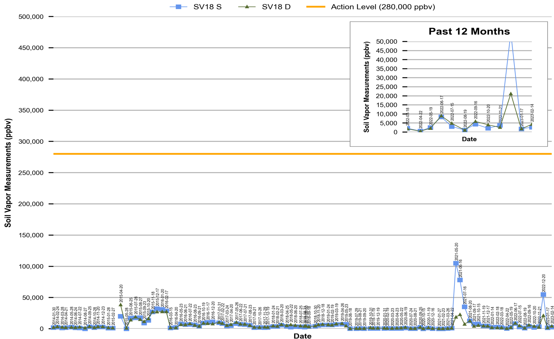
Figure 17 Red Hill - Tank 18 (JP-5) EMPTY Soil Vapor Measurements (Jan 2014 Through Feb 2023)
