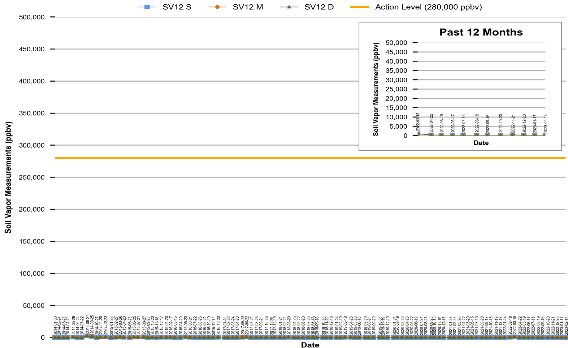
Figure 11 Red Hill - Tank 12 (JP-5) Soil Vapor Measurements (Jan 2014 Through Feb 2023)
