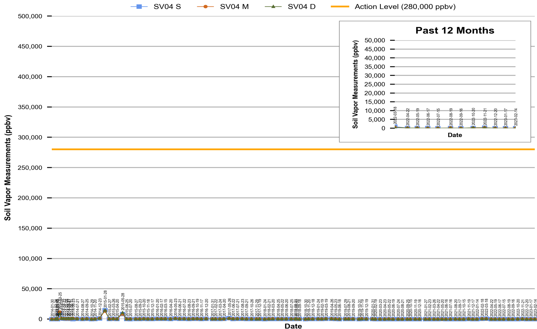
Figure 3 Red Hill - Tank 04 (F-24) Soil Vapor Measurements (Jan 2014 Through Feb 2023)
