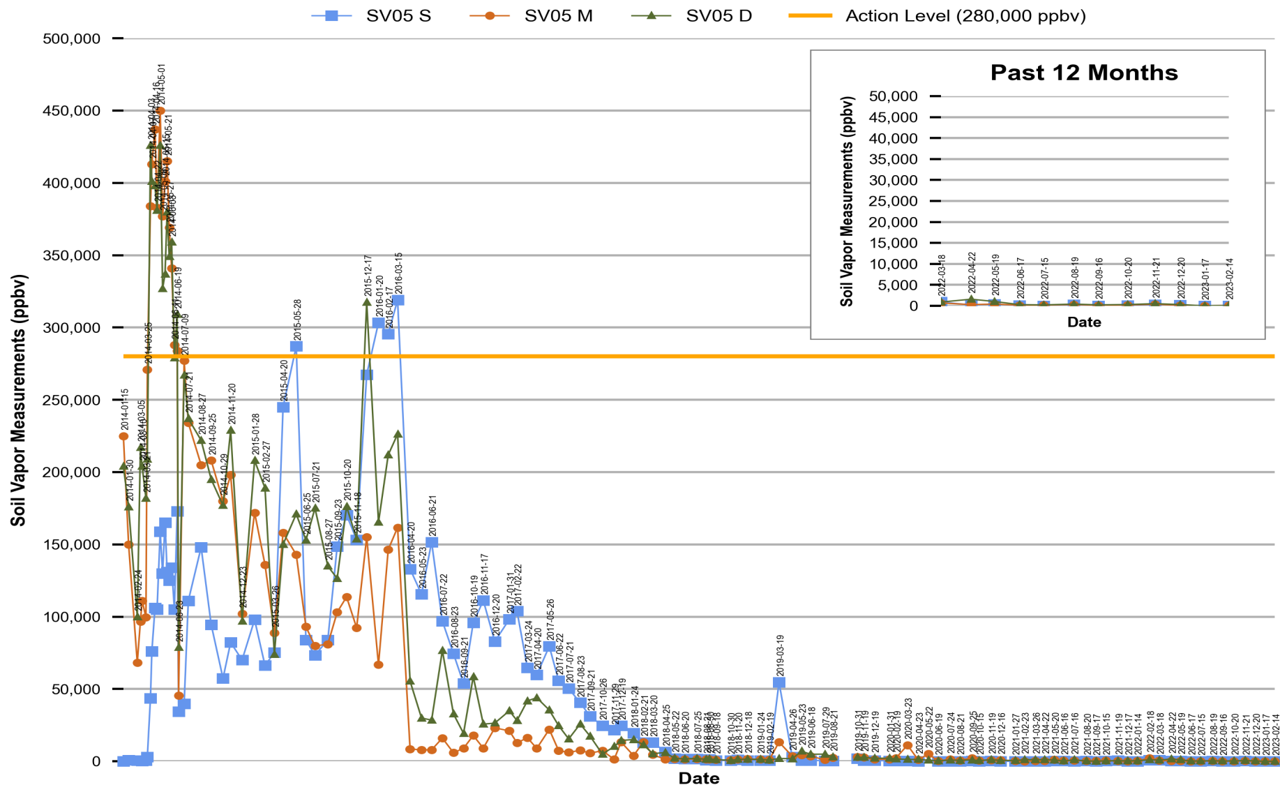
Figure 4 Red Hill - Tank 05 (F-24) Soil Vapor Measurements (Jan 2014 Through Feb 2023)
