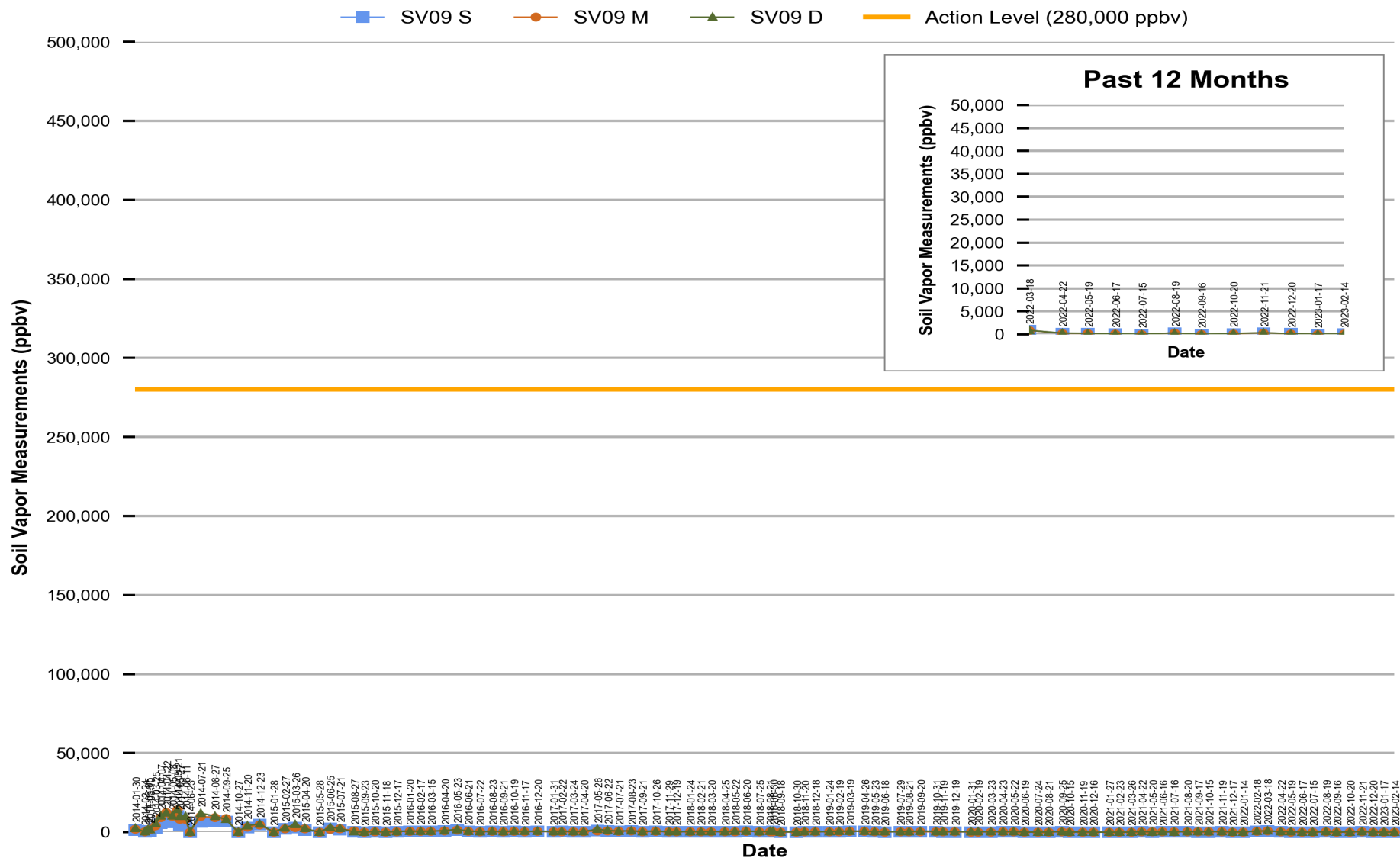
Figure 8 Red Hill - Tank 09 (JP-5) Soil Vapor Measurements (Jan 2014 Through Feb 2023)
