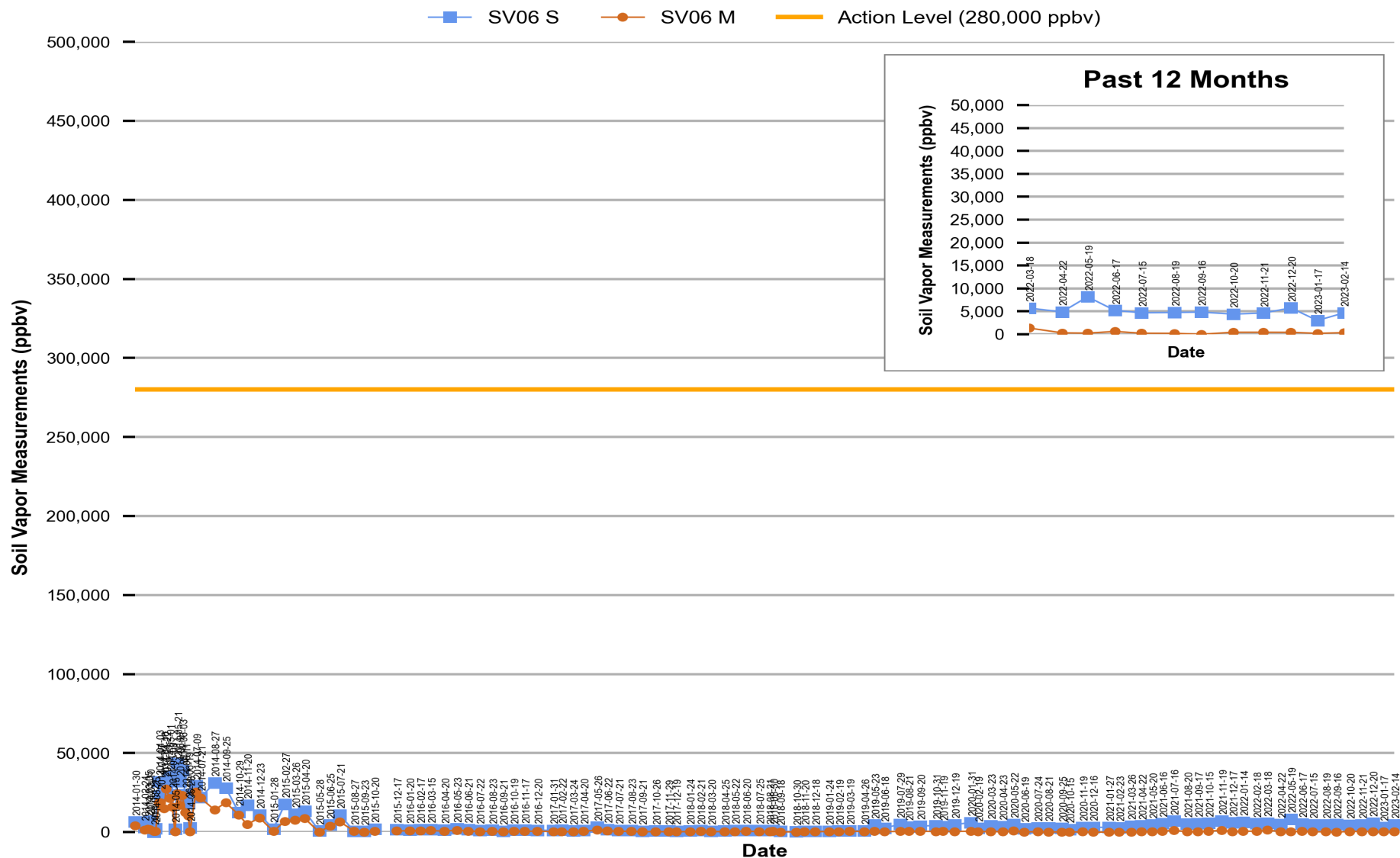
Figure 5 Red Hill - Tank 06 (F-24) Soil Vapor Measurements (Jan 2014 Through Feb 2023)
