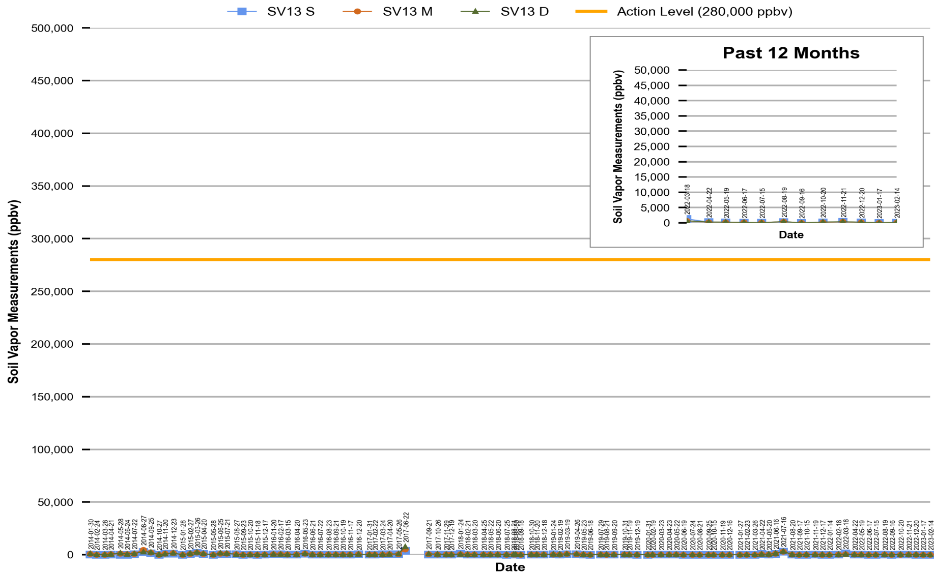
Figure 12 Red Hill - Tank 13 (JP-5) EMPTY Soil Vapor Measurements (Jan 2014 Through Feb 2023)
