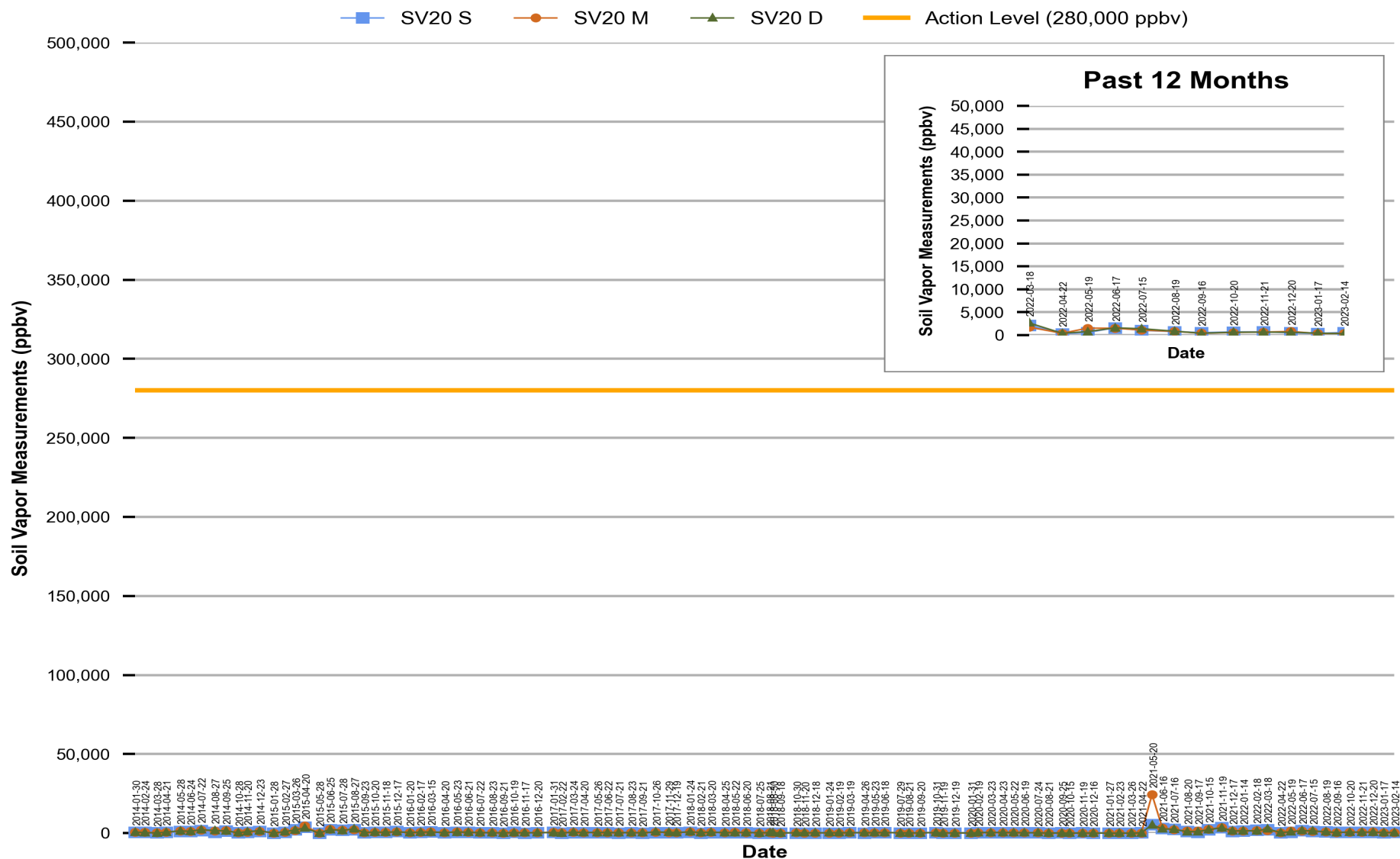
Figure 18 Red Hill - Tank 20 (JP-5) Soil Vapor Measurements (Jan 2014 Through Feb 2023)
