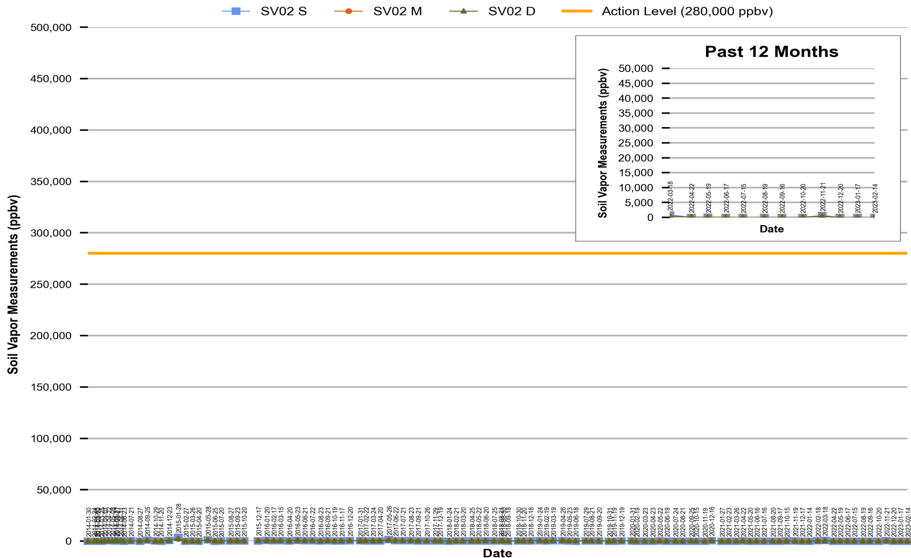
Figure 1 Red Hill - Tank 02 (F-24) Soil Vapor Measurements (Jan 2014 Through Feb 2023)
