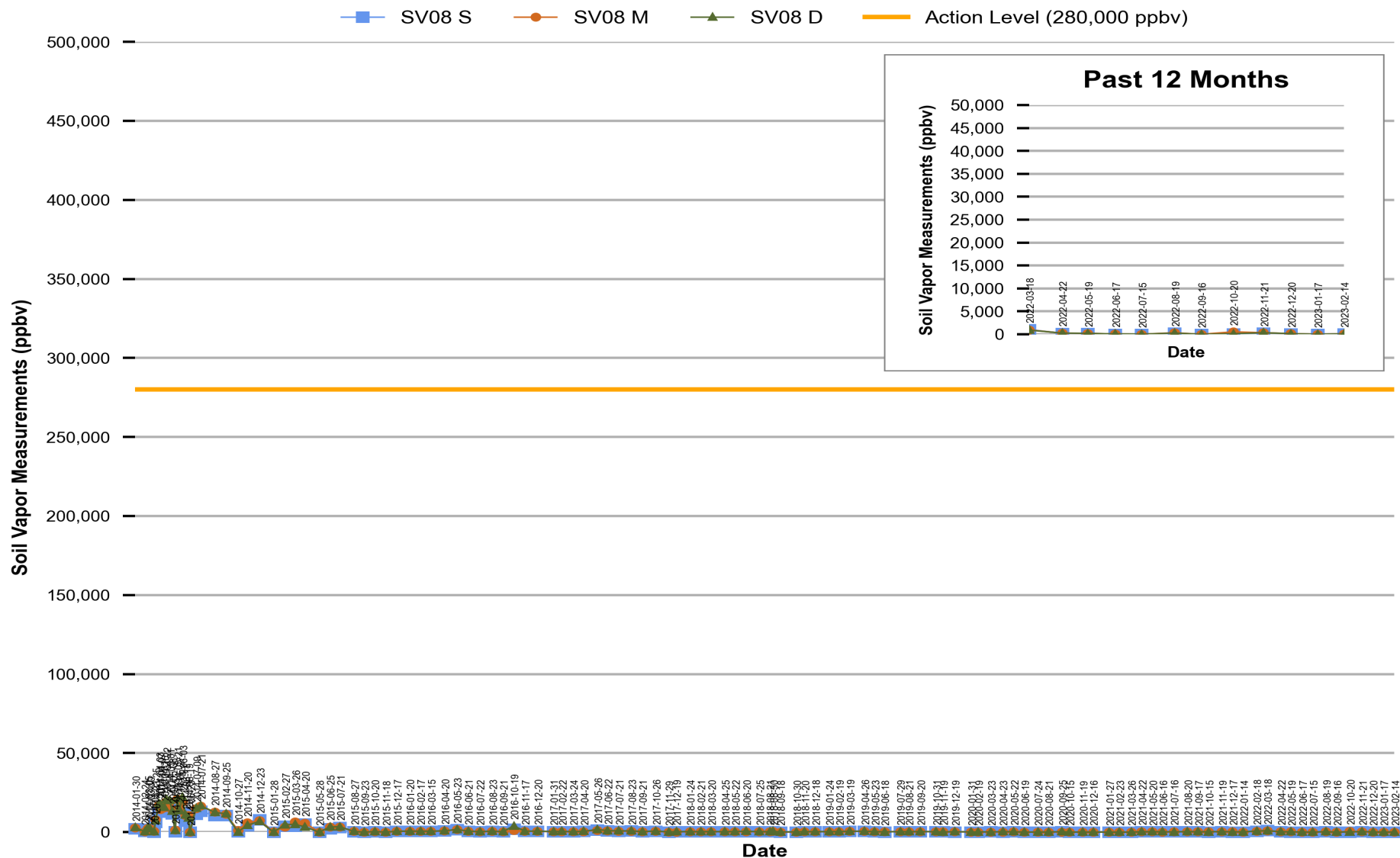
Figure 7 Red Hill - Tank 08 (JP-5) Soil Vapor Measurements (Jan 2014 Through Feb 2023)
