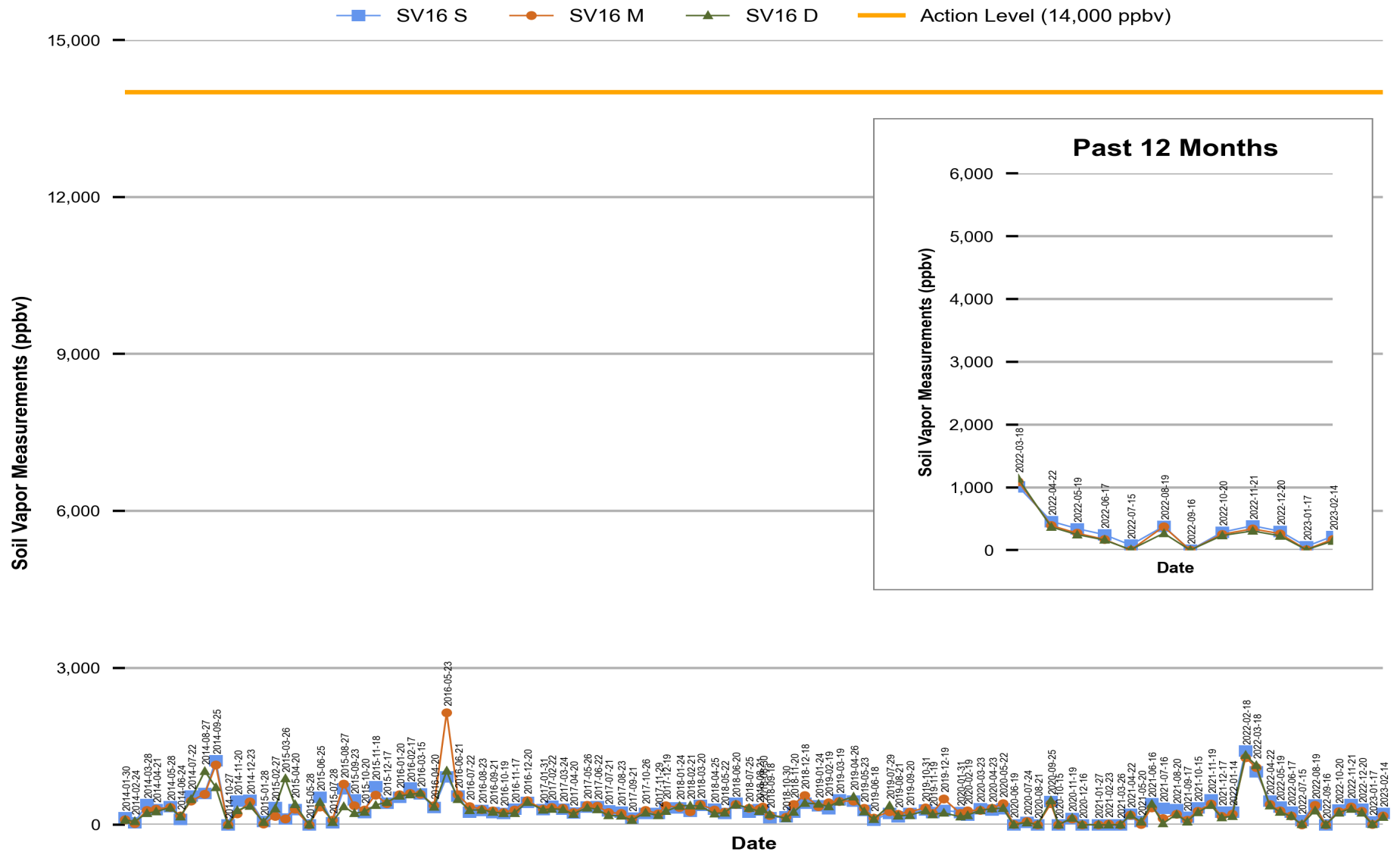
Figure 15 Red Hill - Tank 16 (F-76) Soil Vapor Measurements (Jan 2014 Through Feb 2023)
