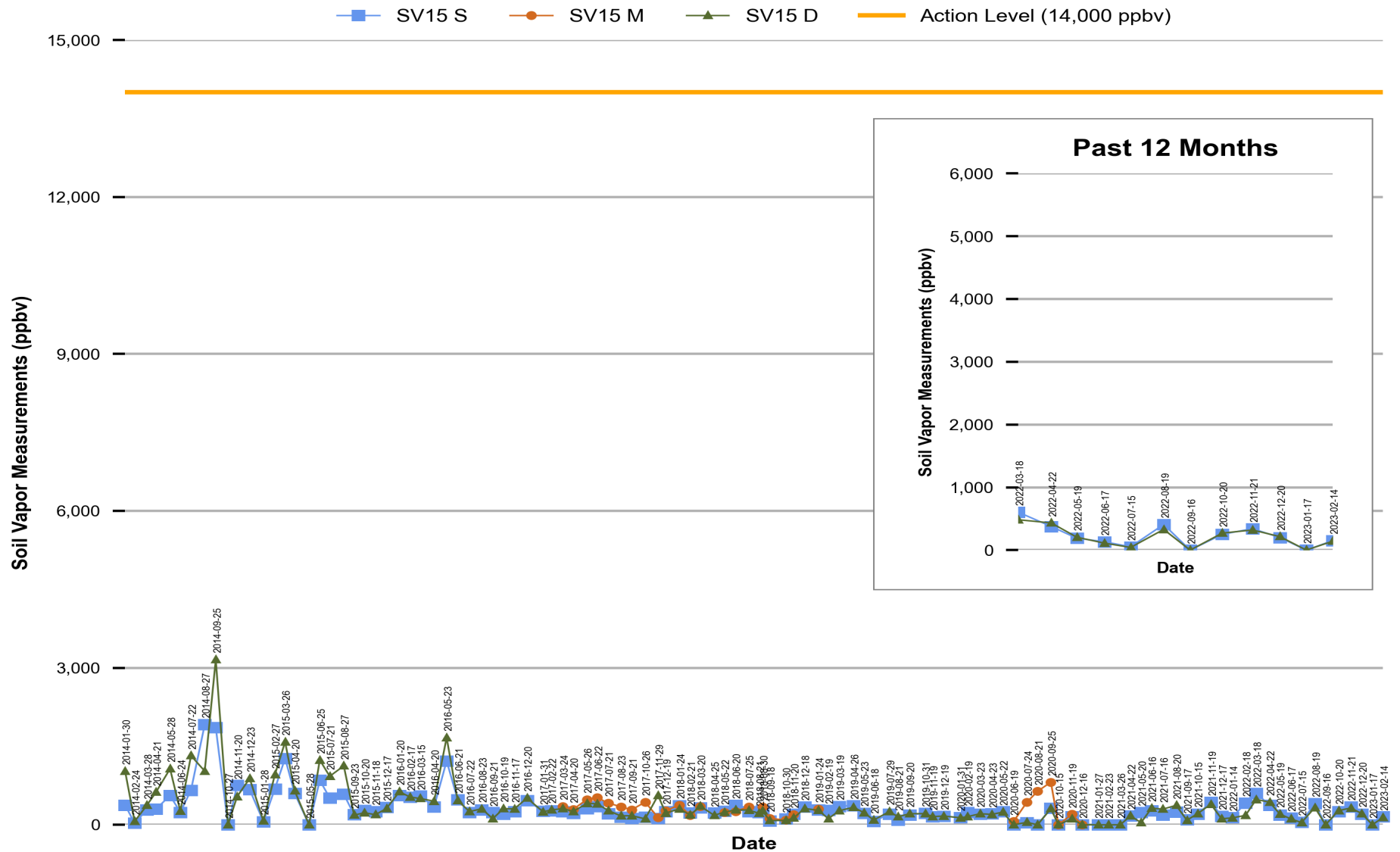
Figure 14 Red Hill - Tank 15 (F-76) Soil Vapor Measurements (Jan 2014 Through Feb 2023)
