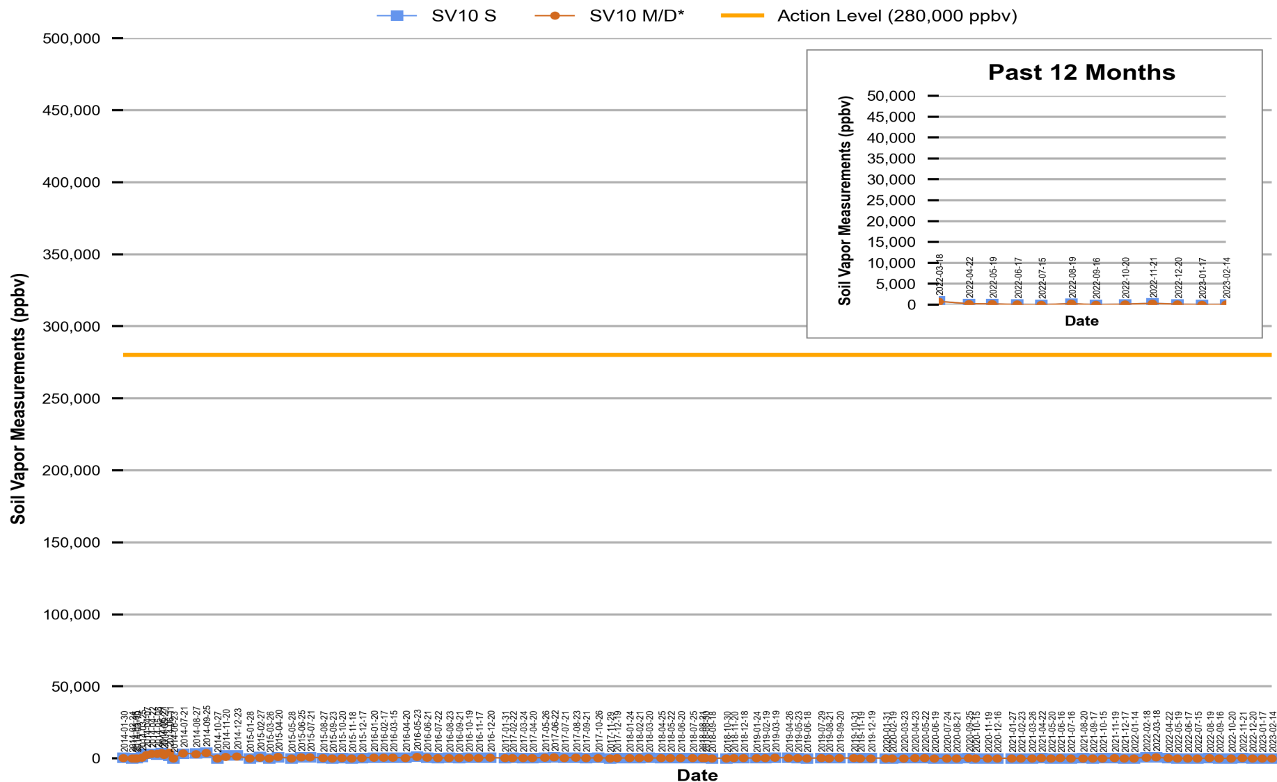
Figure 9 Red Hill - Tank 10 (JP-5) Soil Vapor Measurements (Jan 2014 Through Feb 2023)
