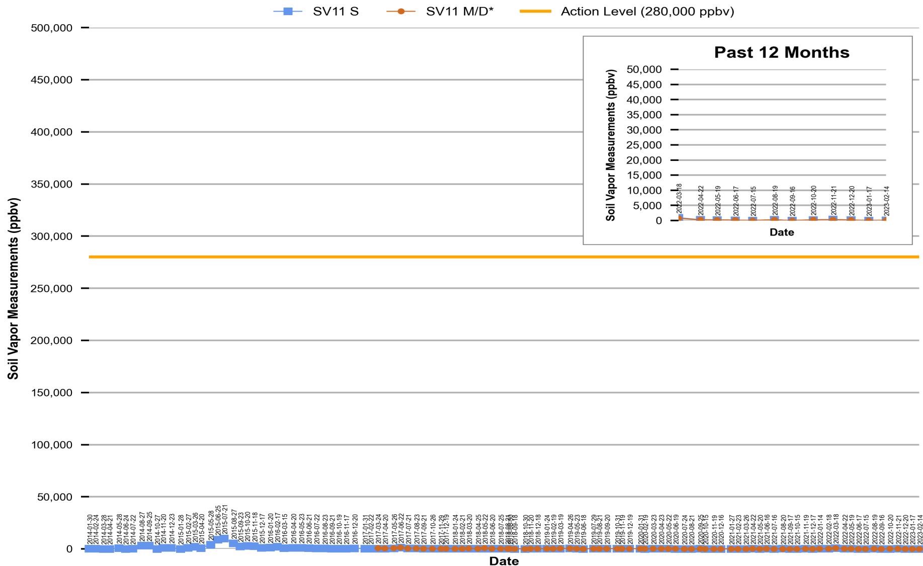
Figure 10 Red Hill - Tank 11 (JP-5) Soil Vapor Measurements (Jan 2014 Through Feb 2023)
