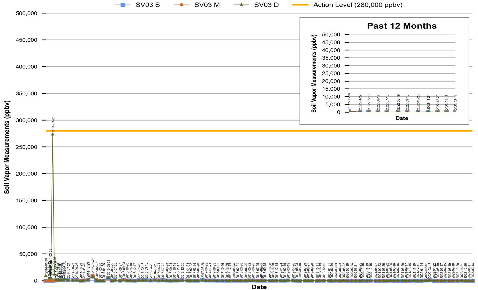
Figure 2 Red Hill - Tank 03 (F-24) Soil Vapor Measurements (Jan 2014 Through Feb 2023)
