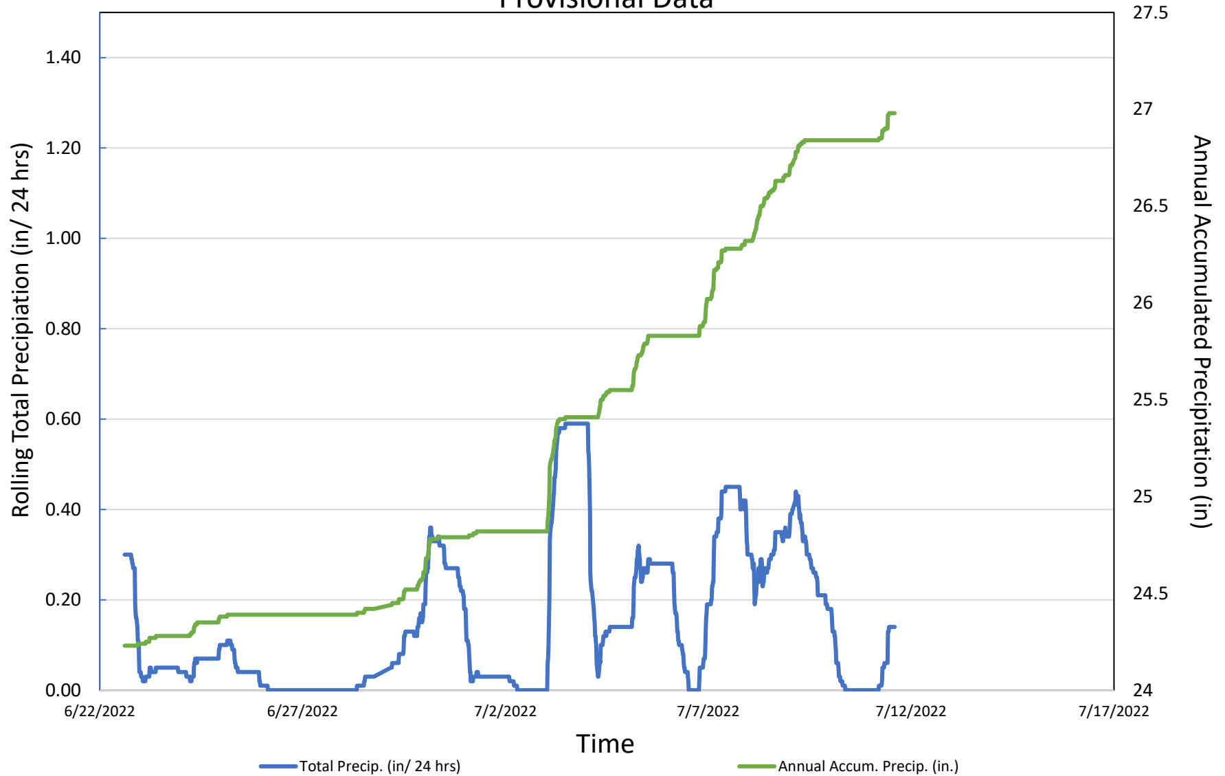
Figure 2: Rain Gauge MOAH1 Chart Voanalua 2N, No. 1900B66A Provisional Data
