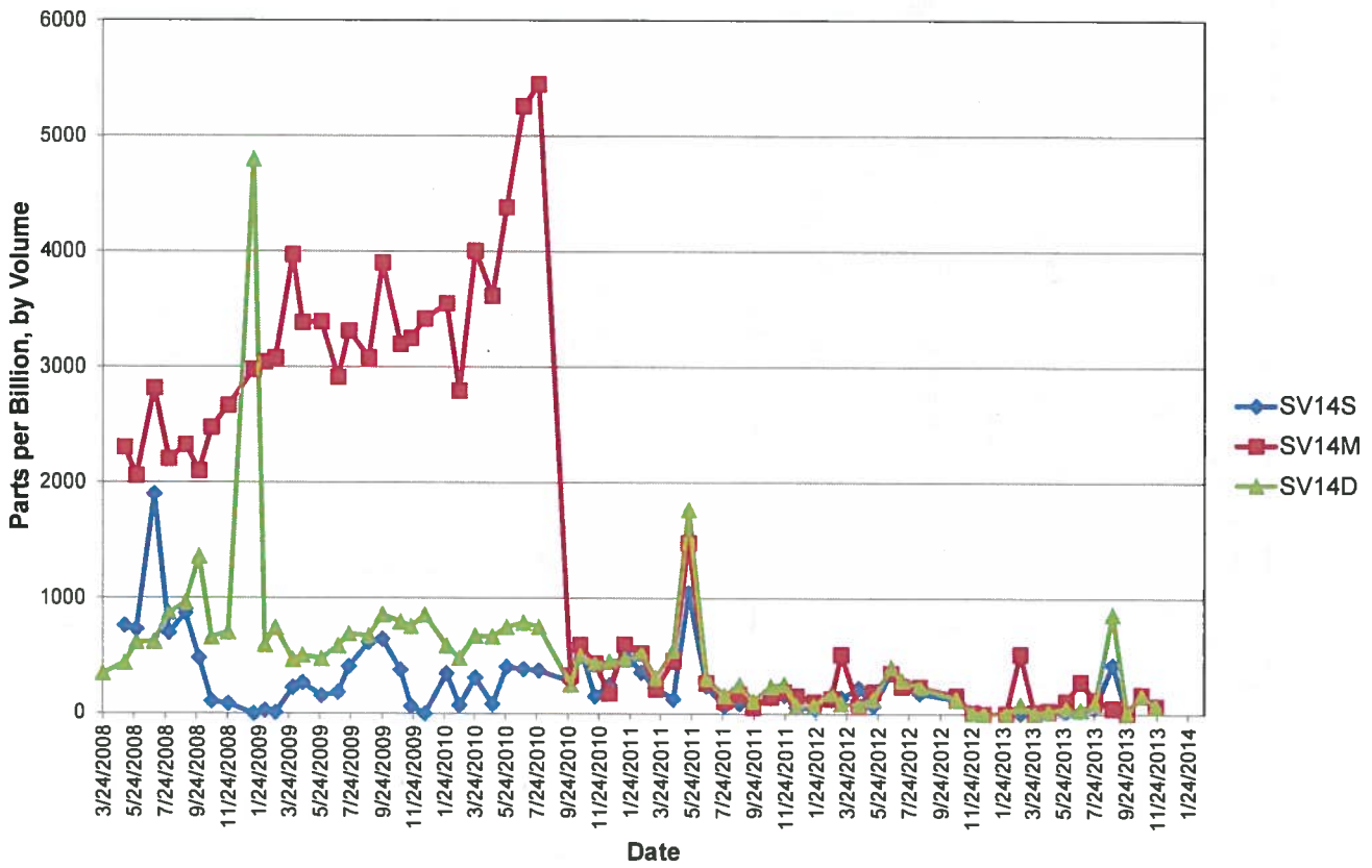
Figure 13 Soil Vapor Measurements SV14
