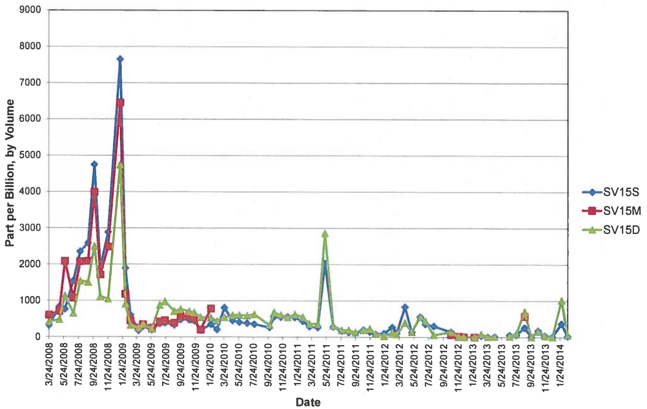
Figure 14 Soil Vapor Measurements SV15
