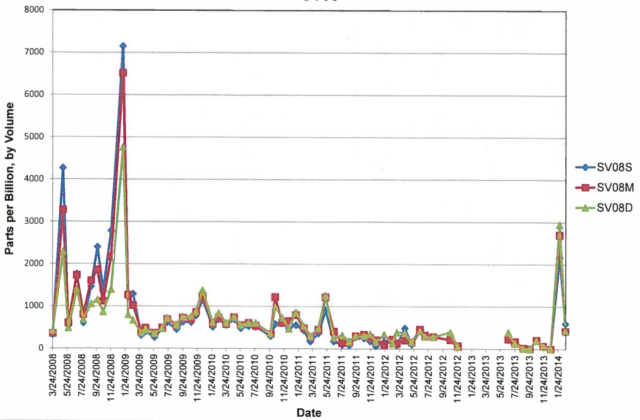
Figure 7 Soil Vapor Measurements SV08
