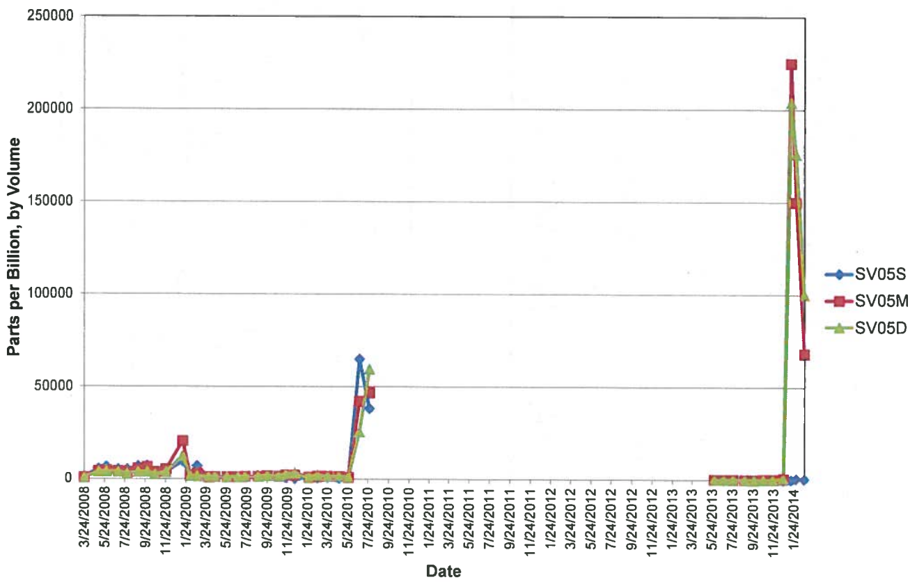
Figure 4 Soil Vapor Measurements SV05
