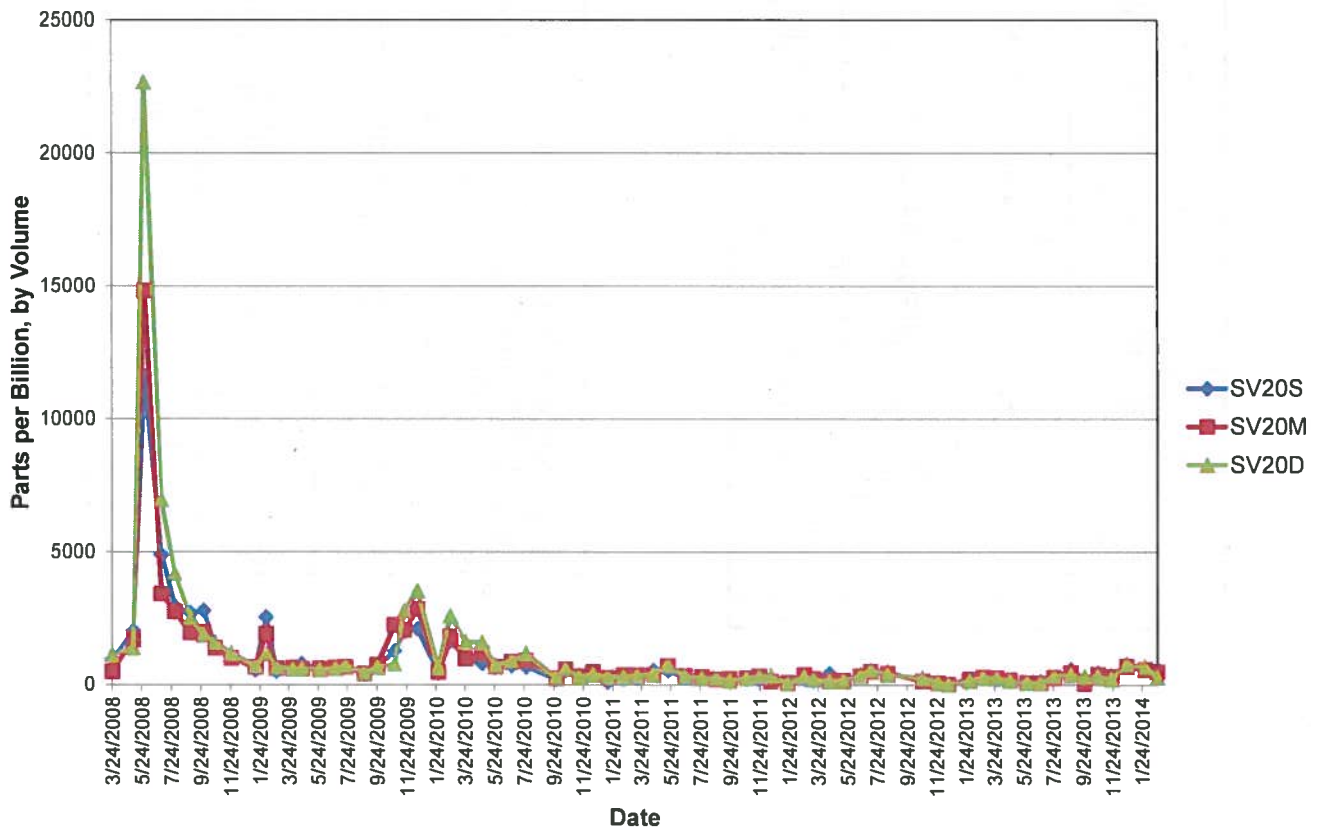
Figure 18 Soil Vapor Measurements SV20
