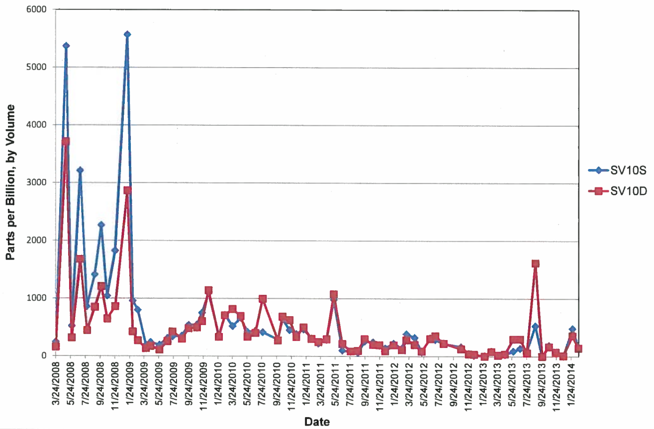
Figure 9 Soil Vapor Measurements SV10
