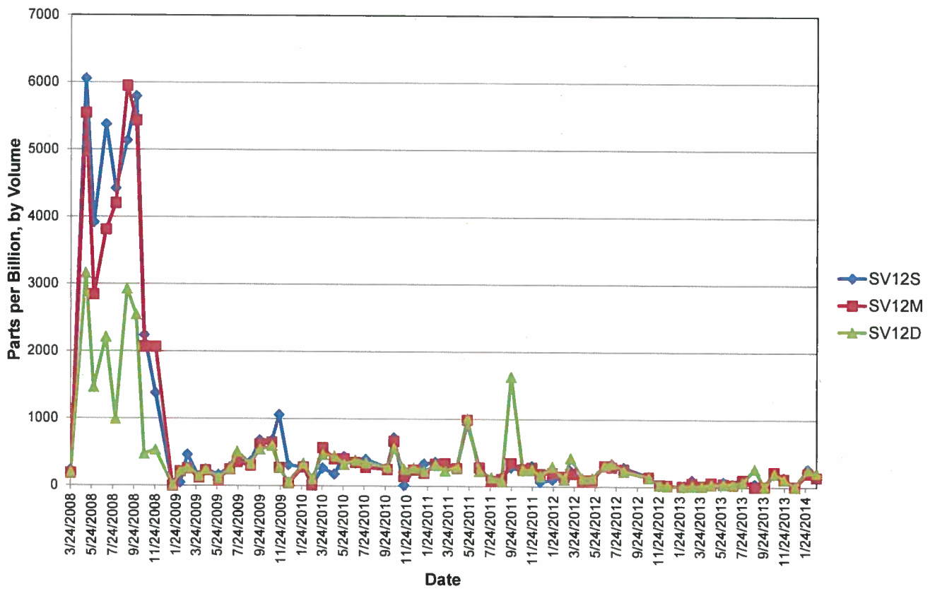
Figure 11 Soil Vapor Measurements SV12
