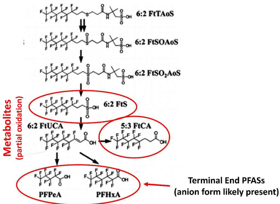
Figure 4. Example biological degradation of 6:2 FtTAoS - into fluoretelomer sulfonates and carboxylates before ultimately degrading to the Secondary Terminal PFAS compounds PFPeA - and PFHxA - (after Marjanoic et al. 2015). Structures should be in anion forms rather than acid forms, as depicted (hydrogen removed from hydroxyl group).
