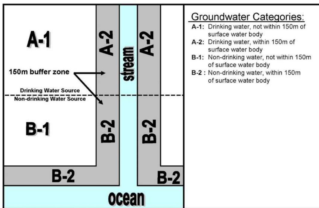
Figure 9. Groundwater categories used to develop the Tier 1 EAL lookup tables (HIDOH 2017a).
