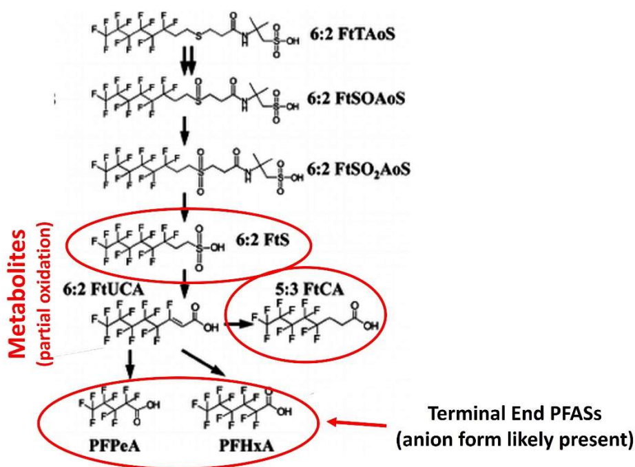
Figure 4. Example biological degradation of 6:2 FtTAoS - into fluotelomer sulfonates and carboxylates before ultimately degrading to the Terminal Endpoint compounds PFPeA - and PFHxA - (after Marjanoic et al. 2015). Structures should be in anion forms rather than acid forms, as depicted (hydrogen removed from hydroxyl group).
