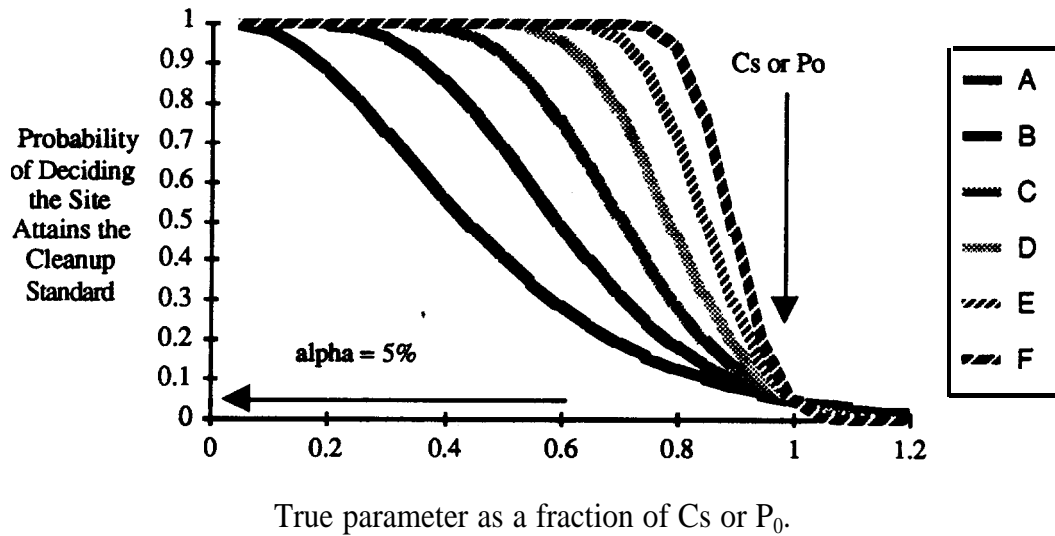
Figure A.2 Power Curves for \alpha = 5\%
