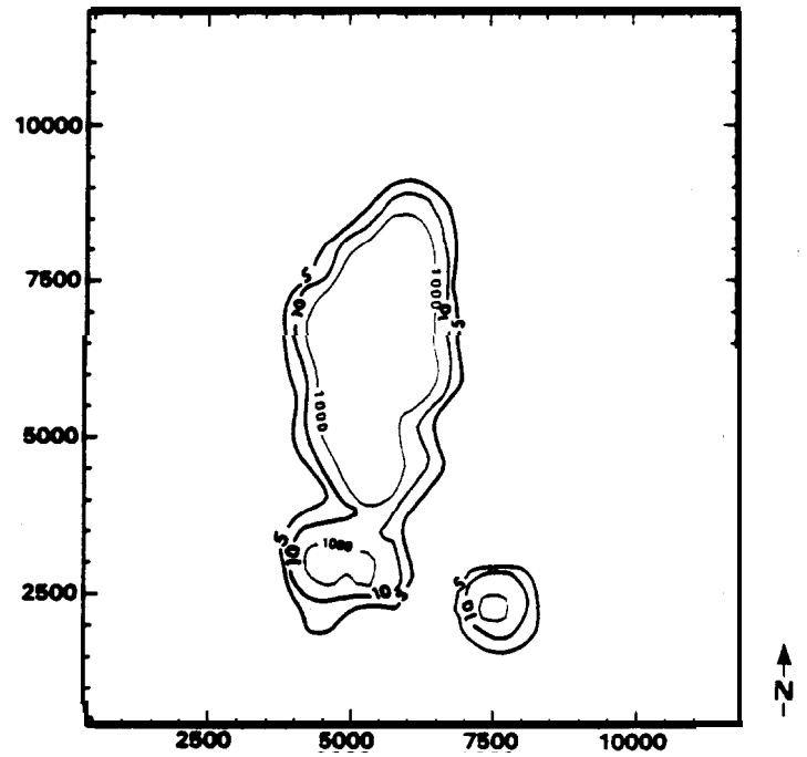
Figure 10.4 Contour Map of the Probability in Percent of a False Negative in the Remedial Action Areas and the 1,000 ppm Contour Line
