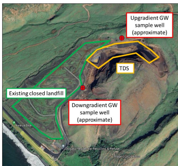
Approximate locations of groundwater monitoring wells.
