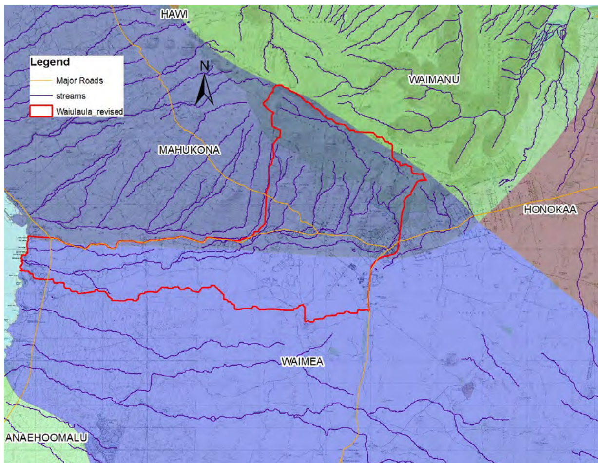
Figure 5: Groundwater Aquifers
