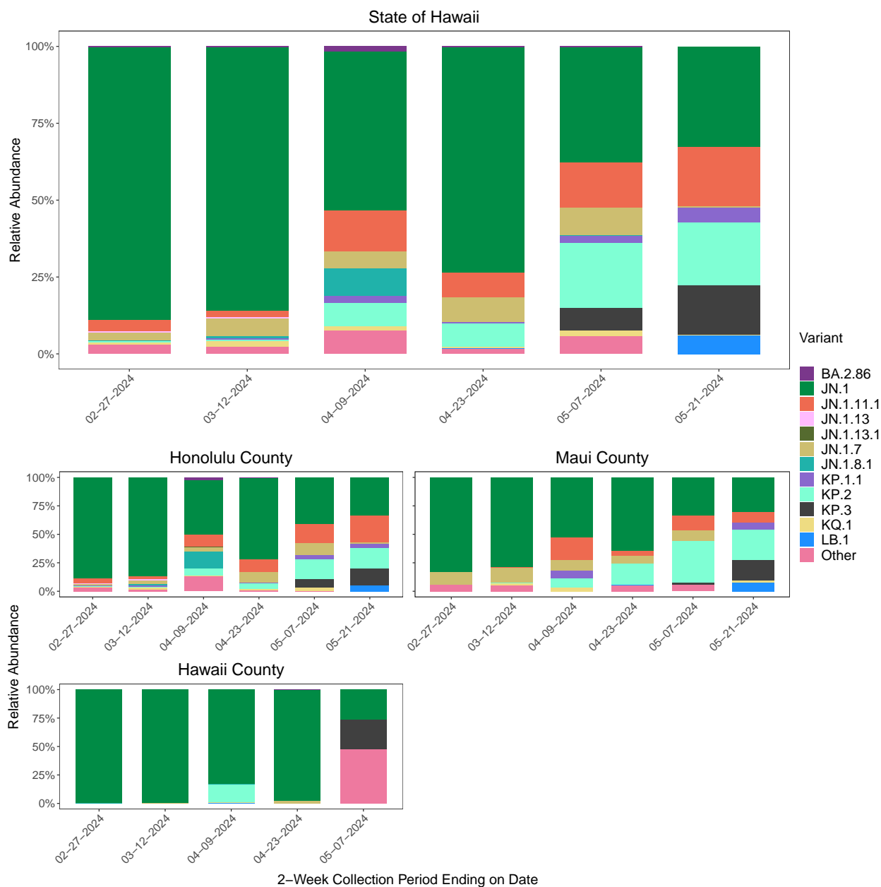
Figure 2. Stacked barplot demonstrating the relative abundance of SARS-CoV-2 aggregated lineages detected in wastewater across the State of Hawaii from 02/13/2024 to 05/21/2024.
