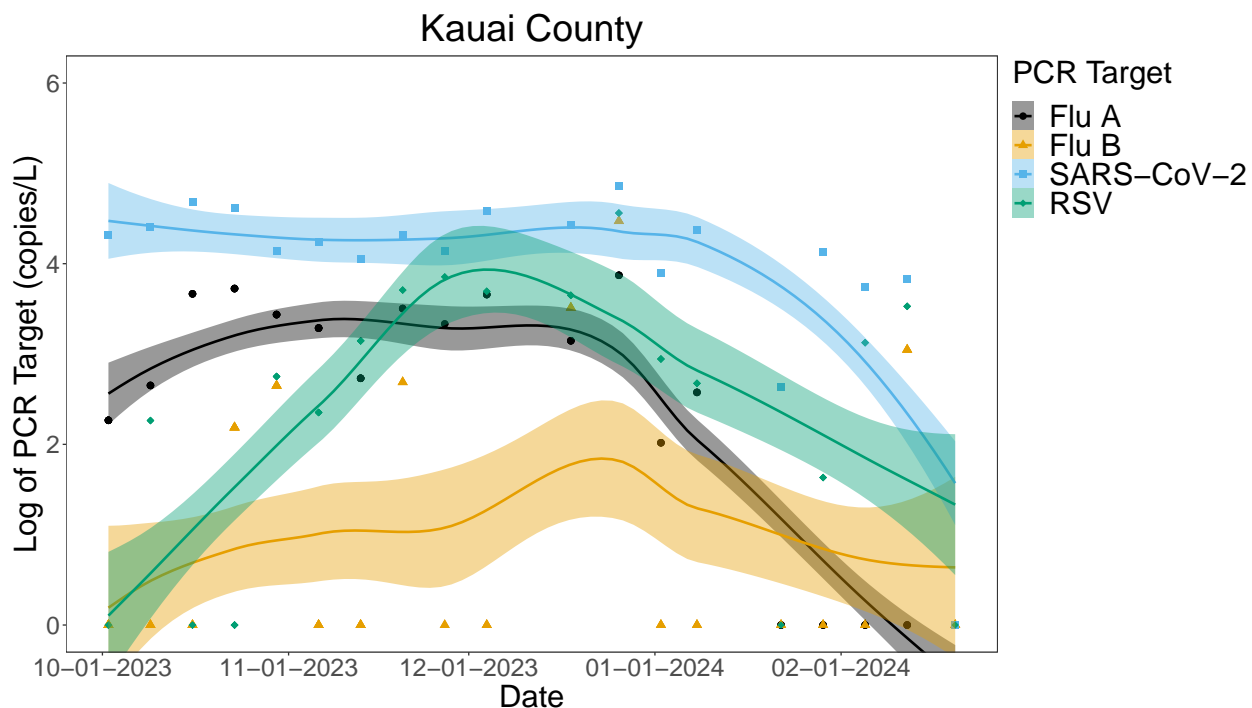
Figure 7. Log transformed average concentrations of Influenza A, Influenza B, SARS-CoV-2, and RSV in sewage from a Kauai County WWTP over time. Regression line created with a prediction interval from a locally weighted (LOESS) regression. Shaded region represents 95% confidence interval. Values below the limit of detection (LOD) are reported as 0 copies/L.
