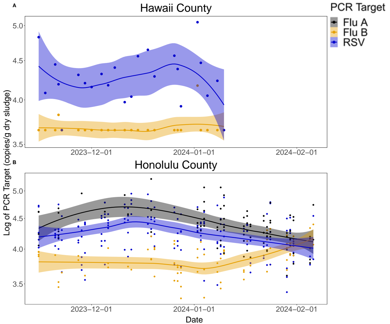
Figure 4. Log transformed normalized concentrations of Flu A, Flu B, and RSV in sewage (copies/g dry sludge) quantified by WastewaterSCAN for one WWTP from (A) Hawaii County and five from (B) Honolulu County. Regression line created with a prediction interval from a locally weighted (LOESS) regression. Shaded region represents 95% confidence interval.
