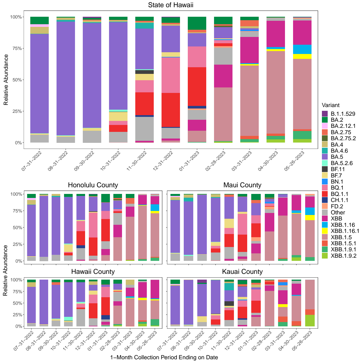
Figure 2. Stacked barplot demonstrating the relative abundance of SARS-CoV-2 aggregated lineages detected in wastewater across the State of Hawaii from samples collected from 07/01/2022 to 05/26/2023.
