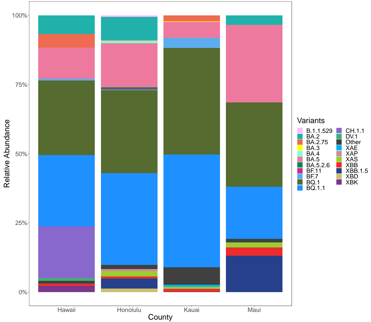
Figure 2. Stacked barplot demonstrating the relative abundance of SARS-CoV-2 aggregated lineages detected in wastewater across all counties in the state of Hawaii from samples collected in December 2022 - January 2023.
