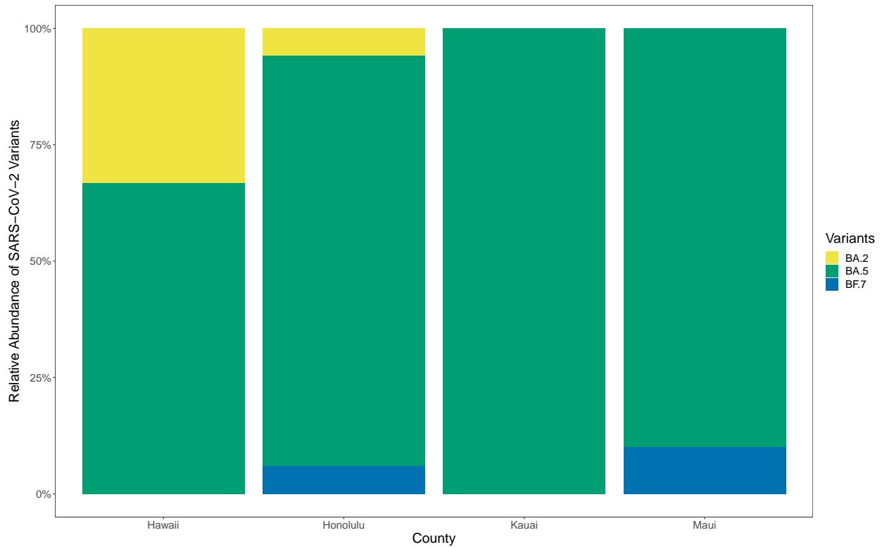
Figure 2. Stacked barplot demonstrating the relative abundance of SARS-CoV-2 variants detected in wastewater across all counties in the state of Hawaii from samples collected in October 2022.
