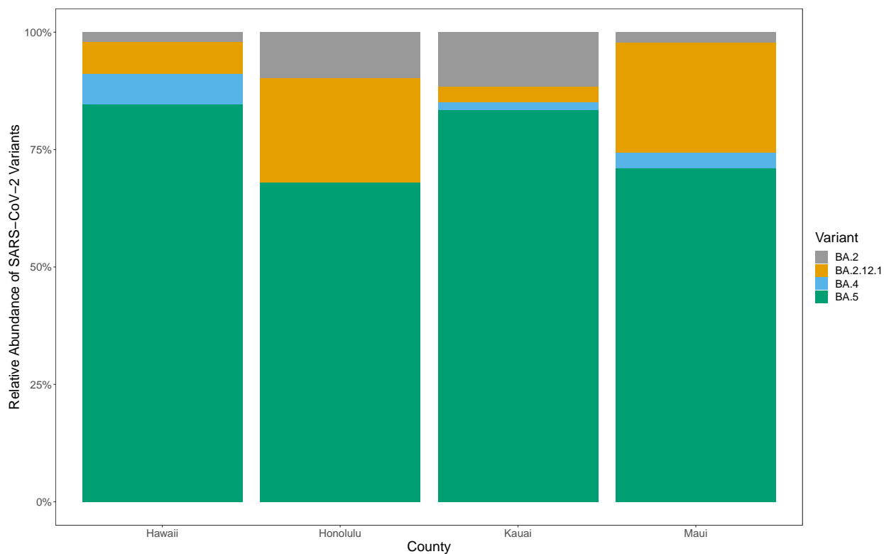
Figure 2. Stacked barplot demonstrating the relative abundance of SARS-CoV-2 variants detected in wastewater across all counties in the state of Hawaii from samples collected from 6/1/22 to 9/22/22.
