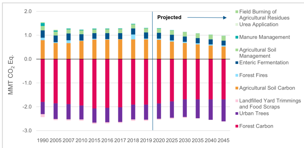
Figure 7-6: GHG Emissions and Projections from the AFOLU Sector under the Baseline Scenario
