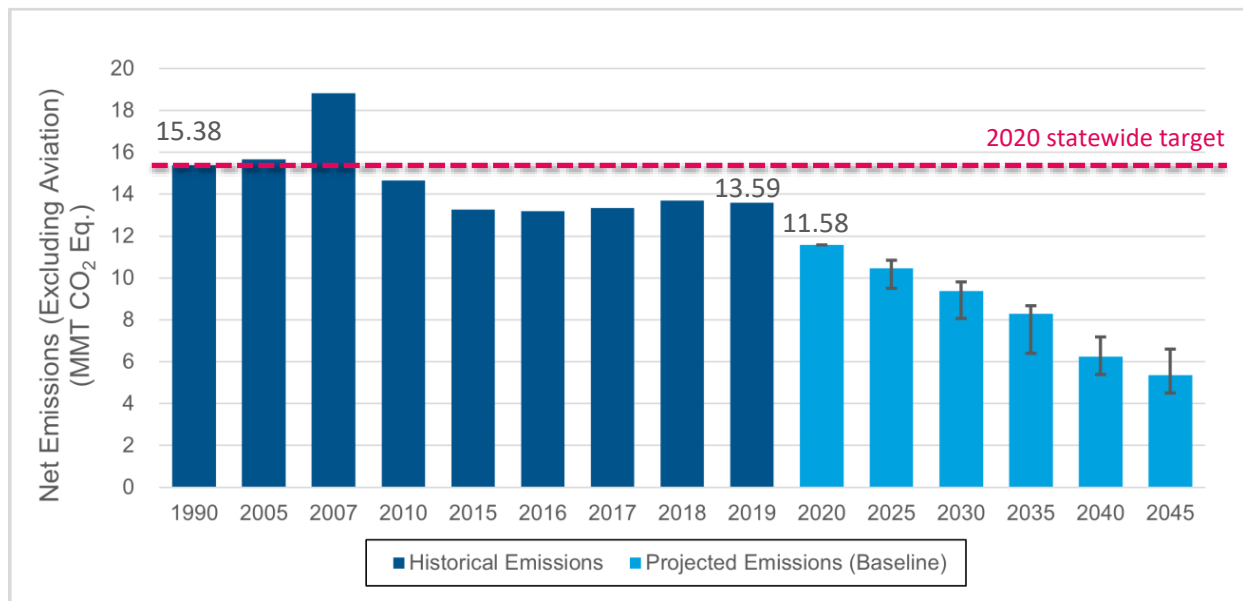
Figure 8-1: Hawai'i Net GHG Emissions Inventory Estimates and Projections (Including Sinks, Excluding Aviation)
