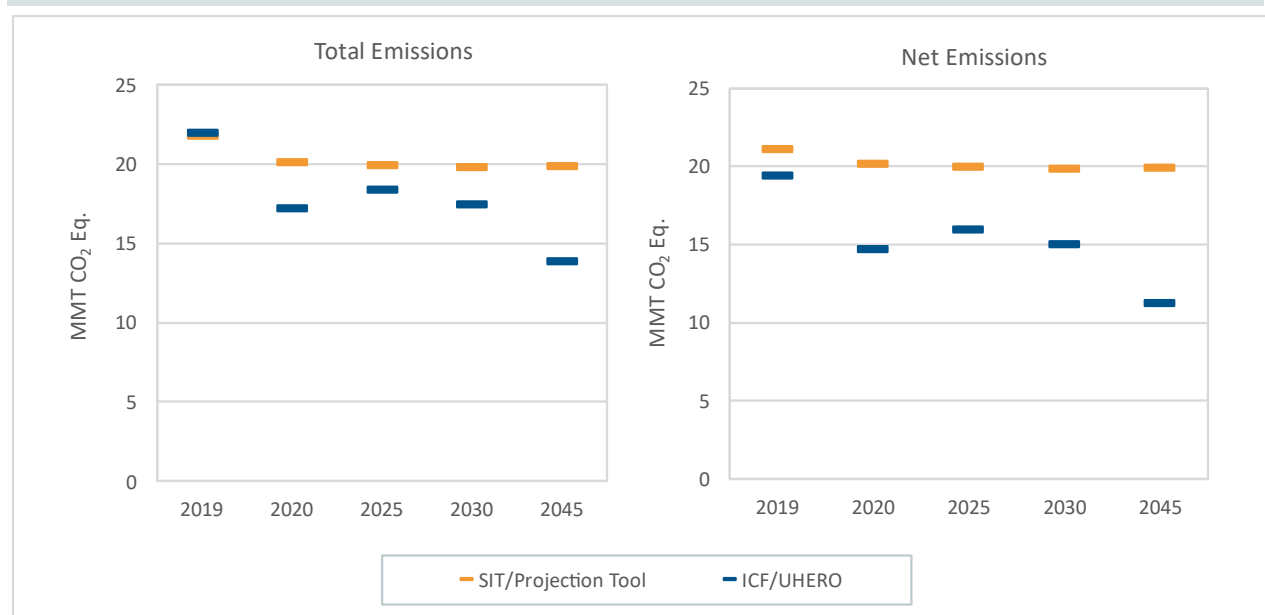
Figure K-2: Comparison of Total and Net GHG Emission Estimates (2019, 2020, 2025, 2030, and 2045)
