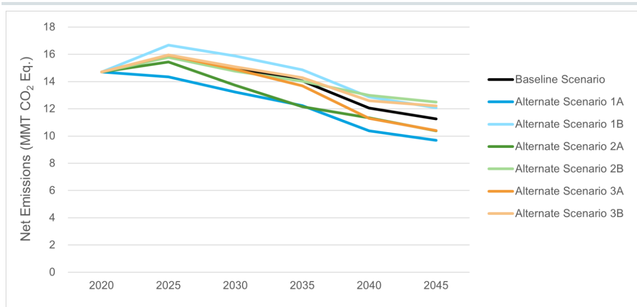
Figure 7-2: Projected Hawai'i Net GHG Emissions under each Scenario (Including Sinks and Aviation)
