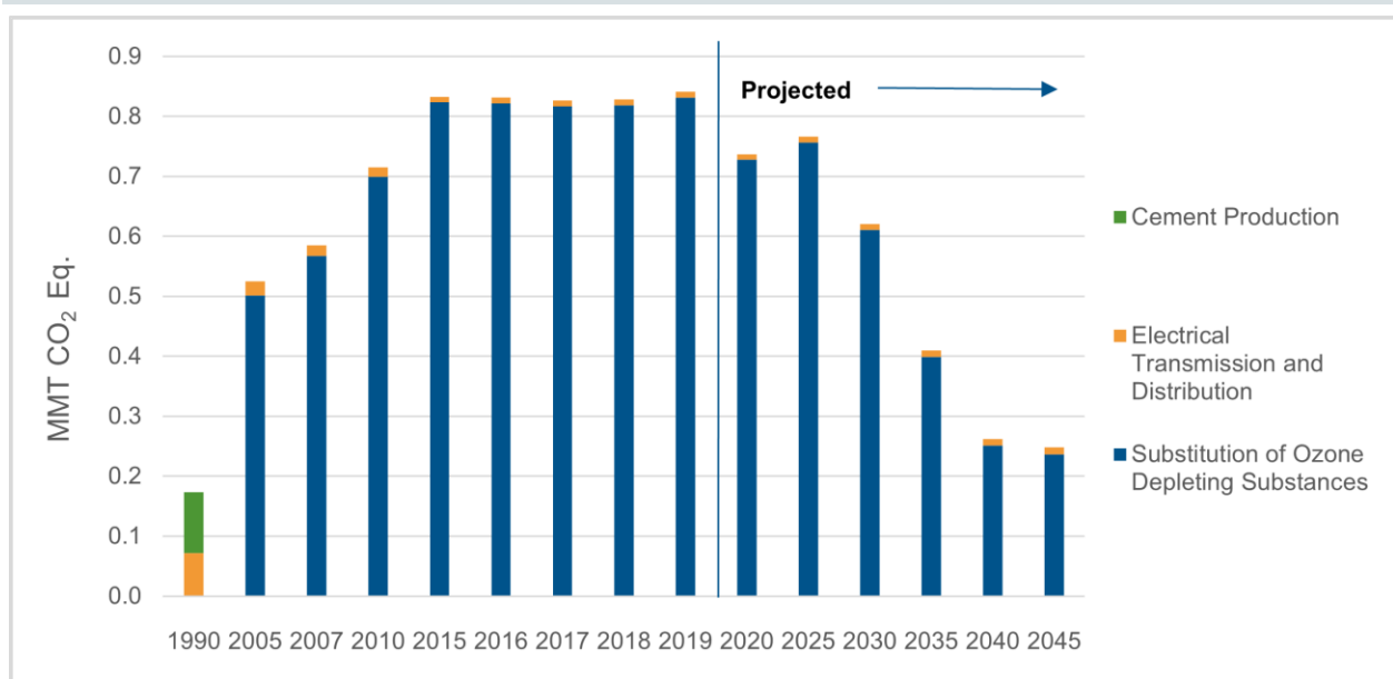
Figure 7-5: GHG Emissions and Projections from the IPPU Sector under the Baseline Scenario
