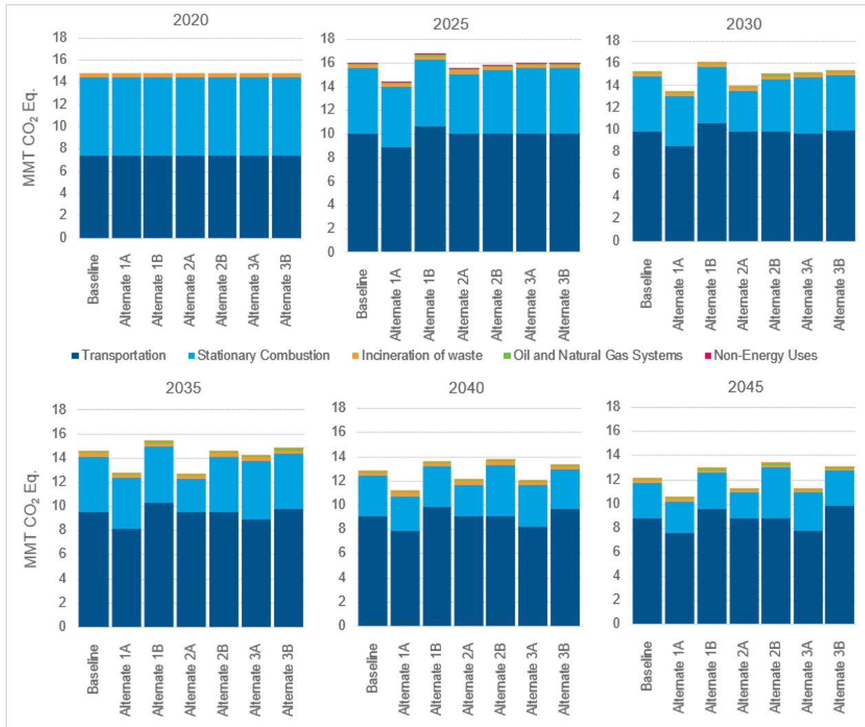
Figure 7-4: GHG Projections from the Energy Sector under each Scenario (Including Aviation)
