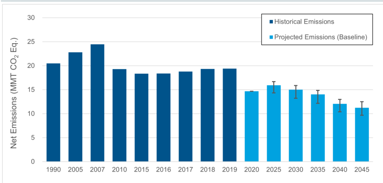
Figure 7-1: Hawai'i Net GHG Emissions by Year (Including Sinks and Aviation)
