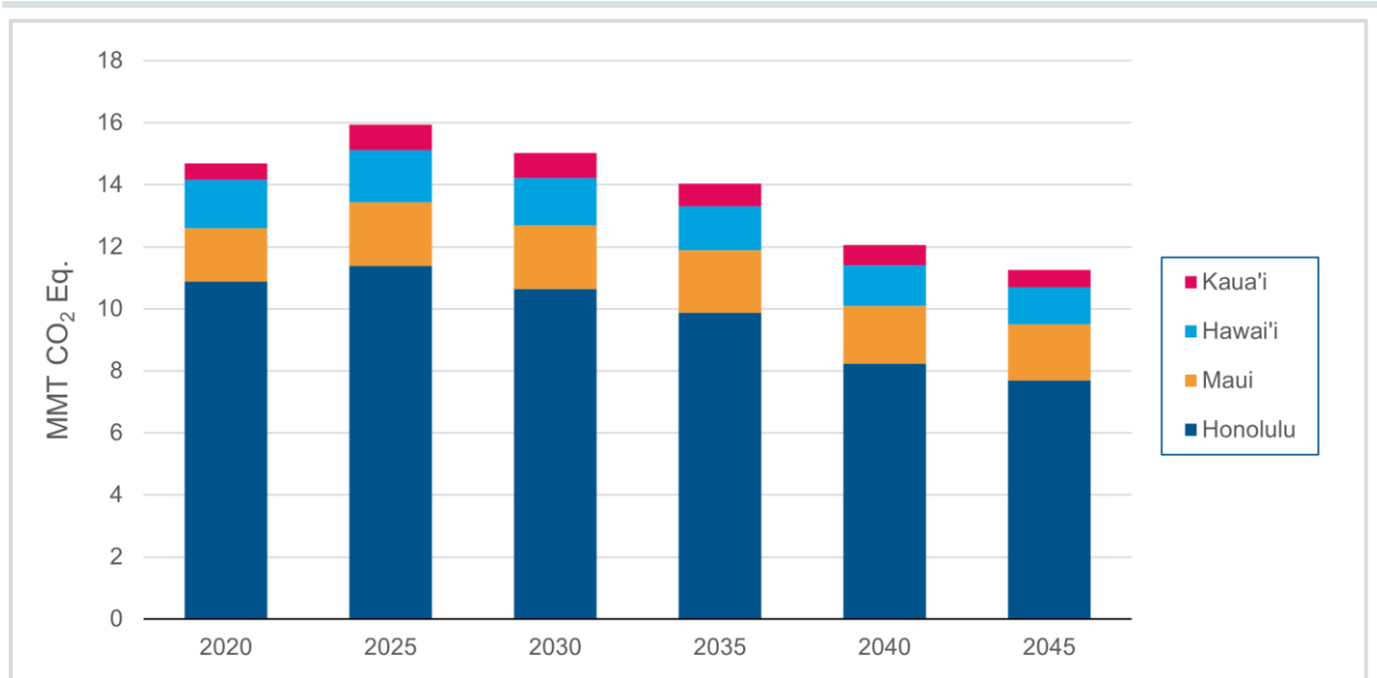
Figure 7-8: Projected Net GHG Emissions under the Baseline Scenario by County (2020, 2025, 2030, 2035, 2040, and 2045) (Including Sinks and Aviation)
