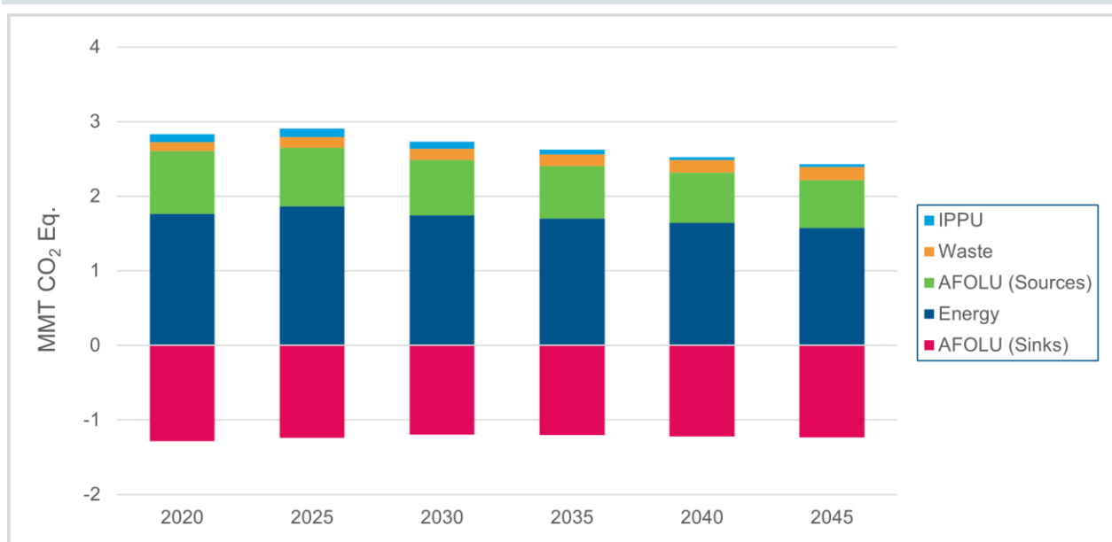
Figure 7-10: Hawai'i County GHG Emission Projections under the Baseline Scenario by Sector (2020, 2025, 2030, 2035, 2040, and 2045) Including Sinks and Aviation)
