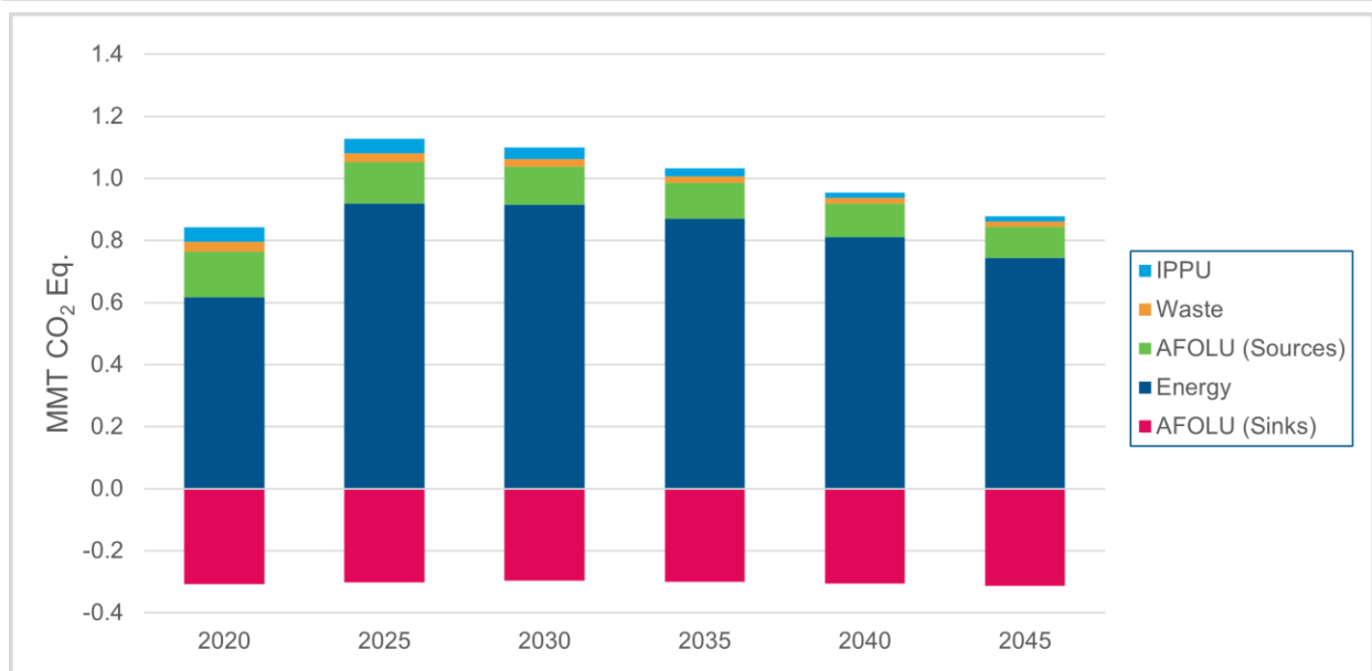
Figure 7-12: Kaua'i County GHG Emission Projections under the Baseline Scenario by Sector (2020, 2025, 2030, 2035, 2040, and 2045) (Including Sinks and Aviation)
