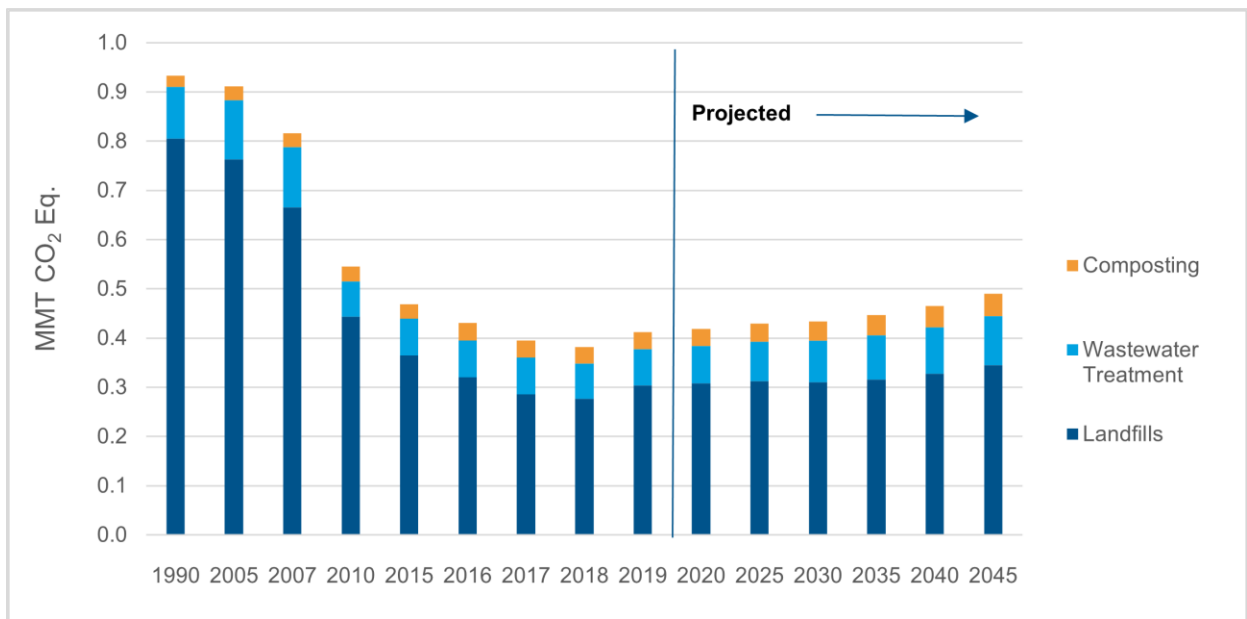
Figure 7-7: GHG Emissions and Projections from the Waste Sector under the Baseline Scenario
