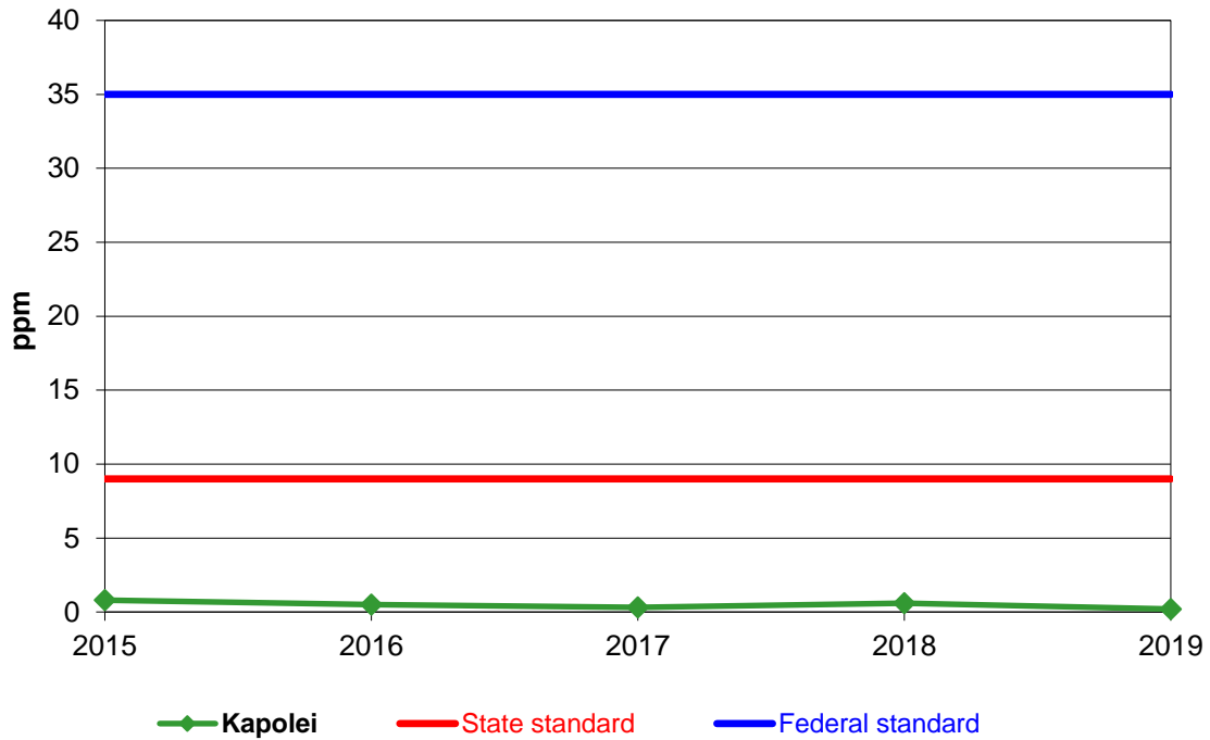
Figure 2. Annual Average of Maximum 8-hour Carbon Monoxide: 2015 - 2019
