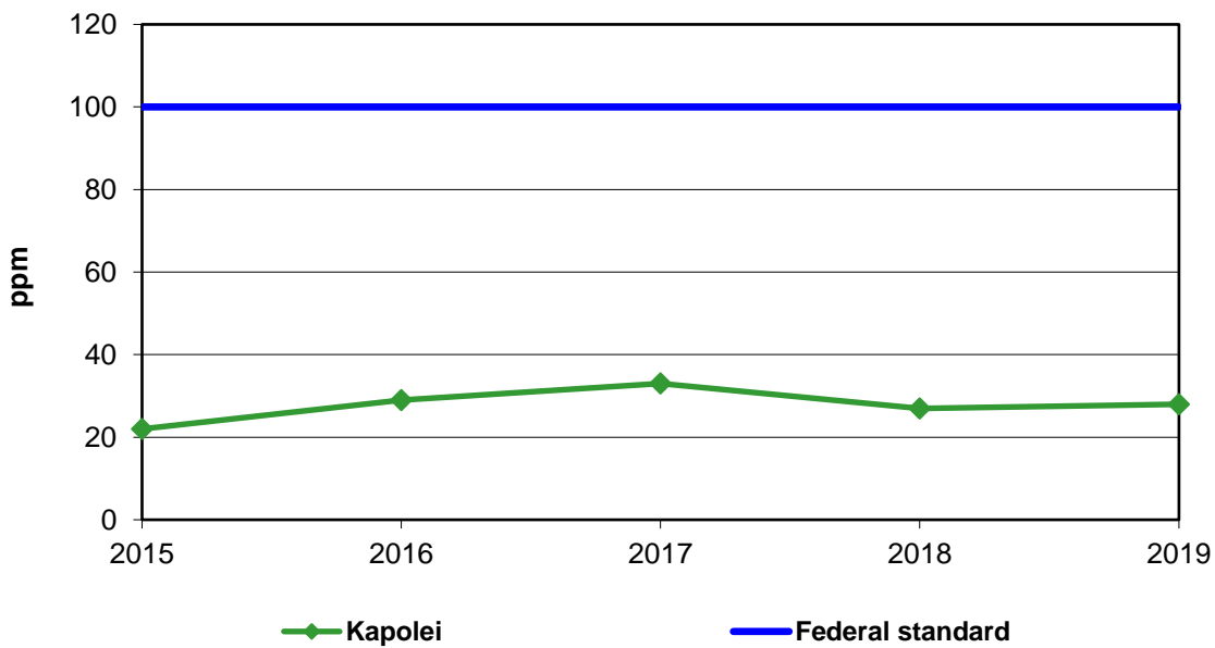
Figure 8. 98 th Percentile 1-hour Nitrogen Dioxide: 2015 - 2019
