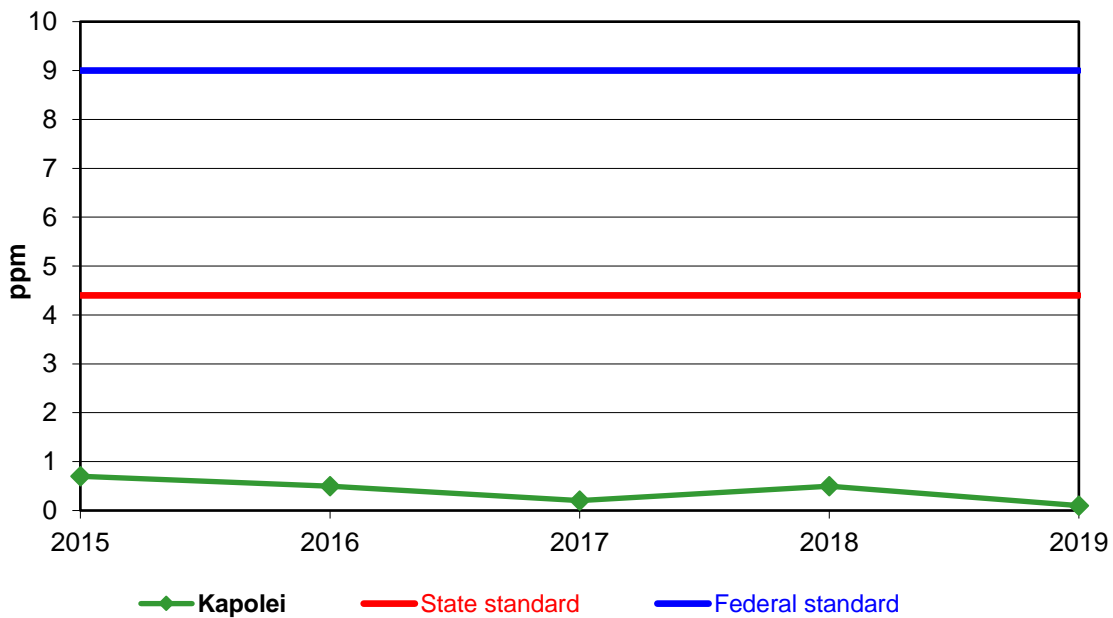
Figure 2. Annual Average of Maximum 8-hour Carbon Monoxide: 2015 - 2019
