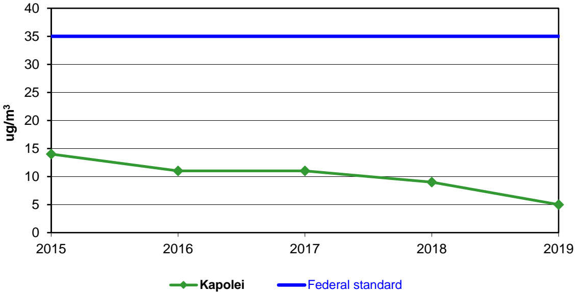
Figure 11. 98 th Percentile 24-hour PM 2.5 : 2015 - 2019
