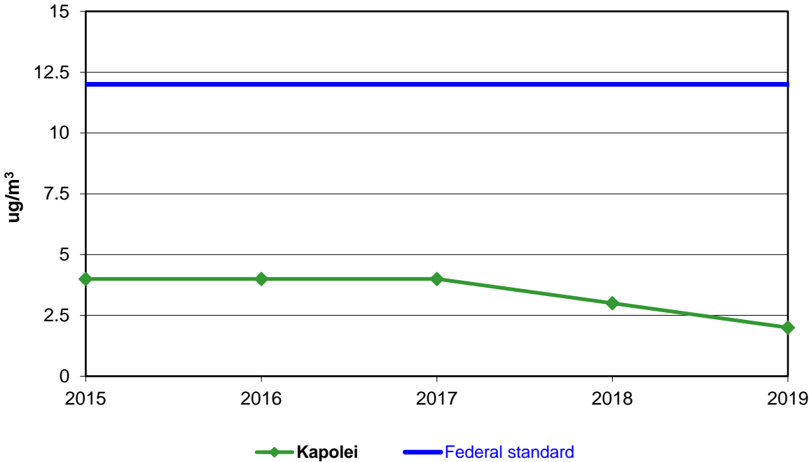
Figure 12. Annual Average of PM 2.5 : 2015 - 2019 (Average of all valid 24-hour values in the year)
