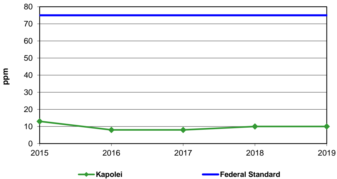
Figure 6. 99 th Percentile 1-hour Sulfur Dioxide: 2015 - 2019
