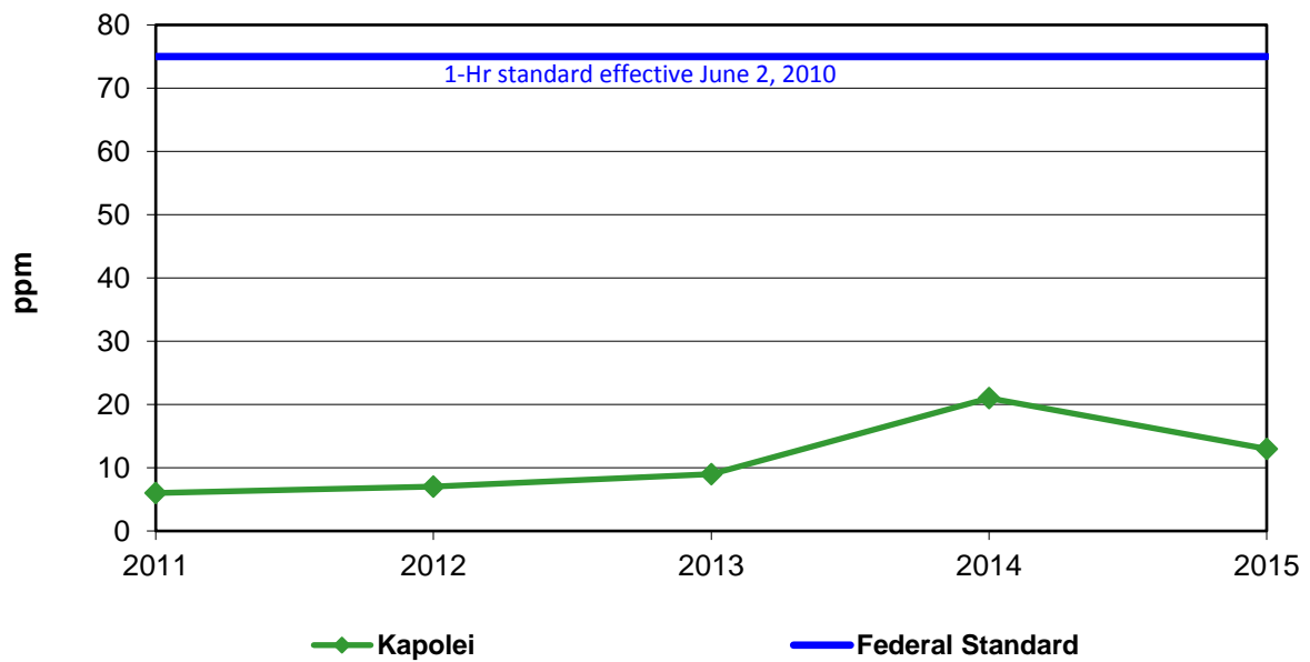
Figure 6. 99 th Percentile 1-Hour Sulfur Dioxide 2011 - 2015
