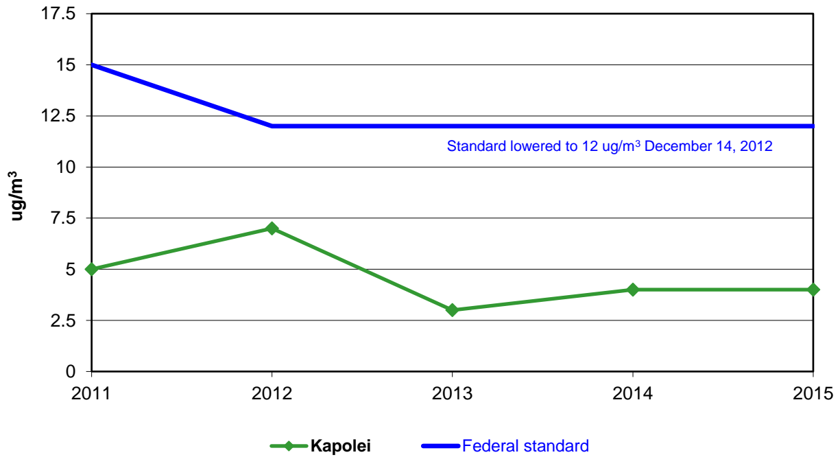
Figure 12. Annual Average of PM 2.5 : 2011 - 2015 (Average of all valid 24-hour values in the year)
