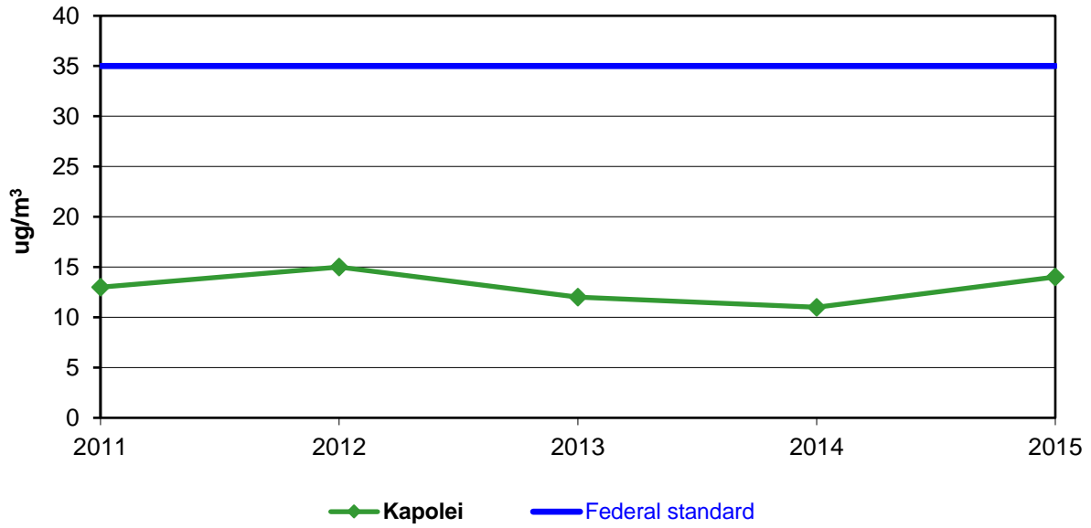
Figure 11. 98 th Percentile 24-hour PM 2.5 2011 - 2015
