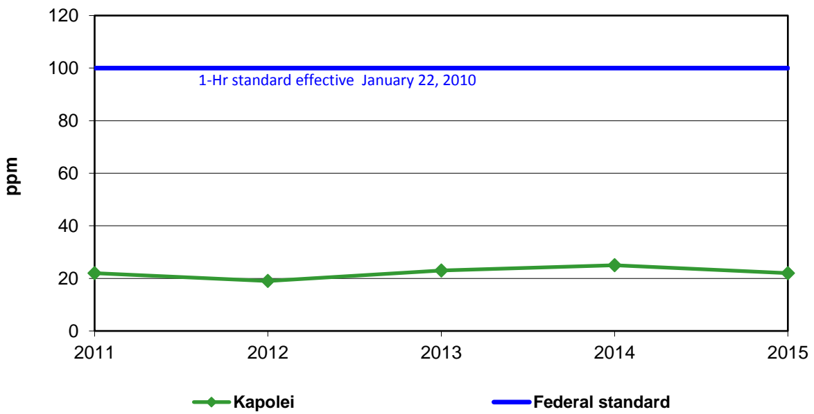
Figure 8. 98 th Percentile 1-Hour Nitrogen Dioxide 2011 - 2015
