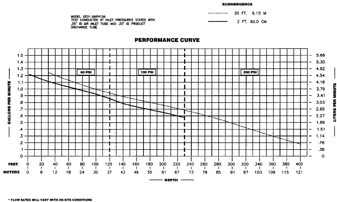
Figure 8 – Performance Curve 13
