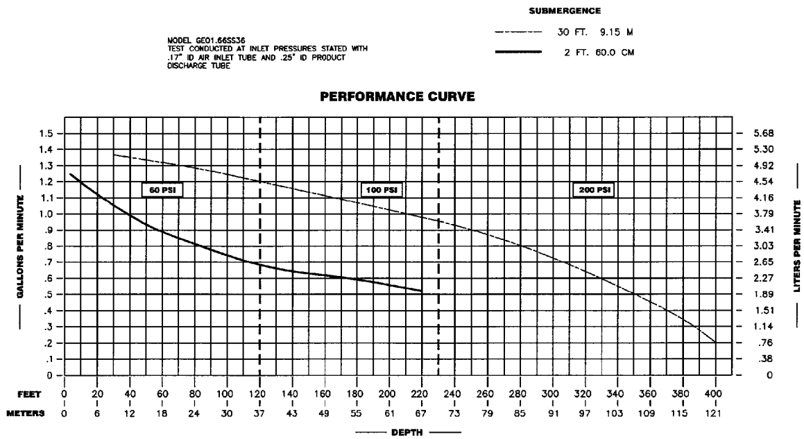
Figure 5 – Performance Curve 10
