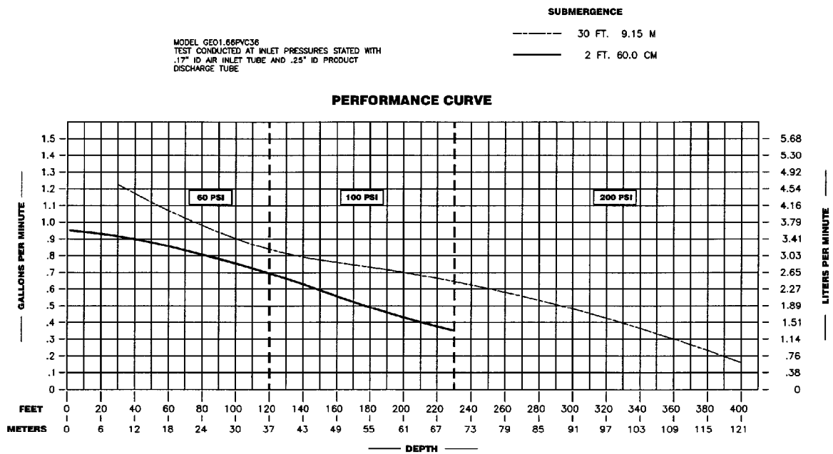
Figure 7 – Performance Curve 12
