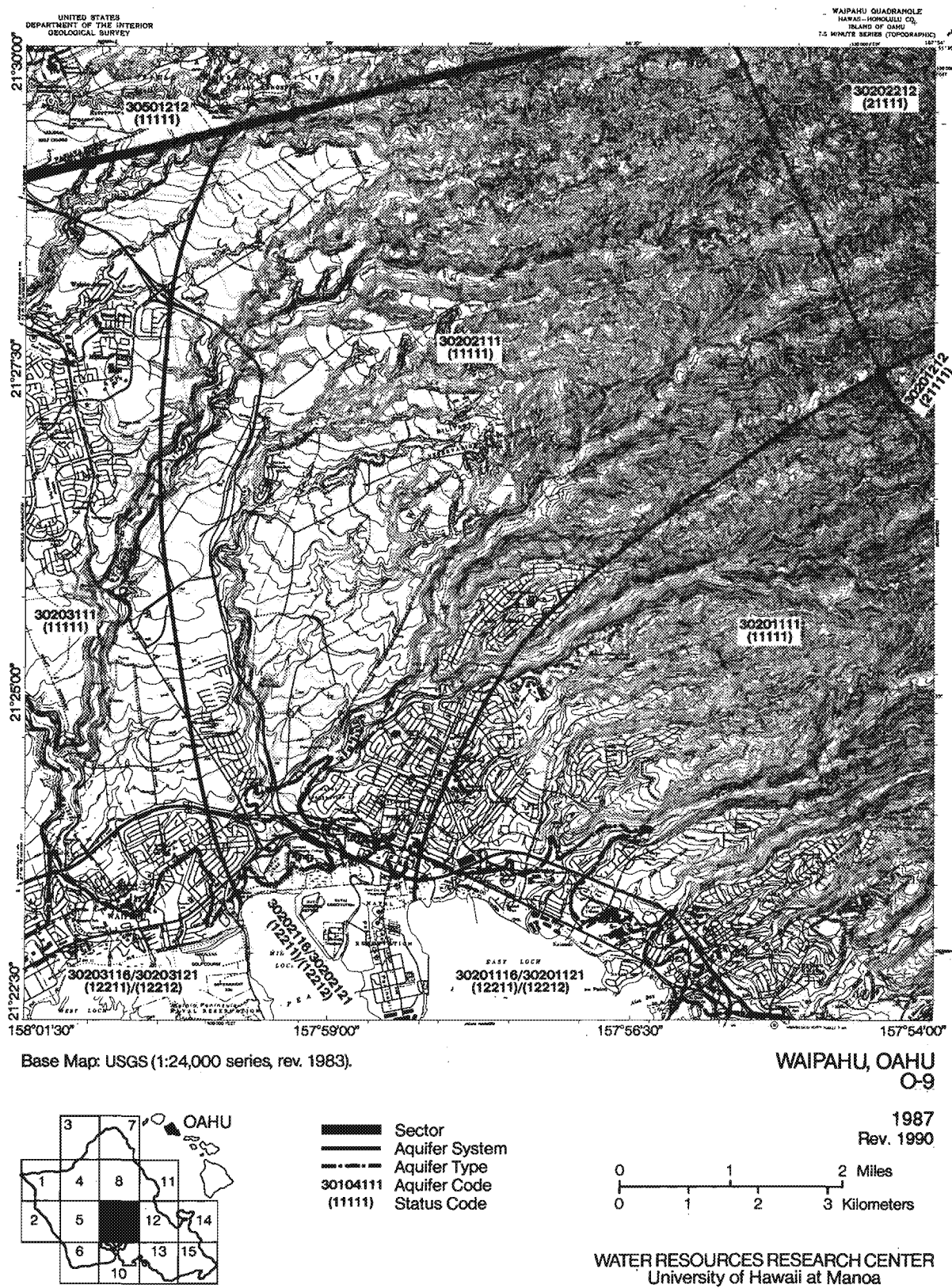
Figure 1.9. Aquifer classification map, Waipahu, O'ahu, Hawai'i
