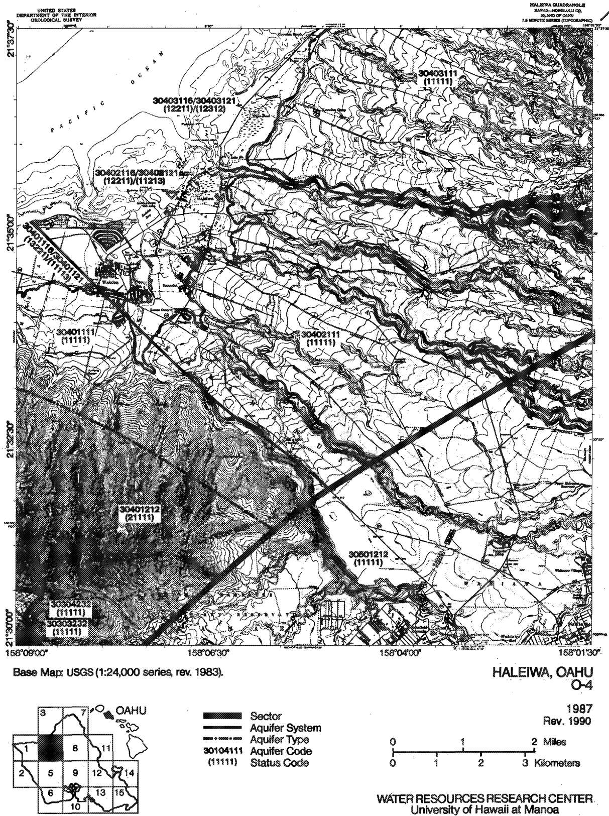
Figure 1.4. Aquifer classification map, Haleiwa, O'ahu, Hawai'i
