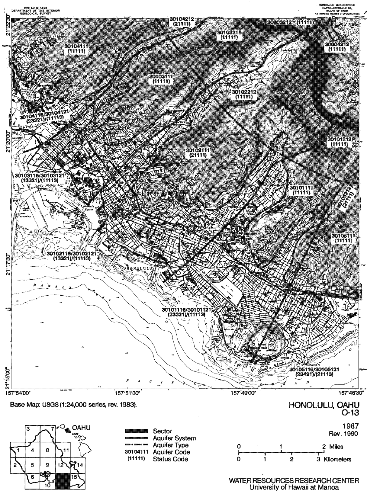
Figure 1.13. Aquifer classification map, Honolulu, O'ahu, Hawai'i
