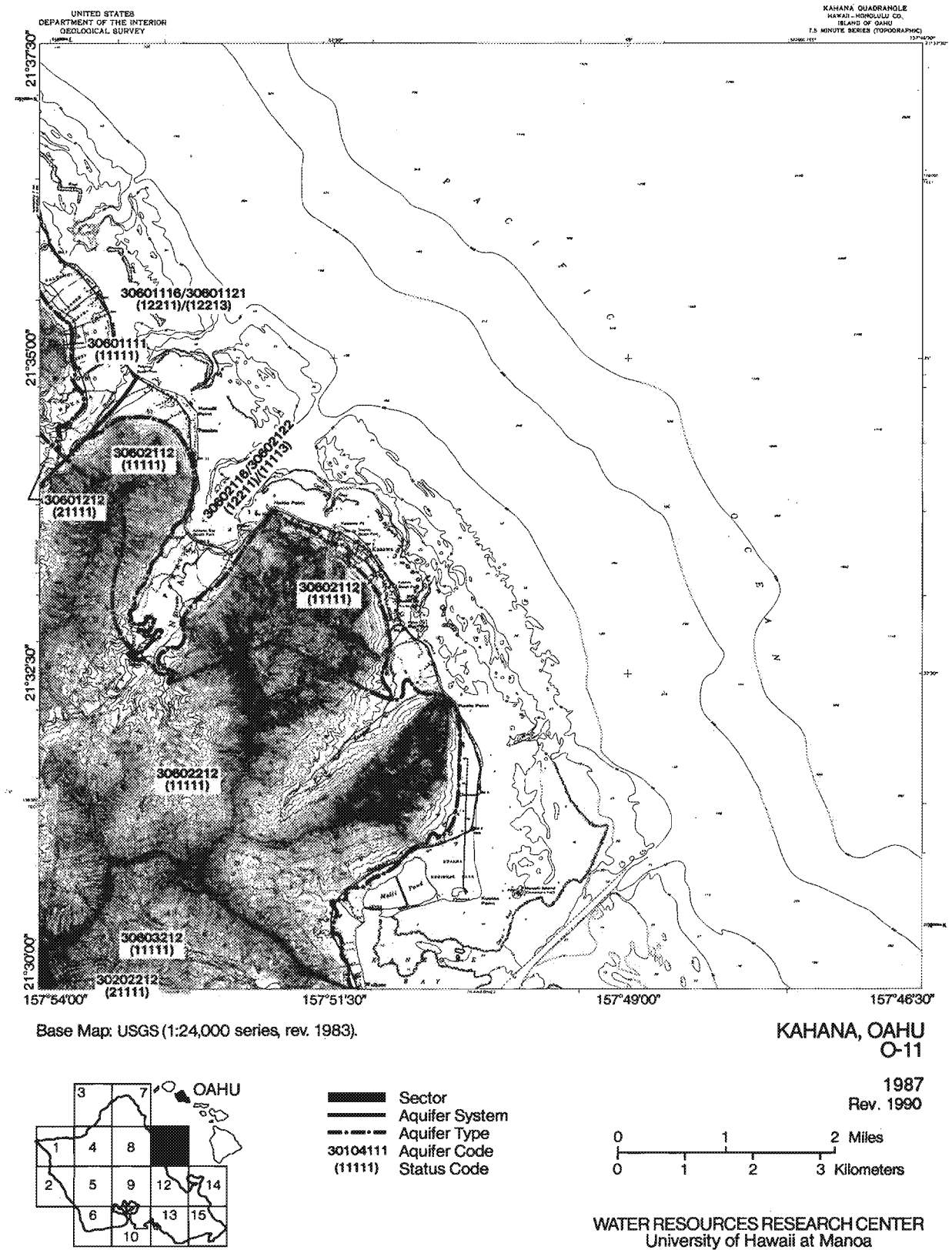
Figure 1.11. Aquifer classification map, Kahana, O'ahu, Hawai'i
