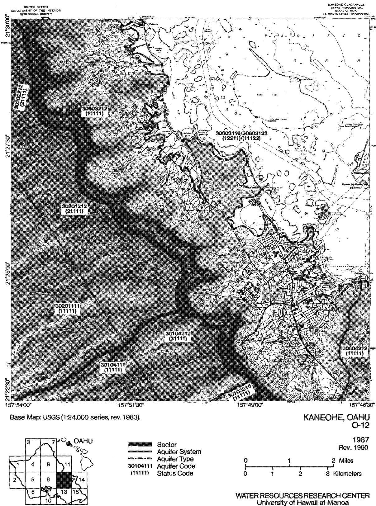
Figure 1.12. Aquifer classification map, Kaneohe, Oahu, Hawaii
