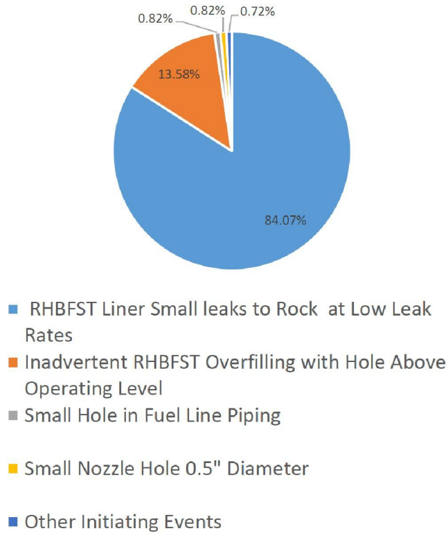
Figure 18: Initiating Event Category Contributors to the Frequency of All Acute Sequences
