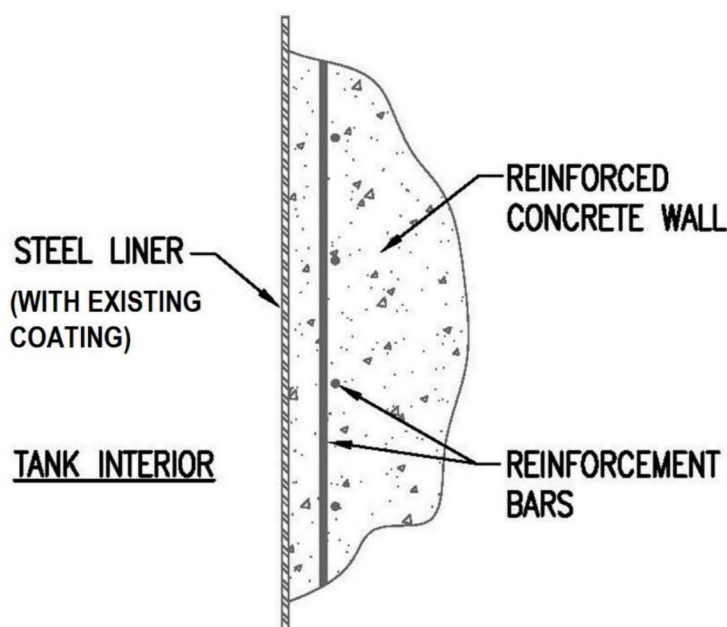
Figure 9: Tank Upgrade Alternative 1A - Typical Wall Section
