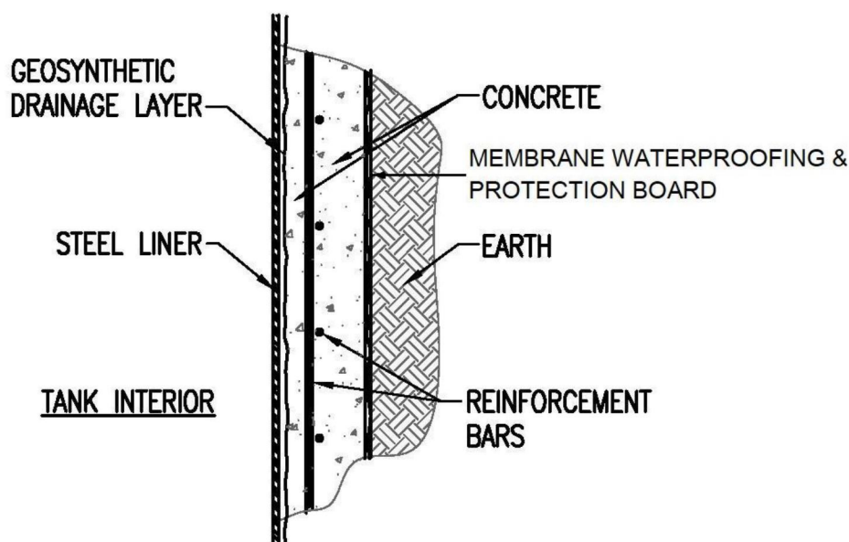
Figure 17: New Cut-and-cover Tanks - Typical Wall Section
