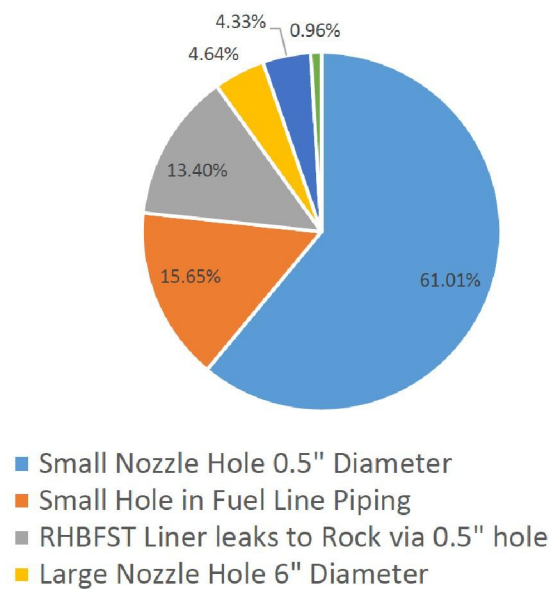
Figure 19: Initiating Event Category Contribution to the Frequency of Acute Sequences Releasing More than 120,000 Gallons
