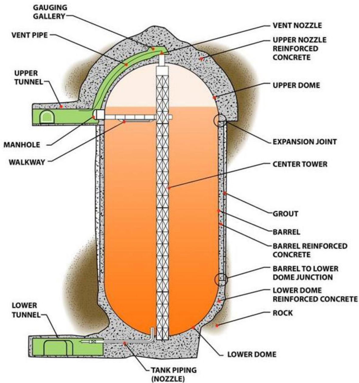
Figure 5: Cross-Section of Typical Red Hill Bulk Fuel Storage Tank
