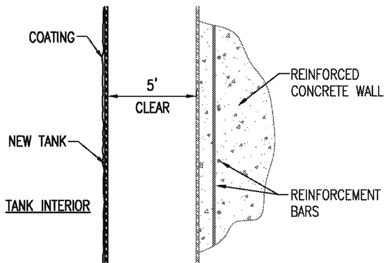
Figure 15: TUA 3A - Typical Wall Section
