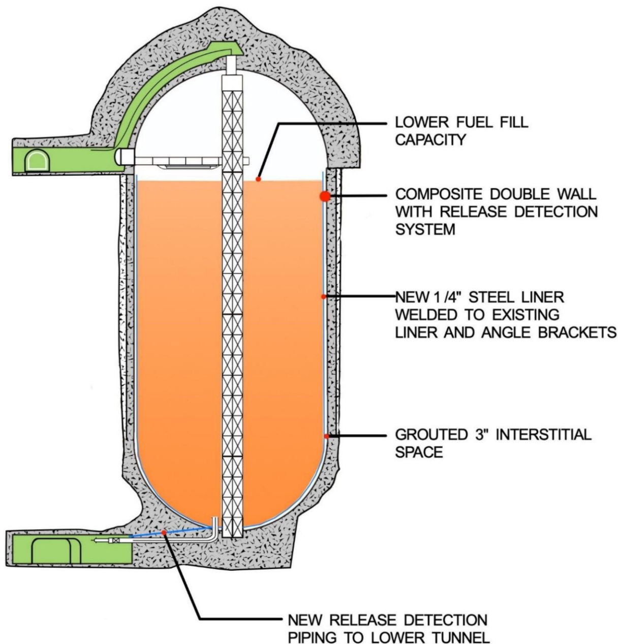
Figure 13: Tank Upgrade Alternative 2A/2B – Typical Tank Section
