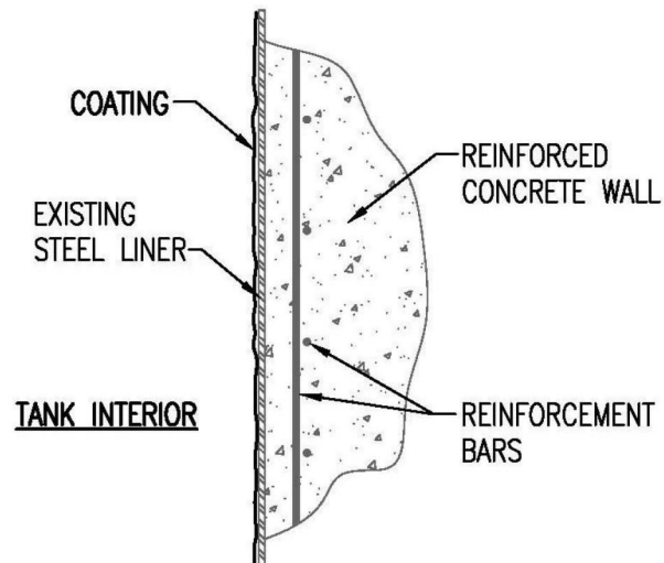
Figure 10: Tank Upgrade Alternative 1B - Typical Wall Section
