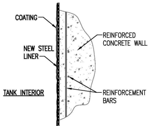
Figure 11: Tank Upgrade Alternative 1D - Typical Wall Section
