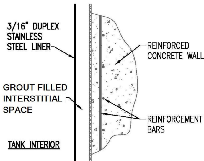
Figure 14: Tank Upgrade Alternative 2B - Typical Wall Section
