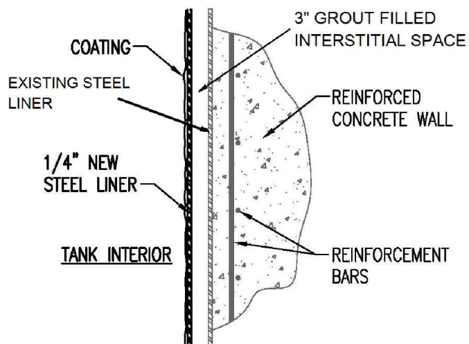
Figure 12: Tank Upgrade Alternative 2A - Typical Wall Section
