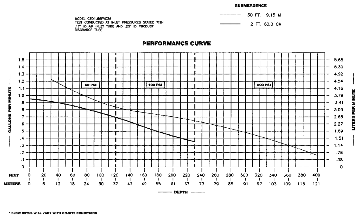
Figure 7 – Performance Curve 12
