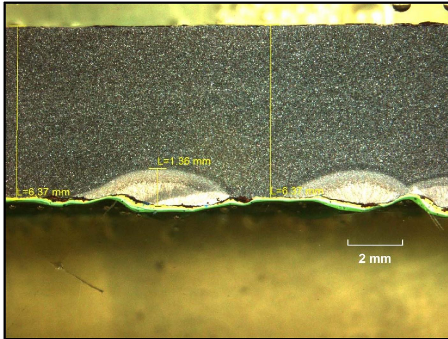
Figure 207. The prepared metallographic cross-section from Sample A2-4 is shown during examination with a stereomicroscope. The NDE indication was most likely locations of melting/re-solidification underneath the painted surface. No pitting was observed. (7X)
