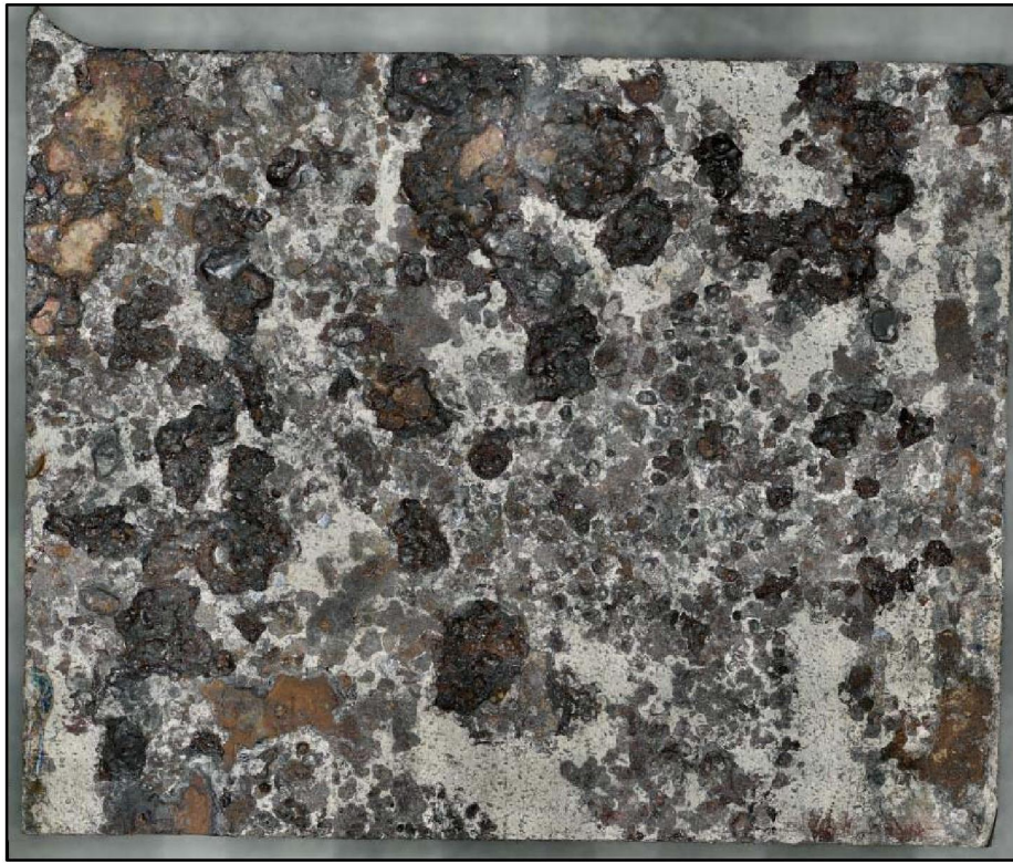
Figure 151. A screenshot of the 3D digital image of a specimen excised from Coupon 1 labeled as 1-3, after CO 2 blast cleaning
