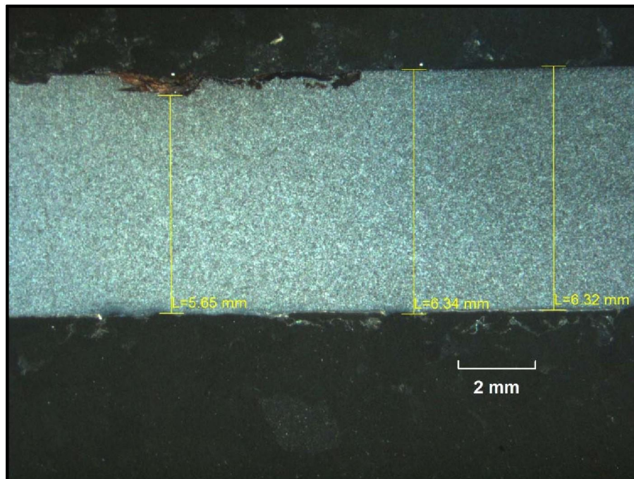
Figure 180. The prepared metallographic cross-section from Sample 1-1 is shown during examination with a stereomicroscope. The thickest location(s) are shown, as well as the thickness remaining underneath the deepest observed pit. (7X)
