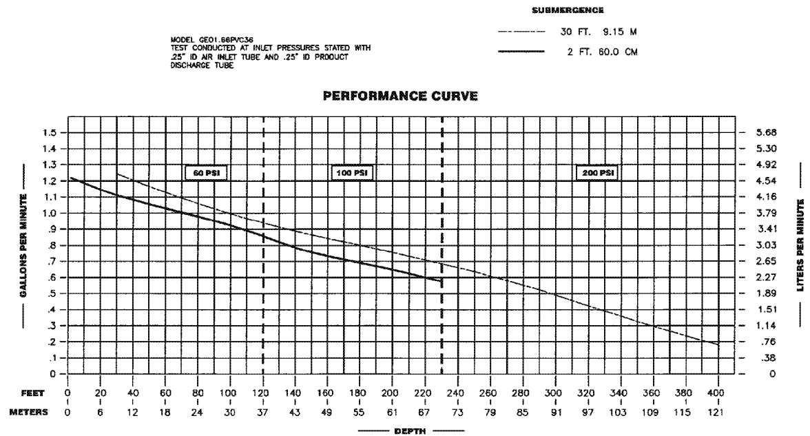
Figure 8 – Performance Curve 13
