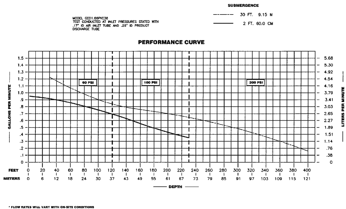
Figure 7 – Performance Curve 12
