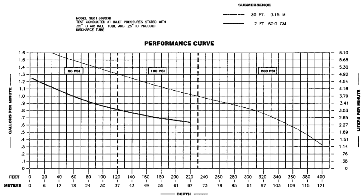
Figure 6 – Performance Curve 11
