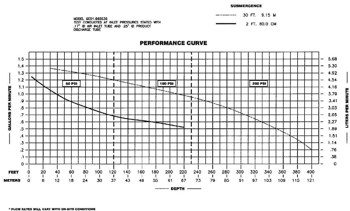
Figure 5 – Performance Curve 10
