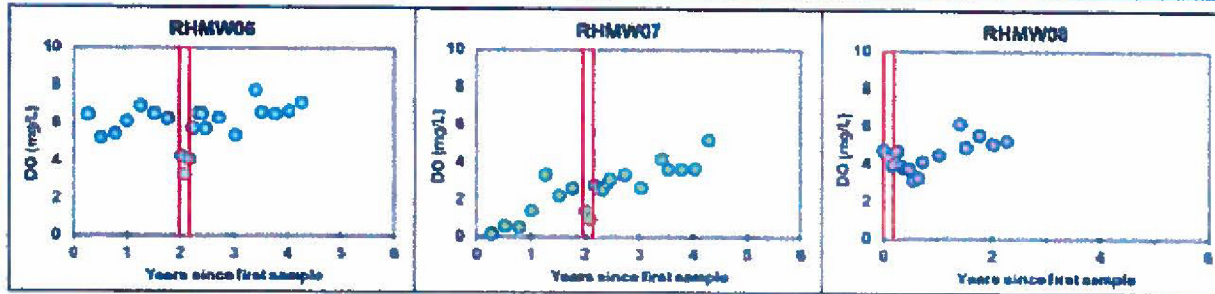
Dissolved Oxygen Concentration vs. Time Since Installation for Three Facility Monitoring Wells Drilled Near Saprolite Zones. RHMW06 and RHMW07 were Completed in Oct. 2014; RHMW08 in Oct. 2015.
