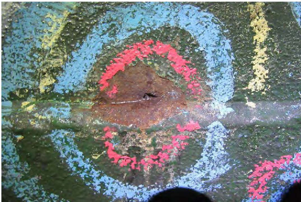
Photo 9: Liner damage in extension ring plate in course 2. The area was corroded and included coating failure at the margins. No evidence of cut marks or gouges was observed.
