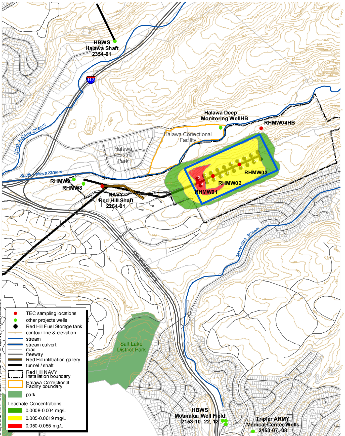
Figure 4-3 Benzene Contours for the Maximum Leachate Scenario Red Hill Fuel Storage Facility Oahu, Hawaii 0 255 510 Meters 0 380 760 1,520 Feet N S000933
