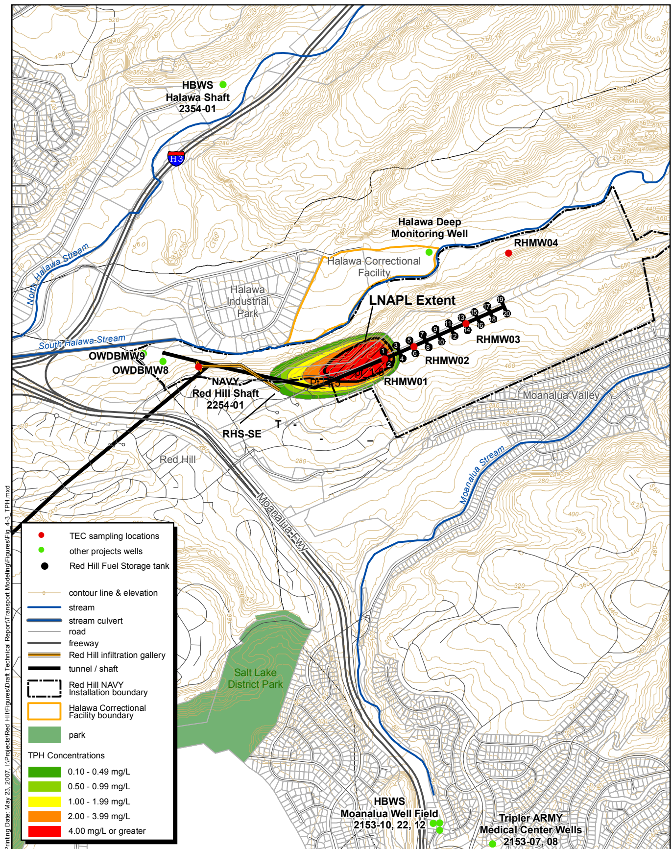
Figure 4-4 TPH Contours for the Exceedance Scenario Red Hill Fuel Storage Facility Oahu, Hawaii 0 255 510 0 375 750 1,500 Meters Feet N S000934
